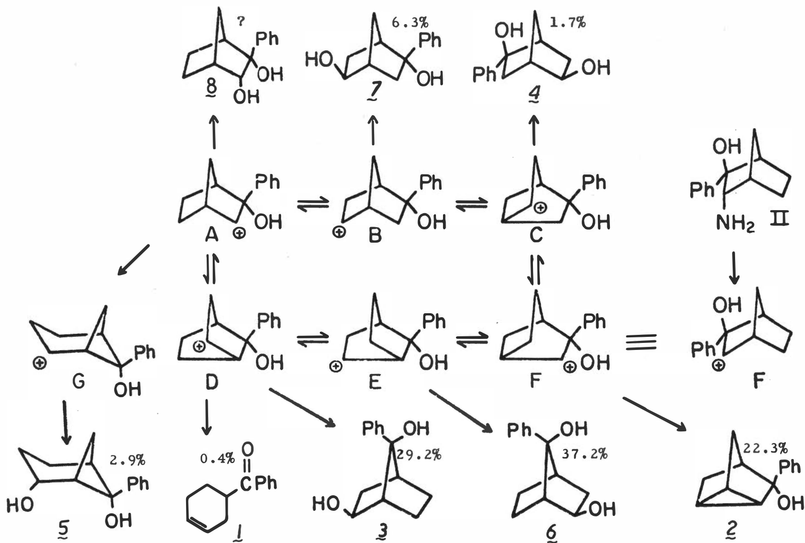
Figure 29. Yields from amine II; 2-exo-hydroxy-2-phenyl-3-endo-aminonorbornane.
