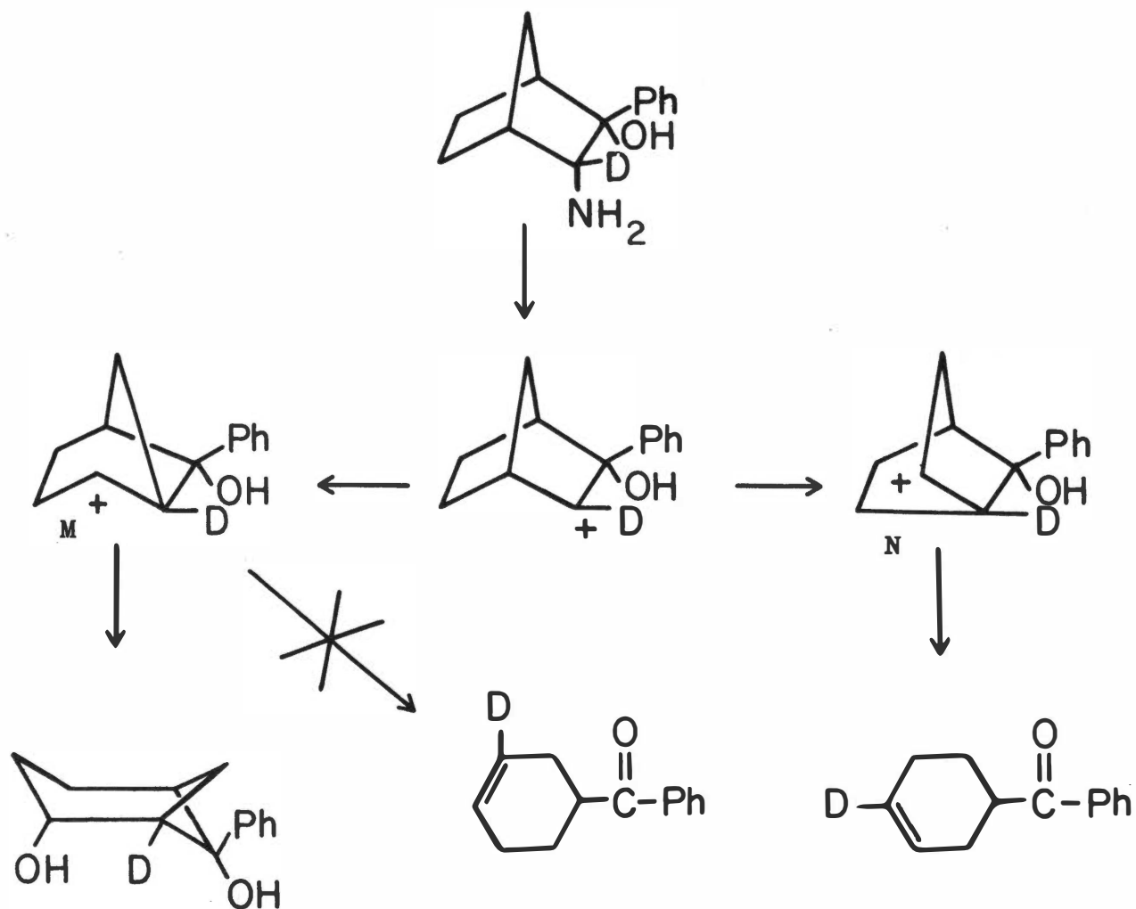
Figure 26. Formation of cyclohexenyl phenyl ketone.
