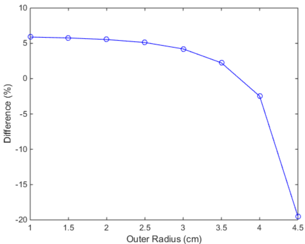
Figure 4-10. Differences between actual and calculated ^{240}\text{Pu} content plotted against varying Pu spherical shell outer radii.
