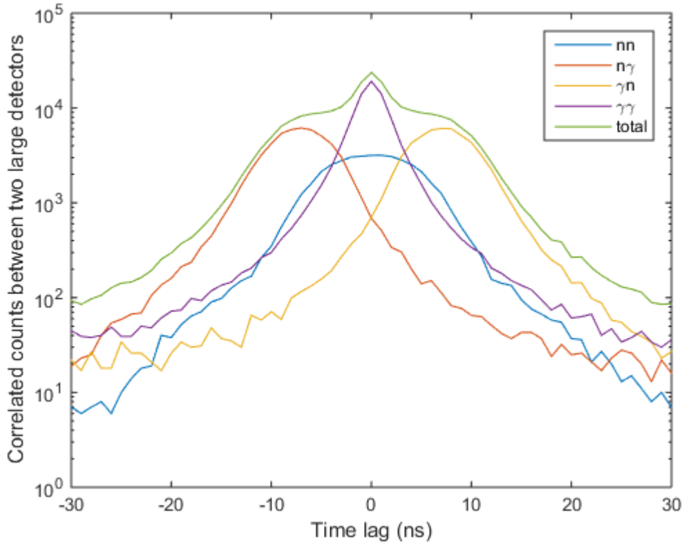
Figure 1-5. Example of time distribution of cross-correlated events for a spherical shell, including regions containing primary gamma pairs, neutron-neutron pairs, neutron-gamma pairs and gamma-neutron pairs. In this system, gammas are distinguished from neutrons only based upon time of flight.
