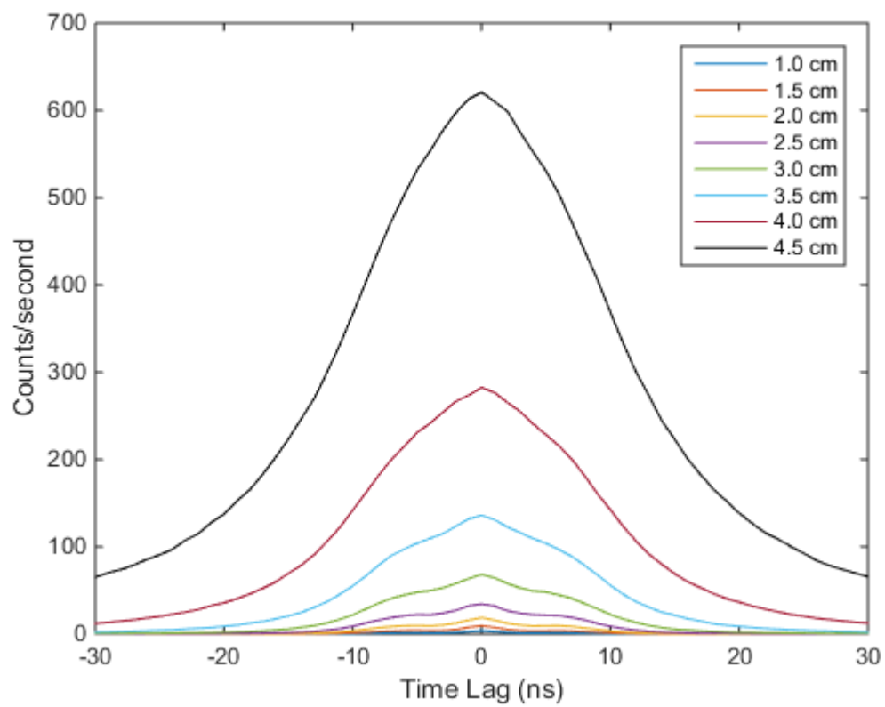
Figure 4-9. Simulation of time correlated distributions for various outer radii for an alpha-phase Pu sphere.
