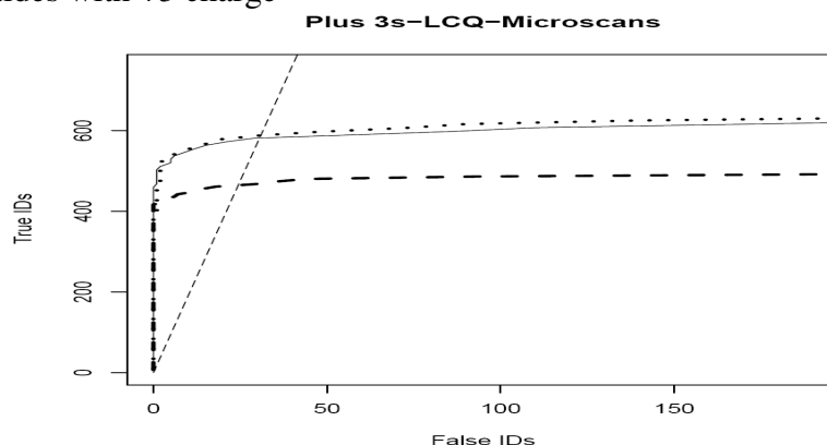
Figure 2. 6 ROC curves of pooled LCQ EPSM microscan data
