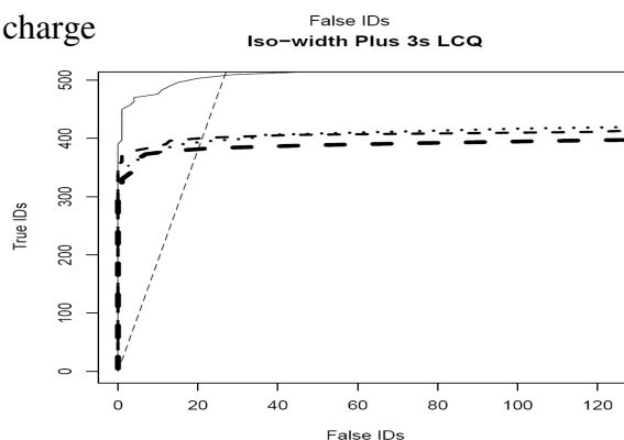
Figure 2. 4 ROC curves of LCQ isolation width EPSM data
