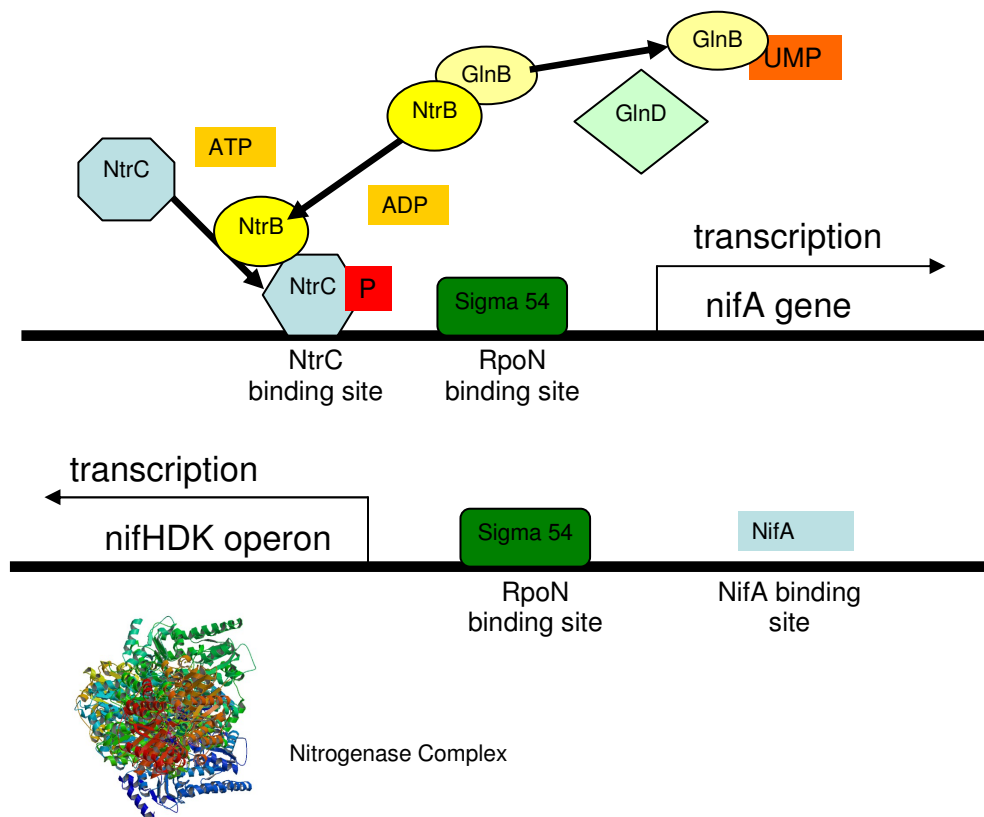
Figure 1. 5 Levels of regulation in expression of nitrogenase structural proteins and related synthesis proteins
