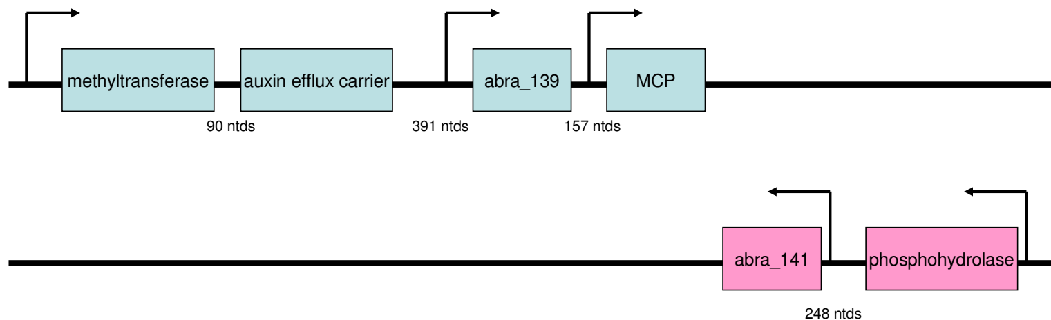
Figure 3. 4 Schematic representation of genomic region surrounding Abra_0139 and Abra_0141
