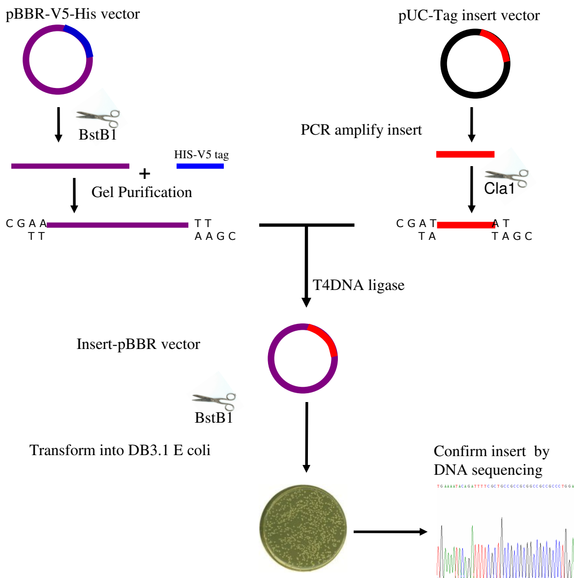
Figure 5. 1 Flow chart of vector construction steps
