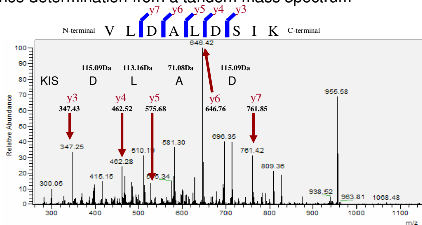
Figure 1. 2 Creation of fragment ions in tandem mass spectrometry A) CID energy transfer process, B) Fragmentation patterns of peptides C) MS/MS spectra of peptide VLDALDSIK from carbonic anhydrase.
