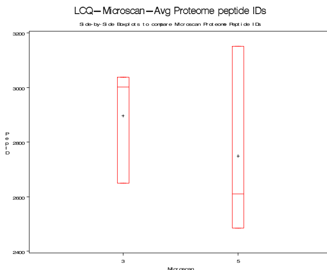
Figure 2. 7 Box plot representation of statistical results from pooled LCQ proteome microscan data Data from 6 individual replicates was analyzed via one-way ANOVA and means and standard deviation determined. The x-axis represents the number of MS/MS microscans (either 3 or 5) tested on LCQ proteome samples. The box encloses two standard deviations within the data range, while the star in the center represents the mean, and the line represents the median. A) Mean numbers and standard deviation of total numbers of protein identifications. B) Mean numbers and standard deviation of total numbers of peptide identifications. Statistical analysis showed that there is no significant difference between the groups in the numbers of protein ( p = 0.2046 ) or peptide ( p = 0.5711 ) identifications obtained when proteome samples are tested.
