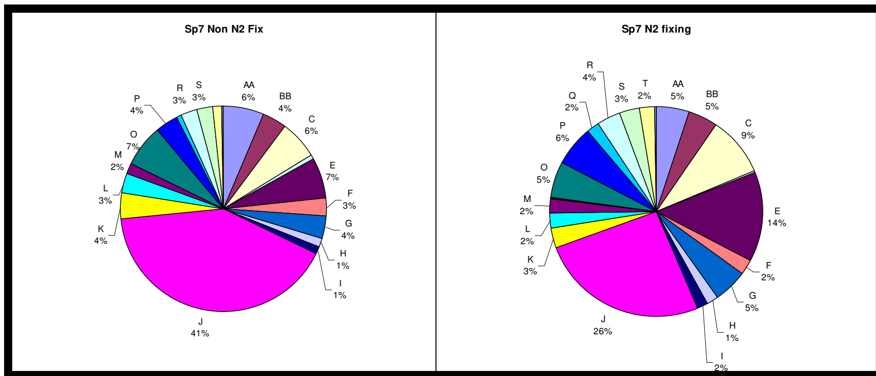
Figure 3. 2 Sp7 protein expression by functional category in A) Sp7 optimal growth controls and B) Sp7 nitrogen fixing cultures
