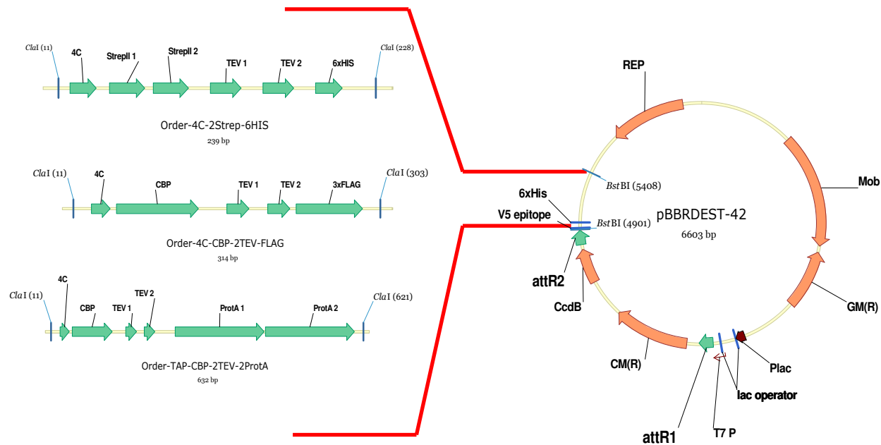
Figure 5. 3 New set of pBBR-Dest42-based vectors showing expansions of the three new C-terminal tag constructs
