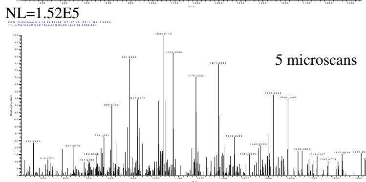
Figure 2. 3 Representative fragmentation spectra from peptide sequence derived from protein concanavalin A collected using different microscans
