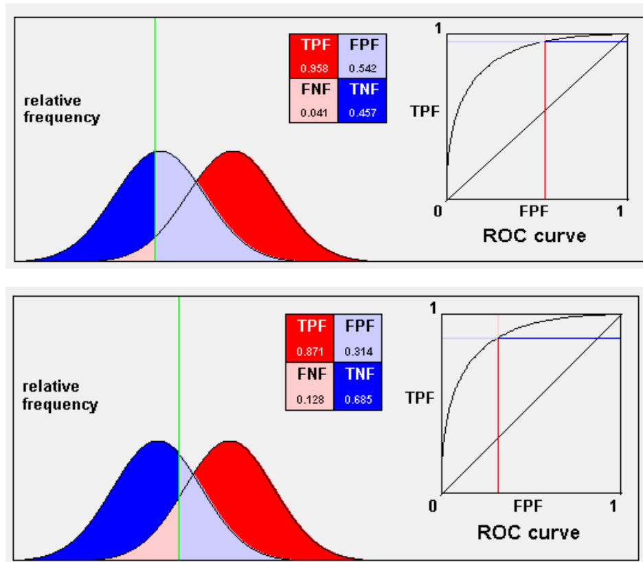
Figure 2. 10 Development of an ROC curve (Adapted from http://www.anaesthetist.com/mnm/stats/roc/ )
