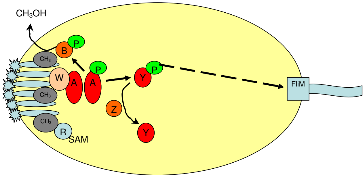
Figure 1. 6 Prototypical chemotaxis pathway in E. coli
