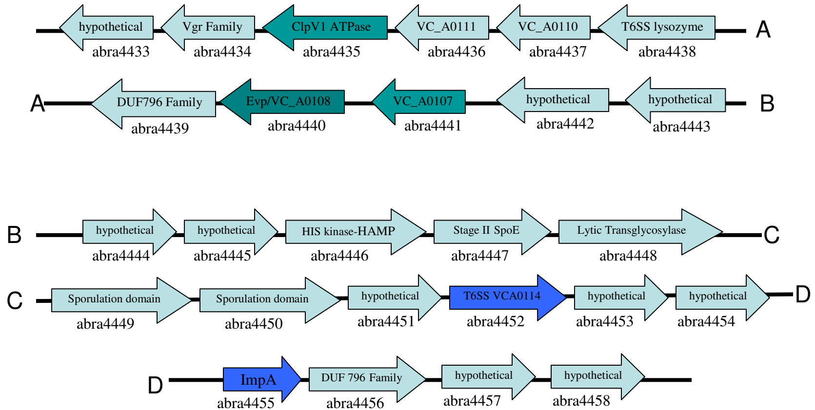
Figure 4. 5 Schematic representation of extended genomic region surrounding the type VI secretion system components in the Sp245 genome
