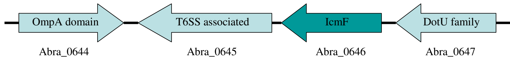
Figure 4. 4 Schematic depiction of genomic region containing type VI secretion system homologs to IcmF (abra_0646) and and DotU (abra_0647) Abra0645 is a type VI secretion associated protein of the BMA_A0400 family, while abra_0646 is an IcmF homolog, and abra_0647 is a DotU family homolog. Abra_0646 IcmF homolog is upregulated in CheY1 mutants, but not in Sp7 or in CheB1CheR1 mutants. IcmF homologs contain a transmembrane domain and a Walker A nucleotide binding motif, while DotU-like proteins contain a transmembrane segment in the C-terminal end, often with C-terminal extensions that show similarity to OmpA proteins. T6SS secretory apparatus are thought to function through association of IcmF and DotU family homologs.
