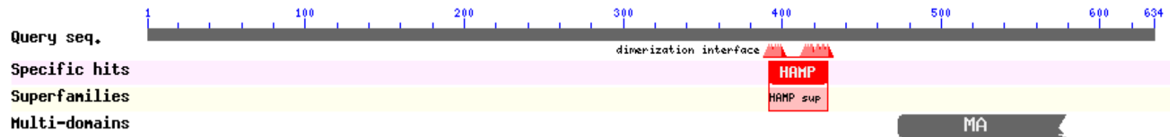
Figure 4. 3 BLASTp depiction of conserved domains in abra_6288
