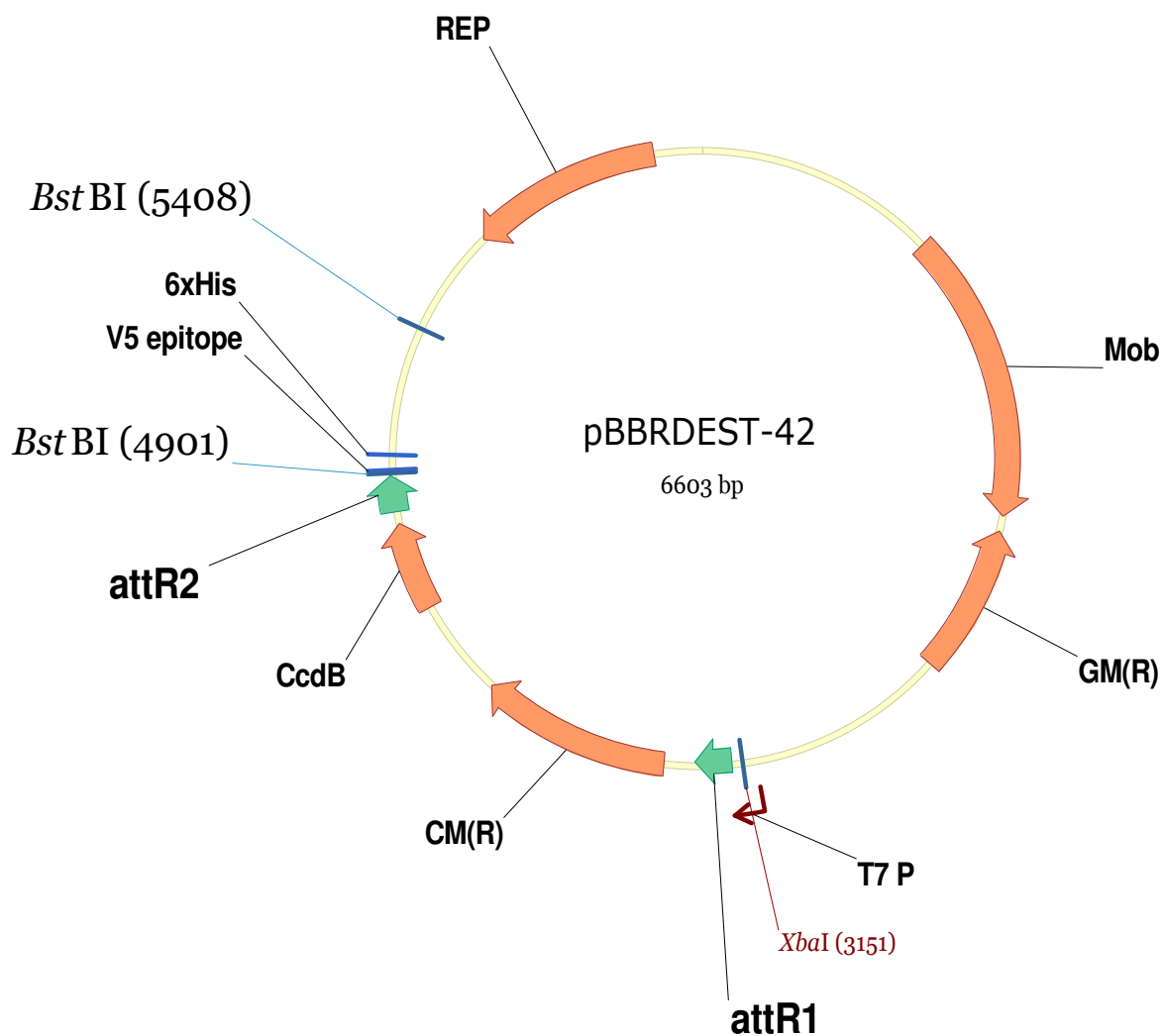
Figure 5. 2 Schematic drawing of the initial pBBR-Dest42 parent vector
