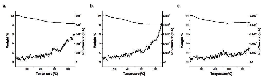
Figure 31. TGA-MS plots showing respective ion currents ( m/z=44 ) for a) BN1, b) BN2, and c) BN3
