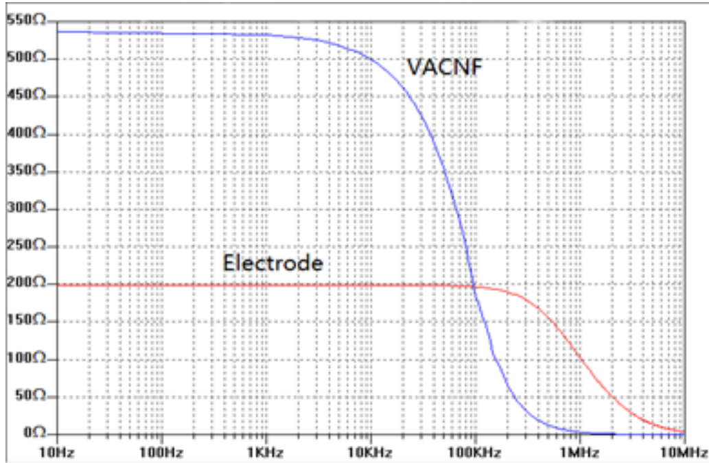
Figure 22. Impedance difference with cell and without cell for VACNF model coplanar electrode model
