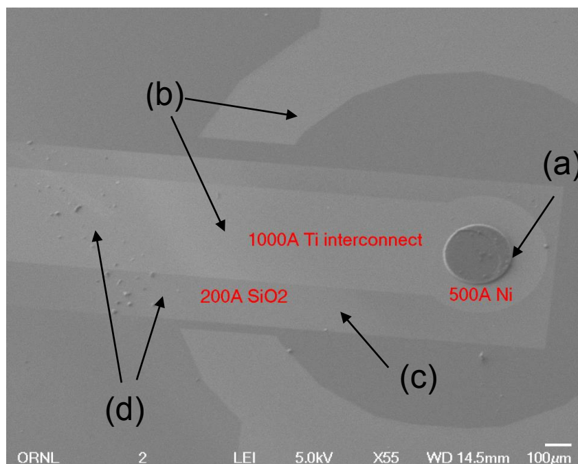
Figure 13. Image of a single VACNF measurement unit with passivation layer (a) VACNF, (b) interconnection (c) passivation layer (d) Cr particle
