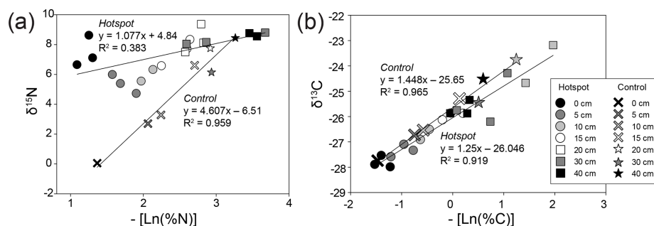
Figure 6. Bulk soil stable isotopic composition and corresponding negative natural log % N (a) and % C (b) for hotspot and control soils with depth. Linear regressions were fit to hotspot and control datasets.
