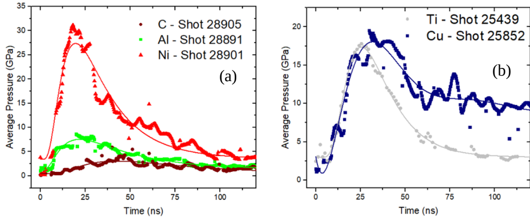
Figure 4.4: Inferred plasma pressures for targets of (a) Al, Ni, C, and (b) Ti, and Cu. All foils are 100- \mu m-thick.
