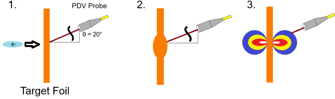
Figure 3.2: Illustration for target heating and PDV measurement.
