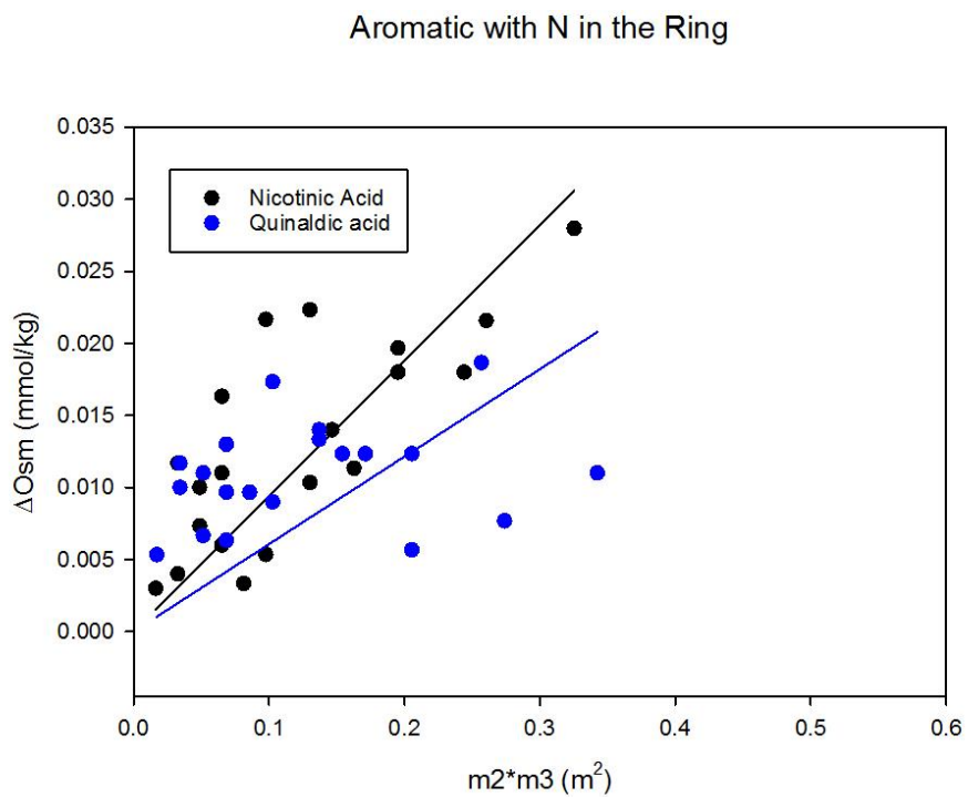
Figure 9. Graph of \Delta\text{Osm} versus m_2 \cdot m_3 for aromatic compounds with nitrogen in the ring and their corresponding linear fits.
