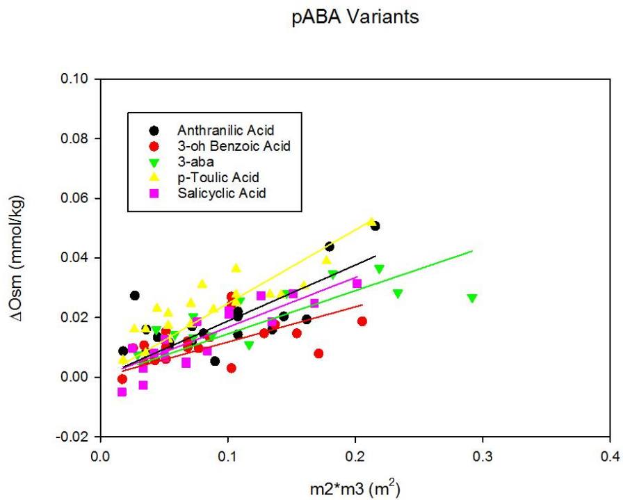
Figure 8. Graph of \Delta\text{Osm} versus m_2 \cdot m_3 for pABA variants and their corresponding linear fits.
