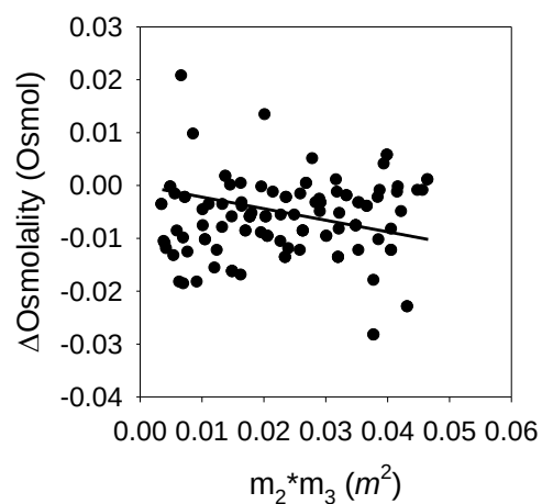
Figure 3. Preferential interaction graph for trehalose and folate. The preferential interaction coefficient was found to be -0.165 \pm 0.044 \text{ m}^{-1} meaning that folate preferentially interacts with trehalose over water (Unpublished data Nambiar, Arrieta, 2016).
