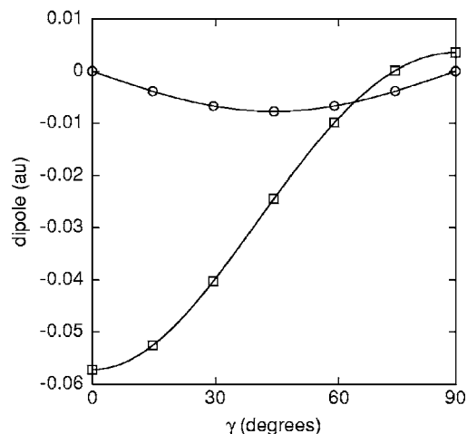
FIG. 2. Dependence of the frozen-core Ar–H 2 dipole moment on \gamma at R=5\ a_0 and r=1.4\ a_0 . The open circles indicate values of M_{FC,x} ; the open squares indicate values of M_{FC,z} . The lines are fits to truncated Legendre polynomial expansions [Eqs. (1) and (2)] as described in the text.
