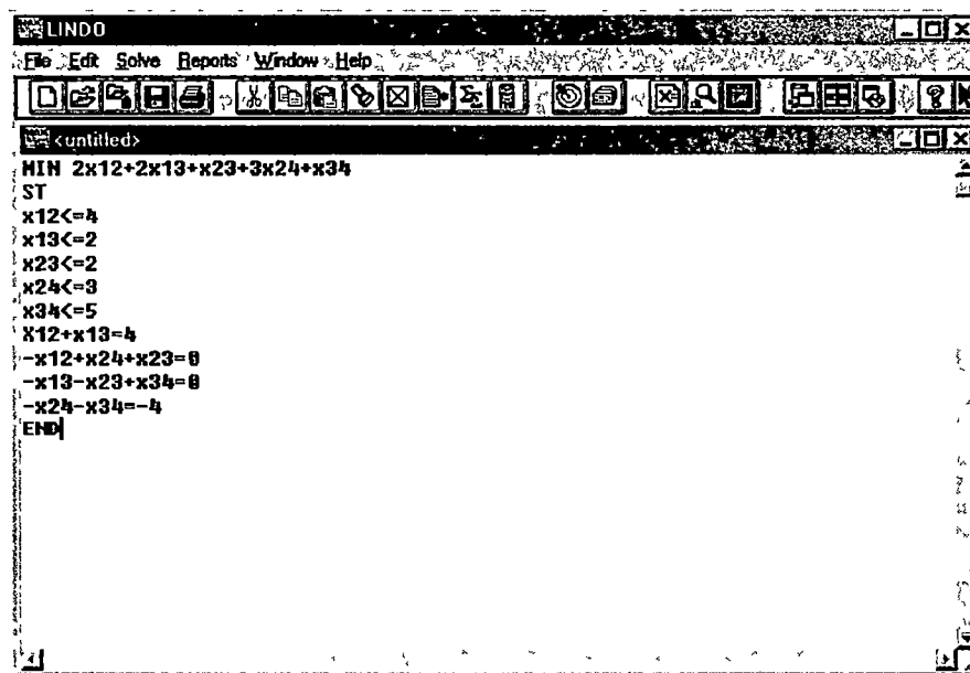
Figure 5.3.10 LP Formulation of MCF Problem
