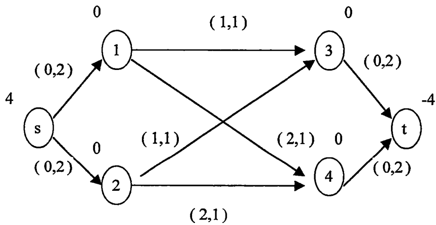
Figure 5.3.9 New Network after Transformation
