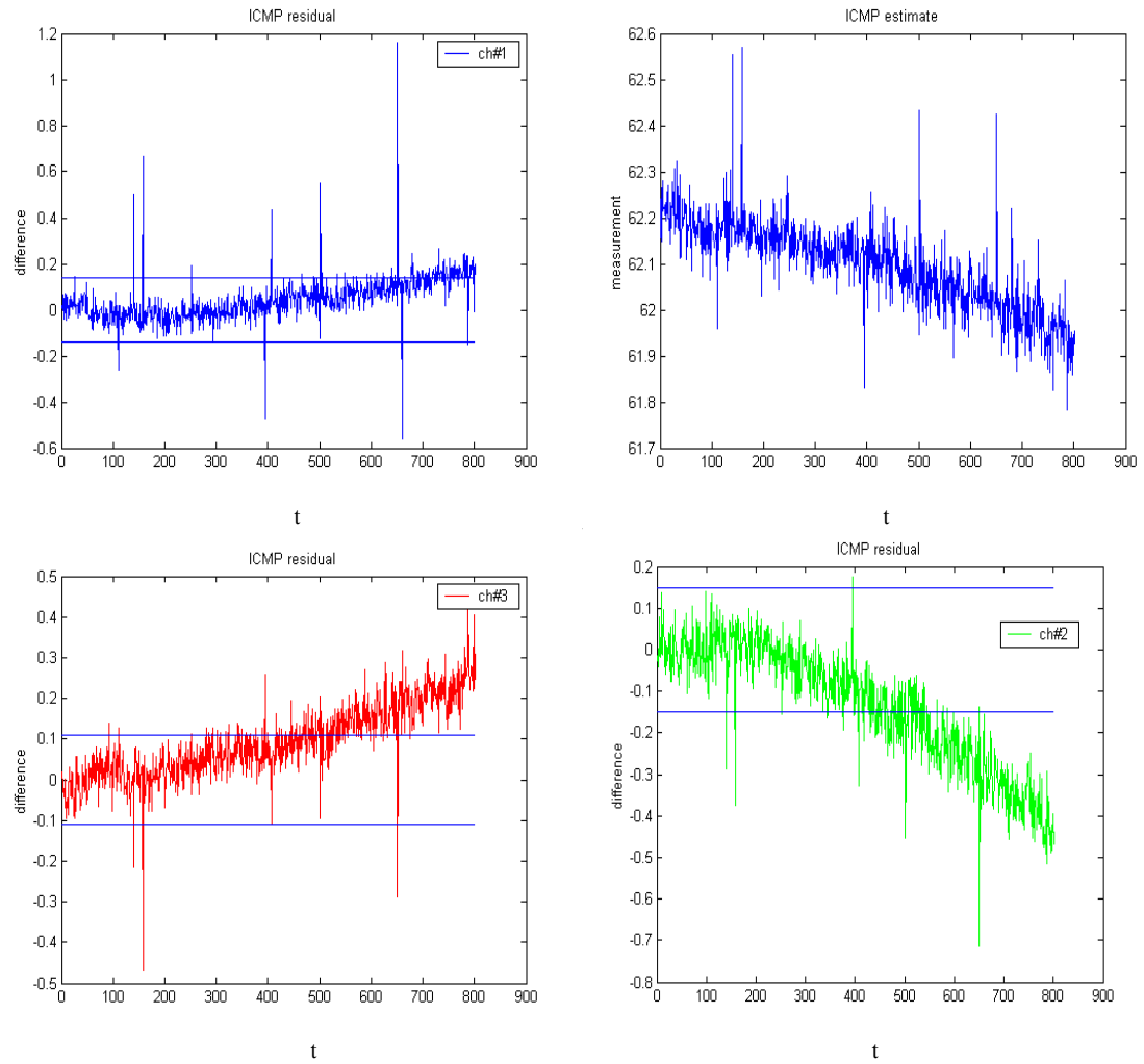
Figure 4.7. ICMP results for drift detection.
