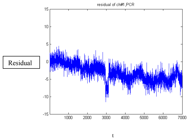
Figure 4.37. Channel 1 residual plot.
