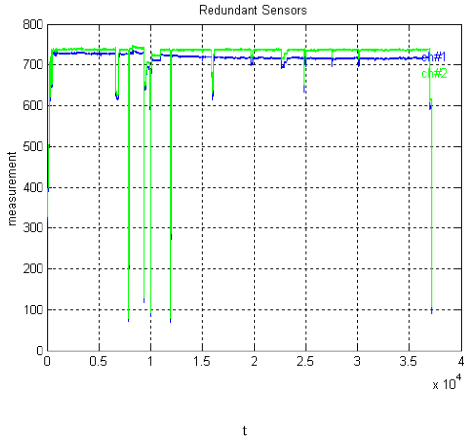
Figure 4.33. Turbine first stage pressure.
