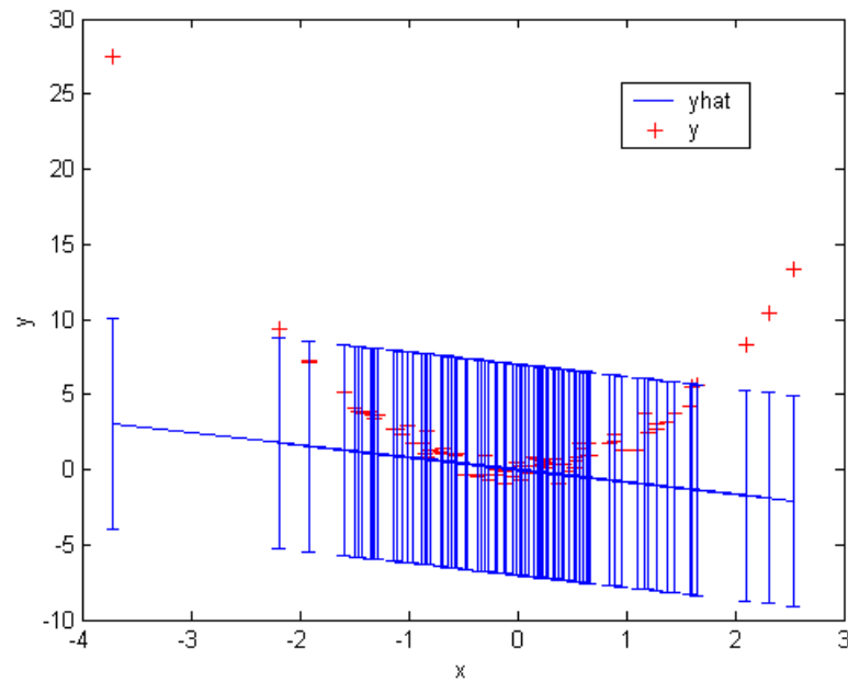
Figure 5.7. 95% prediction interval for a biased model
