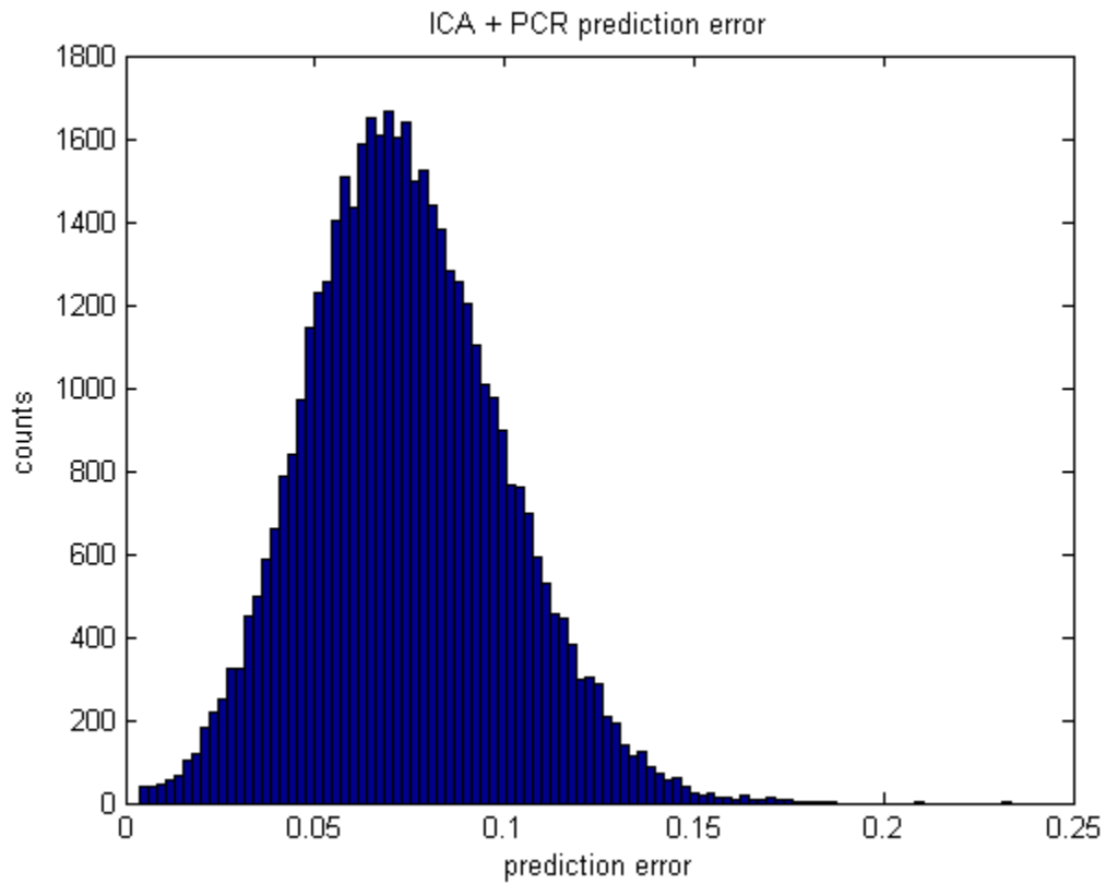
Figure 5.16 Histogram of bootstrap prediction error for ICA + PCR hybrid model.
