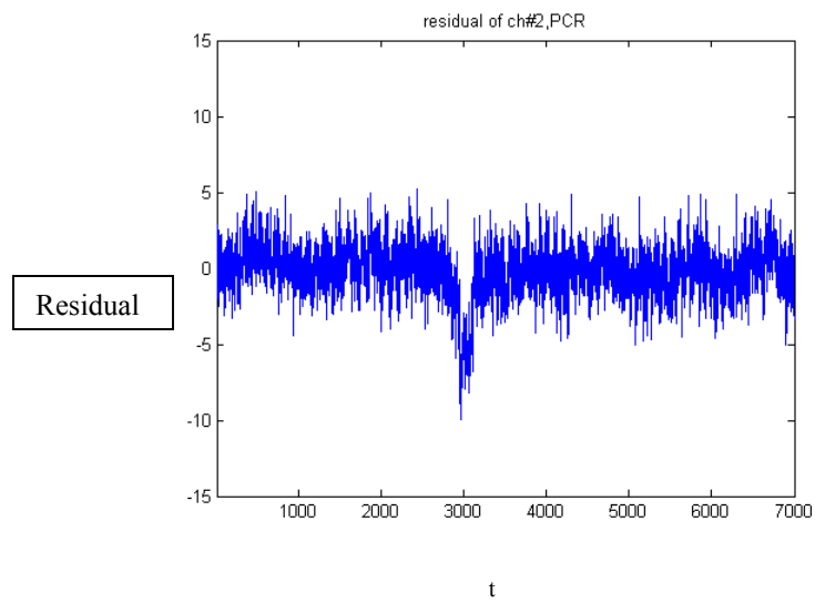
Figure 4.38. Channel 2 residual plot.
