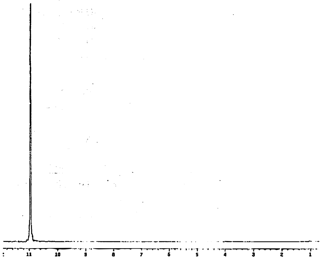
Figure 2.3: ^1\text{H} NMR spectrum for \text{FSO}_3\text{H} .
