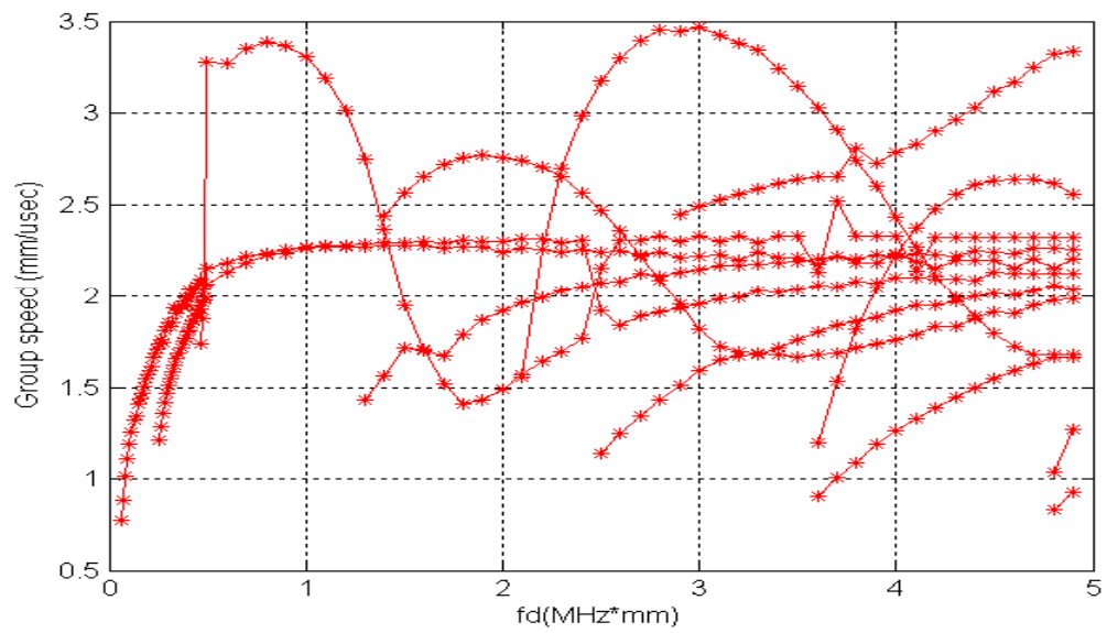
Figure 3.11. The third circumferential order flexural modes in a brass tube: (a) phase speed; (b) group speed.
