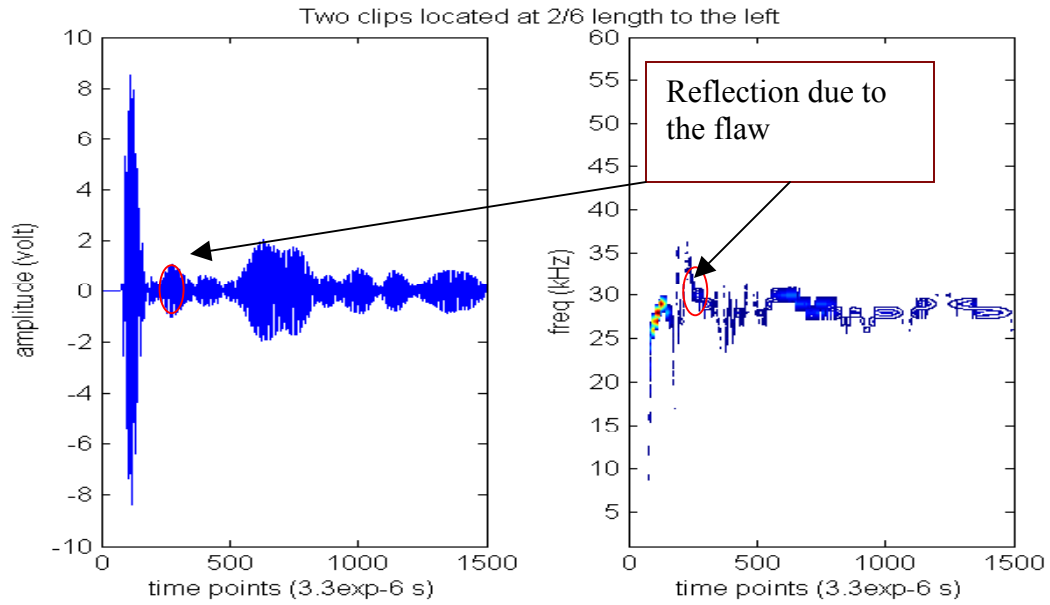
Figure 6.9. Lamb wave signal from an aluminum beam with two clips located at 2/6 th of the length near the left end and its HHT.
