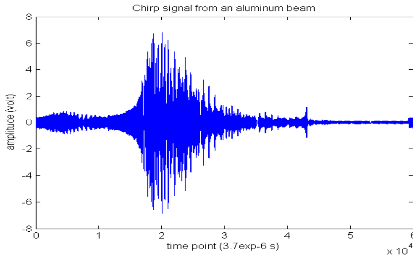
Figure 6.16. Chirp signal scanning a wide band from 100 to 90k Hz.
