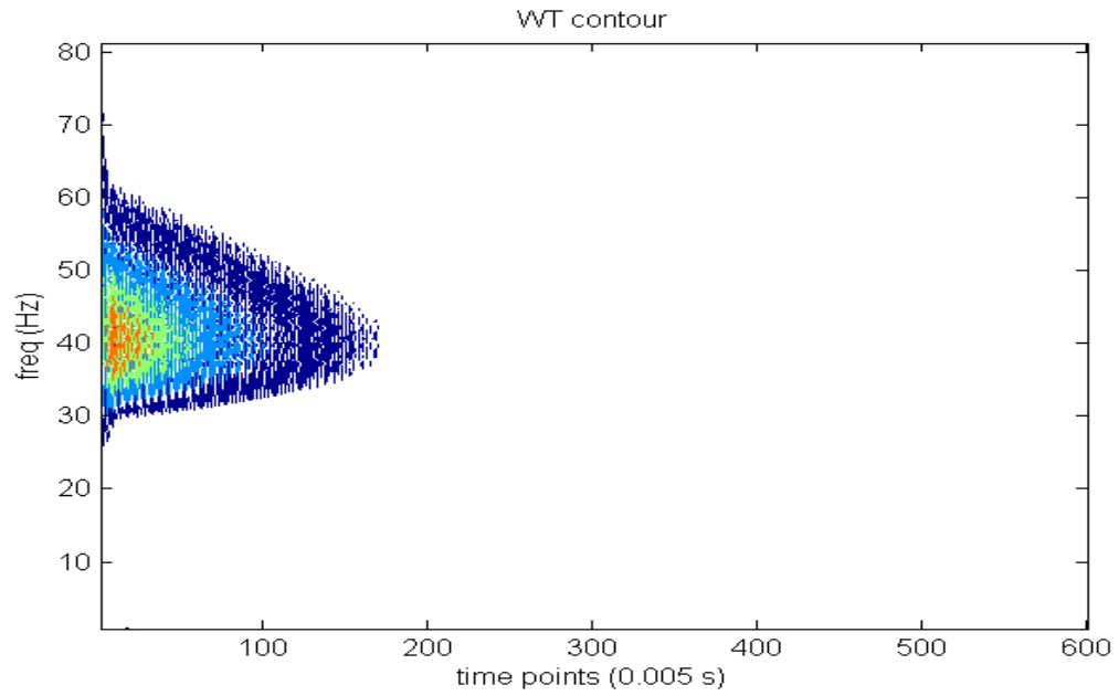
Figure 4.6(c). WT of amplitude-modulated signals.
