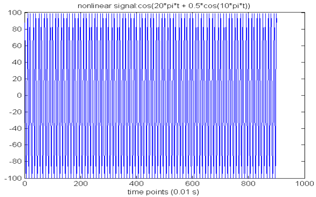
Figure 4.7(a). Nonlinear signal defined by 100 \cdot \cos(20\pi t + 0.5 \cdot \cos(10\pi t)) .
