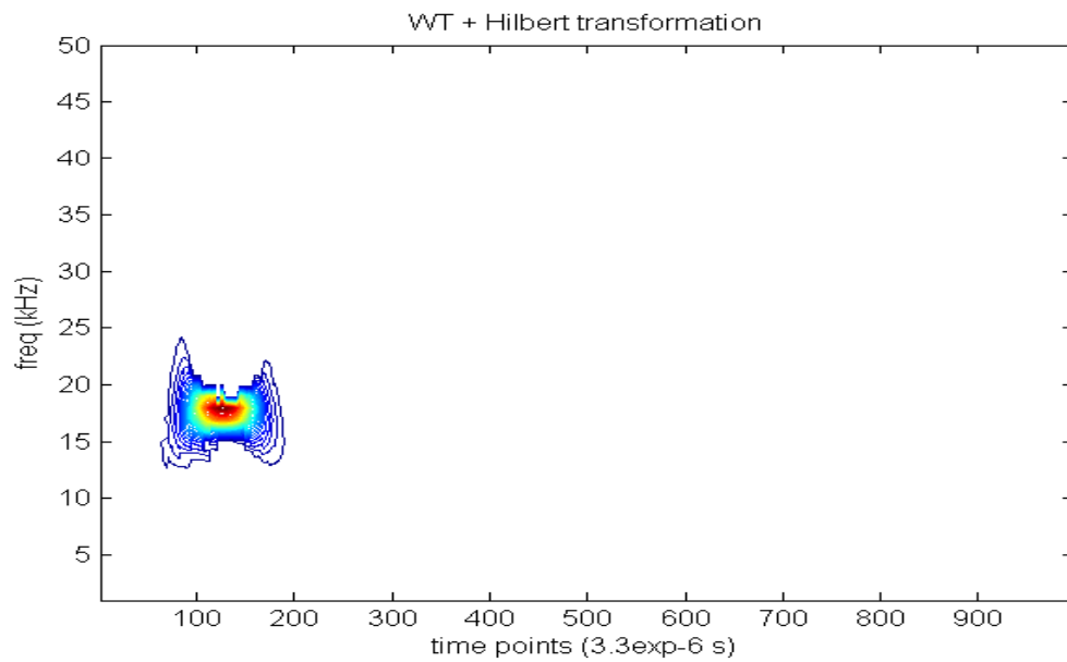
Figure 4.5(d). WT + Hilbert transform can improve the concentration of instant frequency.
