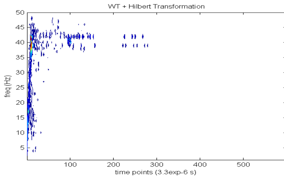
Figure 4.6(d). WT + Hilbert transform for amplitude modulated signals.
