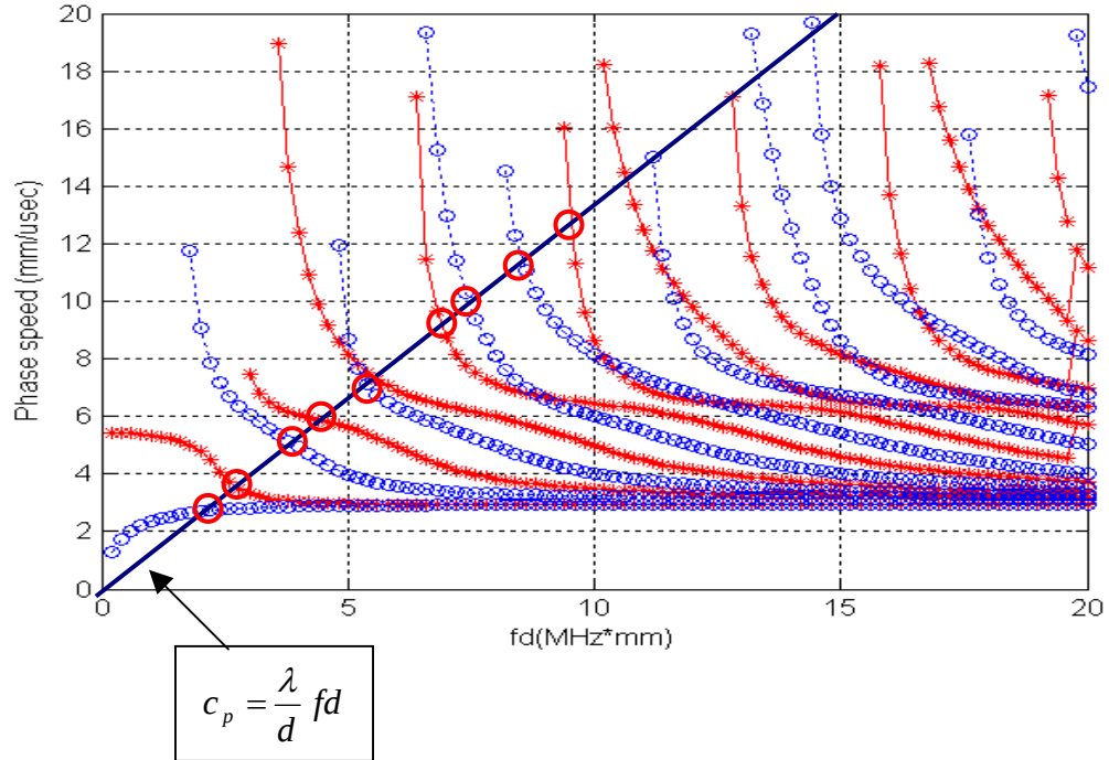
Figure 2.7. The resonant frequency is decided by slot width d and the Lamb wave mode.
