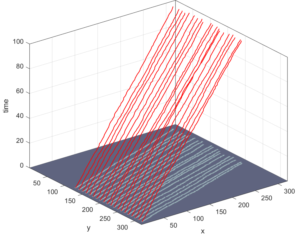
Figure 3.5: Case I: The frame size is 320 by 320 pixels. Trajectories of 20 organelles are in red spanning from time t = 0 s to t = 99 s. Their motion is described by a diffusion process containing both a diffusion and a drift term. The starting distance of any two adjacent organelles at t = 0 s is 10 pixels.
