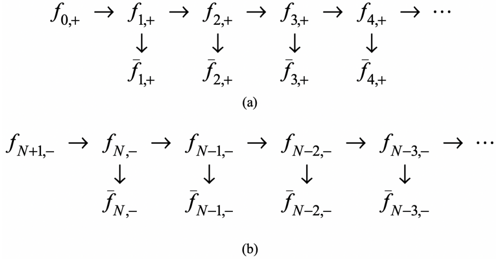
Figure 3.3: The relations of forward fields and backward fields are indicated here. (a) shows the approach depiction of forward displacement fields, (b) shows the approach depiction of backward displacement fields. For clarity, time marches forward in (a) and backward in (b).
