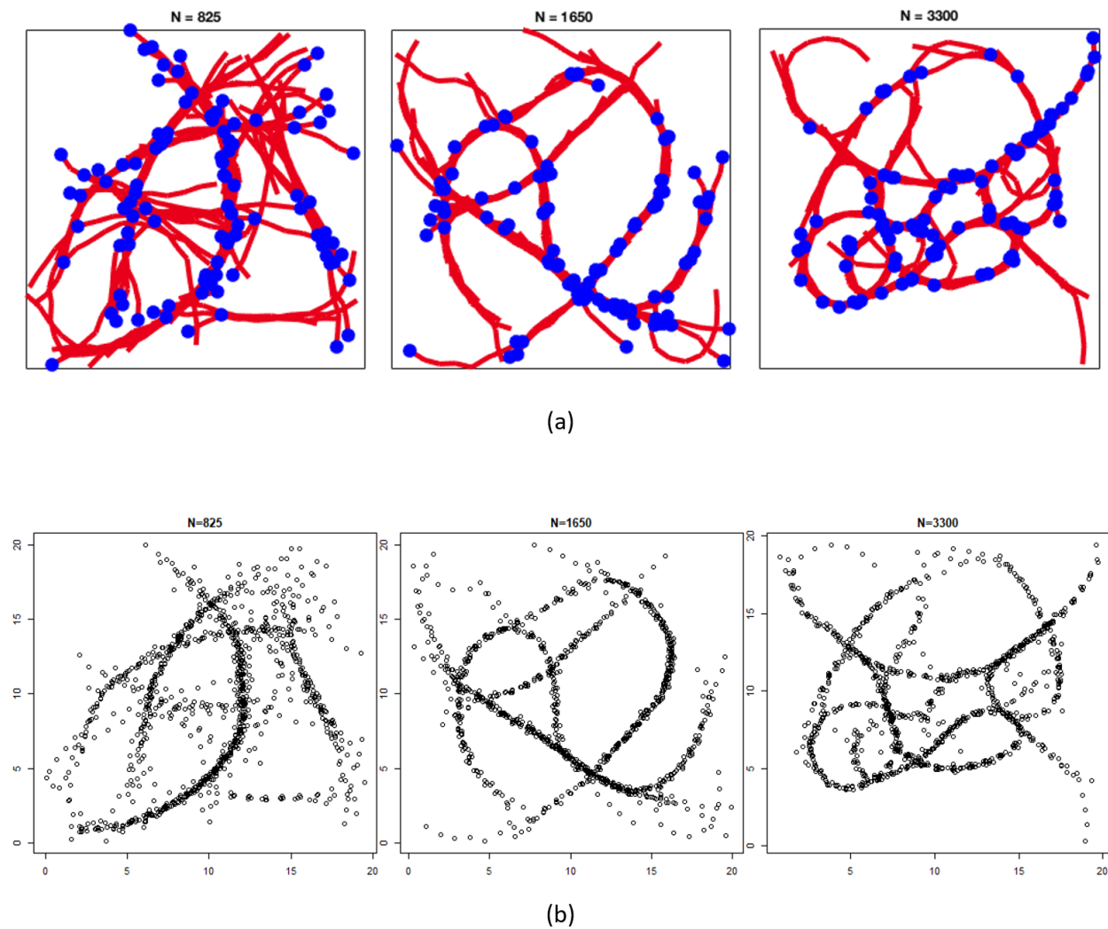
Figure 4.1: Filament networks. Panel (a) shows three filament networks generated by 825, 1650 and 3300 cross-linkers, respectively, in a 20\text{ }\mu\text{m} \times 20\text{ }\mu\text{m} area. Each network contains 100 filaments which are represented as red lines. The blue dots are the barbed ends of these filaments. Panel (b) shows the locations of the actin beads that make up the filaments exhibited in Panel (a).
