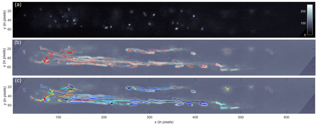
Figure 3.13: Case III: Panel (a) is the first frame of the video. Panel (b) exhibits all estimated trajectories in red. Panel (c) further shows each estimated trajectory in different colors.
