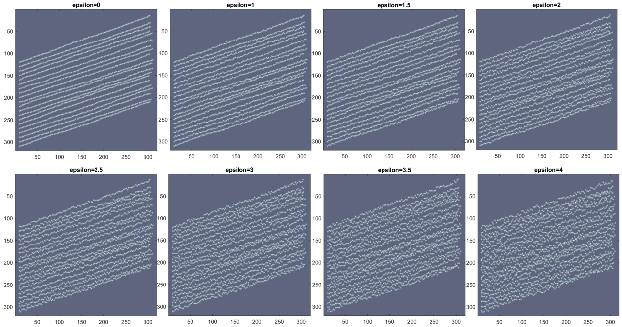
Figure 3.8: Case I: Positions of organelles over time after adding perturbation U(-\epsilon, \epsilon) when \epsilon = 0, 1, 1.5, 2, 2.5, 3, 3.5, 4 pixels, respectively. If \epsilon increases, it is more difficult to detect trajectories, especially, when \epsilon = 4 pixels, there are no clear patterns for all trajectories to be reconstructed.
