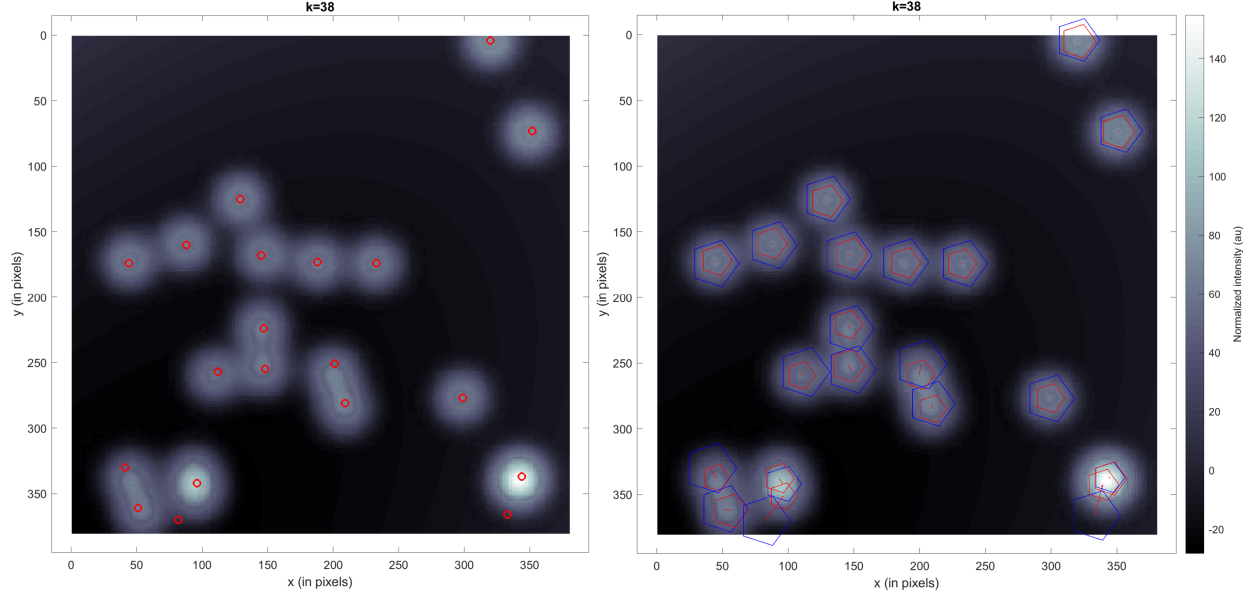
Figure 3.9: Case II: The left shows the rough detection result, the right show the locations after correction. The red dots in the left penal and blue pentagons in the right penal are the original locations before Bayesian identification. The red pentagons in the right panel are the fitted location after Bayesian identification.
