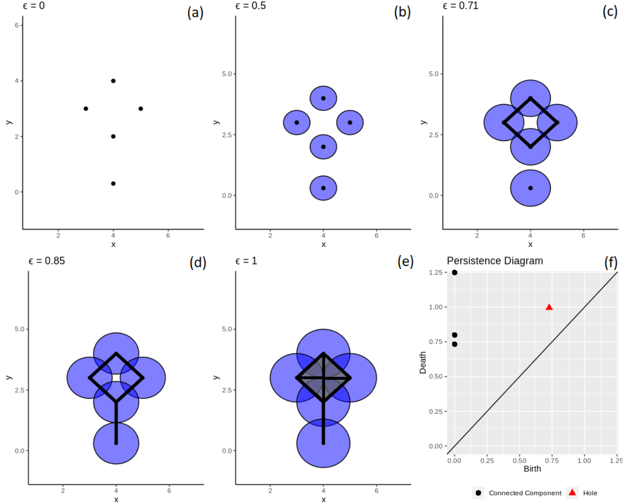
Figure 2.3: Approach depiction of making persistence diagram. Beginning from \epsilon = 0 , there are five components in Panel (a). When \epsilon = 0.5 , five components stay alive in Panel (b). In Panel (c), when \epsilon = 0.71 , four components connect into one connected component, forming a hole, thus three components die and one hole is born. In Panel (d), when \epsilon = 0.85 , the two components further merge into one, therefore, one more component dies. Finally, when \epsilon = 1 , the only one hole dies but the only one connected component survives in Panel (e). No additional homological change while \epsilon is grown to 1.25. Panel (f) summarizes the persistent homology as a persistence diagram.
