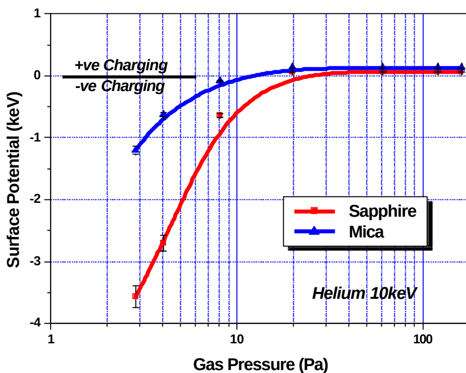
Figure 3.20 Surface potential on sapphire and mica varies as a function of gas pressure by 10keV beam irradiation within helium atmosphere. The acquisition time for the x-ray spectrum was 100 seconds. The plate electrode of the SE detector is in SSE mode. The magnification is 90 \times . Working distance is 12mm. No objective aperture.
