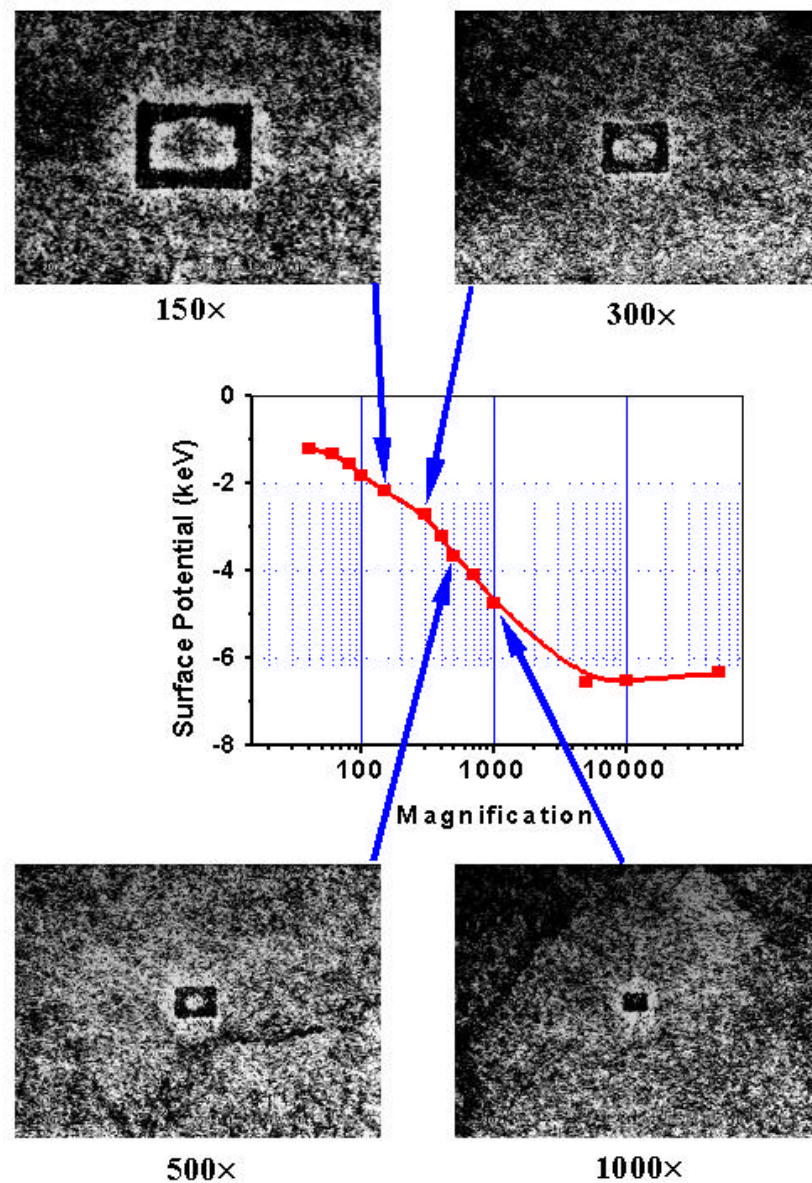
Figure 5.3 Variation of the toner powder patterns with magnification. Quartz substrate was irradiated by 15keV electron beam in 5Pa air. Magnification varies as 150×, 300×, 500×, and 1000×, scanning rate TV1 16ms/frame, duration time 30seconds. The resulting patterns were observed by a 10keV electron beam, magnification 40×, and 15Pa air. Center is the relationship of surface potential, magnification (dose density) in 5Pa air environment on quartz surface. Incident beam energy is 15keV, working distance 12mm.
