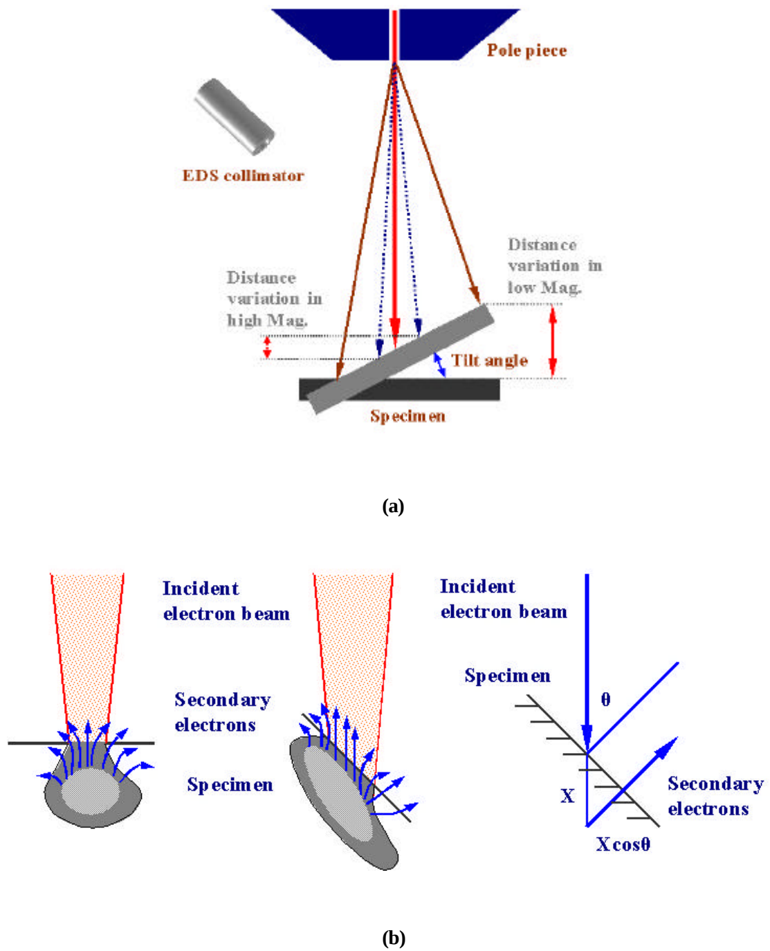
Figure 3.30 Schematically draw the sample tilt set up (a) The amount of secondary electrons generated depends on the specimen tilt angle (b)
