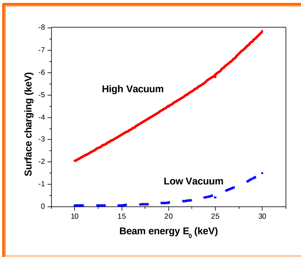
Figure 2.1 The experimental dependence of incident beam energy and surface charging in vacuum and fixed gas pressure for mica (4×2×0.2cm). The acquisition time for the x-ray spectrum was 100 seconds. The electric resistivity of mica is 1\text{E}+16\Omega\cdot\text{m} (CRC materials Science and Engineering Handbook). The plate electrode of the SE detector is present inside the chamber with 250volts bias voltage in standard SE mode (SSE).
