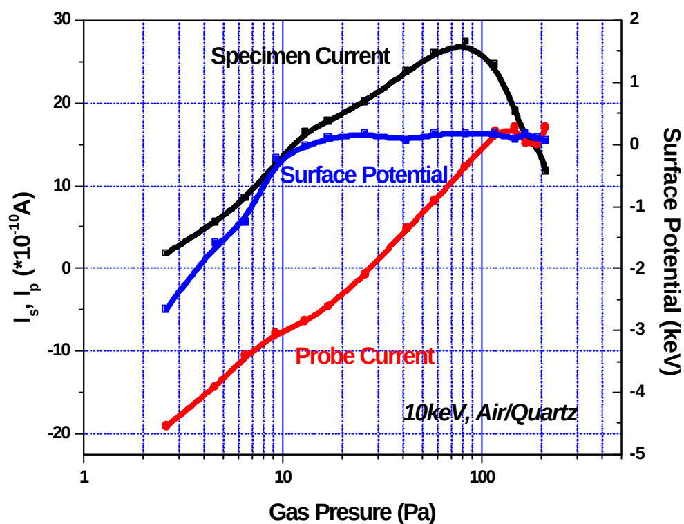
Figure 3.46 The relationship of specimen current, primary current, and surface potential as the function of air pressure on quartz by 10keV beam irradiation. The plate electrode of the SE detector is in SSE mode.
