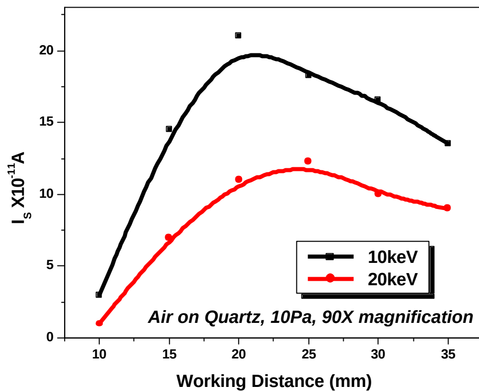
Figure 3.36 Schematically show the relationship of working distance and sample current on quartz in 10Pa air environment by 10 and 20keV beam irradiation. Magnification is 90×. The plate electrode of the SE detector is in SSE mode.
