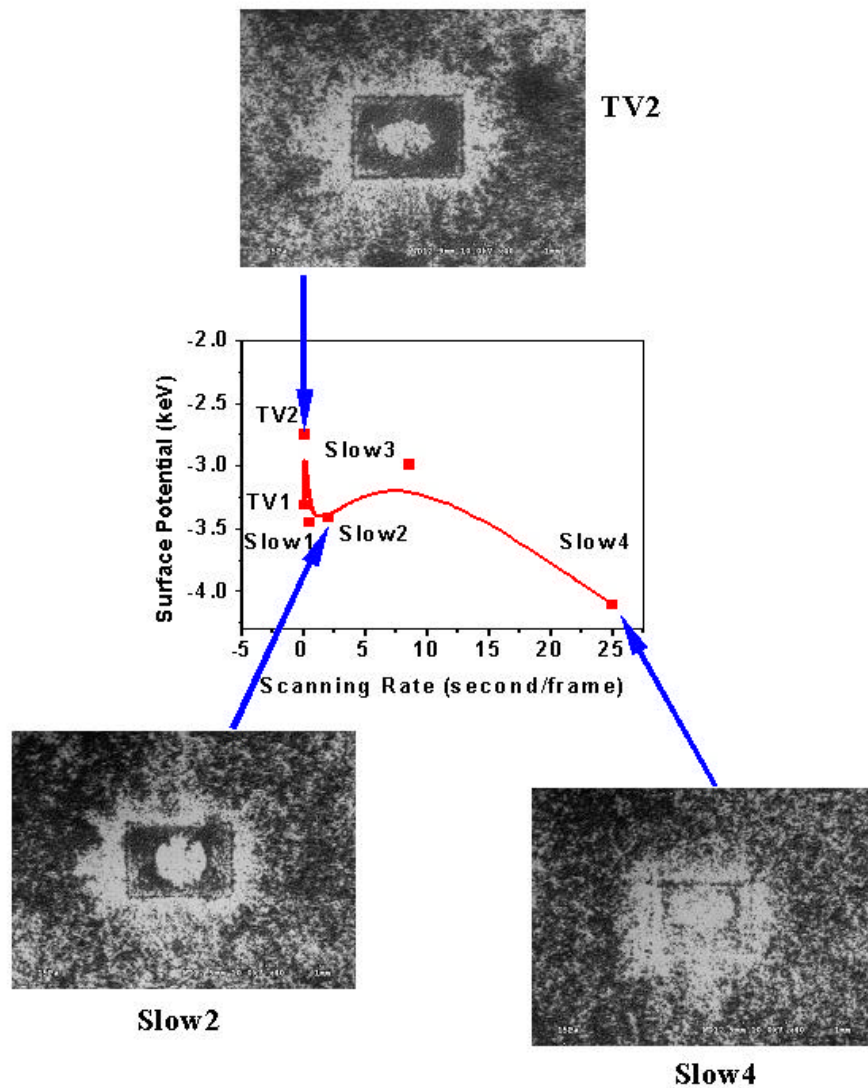
Figure 5.5 Variation of the toner powder patterns with scanning speed. Quartz substrate was irradiated by 20keV electron beam in 5Pa gas with magnification 150 \times . The scanning rates are TV2-33ms/frame, Slow2-2s/frame, and Slow4-25s/frame at 60Hz. Scanning time 30seconds. The resulting patterns were observed by a 10keV electron beam, magnification 40 \times , and 15Pa air. Center is the relationship of surface potential and scanning speed in 5Pa air environment on quartz surface. Incident beam energy is 20keV, working distance 13mm.
