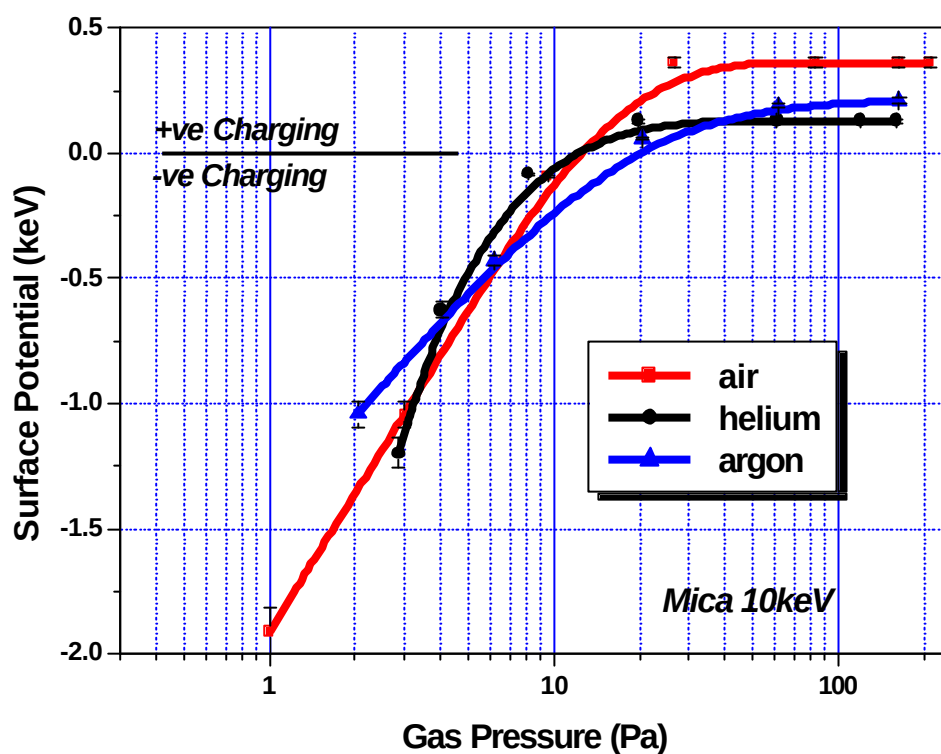
Figure 3.10 The charging potentials vary with gas pressure inside the gaseous environment of air, helium, and argon on mica by 10keV beam irradiation. The acquisition time for the x-ray spectrum was 100 seconds. The plate electrode of the SE detector is in SSE mode (250 volts). No objective aperture. The magnification is 90 \times . Working distance is 12mm.
