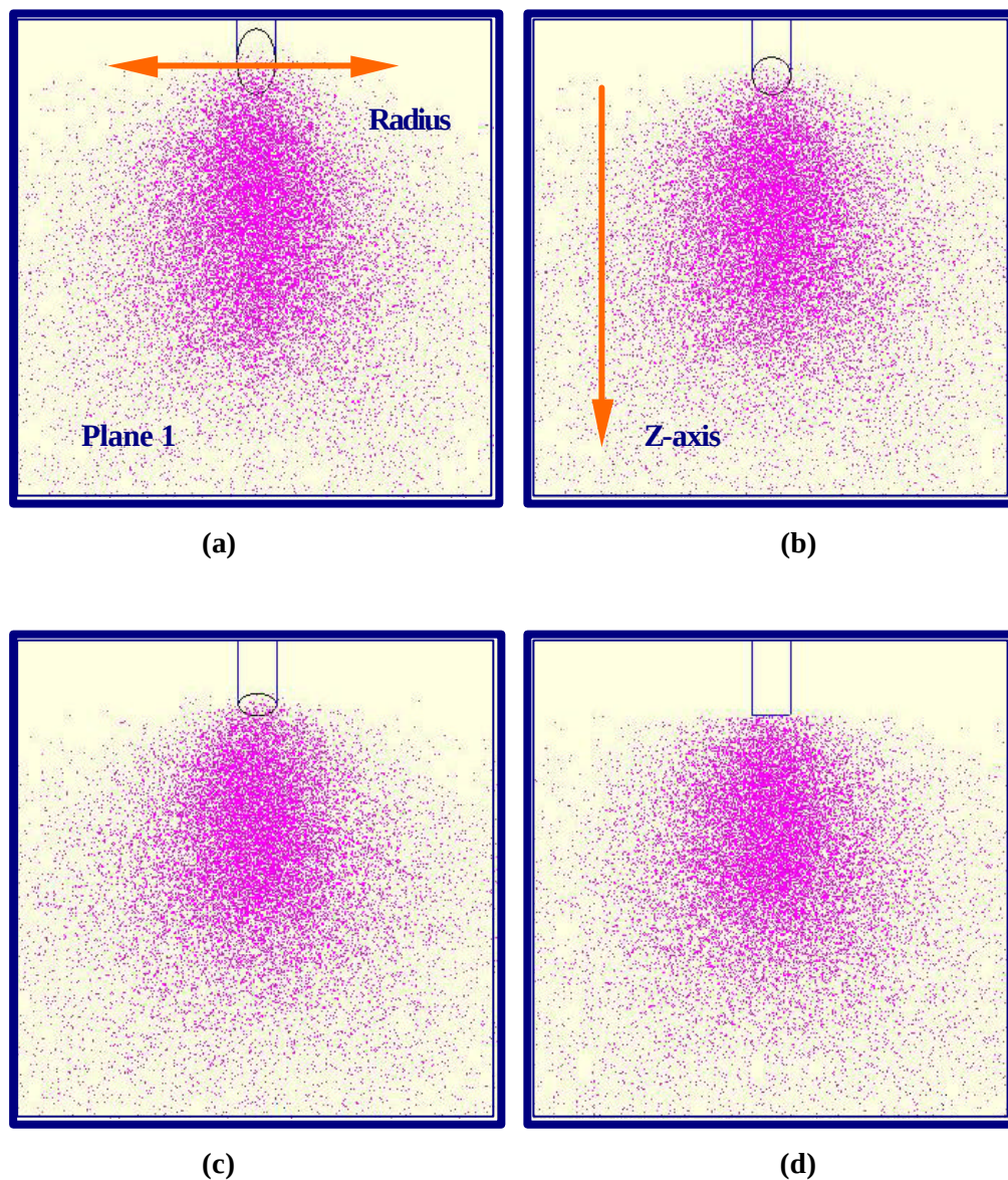
Figure 4.10 The molecules distribution on plane 1 varies with the ending-angle of pipe. The distance between the pipe axis and plane 1 is twice of the pipe radius. The number of molecules simulated was 50000. The ratio of length to radius is 10 times of the pipe radius. The angle between the end cross-section plane and the Z-direction increased from 30^\circ , 45^\circ , 60^\circ , and 90^\circ as the sequence of (a), (b), (c), and (d).
