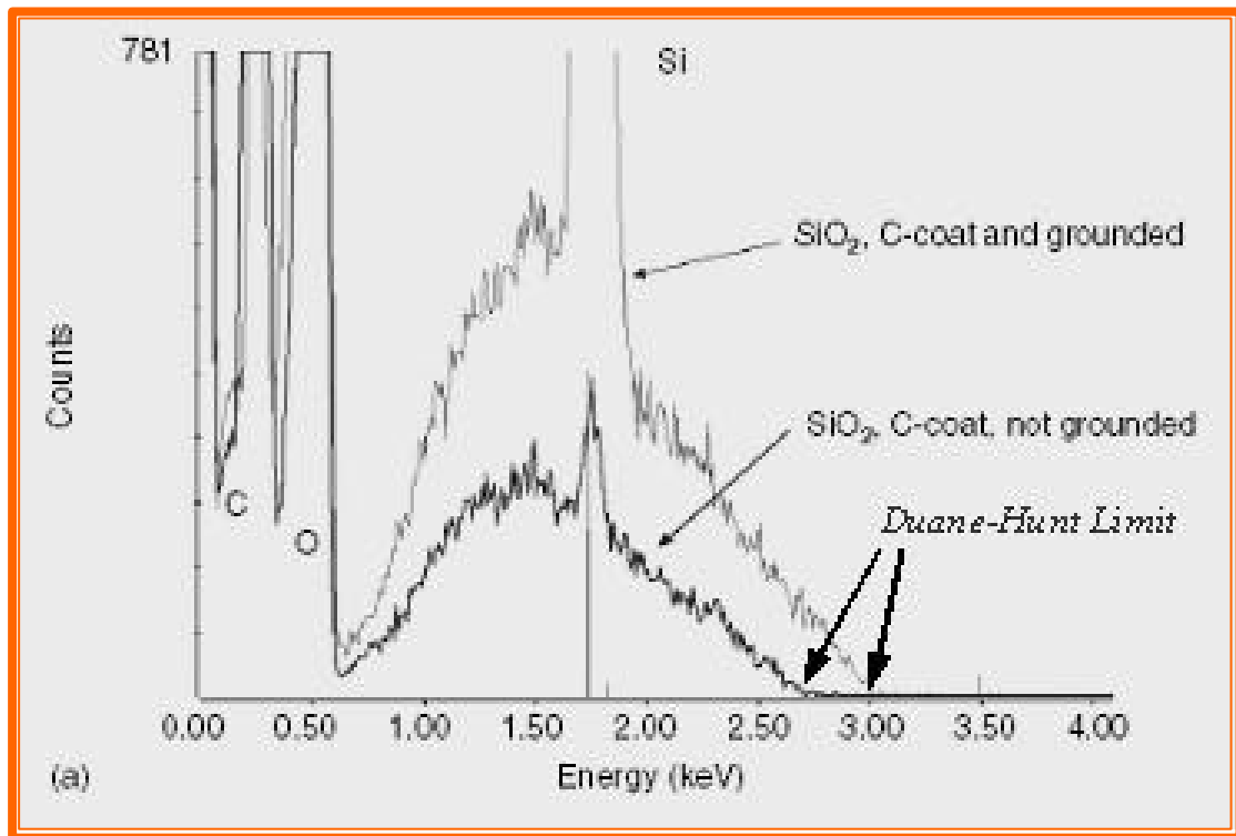
Figure 2.9 Spectra of \text{SiO}_2 with a thin conductive carbon layer irradiated by 3keV electron beam with and without grounded
