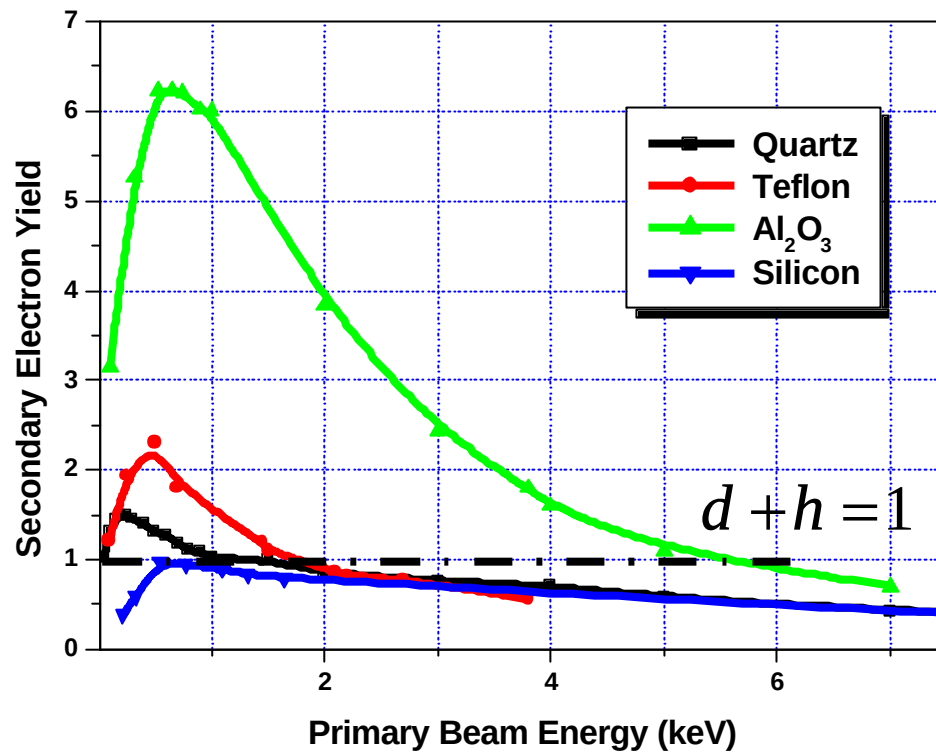
Figure 3.19 Illustration of the secondary electron yield curve as the function of the incident beam energy based on samples of quartz, Teflon, \text{Al}_2\text{O}_3 , and silicon
