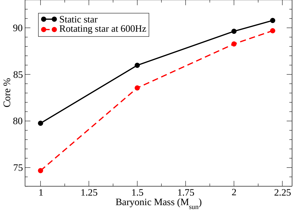
Figure 2.7: (Color on-line) Percentage of the core in a static star (by mass) and a star rotating at 600 Hz as a function of M_B . For more explanation see the text.
