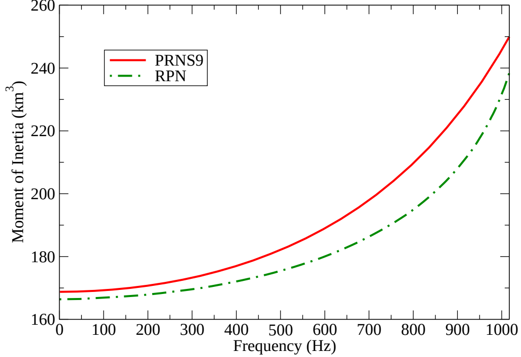
Figure 2.1: (Color on-line) MoI as a function of frequency for a pulsar with M_B = 2.0 M_\odot as calculated with both RPN and PRNS9 numerical codes.
