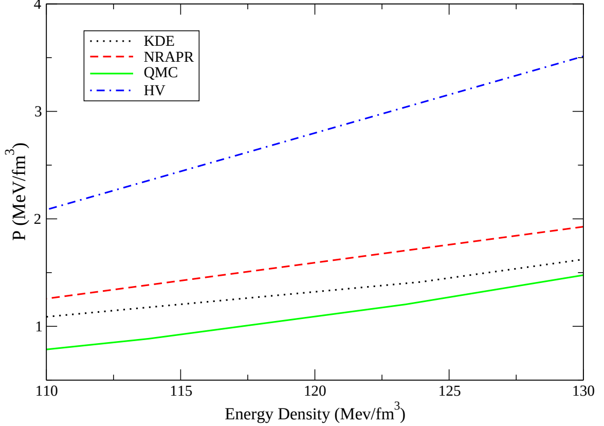
Figure 2.8: The four physical EoS's used in this study. We show the behavior of each EoS around the crust/core transition density of 120 \text{ MeV}/f m^3 .
