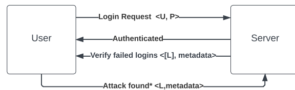
Figure 6.2: Mechanism to register and detect nonces
