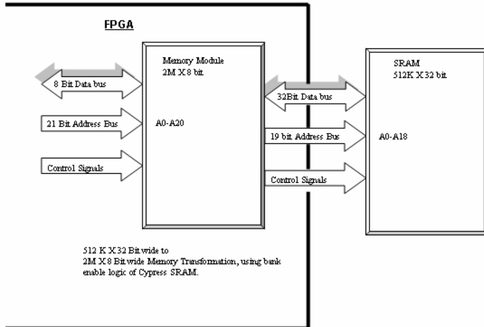
Figure 23 : Memory Interface
