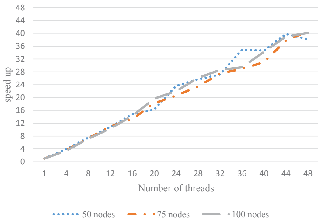
Figure 3.2: Parallel multi-start tabu search
