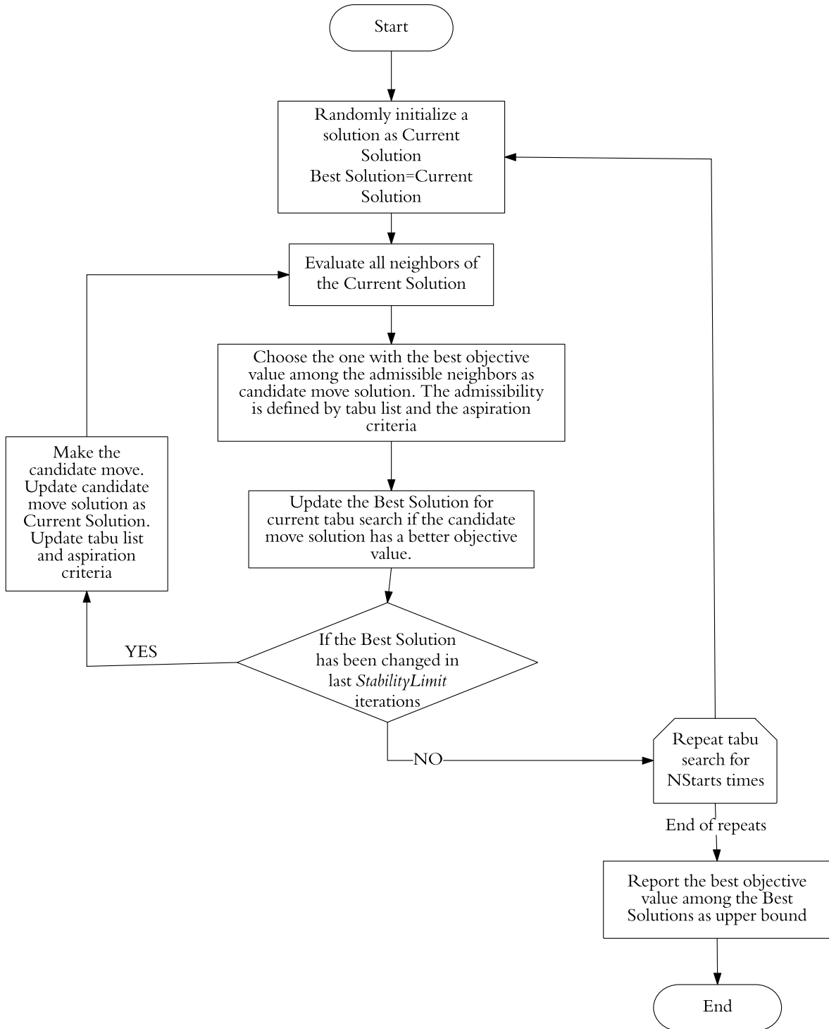
Figure 3.1: Flowchart of the multi-start tabu search
