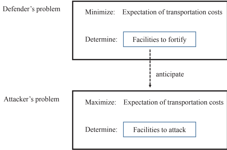
Figure 4.1: Bi-level problem
