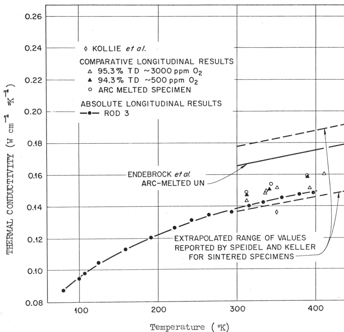
Figure 16. Thermal Conductivity of Uranium Mononitride to 400 ^\circ\text{K} .
