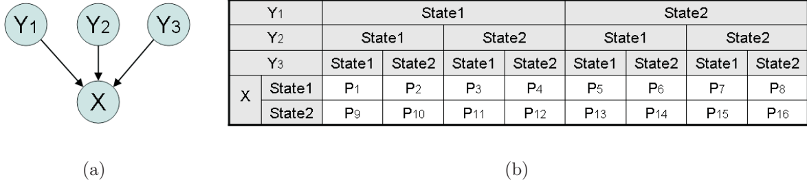
Figure 3.4: (a) A simple Bayesian network with three parents nodes ( Y_1, Y_2, Y_3 ) and one child node ( X ). (b) The conditional probability table of X .
