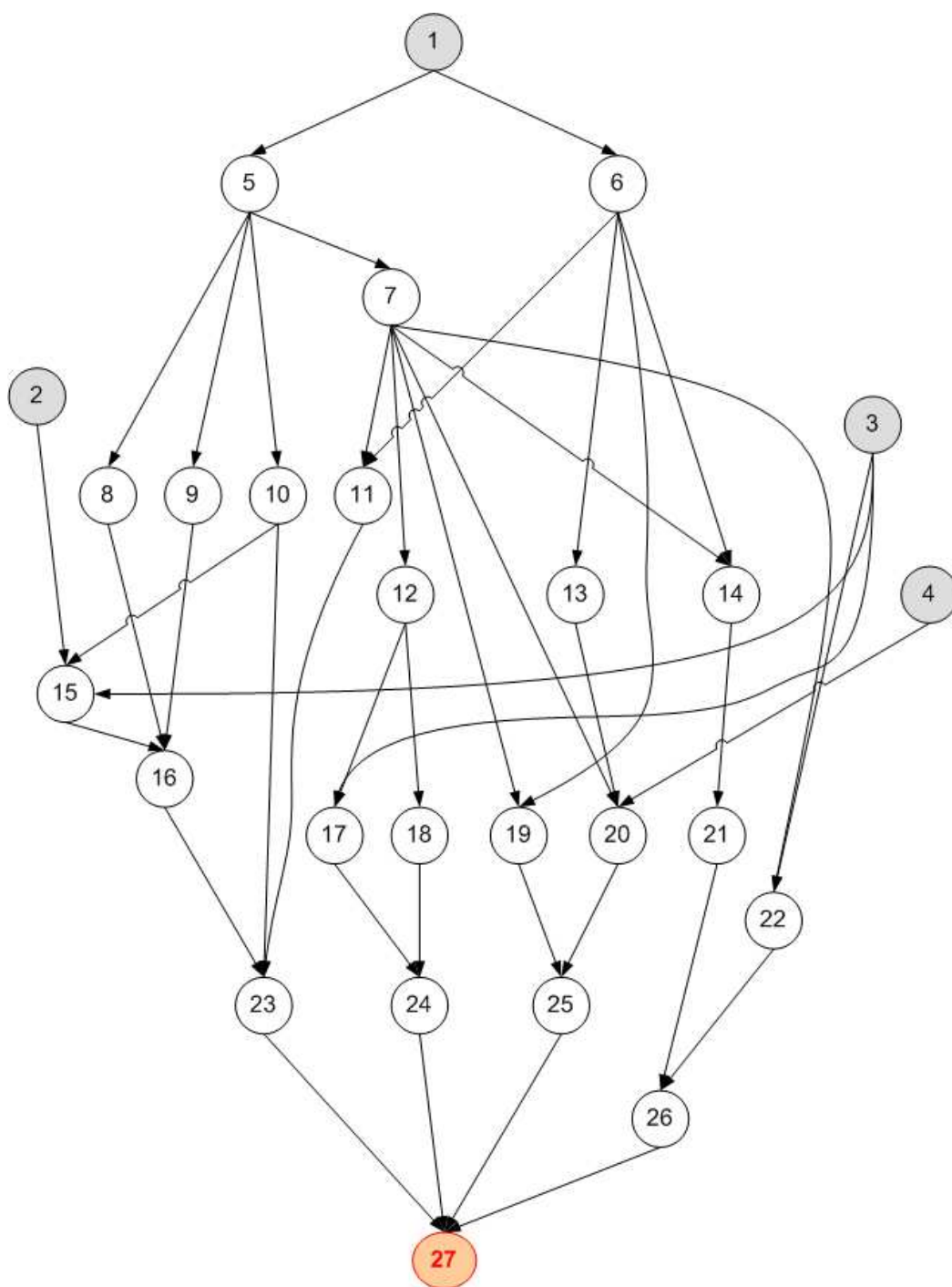
Figure 4.6: BN Graphic Model
