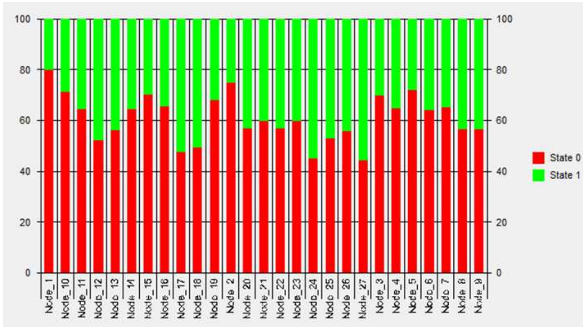
Figure 4.7: Unconditional Probabilities of All Events
