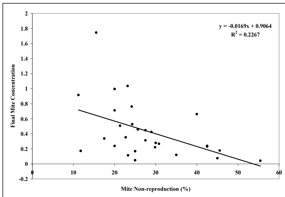
Figure 3.3 Linear regression analyses between non-reproductive mites and final mite concentration in colonies
