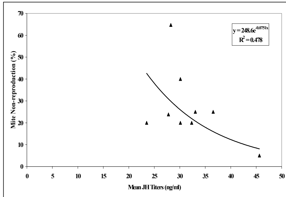
Figure 4.2 Regression analyses between mite non-reproduction and mean JH titers in nine honey bee colonies
