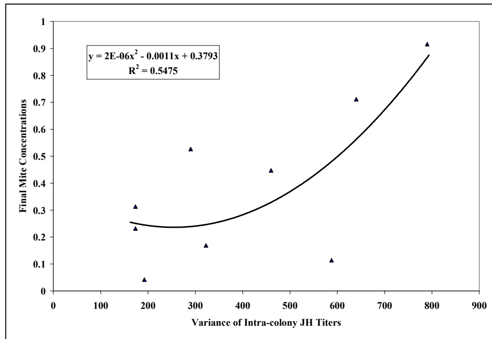
Figure 4.3 Regression analyses between final mite concentrations and variance of JH titers in nine honey bee colonies
