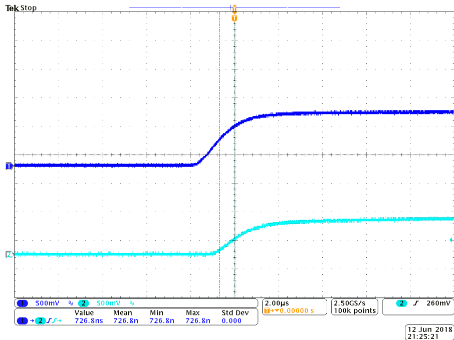
Figure 3.21: 1PPS test waveform at 2µs/div. Note \Delta t between rise times of 700 ns.
