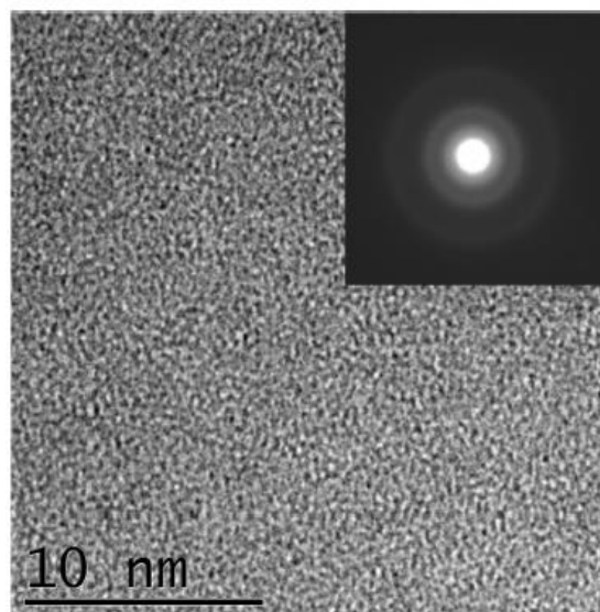
Figure 19: HRTEM image of a\text{-B}_{2.5}\text{C} material, with SAED pattern shown in inset [26].
