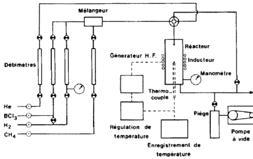
Figure 5: System setup for the cold-walled CVD growth process [12].
