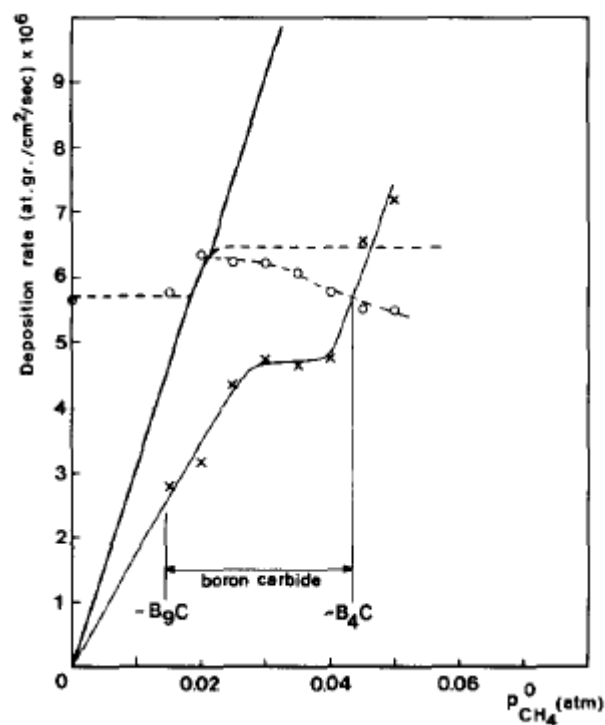
Figure 7: Theoretical and experimental deposition rates of boron and carbon at set conditions ( T=1527^{\circ}\text{C} , partial pressure of \text{BCl}_3=0.2 atm, and mass flow rate of 0.04 \text{ g cm}^{-2}\text{-sec}^{-1} [12].
