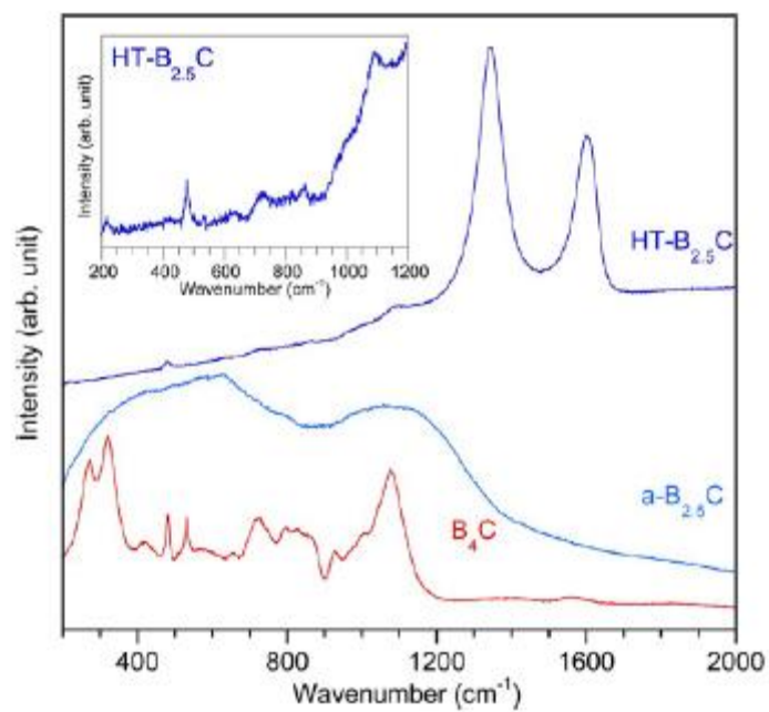
Figure 20: Raman spectra of the a\text{-B}_{2.5}\text{C} and heat-treated coating, with the 200-1200 \text{cm}^{-1} region of the heat-treated spectrum highlighted in the inset [26].
