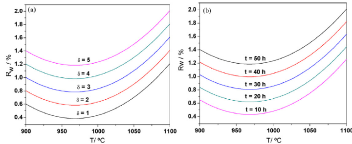
Figure 17: Relation curves between R_w and T . (a) Presents five inlet gas ratios at t=50\text{ h} and H_2 ratio=3.5. (b) Presents five deposition times at \delta=5 and H_2 ratio=3.5 [24].
