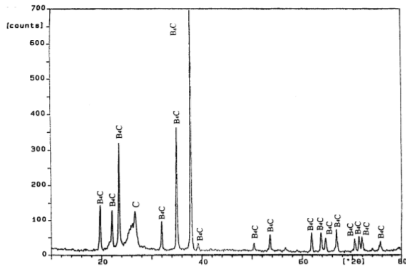
Figure 46: XRD analysis of boron carbide [42].
