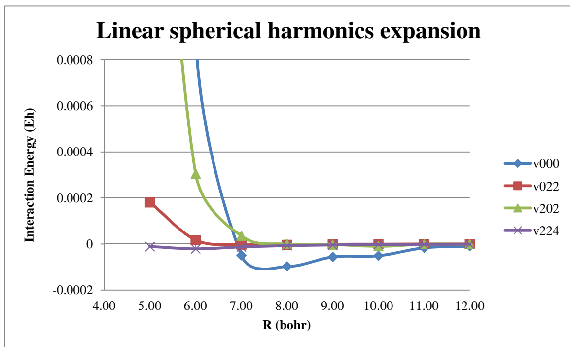
Figure 7: Values of the four-term spherical harmonics expansion.
