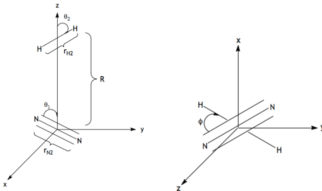
Figure 1: Example orientation of the molecules with angle assignments shown. The value R is the center-of-mass distance between the molecules and the value r represents the \text{N}_2 and \text{H}_2 monomer bond lengths.
