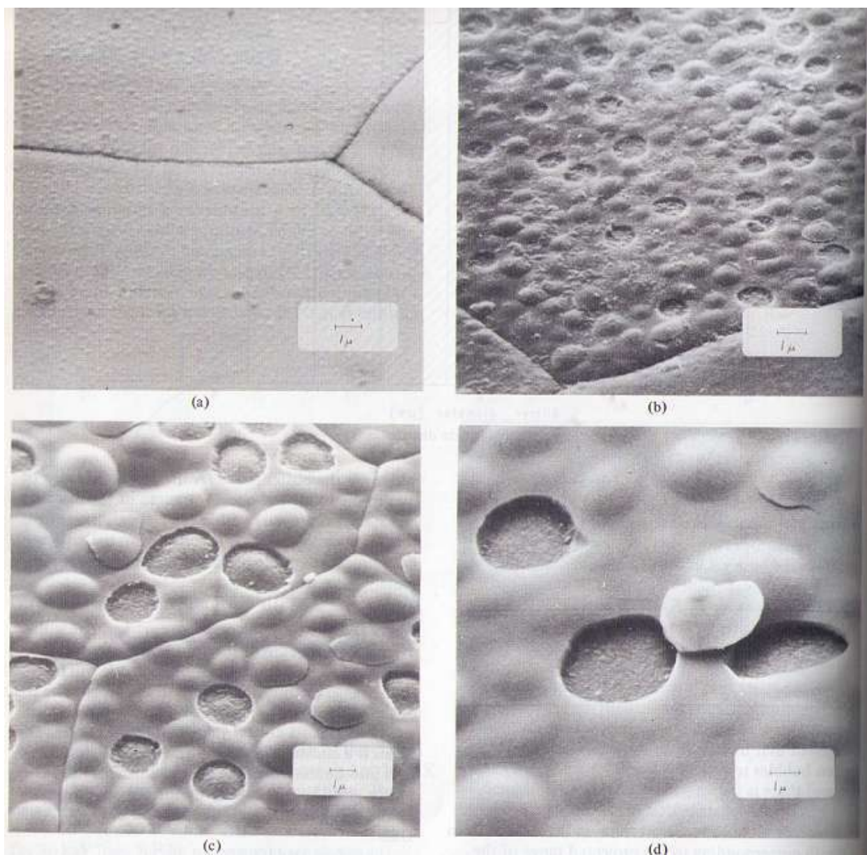
Figure 2.16 Shows blistering of molybdenum after bombardment He + ions of different energies (a) 7 KeV (b) 20 KeV (c) 50 KeV (d) 80 KeV. Courtesy of Erents et.al [74]
