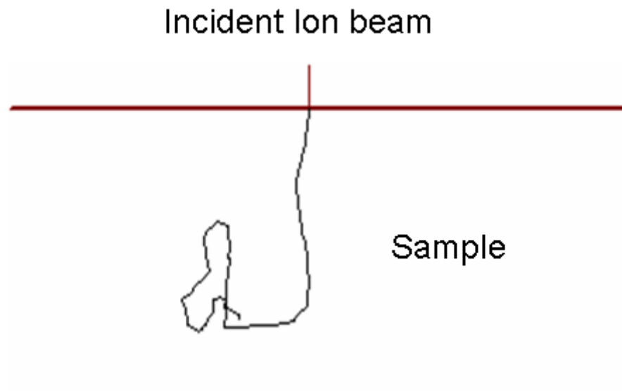
Figure 3.01 An ion beam trajectory showing the successive deflections of the ion as it travels in the sample
