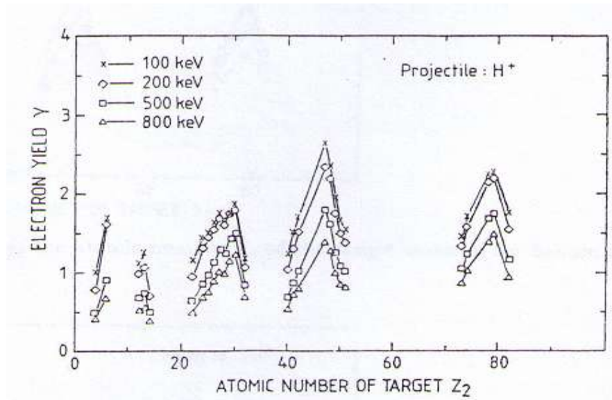
Figure 4.14 showing the iSE yields for proton impacts on targets with Different atomic number. Courtesy of Hasselkamp et al [34]
