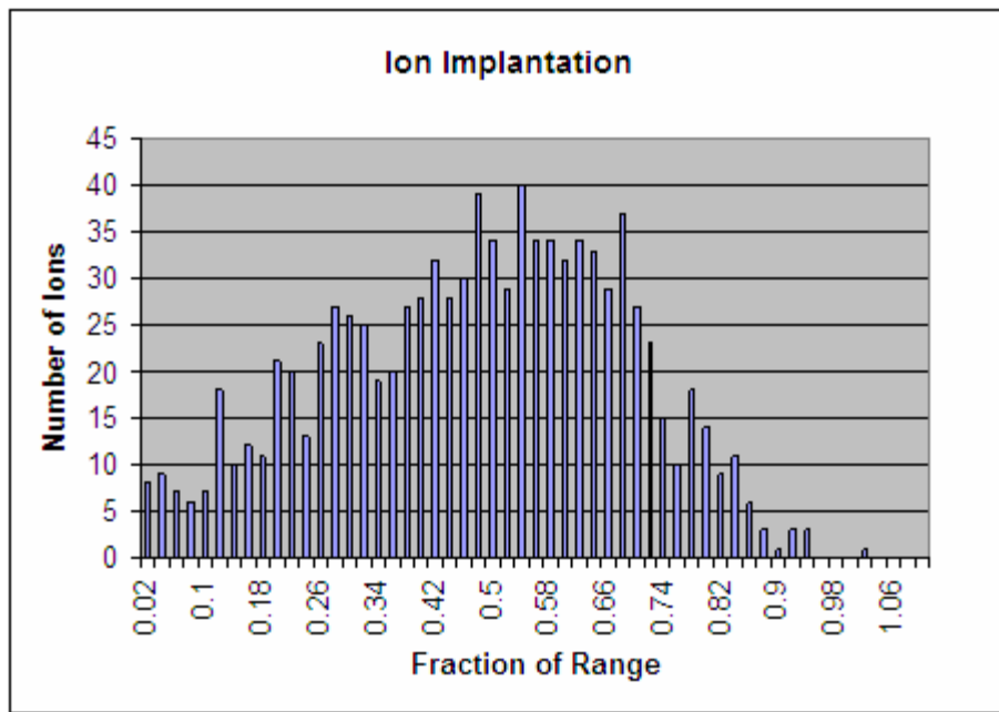
Figure 1.08 Helium ion depth distribution profile in Al
