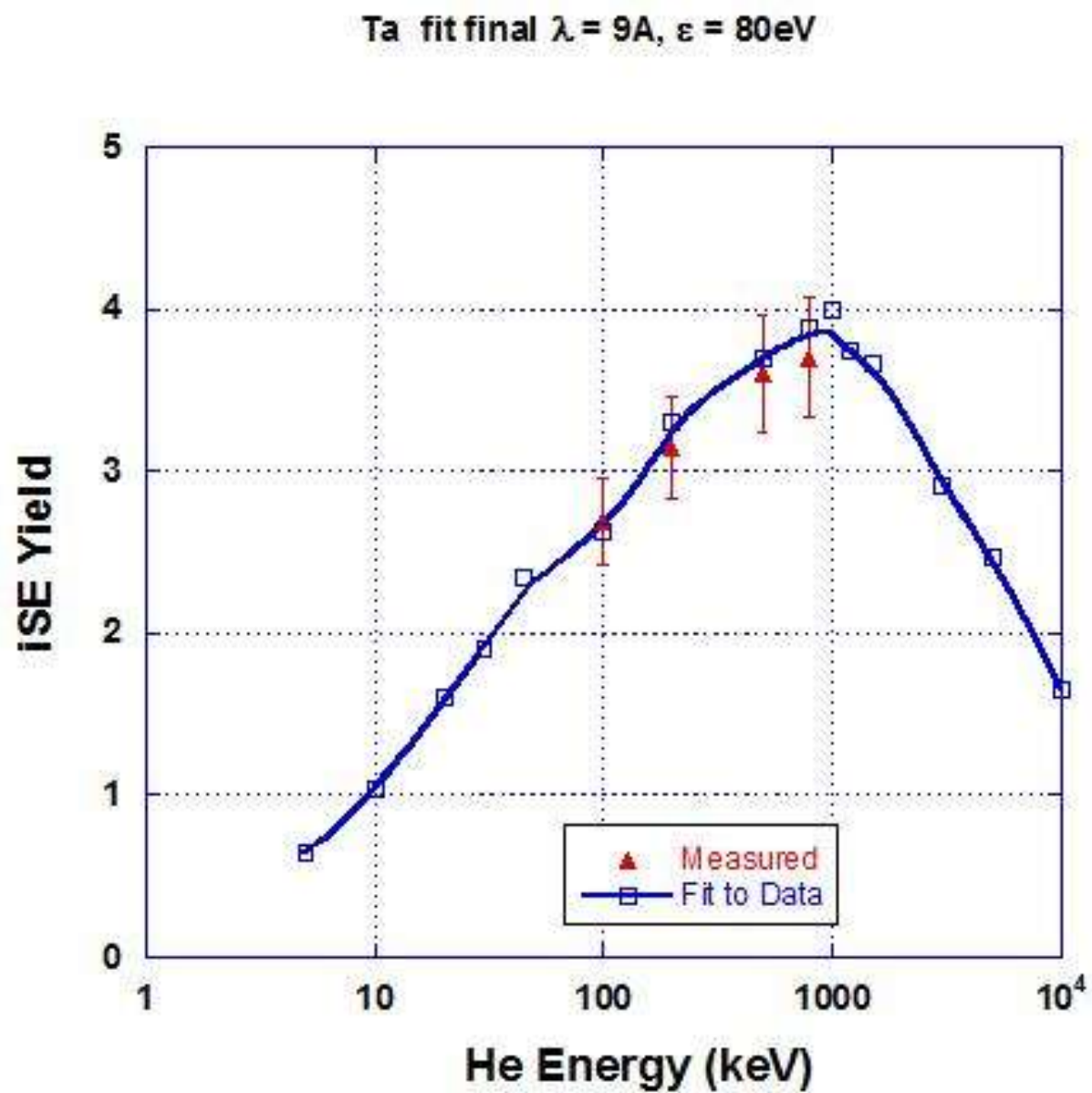
Figure 5.22 Showing the iSE yield parameters and data fit for Tantalum
