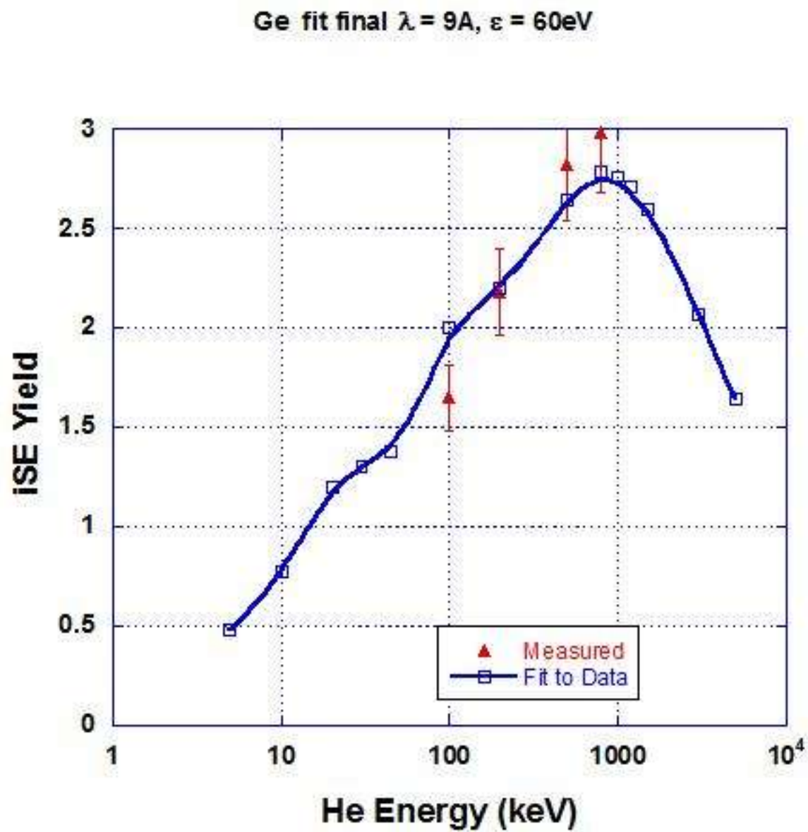
Figure 5.14 Showing the iSE yield parameters and data fit for Germanium
