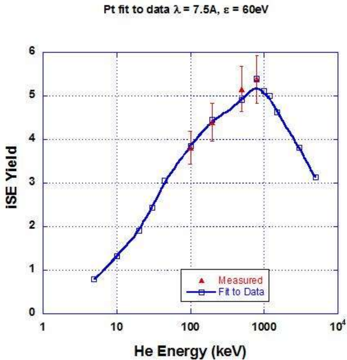
Figure 5.24 Showing the iSE yield parameters and data fit for Platinum
