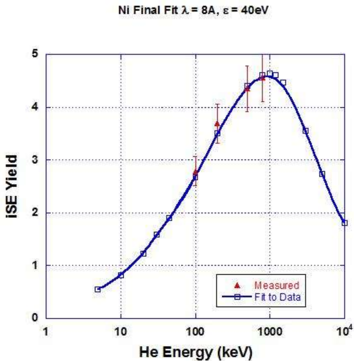
Figure 5.11 Showing the iSE yield parameters and data fit for Nickel
