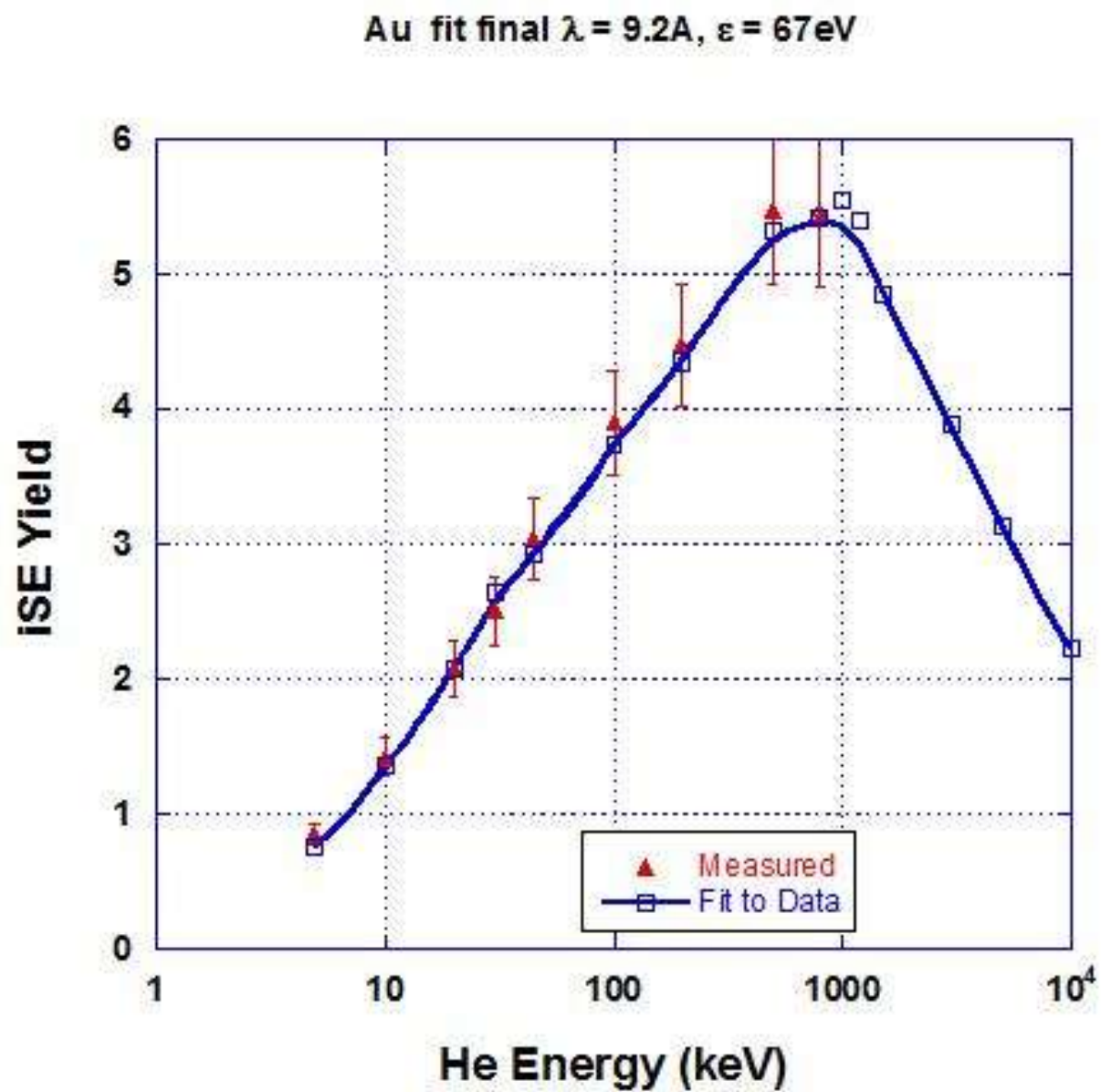
Figure 5.25 Showing the iSE yield parameters and data fit for Gold
