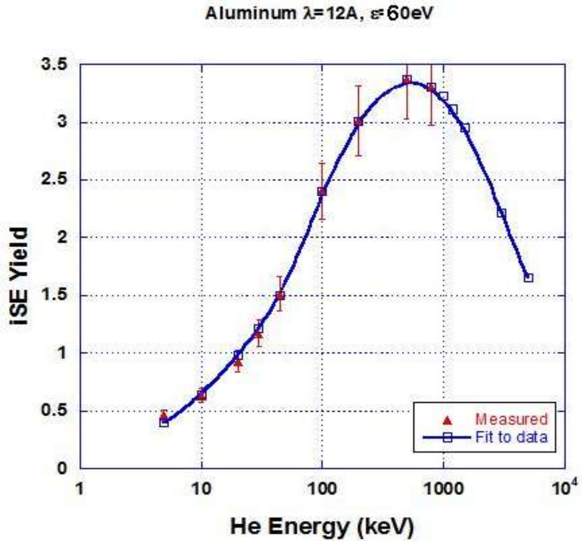
Figure 5.06 Showing the iSE yield parameters and data fit for Aluminum
