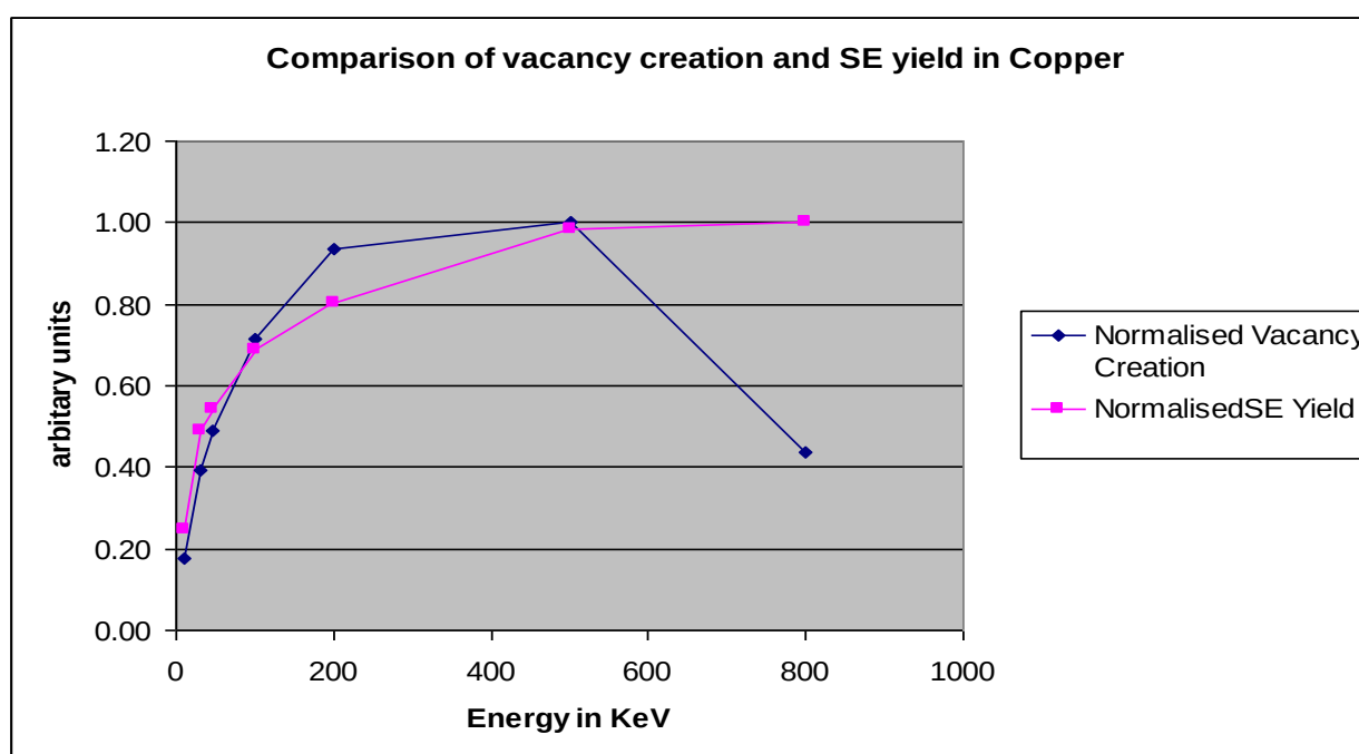
Figure 5.33 Comparing the iSE and Vacancy yields for \text{He}^+ ions. Data from IONiSE and SRIM [3]
