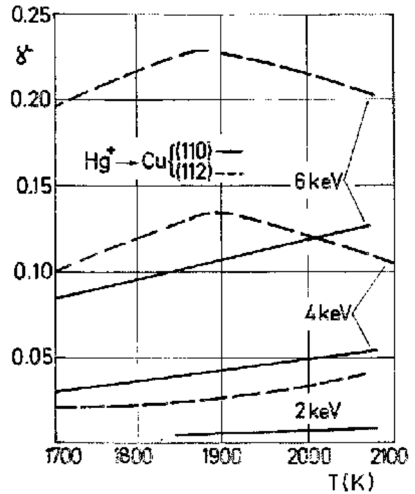
Figure 4.26 Showing the SE yields as a function of temperature for H_2^+ and Hg^+ ions incident on monocrystalline W and Cu. Courtesy of Petrov [48].
