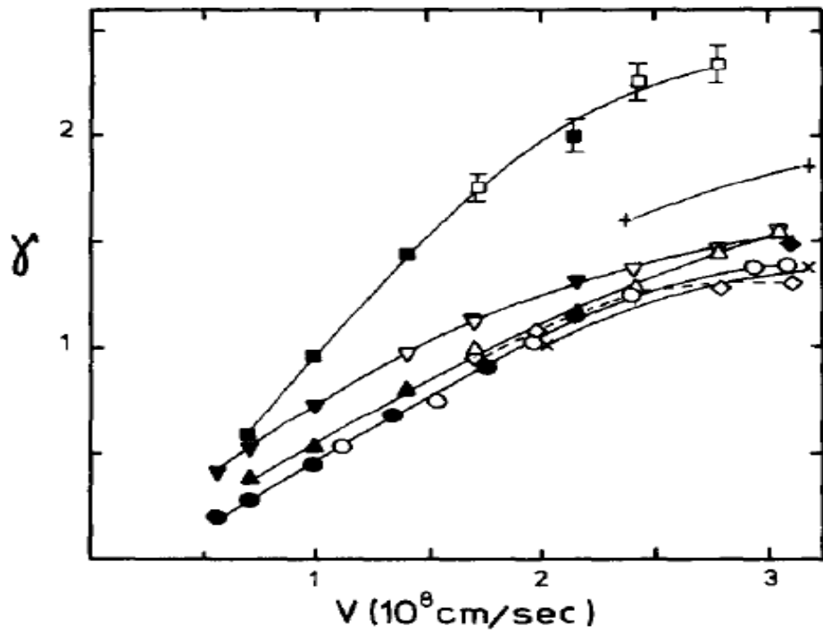
Figure 4.25 Showing the yields for H^+ (open symbols) and D^+ (closed symbols) : (\nabla, \circ, \Delta, \square) for Li, Al, Cu and Ag respectively. Courtesy of Baragiola et al [47]
