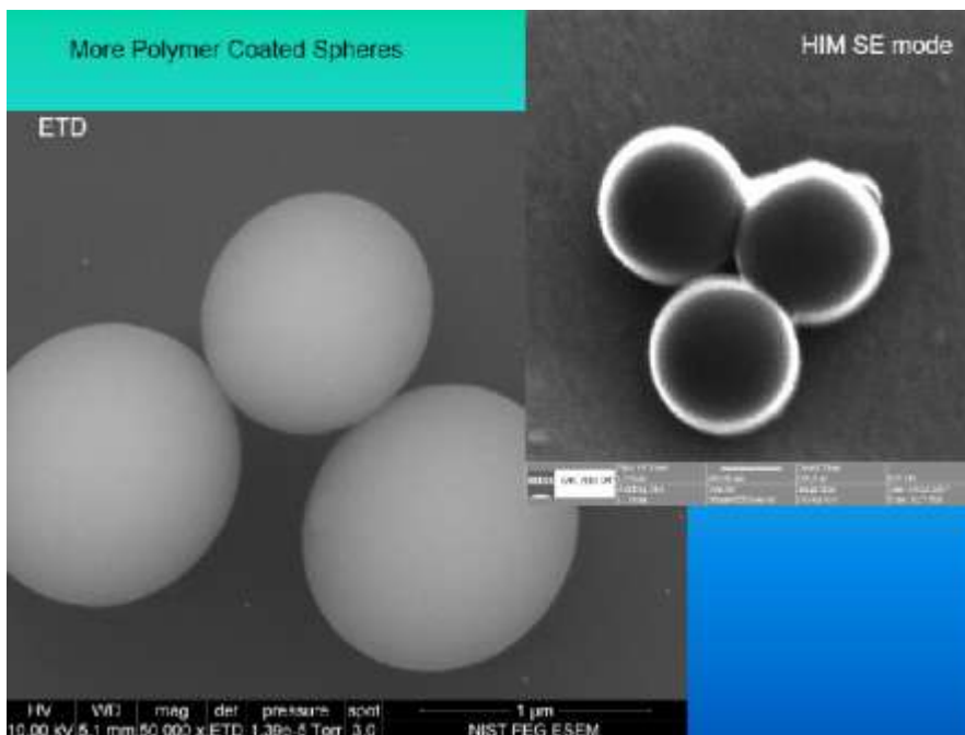
Figure 2.13 Shows the magnified image on coated polymer spheres in a SHIM image (Right image) as compared to a SEM image Left image). Courtesy of Wight [69]
