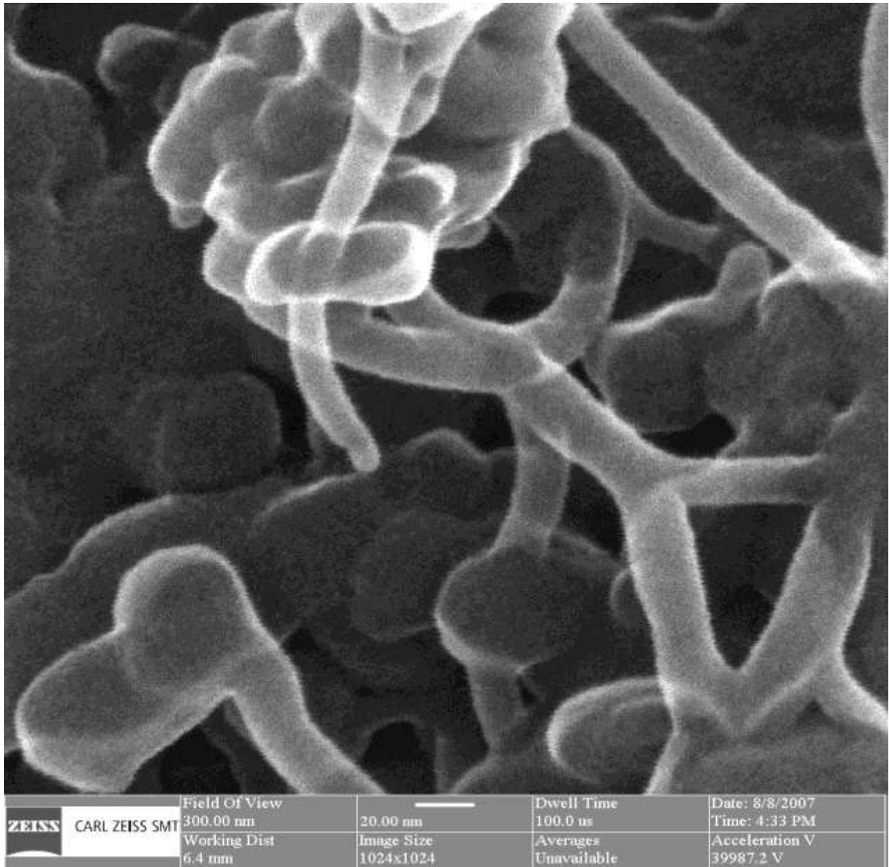
Figure 1.10 Shows the He ion SIM image of a CNT, the size of fiber is about 20 nm and image shows excellent background information even at such a high resolution.
