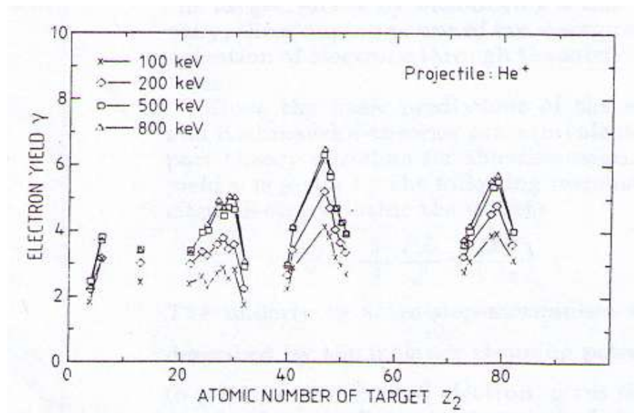
Figure 4.15 Showing the iSE yields for helium impacts on targets with Different atomic number. Courtesy of Hasselkamp et al [34]
