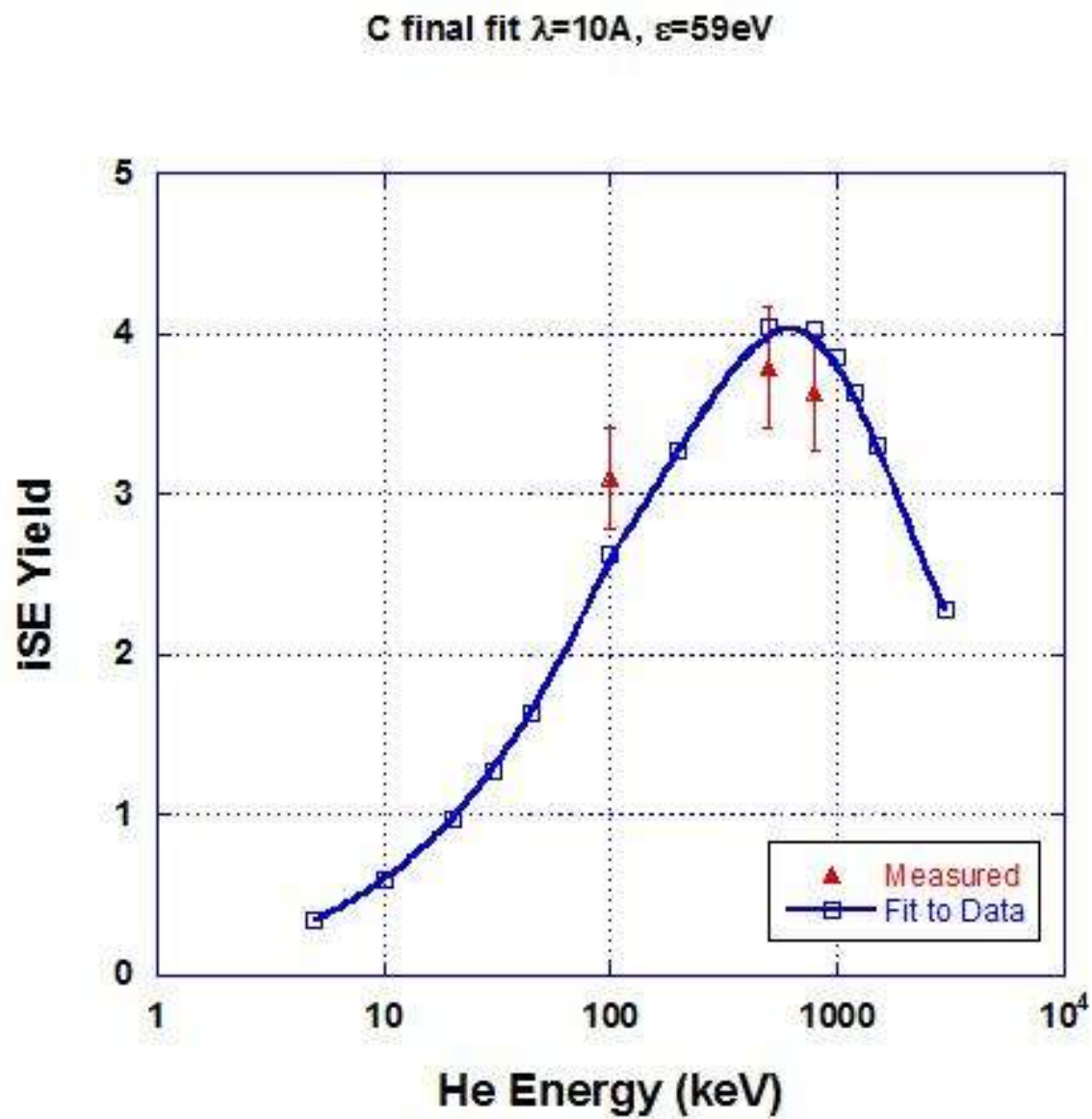
Figure 5.04 Showing the iSE yield parameters and data fit for Carbon
