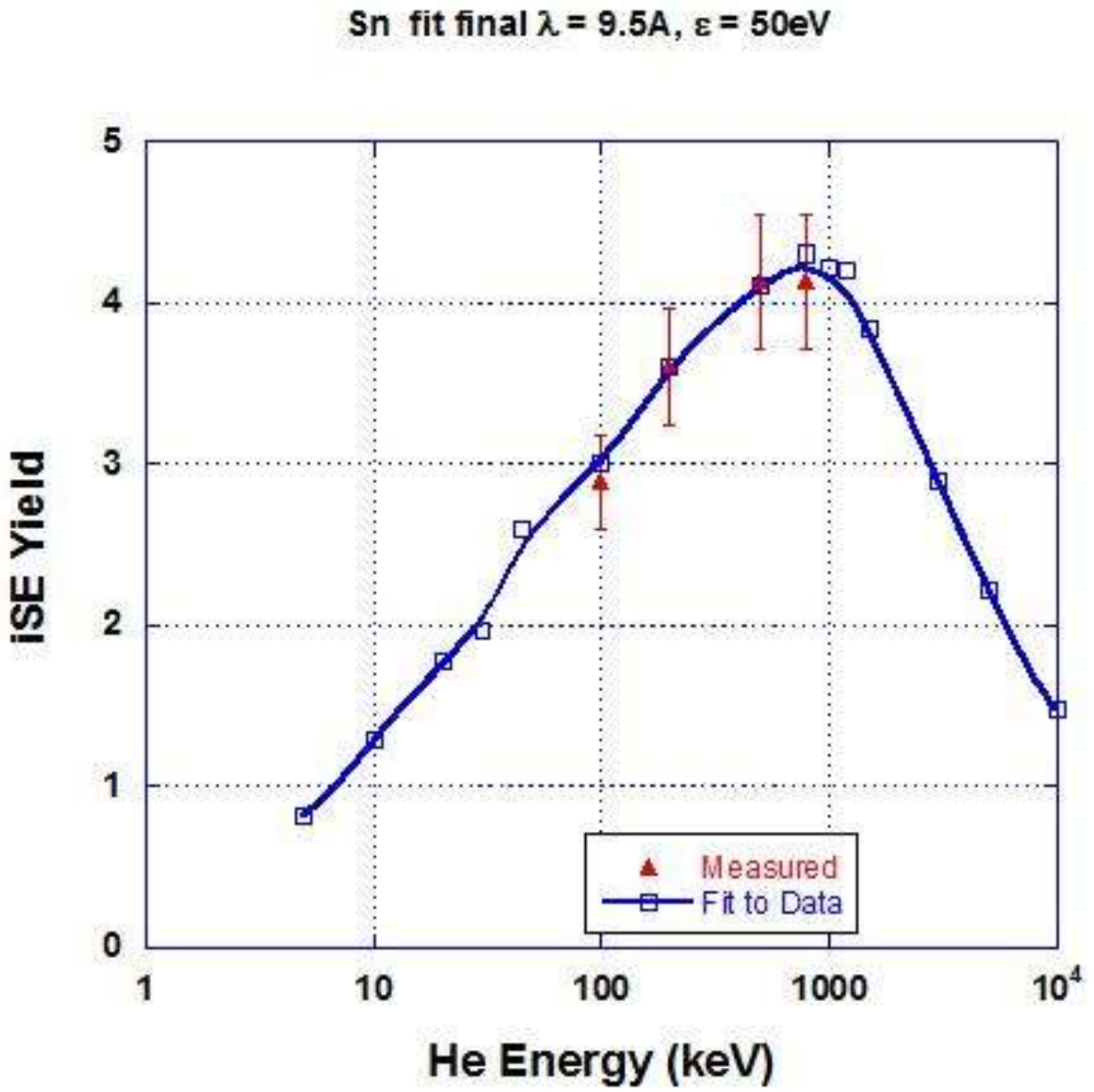
Figure 5.20 Showing the iSE yield parameters and data fit for Tin
