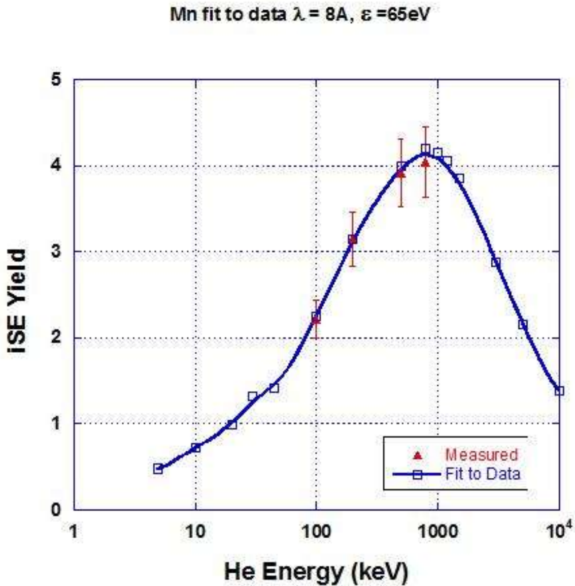
Figure 5.09 Showing the iSE yield parameters and data fit for Manganese
