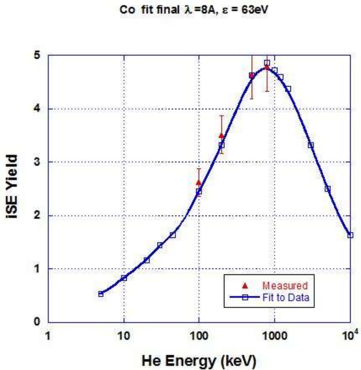
Figure 5.10 Showing the iSE yield parameters and data fit for Cobalt
