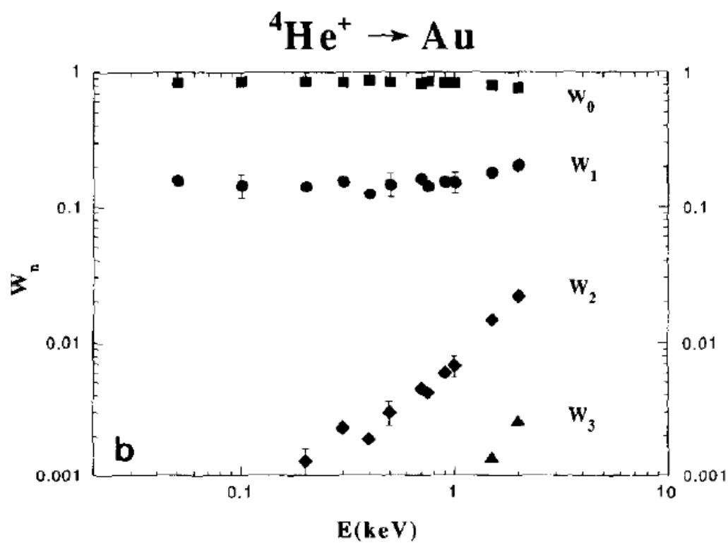
Figure 4.10 Showing the Probability of electron emission statistics for \text{He}^+ on Au. Courtesy of Toglhofer[49]
