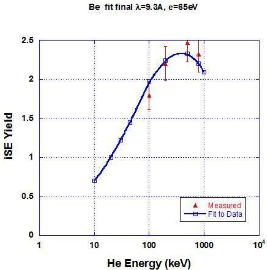
Figure 5.03 Showing the iSE yield parameters and data fit for Beryllium
