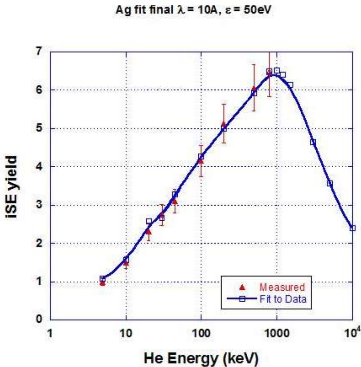
Figure 5.17 Showing the iSE yield parameters and data fit for Silver
