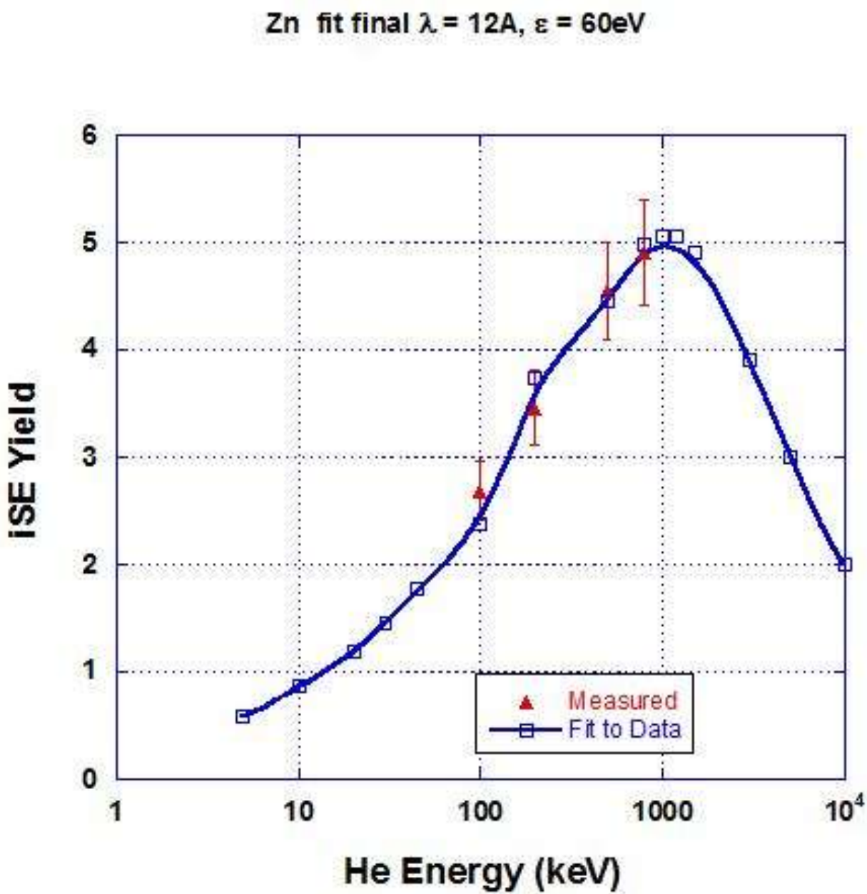
Figure 5.13 Showing the iSE yield parameters and data fit for Zinc
