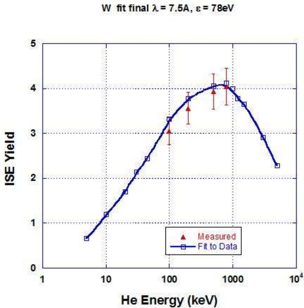
Figure 5.23 Showing the iSE yield parameters and data fit for Tungsten
