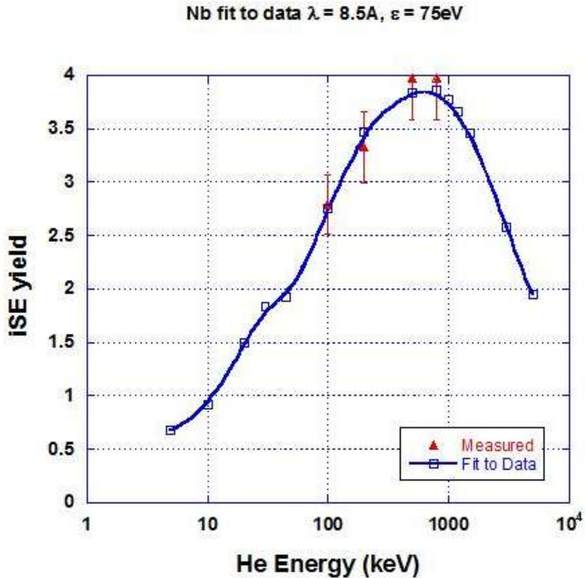
Figure 5.16 Showing the iSE yield parameters and data fit for Niobium
