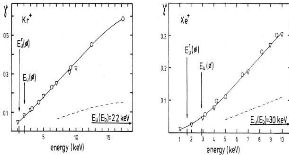
Figure 4.24 Showing the relative contributions of the recoil target atoms on the total electron yield of Kr^+ and Xe^+ , the dashed line showing the recoil atom contribution.
