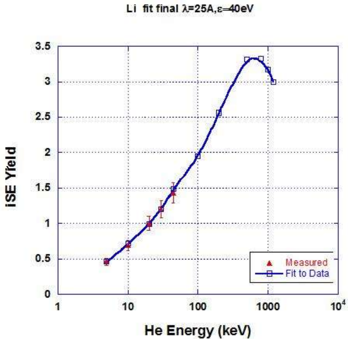
Figure 5.02 Showing the iSE yield parameters and data fit for Lithium
