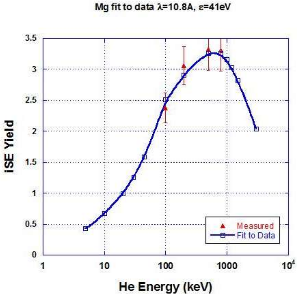
Figure 5.05 Showing the iSE yield parameters and data fit for Magnesium
