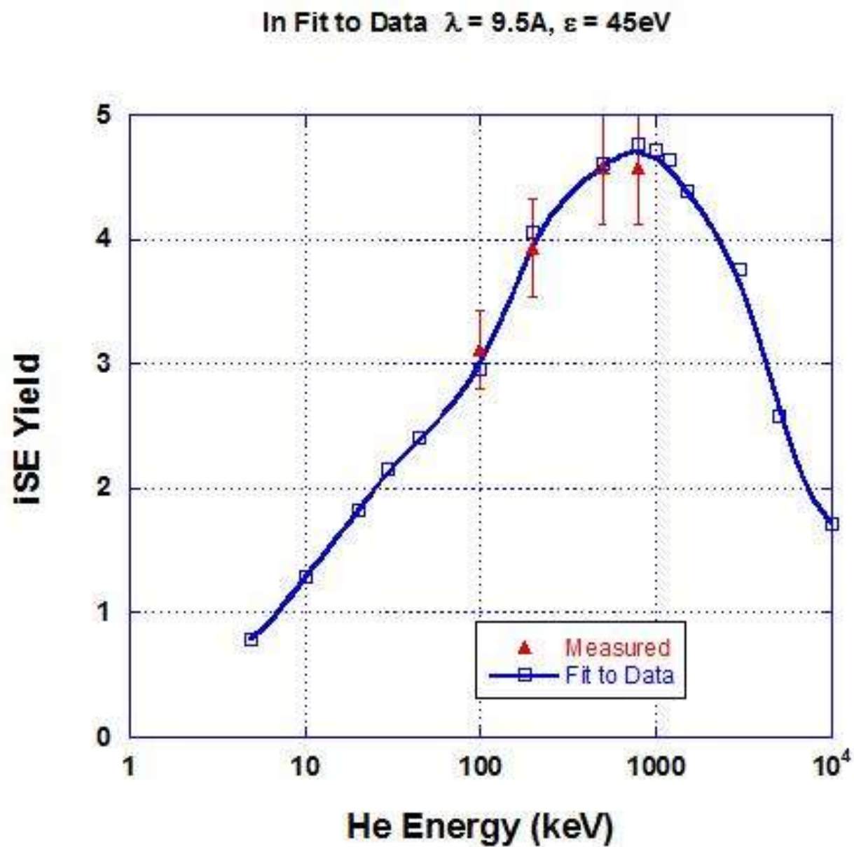
Figure 5.19 Showing the iSE yield parameters and data fit for Indium
