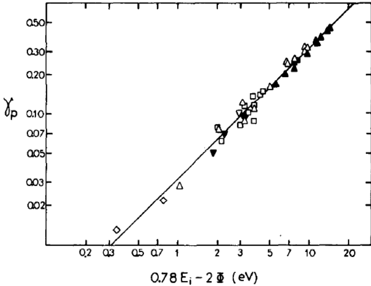
Figure 4.05 Showing the PEE yield fit closely to the yield equation proposed by Hagstrum.
