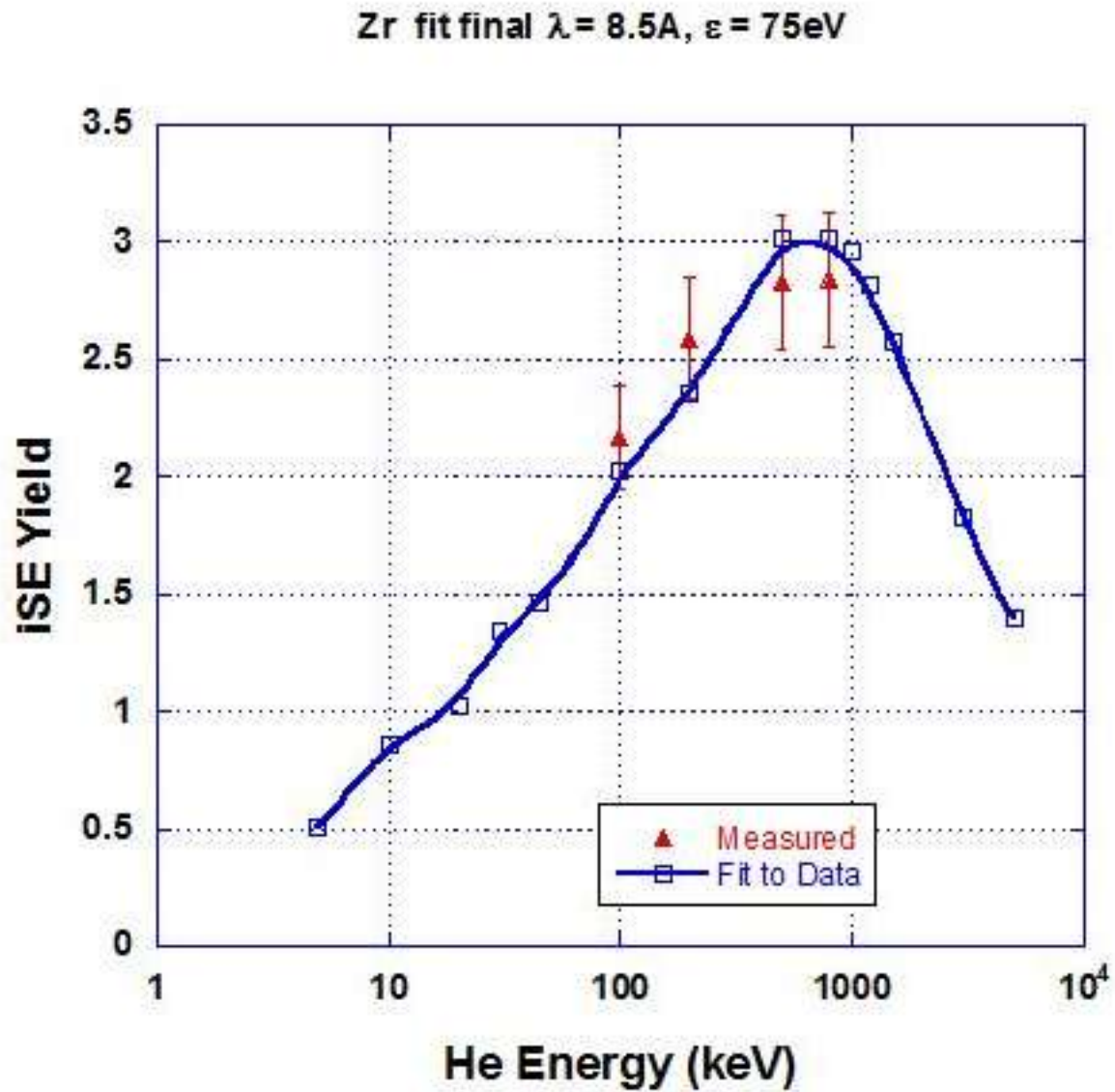
Figure 5.15 Showing the iSE yield parameters and data fit for Zirconium
