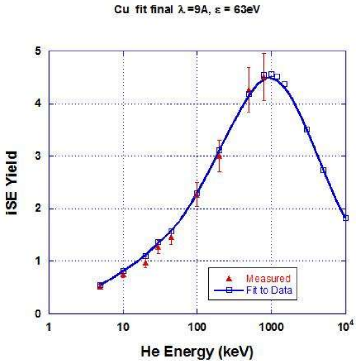
Figure 5.12 Showing the iSE yield parameters and data fit for Copper
