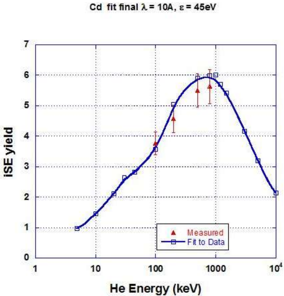
Figure 5.18 Showing the iSE yield parameters and data fit for Cadmium
