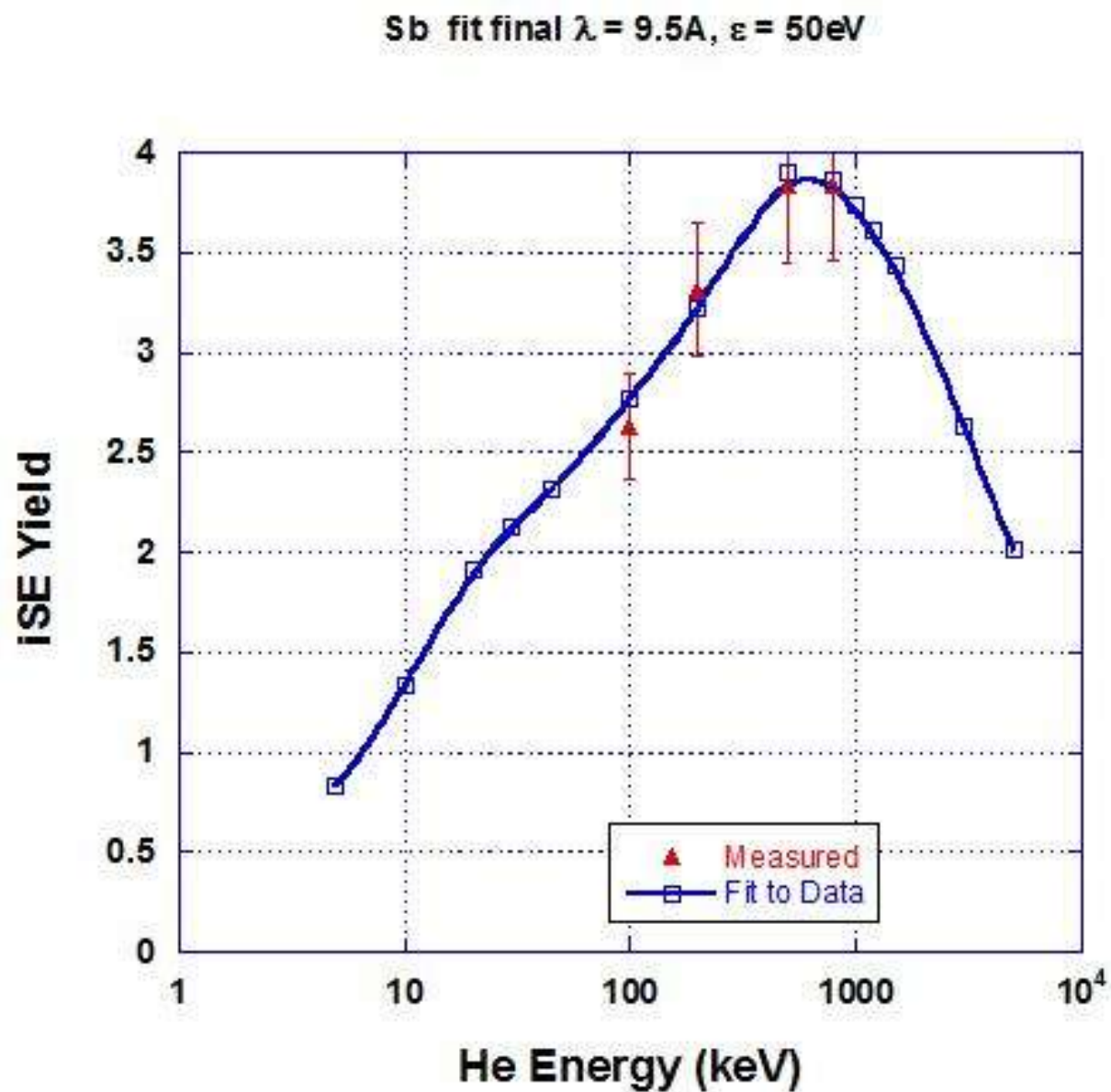
Figure 5.21 Showing the iSE yield parameters and data fit for Antimony
