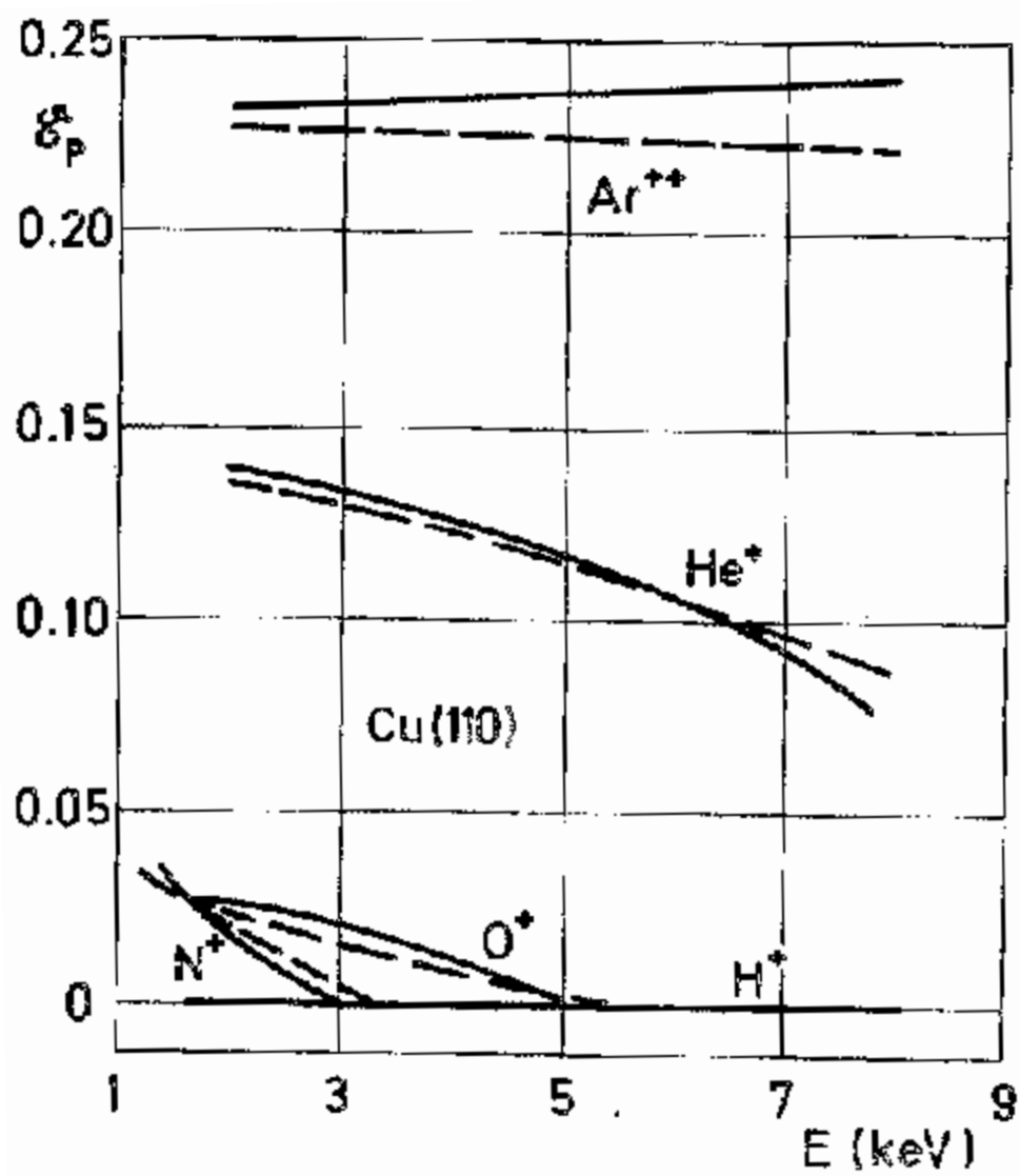
Figure 4.06 Showing the PEE versus Energy E for Ar^{++} , He^+ , N^+ , O^+ and H^+ On monocrystalline copper Cu(110). Courtesy of Petrov [48]
