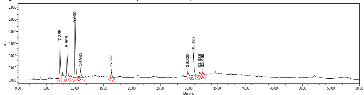
Figure 194. HPLC@280 nm, charred layer 7, control rep 2, run 1
