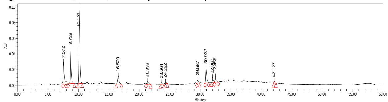
Figure 182. HPLC@280 nm, charred layer 6, control rep 2, run 1
