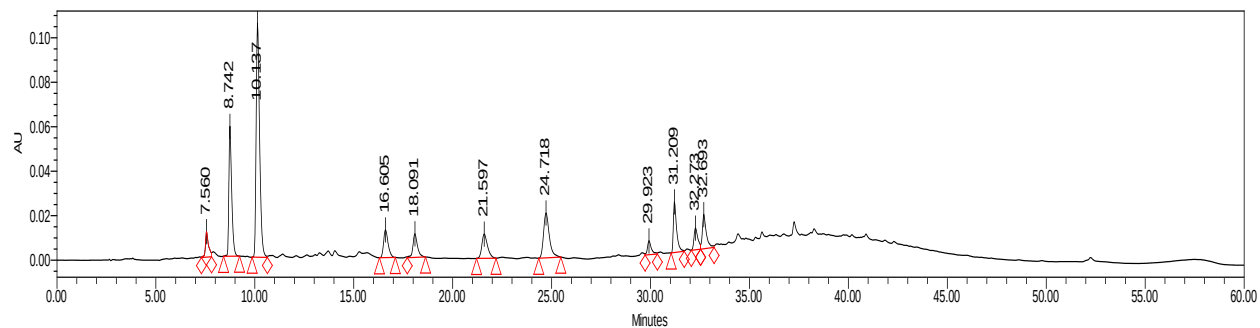
Figure 270. HPLC@280 nm, charred layer 3, control rep 1, run 1
