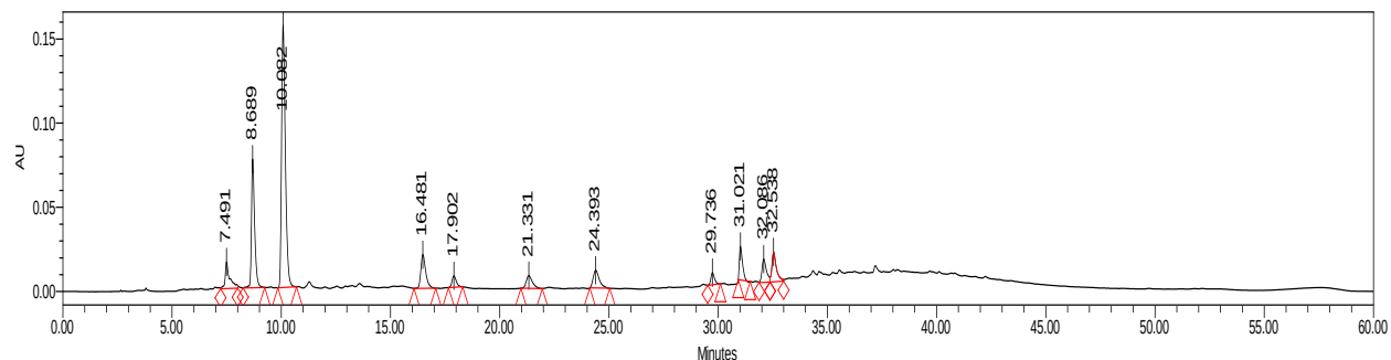
Figure 348. HPLC@280 nm, toasted layer 3, sonicated rep 2, run 1
