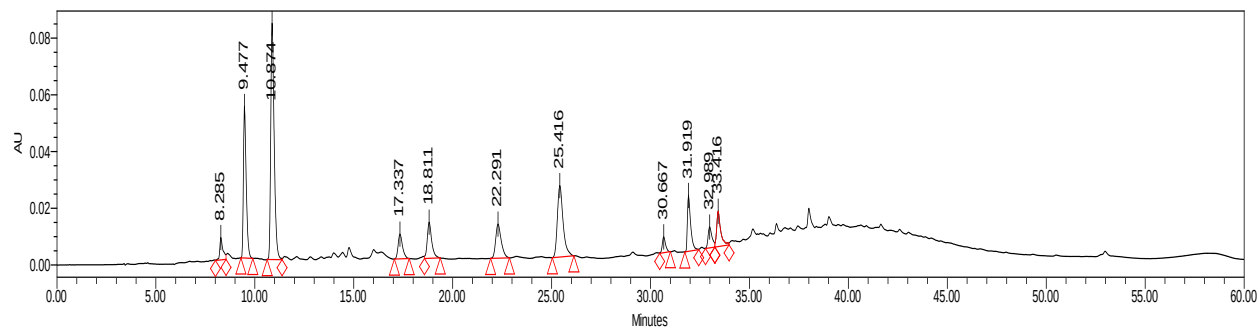
Figure 255. HPLC@280 nm, charred layer 2, sonicated rep 2, run 2
