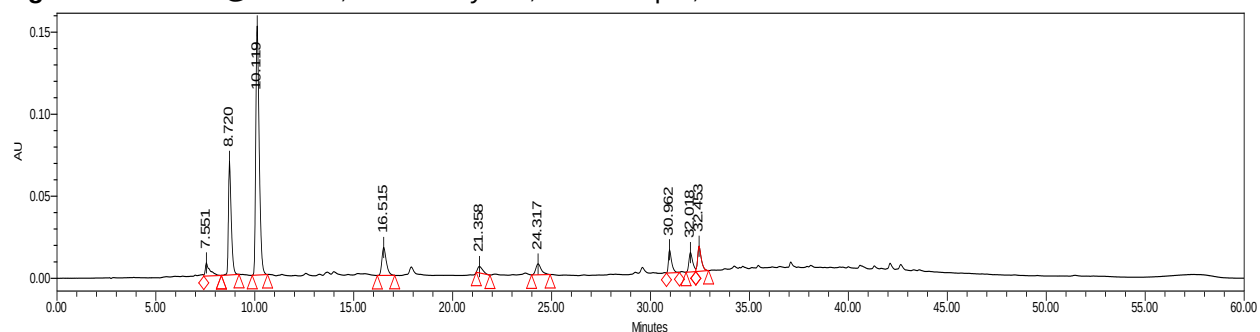
Figure 215. HPLC@280 nm, toasted layer 2, control rep 2, run 2
