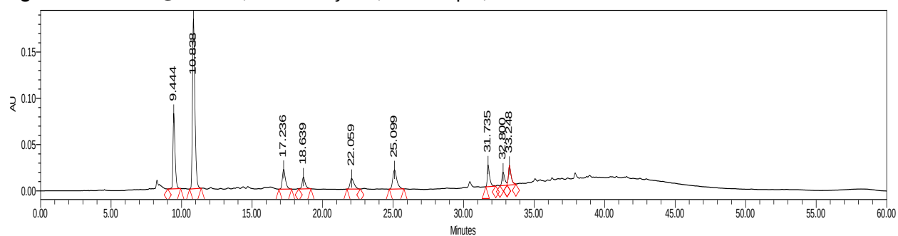
Figure 341. HPLC@280 nm, toasted layer 2, reflux rep 2, run 1
