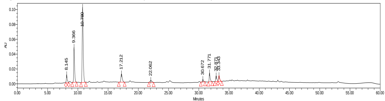
Figure 229. HPLC@280 nm, toasted layer 4, sonicated rep 1, run 2
