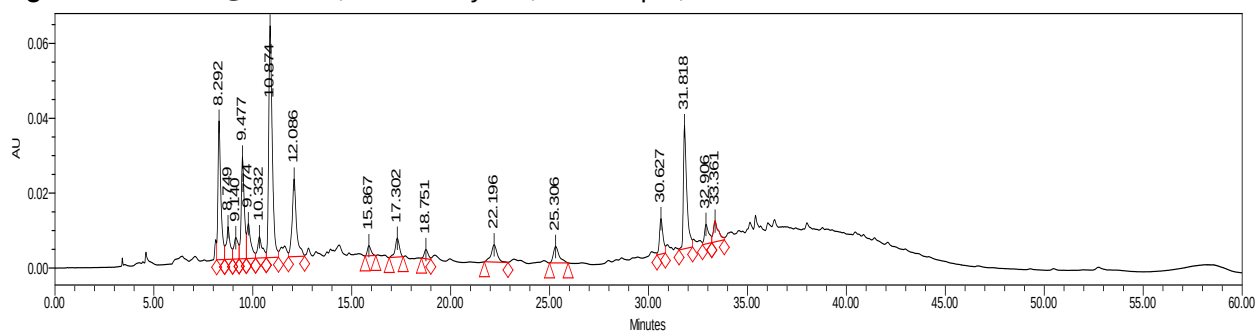
Figure 317. HPLC@280 nm, charred layer 7, reflux rep 2, run 2
