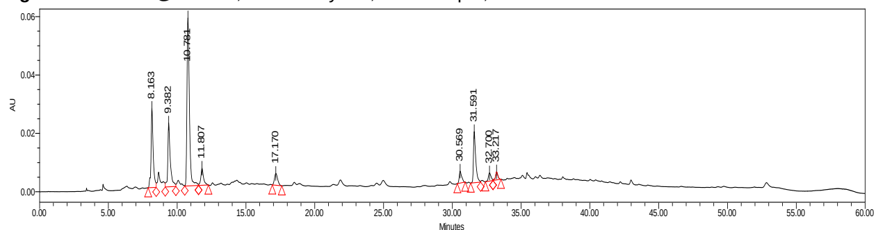
Figure 195. HPLC@280 nm, charred layer 7, control rep 2, run 2
