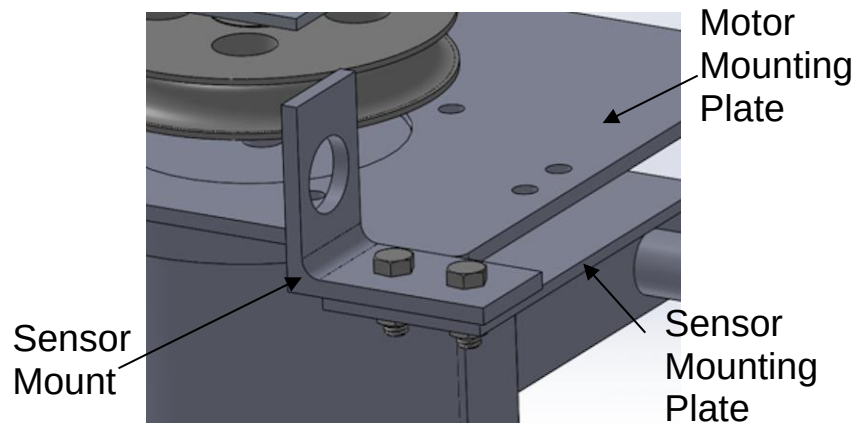
Figure 15: Sensor Mounting Assembly
