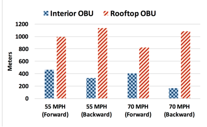
Figure 2.6: Comparison of DSRC Communication Ranges
