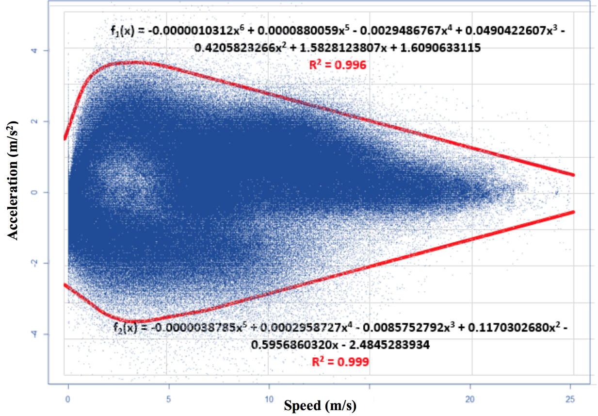
Figure 3.1: Real-world speed-acceleration relationship from Basic Safety Messages (N 65,000,000) and established upper and lower bounds
