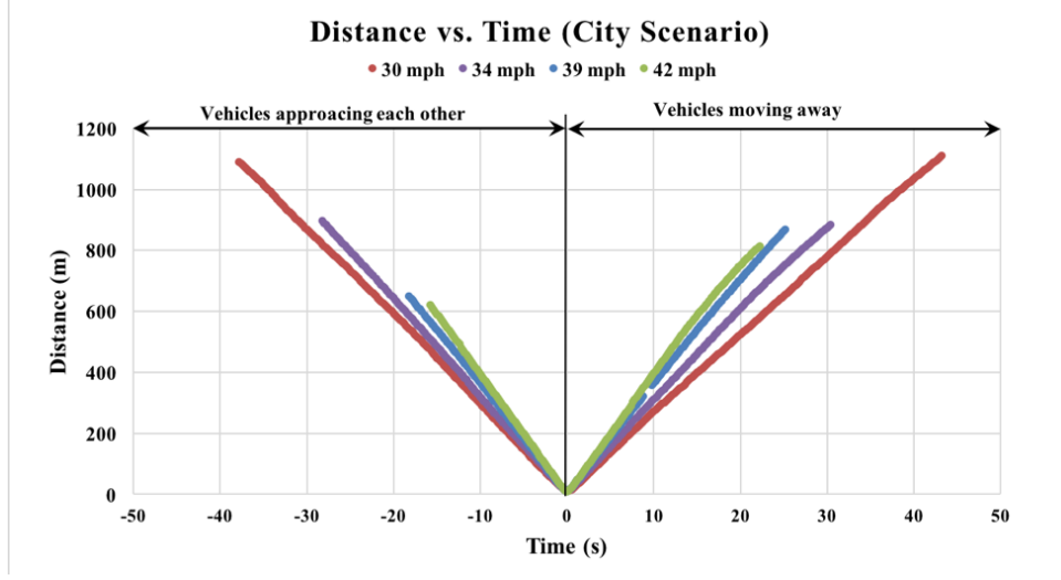
Figure 2.7: Duration of Connectivity and range for city environment (with rooftop OBU)
