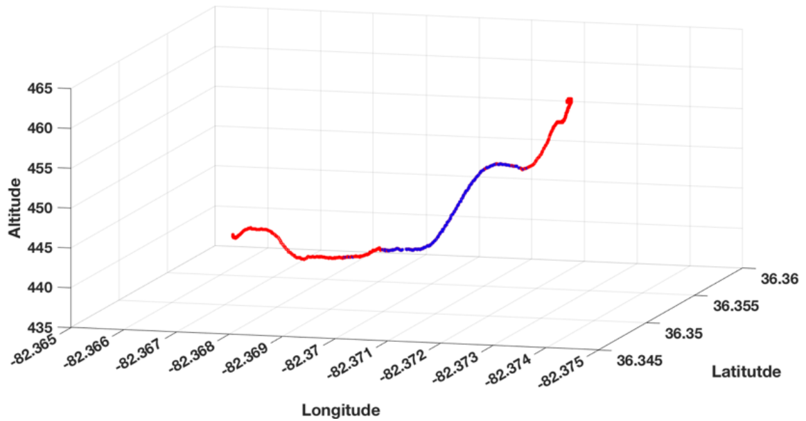
Figure 2.12: Altitude variation within the terrain (red dots indicate that no packet was received at that location)
