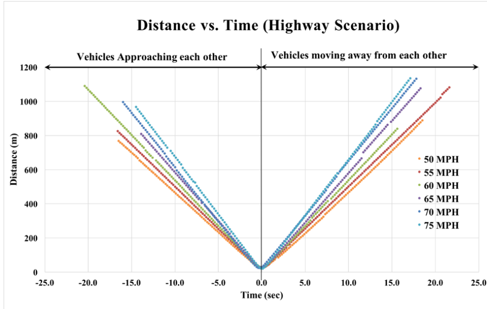
Figure 2.8: Duration of Connectivity and range for highway (with rooftop OBU)
