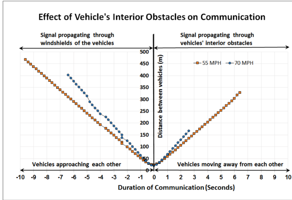
Figure 2.3: DSRC Communication range and duration between opposite vehicular traffic (with OBU placed inside the vehicles)
