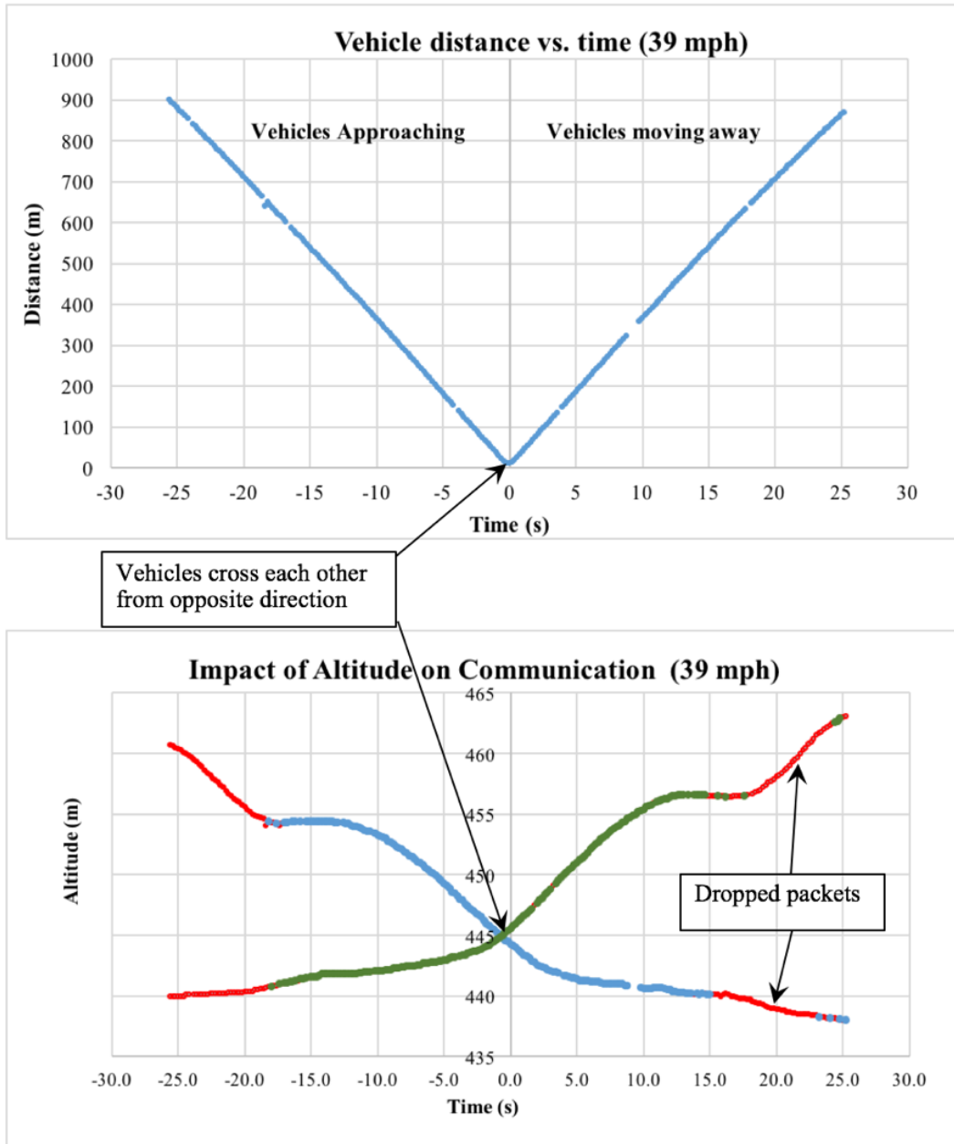
Figure 2.13: Unreliable V2V communication when one of the vehicles gets hidden by valley
