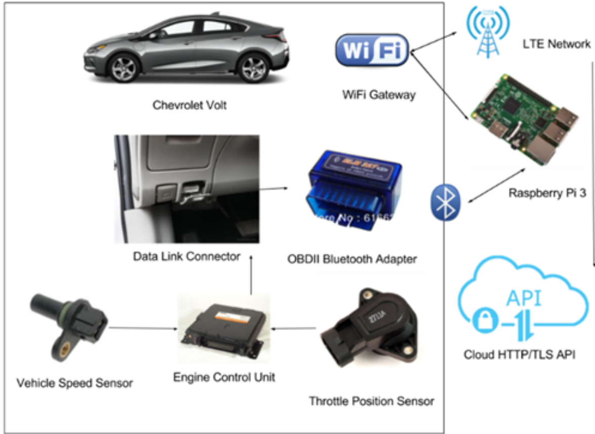
Figure 3.2: System architecture
