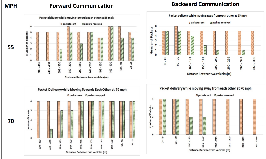
Figure 2.4: Packet delivery ratio for front and rear communication for 55 and 70 mph
