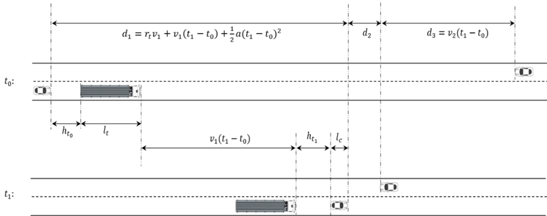
Figure 2.1: Conceptual Diagram to derive mathematical model
