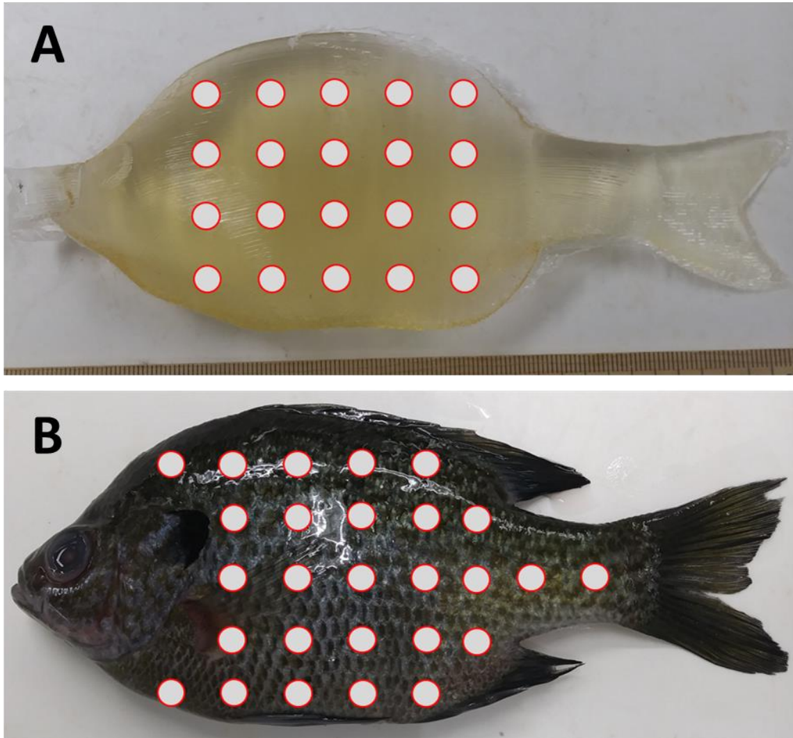
Figure 24. Relative durometer measurement locations (circles) were taken on the left side of (A) Gelfish cast without skin and (B) bluegill with scales. Durometer measurements were replicated for both Gelfish and actual bluegill, i.e., n = 3 for each. The Gelfish models and bluegill were ~16 cm total length and ~90 g mass. We also measured Gelfish with surrogate skin and bluegill without scales at the same approximate locations (not pictured).
