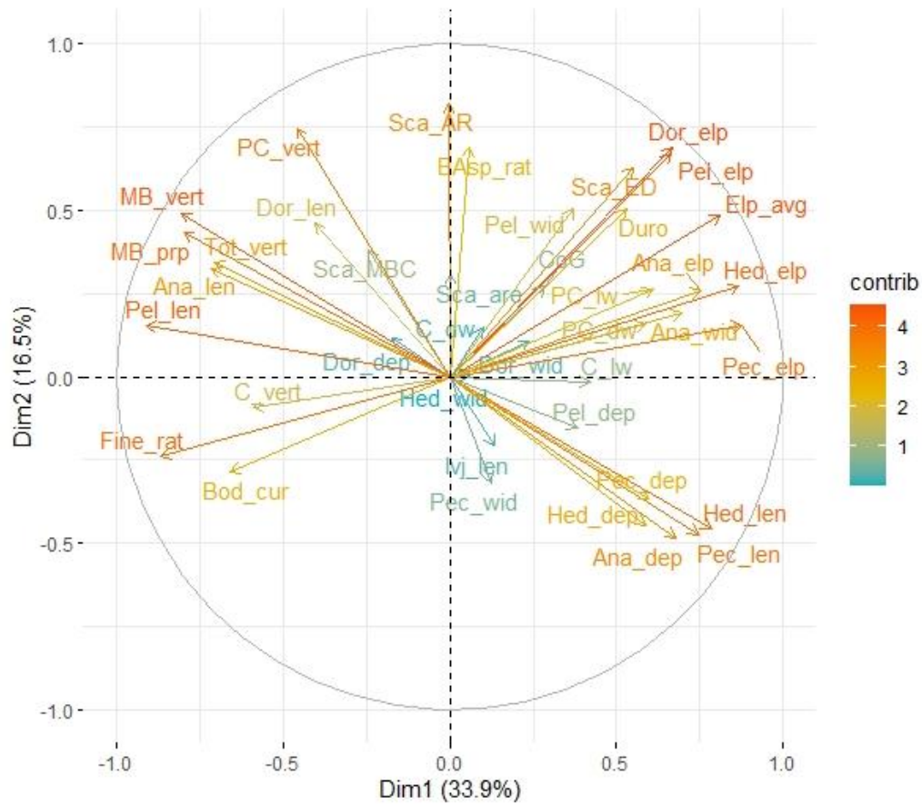
Figure 42. Contribution of each anatomorphic functional variable according to the first two principal component axes. Red colors indicate higher contribution to variation compared to blue colors.
