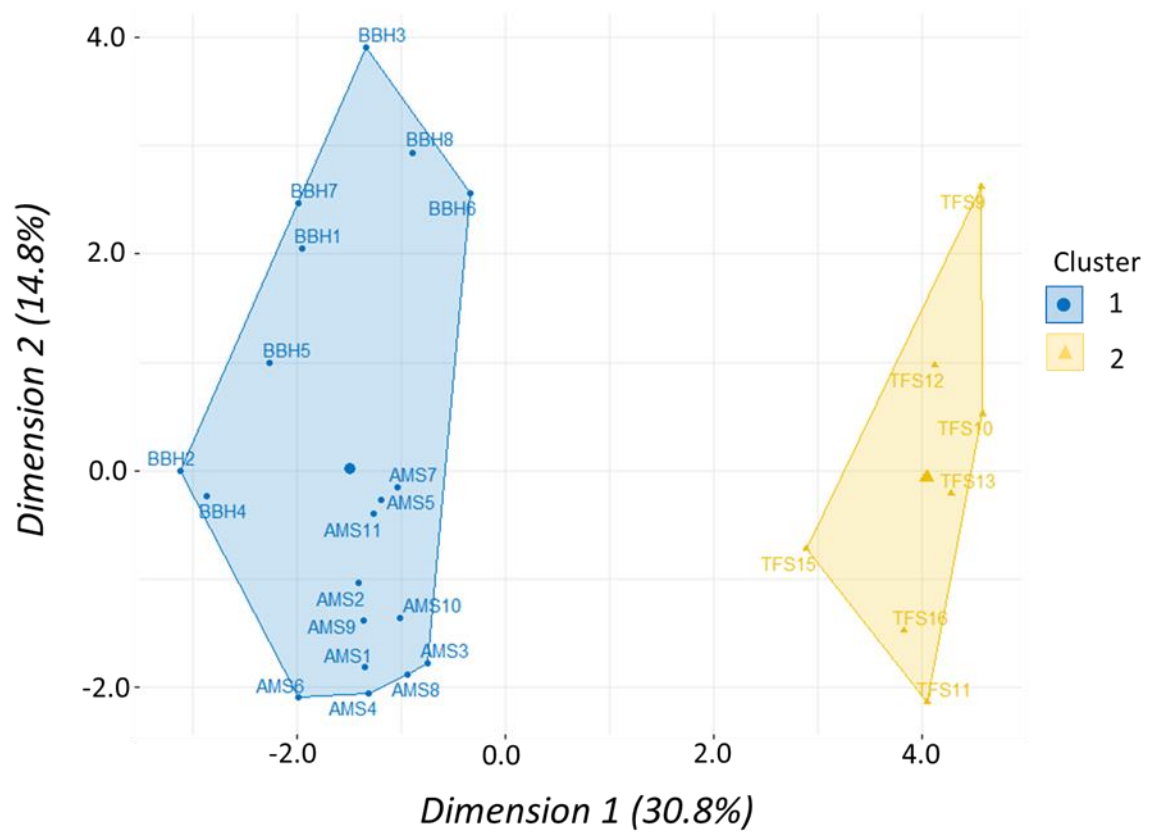
Figure 21. Cluster factor map produced from hierarchical clustering on six principal components for American shad (AMS), blueback herring (BBH), and threadfin shad (TFS) morphometric data.
