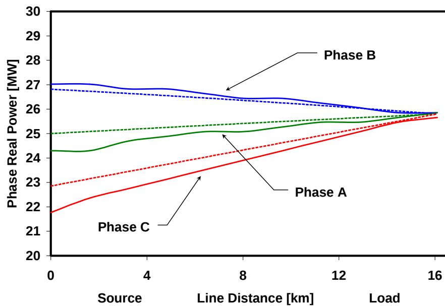
Figure (A.5) Phase real power of a 13.2 kV triaxial cable with an inductive load.
