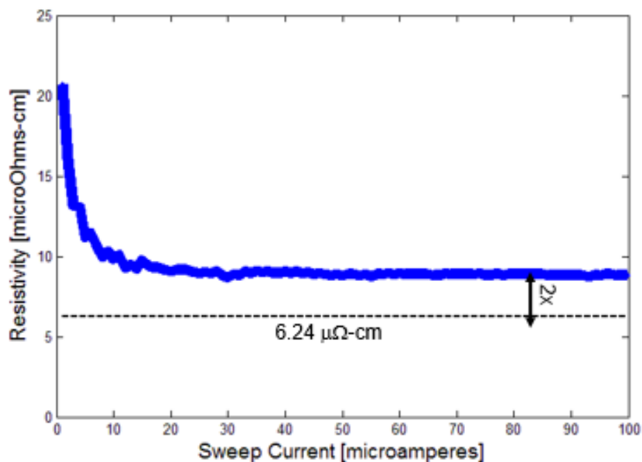
Figure 1.19. Calculated resistivity from the R-I curve for a Co NW made with a He ion beam.
