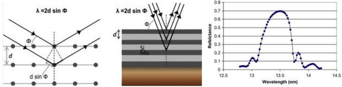
Figure 2.1. In a), Bragg's law showing constructive interference in a Mo/Si multilayer stack mirror, and in b), the reflectance from a Mo/Si mirror at near normal incidence [22].
