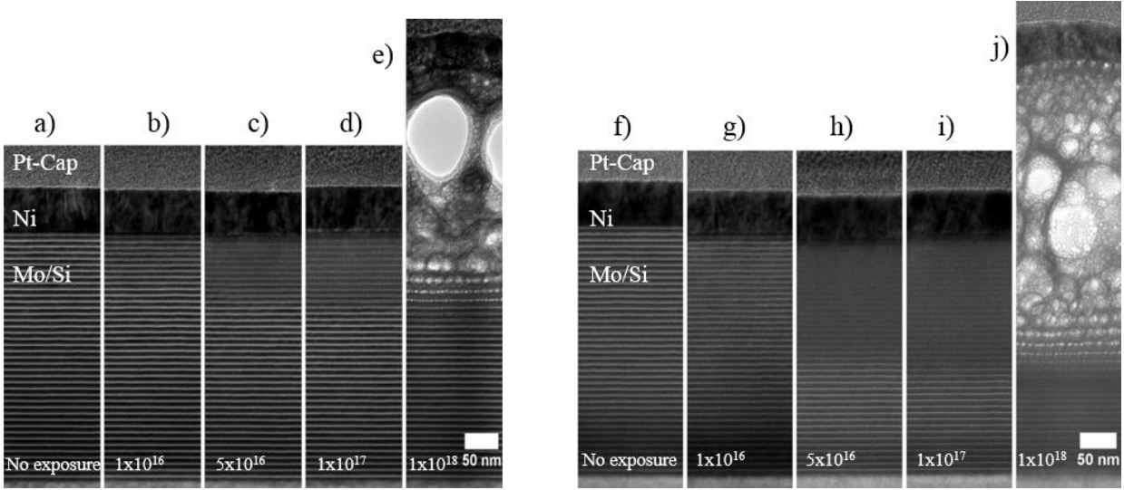
Figure 2.5. TEM cross-sectional micrographs of nickel on top of a Mo/Si multilayer stack that was exposed to 16 (a-e) and to 30 (f-j) keV helium ion energies in doses ranging from 1 \times 10^{16} to 1 \times 10^{18} ions/cm 2 . The direction of the incident He + beam is normal to the top side of each panel from a) to j). Ions travel from top down across the image until they come to rest. The silicon substrate is seen on the bottom of each micrograph and aligned with the adjacent images.
