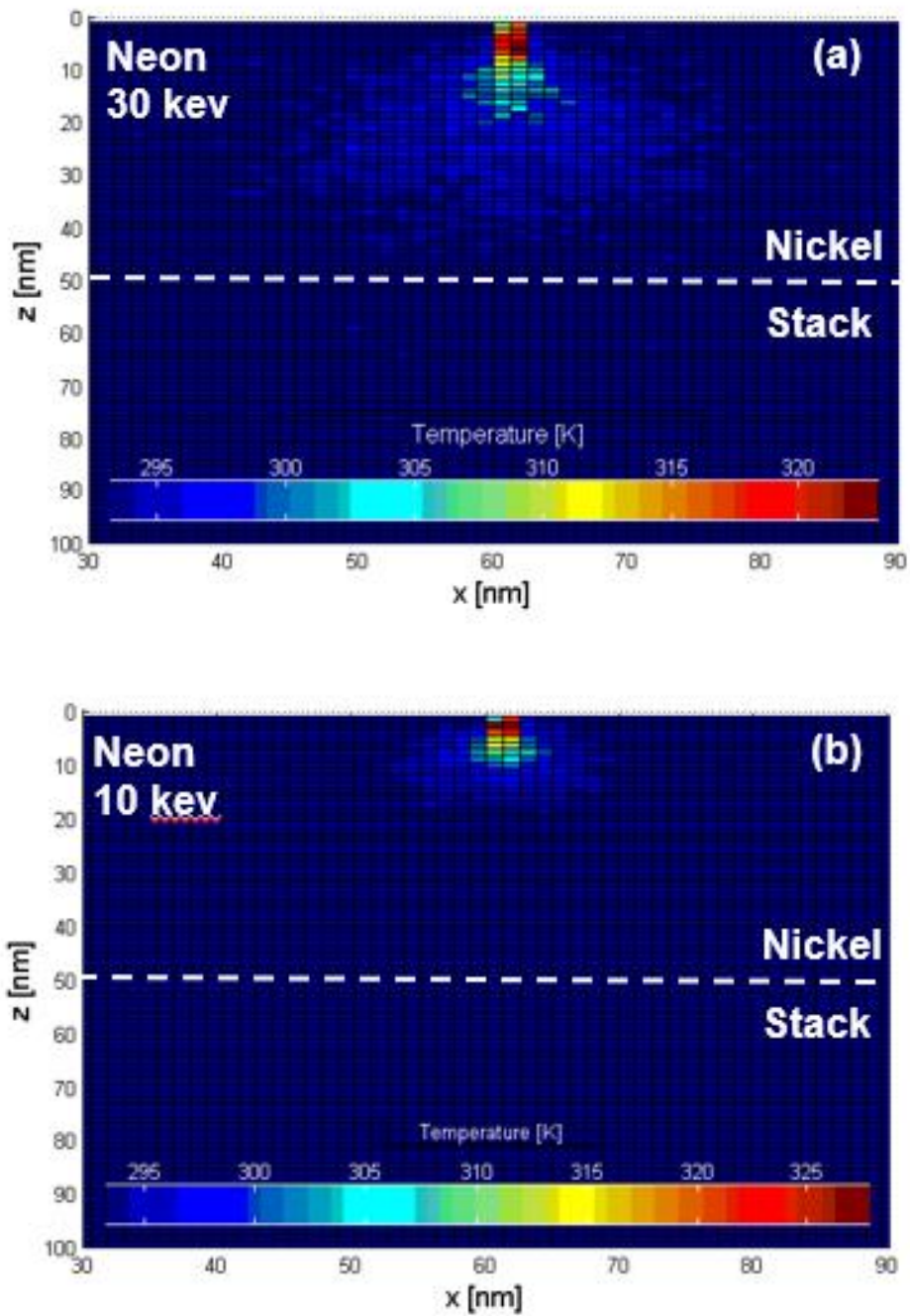
Figure 2.35. In this case, a comparison between 30 and 10 keV neon on the mirror structure. It shows how much more contained and closer to the top surface the temperature spikes are for the lower beam energy. Ion count=1000.
