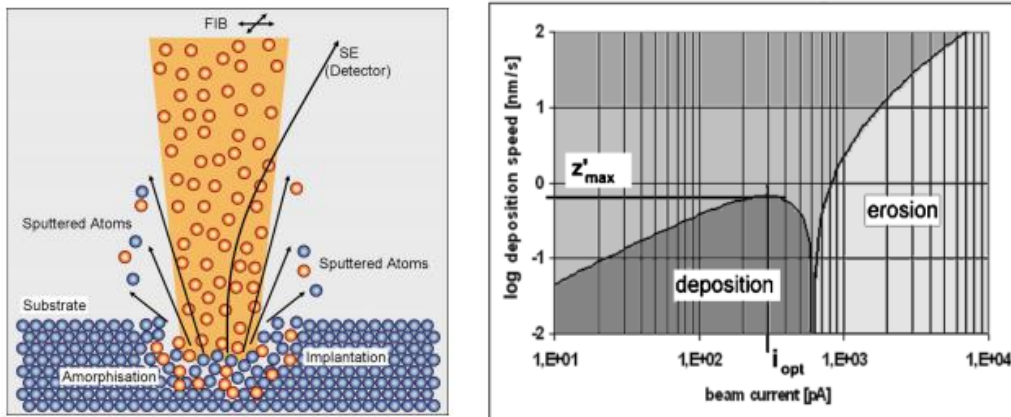
Figure 1.4. Principle of FIB milling or etching in a) [4], and in b), the dependence of deposition rate on the beam current at constant spot size [8].
