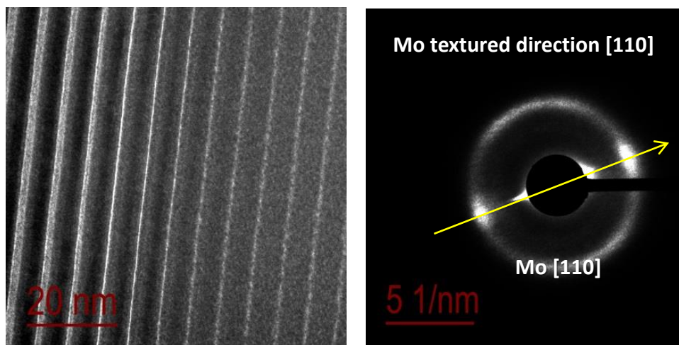
Figure 2.10. SAD analysis on the intermixed region in search of crystalline structure for Mo/Si, namely \text{MoSi}_2 . Diffraction peaks for polycrystalline Mo were identified, while otherwise only an amorphous ring for Mo/Si was observed.
