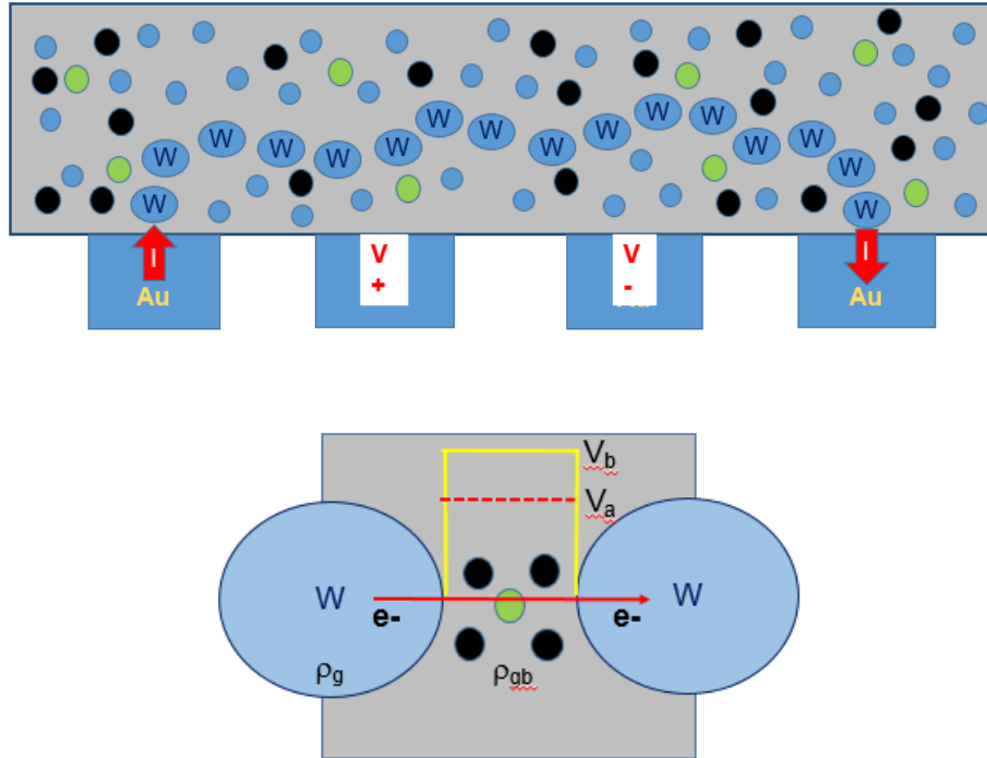
Figure 1.21. Diagrams showing the microstructure in a tungsten nanowire. In a) the entire path of least resistance from one terminal to another, and in b) a closer look at the region between two adjacent nanograins. In the later, the barrier ( V_b ) and applied voltages ( V_a ) are shown.
