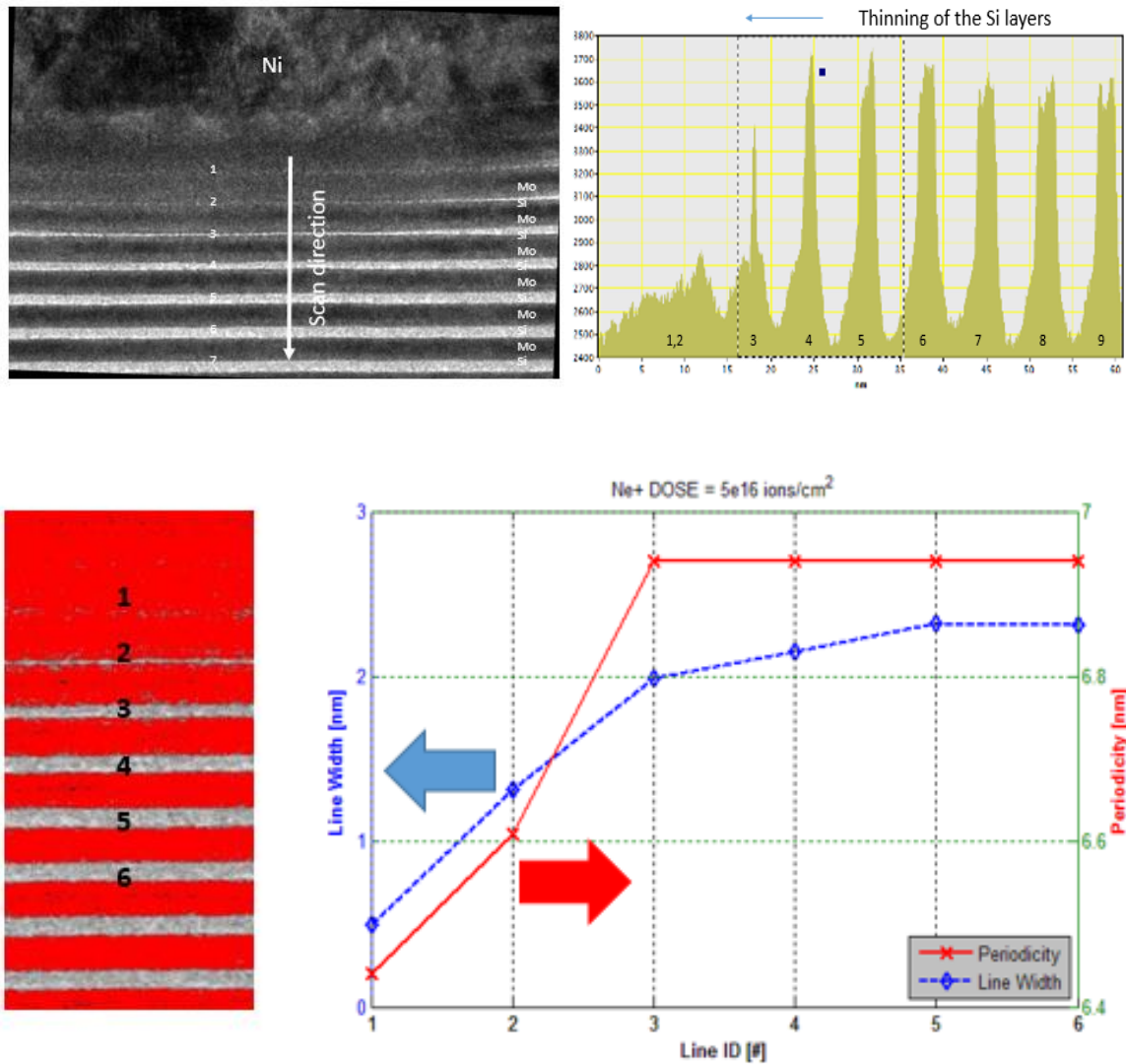
Figure 2.21. Closer look at the condition of a-Si layer in the stack closest to the beam irradiated, or damaged, region by neon. On the right, in b), a line profile showing the line widths increasing as the scan moved away from the irradiated zone. On c), a plot showing measurements for line width and for periodicity between the line centers for 24 keV Ne + and 5 \times 10^{16} ions/cm 2 .
