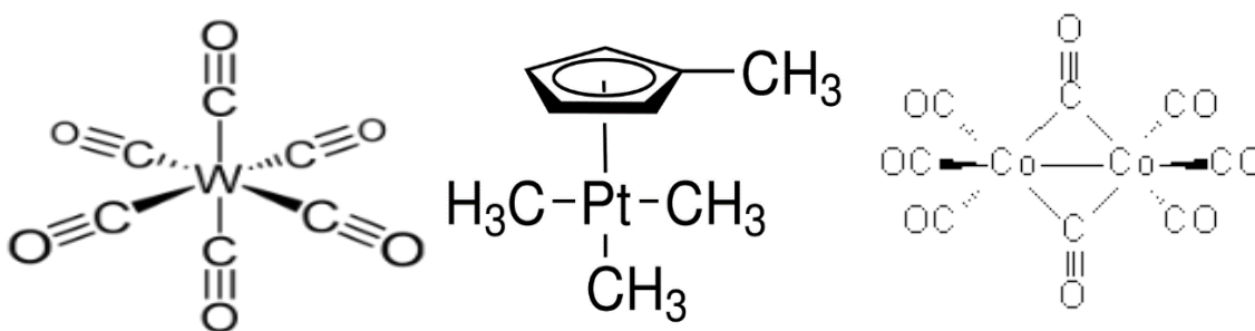
Figure 1.5. Depiction of molecular structures with ligands for \text{W(CO)}_6 in a), for \text{MeCpPtIVMe}_3 in b), and for \text{Co}_2(\text{CO})_8 in c).
