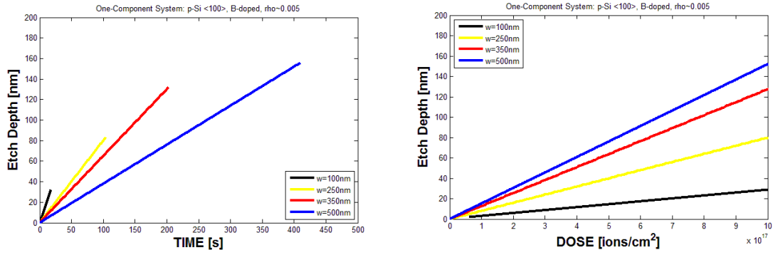
Figure 3.13. Etch depth dependencies on time and dose for a silicon substrate.
