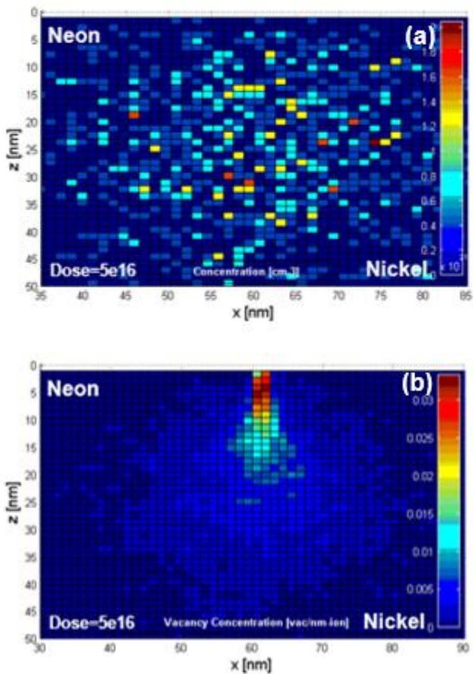
Figure 2.36. Implanted concentration and vacancy concentration profiles for neon ion bombardment at 5 \times 10^{16} \text{ Ne}^+/\text{cm}^2 .
