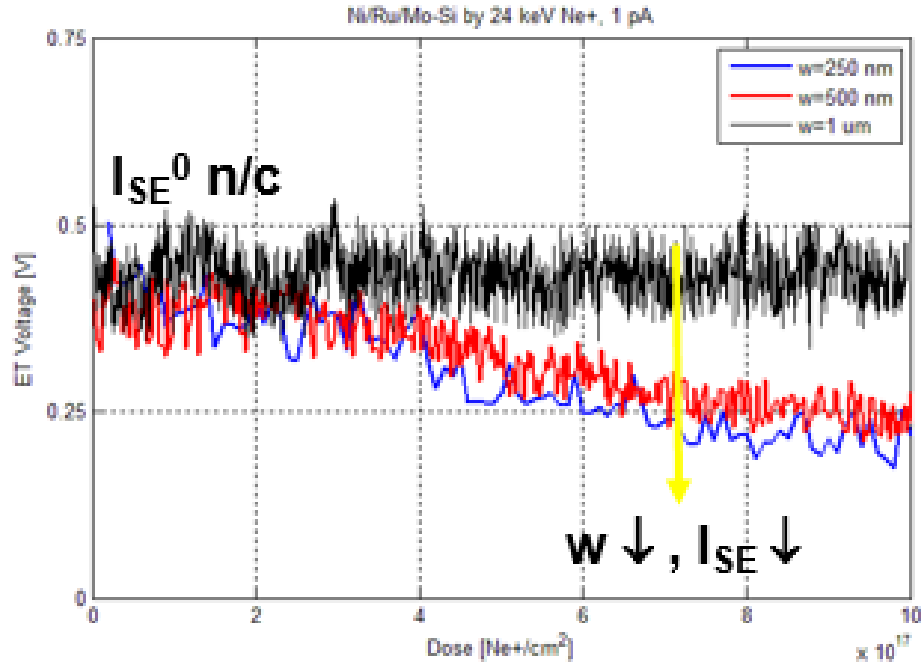
Figure 3.6. A dependence on box size, or width, found during etching of the EUV mask. Three (3) square box sizes, represented by their widths, are shown, where the smaller the width, the greater the slope, or reduction rate in SEs reaching the E-T detector.
