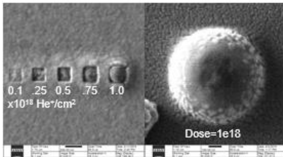
Figure 3.22. HIM image showing a dose study of Au etching by \text{He}^+ (in a) and a closer look at archetypal blistering at high dose (in b).
