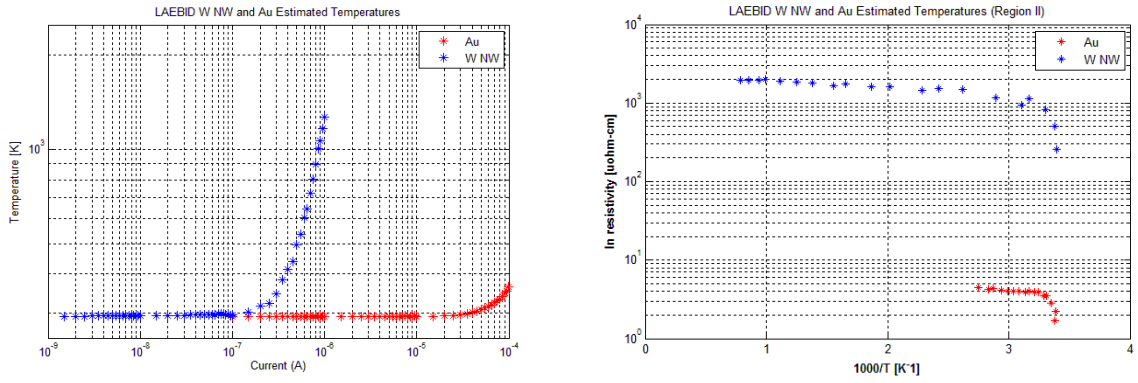
Figure 1.27. On left (a), the estimated temperature as a function of the applied current, and on the right (b), the estimated resistivity dependence on temperature. Both, the W NW (in blue) and Au reference (in red) shown.
