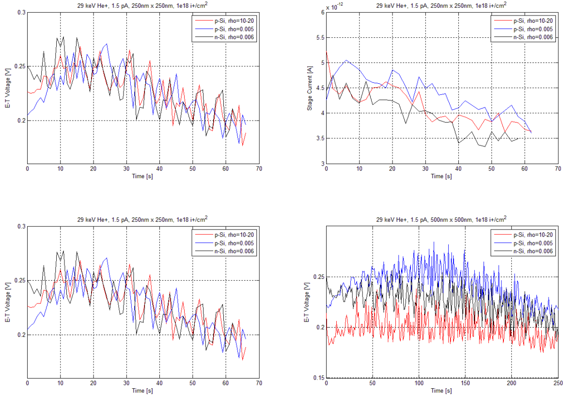
Figure 3.10. At w=250 nm (in a), and at w=500 nm (in b), the signals collected from the E-T detector for 29 keV \text{He}^+ in three (3) different c-Si substrates.
