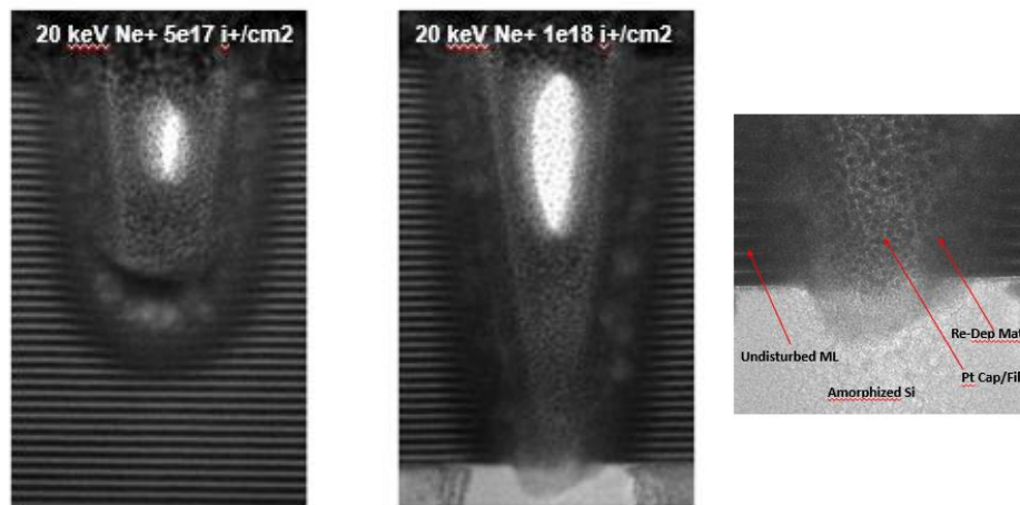
Figure 2.39. Etch profiles at 50 KX for 5x10 17 (in a) and 1x10 18 (in b) Ne + /cm 2 . A closer look (200 KX) near the bottom of the via in c).
