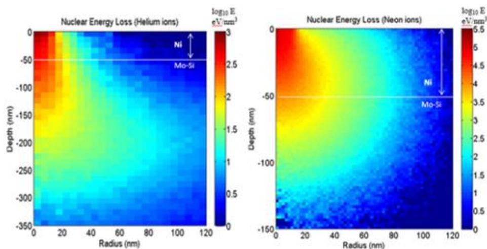
Figure 2.27. Comparison of the simulated volumetric nuclear energy losses of helium and of neon at 30 keV. EnvizION runs of 100k ions corresponded to a dose of \sim 1 \times 10^{17} He + /cm 2 , and of 150k ions corresponded to a dose of \sim 2 \times 10^{17} Ne + /cm 2 .
