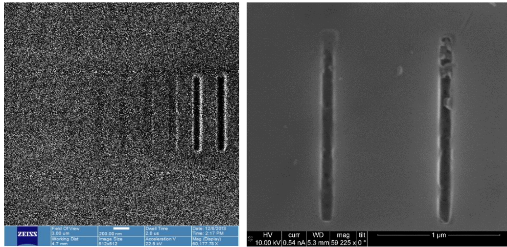
Figure 2.16. Top Ne-HIM view of etched lines (a), and top SEM view for two etched lines.
