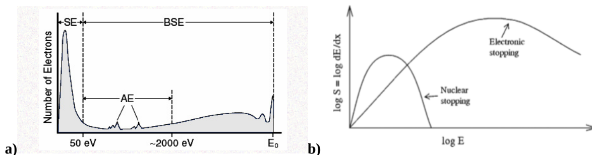
Figure 1.1. In a), the energy ranges for SE, AE and BSE electrons with respect to the primary beam energy [1], and in b), energy losses for ions due to nuclear and electronic interactions [2].
