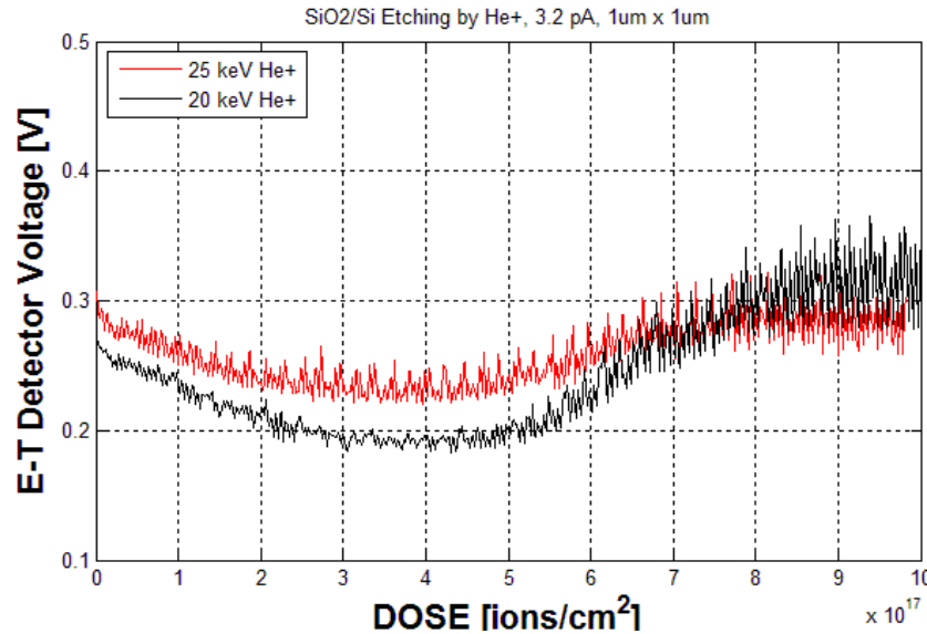
Figure 3.20. Data collected from the E-T detector for helium in SiO 2 /Si at two (2) different beam energies (25 & 20 keV).
