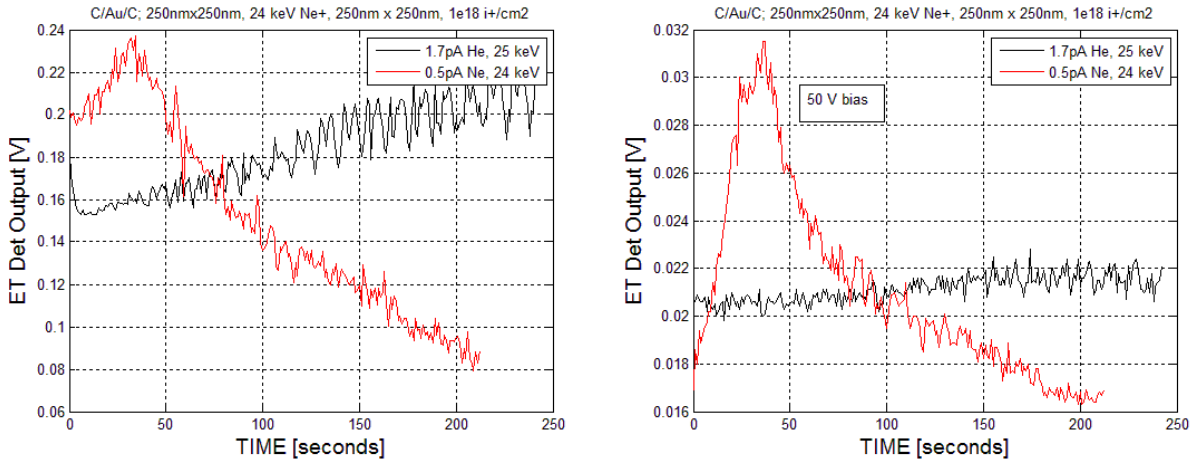
Figure 3.40. Comparison between helium and neon etching of C/Au/C and at two (2) stage biases (0 V, +50V).
