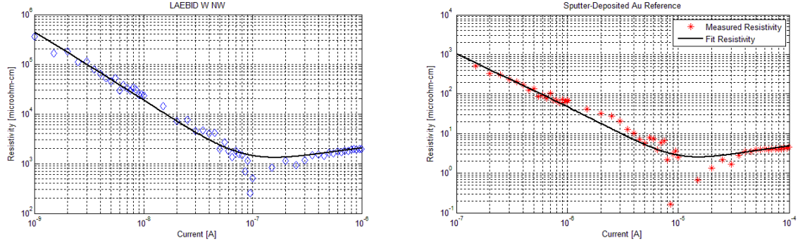
Figure 1.26. Calculated \rho ( =AR/L ) from measured data versus current and fit using the power law (region I) and logarithmic functions (region II) for the W NW (on a), and the Au reference (on b).
