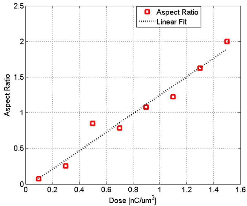
Figure 2.18. Via aspect ratios for 30 keV Ne + exposures of doses ranging from 0.1 to 1.5 nC/μm 2 .
