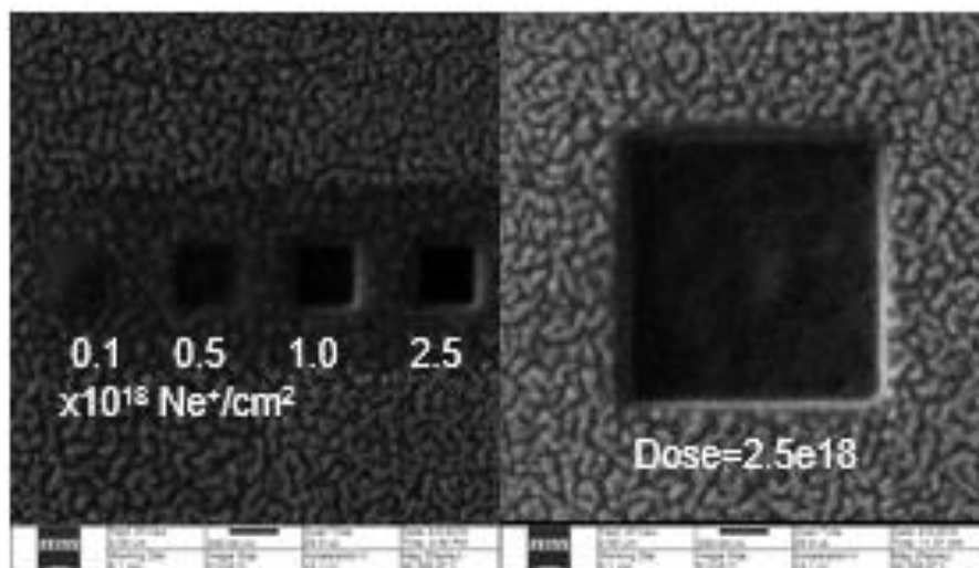
Figure 3.23. NIM image showing a dose study of Au etching by \text{Ne}^+ (in a) and a closer look at the high dose etch (in b).
