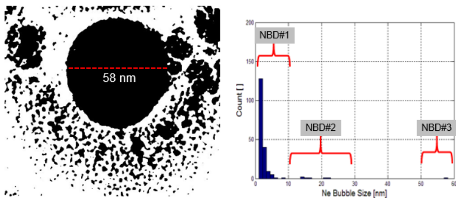
Figure 2.23. For 30 keV Ne + and 4 \times 10^{17} ions/cm 2 , showing in a) the TEM adjusted image with different contrast limits (min, max) and brightness in order to do a particle size analysis as in the histogram on the right (b). Area was converted to diameter by assuming all were circular.
