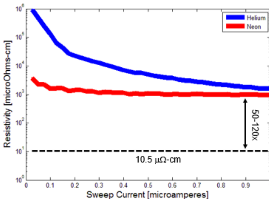
Figure 1.13. For Pt NW deposited using He and Ne, resistivity data for the range between 10 nA to 1 \mu\text{A} , and compared with the target bulk value for platinum.
