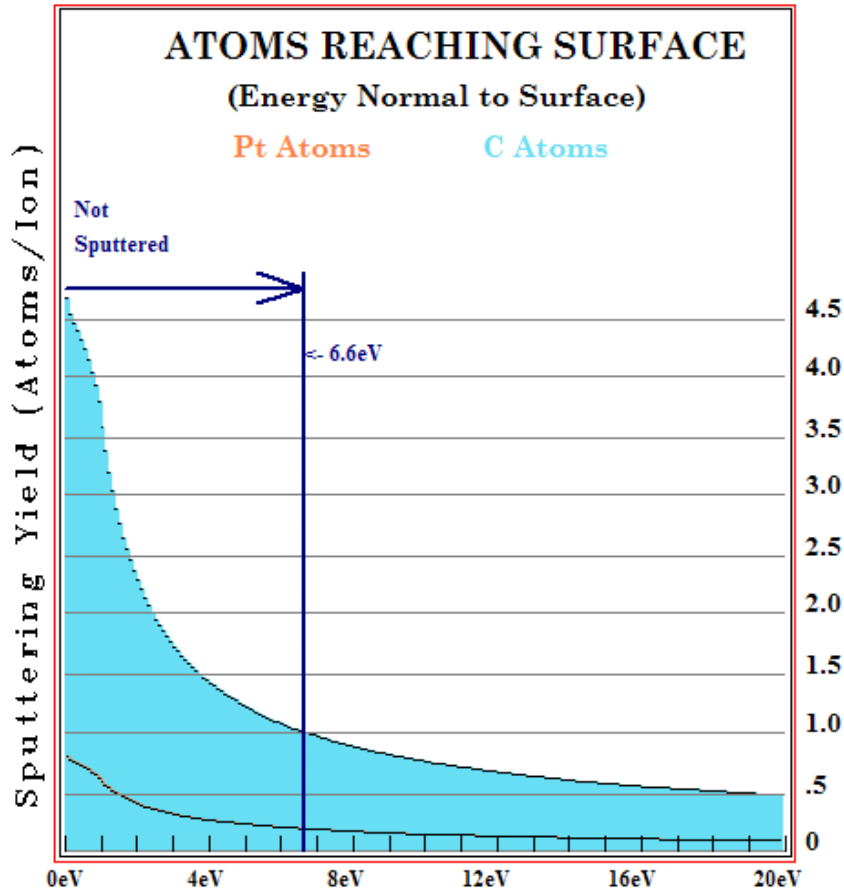
Figure 1.16. Sputtering yields of Pt and C by \text{Ne}^+ at 20 keV from SRIM/TRIM simulations.
