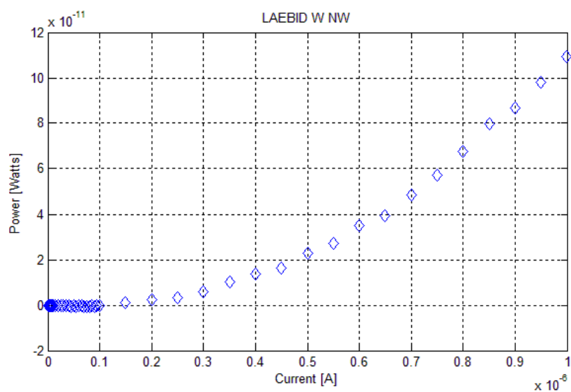
Figure 1.23. Calculated Power ( =VI ) from measured data versus current for the W NW.
