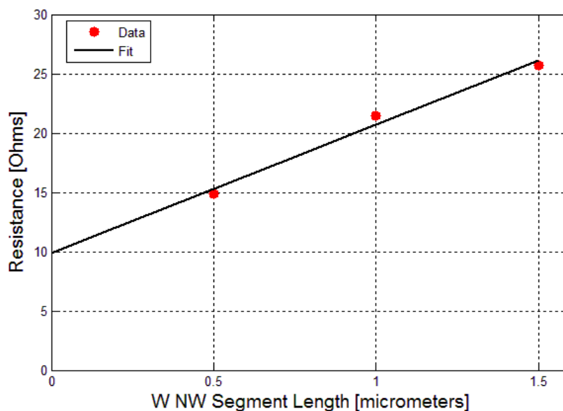
Figure 1.12. Data from Figure 1.11b plotted to determine the contact resistance, R_C , for the W NW. This corresponds to two series contact surfaces with the nanowire, each contributing 4.94 \Omega .
