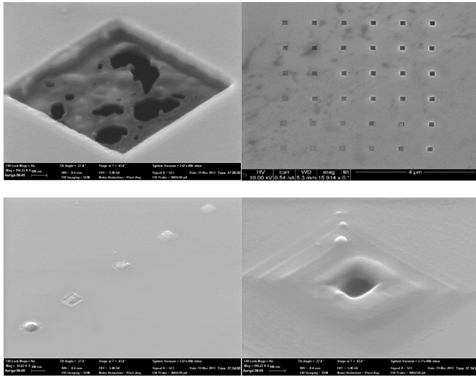
Figure 2.15. A 1\mu\text{m}^2 etch box by neon on \text{Ni}(50\text{ nm})/\text{SiO}_2/\text{Si} (in a). In b), a 6x6 array of 200nm x 200nm etched nanoholes on the nickel top layer in the same sample as in a). Doses increased from left to right on each row. In c) and d), results of using the reactive gas, \text{XeF}_2 , along with the \text{Ne}^+ beam, on the nickel surface.
