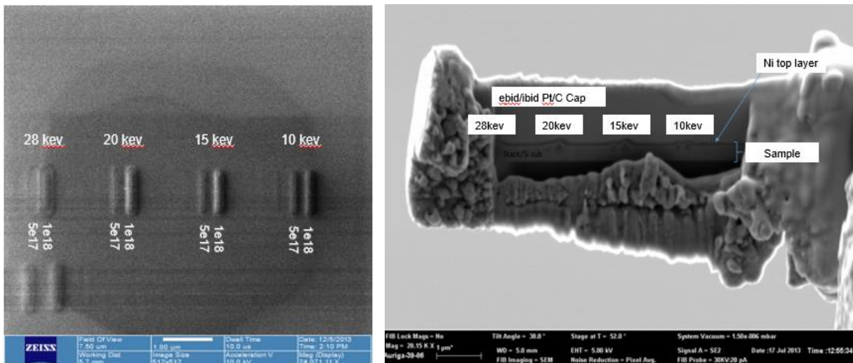
Figure 2.28. Helium energy study. Top HIM (in a) and lamellae side SEM (in b) views.
