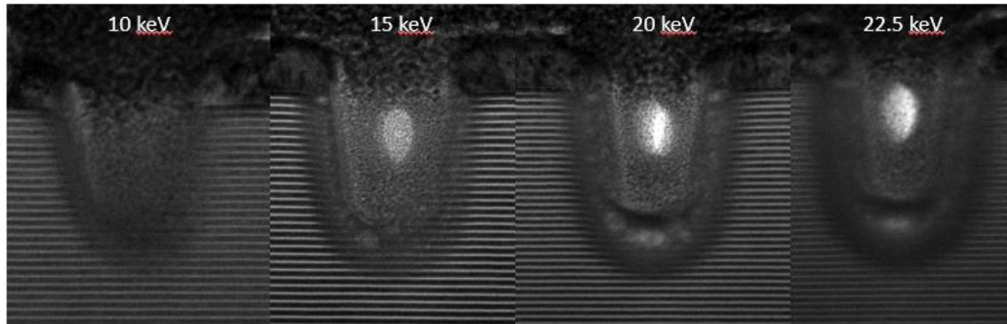
Figure 2.30. Energy study TEM images for neon ion beam etching at 5 \times 10^{17} \text{ Ne}^+/\text{cm}^2 and energies between 10 and 22.5 keV.
