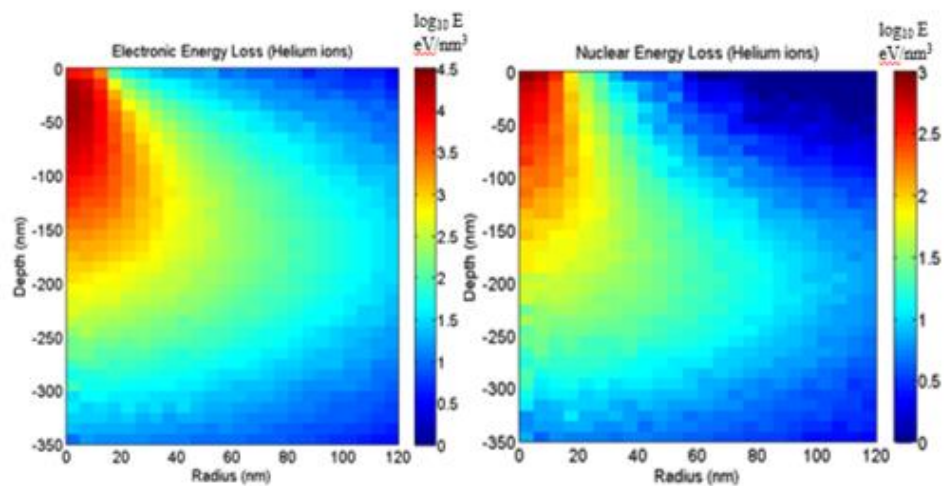
Figure 2.13. Simulated electronic and the nuclear volumetric energy losses for helium ions at 30 keV at a dose of 1 \times 10^{17} ions/ \text{cm}^2 .
