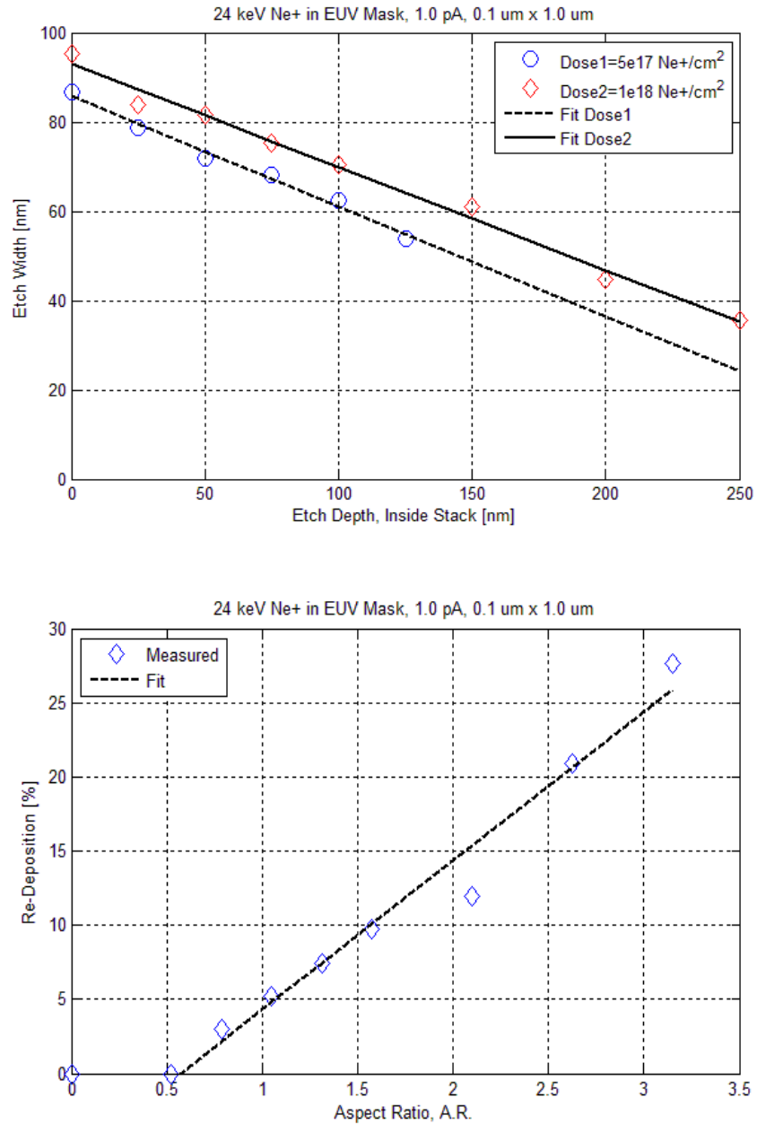
Figure 2.40. Plots showing the change in width and its slope as a function of milling depth, for each case in figure 2.40, and another plot with the re-deposition percentage as a function of aspect ratio ( h/w ).
