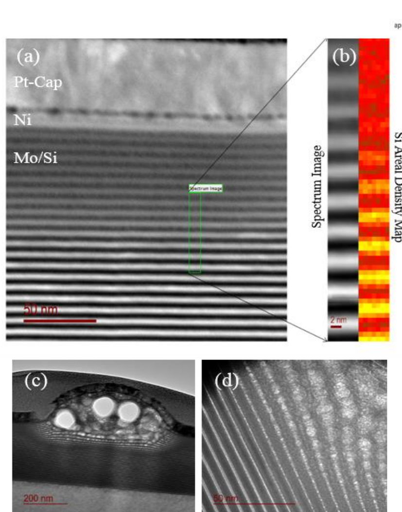
Figure 2.7. High magnification Z-contrast image of a 30 keV, 1 \times 10^{17} \text{He}^+/\text{cm}^2 exposure (a). Spectrum image and a silicon areal density map (b). At higher doses, such as 1 \times 10^{18} \text{He}^+/\text{cm}^2 severe bubbling is observed which originates preferentially in the silicon layer of the stack, as shown in c & d.
