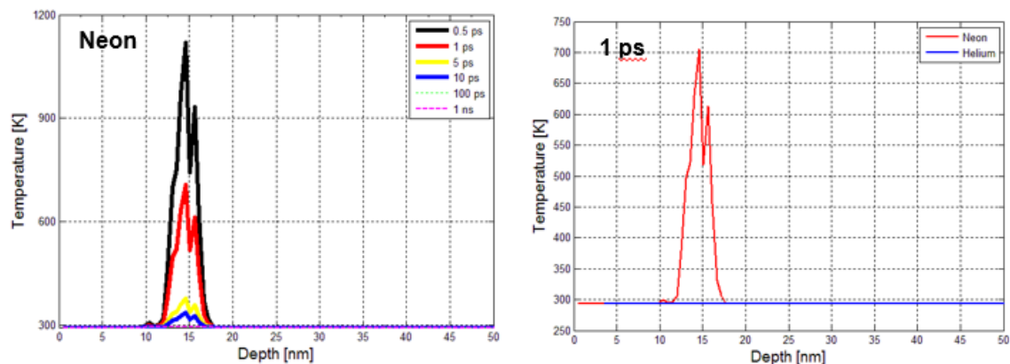
Figure 2.32. On the left in a) the temperature profile versus time showing the rapid quench rate for thermal spike. On the right, in b) a comparison between a neon and a helium thermal spike 1 ps after the ion strike.
