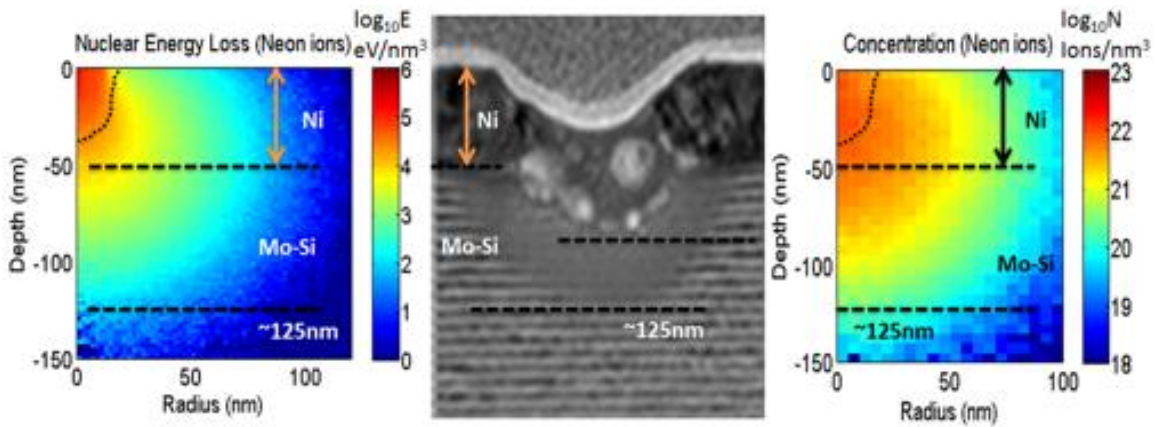
Figure 2.26. Simulated nuclear energy loss (left) and the resultant neon implant concentrations (on right) are compared to the experimental TEM micrograph exposed to 30 keV at a dose of 2 \times 10^{17} \text{ Ne}^+/\text{cm}^2 .
