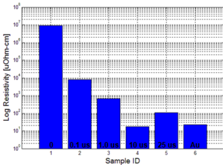
Figure 1.8. Bar plot showing the relative resistivity calculations for the six (6) samples measured at 10 \mu A.
