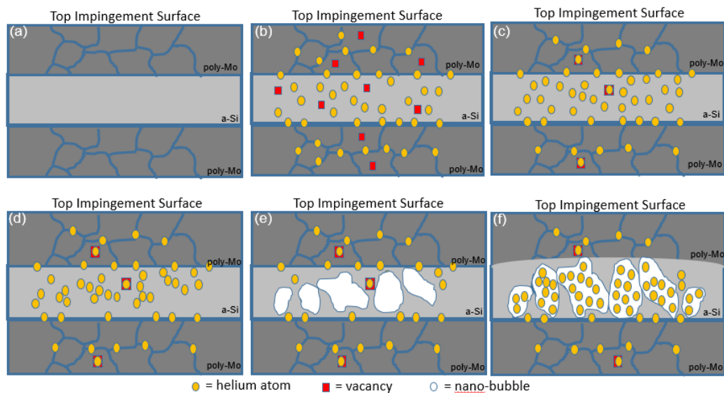
Figure 2.37. Diagram showing the evolution of individual implanted helium and defects leading to the formation of nanobubbles preferentially located in the amorphous silicon layer.
