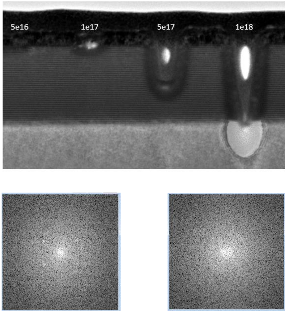
Figure 2.31. For a \text{Ne}^+ beam energy of 22.5 keV, the exposures from 5 \times 10^{16} to 1 \times 10^{18} \text{ Ne}^+/\text{cm}^2 . In b) below, the diffraction pattern for the silicon substrate, and in c) the same but within the region affected by the beam after a 1 \times 10^{18} \text{ Ne}^+/\text{cm}^2 on the structure.
