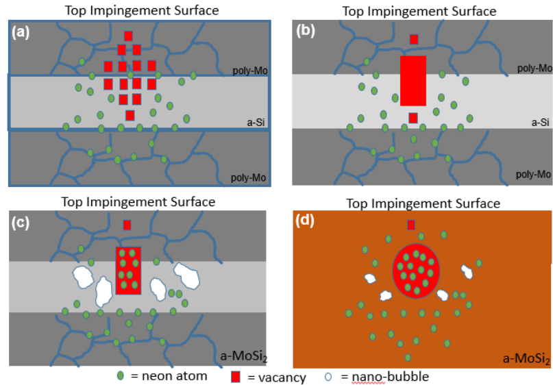
Figure 2.38. Diagram showing the evolution of individual implanted neon and defects leading to the formation of nanobubbles and ultimately Ostwald ripening.
