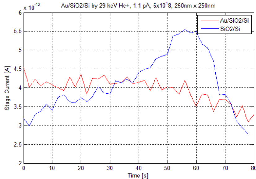
Figure 3.28. Signals for Au/SiO 2 /c-Si undergoing helium etching. When Au (100 nm) is present, it acts as a mask, and swelling is not observed up to 5 \times 10^{18} He + /cm 2 (red trace). On the other hand, when the implantation begins on SiO 2 /Si (no Au cap), swelling begins at low doses (blue trace).
