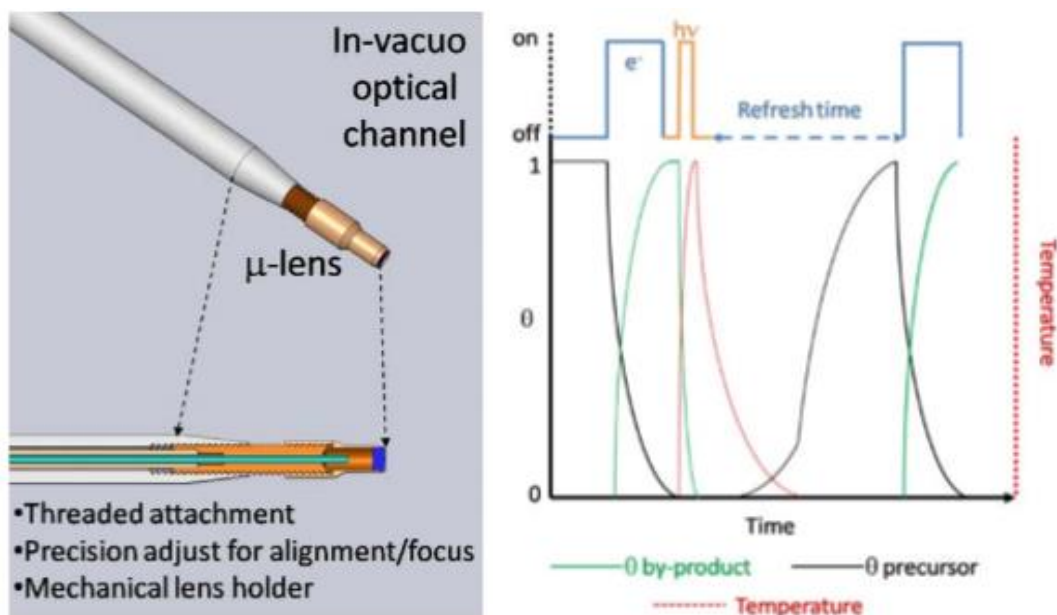
Figure 1.7. Microlens positioned at the end of the fiber optic mounted on the Opto-probe assembly. Idealized schematic depicting deposition process via EBID where precursor gas pulses are followed by a short laser pulse after each pass.
