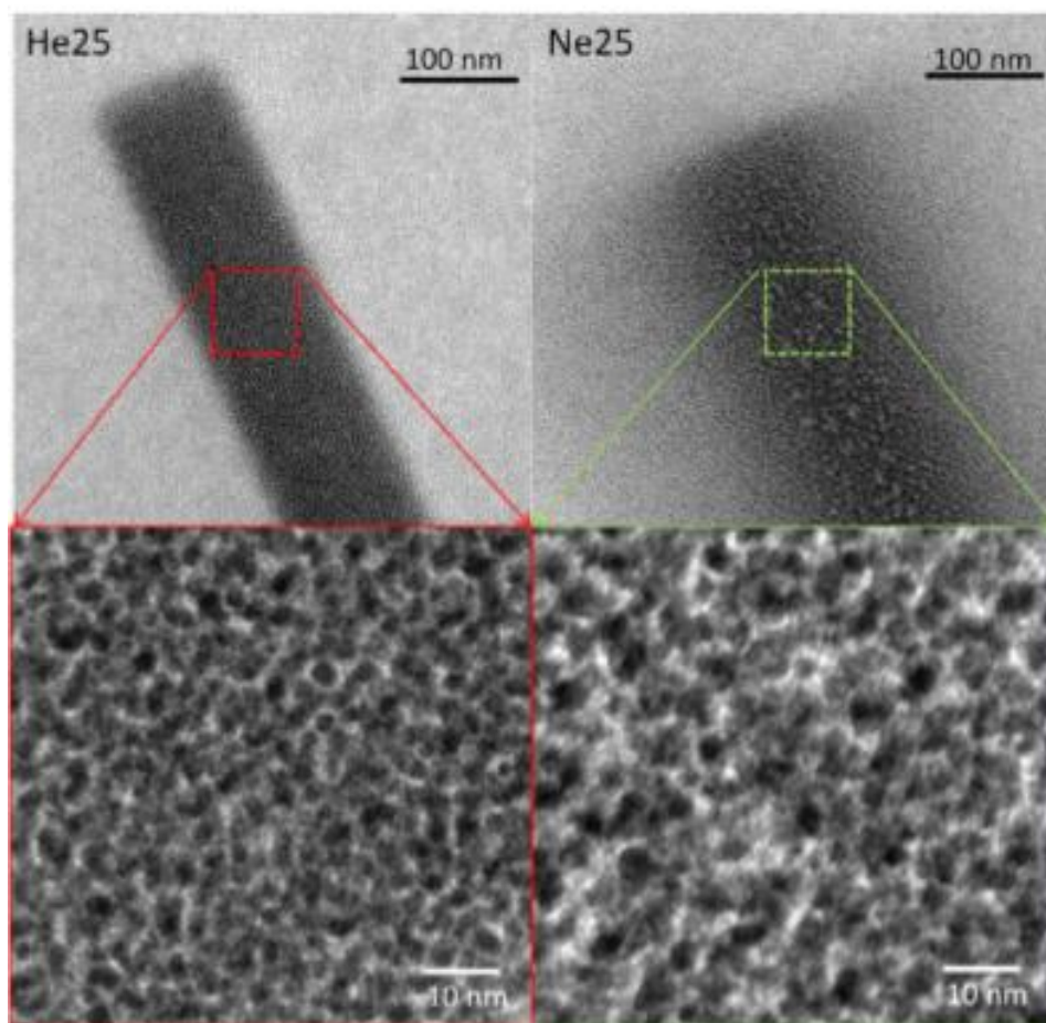
Figure 1.14. Comparison of nanostructures between \text{He}^+ (in a) and \text{Ne}^+ (in b) induced deposition of Pt. The grain sizes are clearly larger on the Ne-BID Pt NW.
