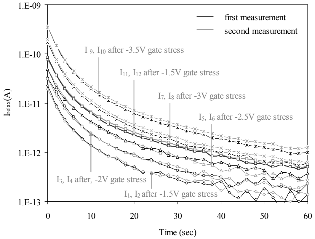
Figure13. Relaxation current decay with time of TiN/ 45s-deposited ZrHfO/1nm SiON/ p -Si Stack. The stress and measurement methods are shown in Figure 12.
