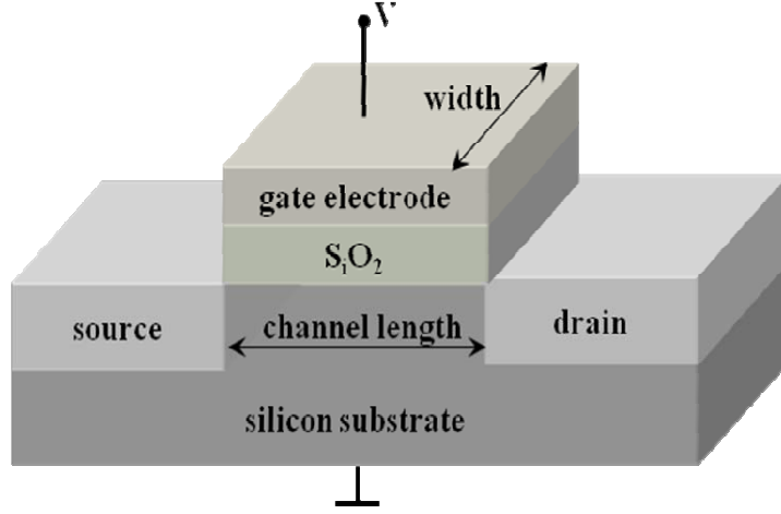
Figure 1. Schematic diagram of a MOSFET
