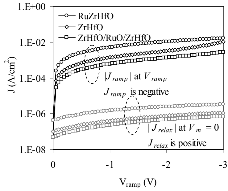
Figure 21. Ramp-relax test results of TiN/ZrHfO/RuO/ZrHfO/p-Si stack
