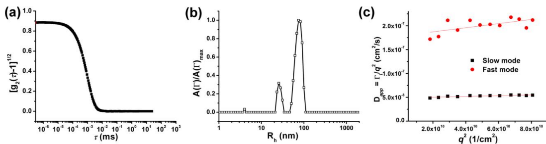
Figure A-27. Light intensity autocorrelation function (a), hydrodynamic radii, R_h , distributions (b) and apparent diffusion coefficient D_{app} versus q^2 (c) for mixture T1+S7 in toluene at c = 8.0 mg/mL.
