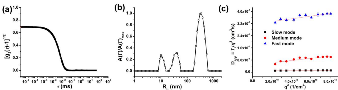
Figure A-20. Light intensity autocorrelation function (a), hydrodynamic radii, R_h , distributions (b) and apparent diffusion coefficient D_{app} versus q^2 (c) for mixture D1+S3 in toluene at c = 8.0 mg/mL.
