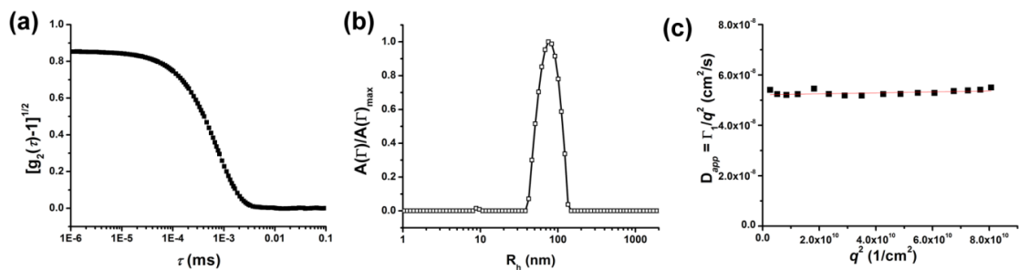
Figure A-13. Light intensity autocorrelation function (a), hydrodynamic radii, R_h , distributions (b) and apparent diffusion coefficient D_{app} versus q^2 (c) for sample S8 in toluene at c = 1.0 mg/mL.
