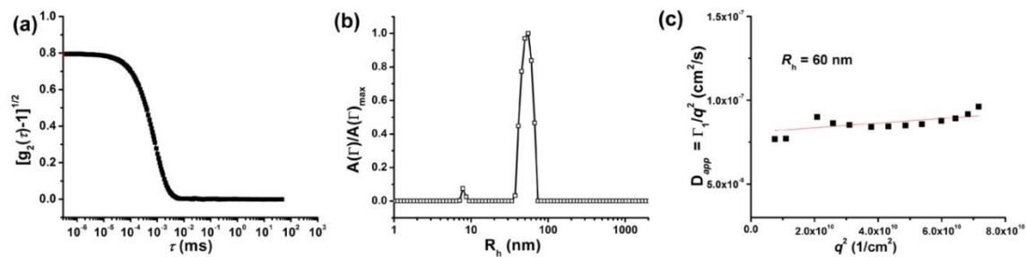
Figure A-33. Light intensity autocorrelation function (a), hydrodynamic radii, R_h , distributions (b) and apparent diffusion coefficient D_{app} versus q^2 (c) for sample S8 in THF at c = 0.5 mg/mL.
