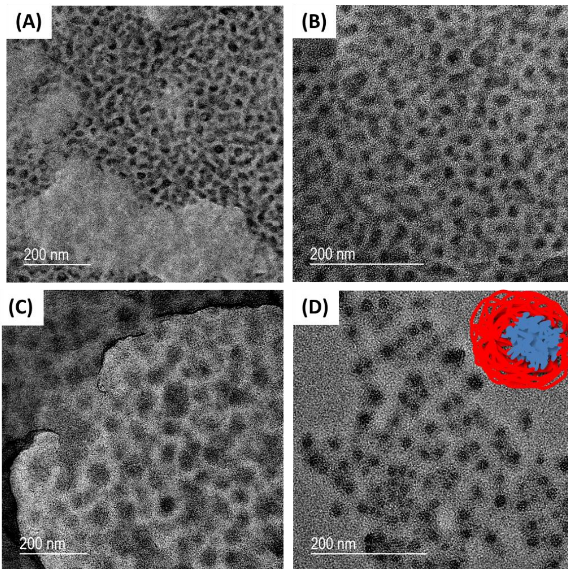
Figure 4-5. TEM images of (A) the 40-arm star [PS 53.8 -PVP 53.8 ] 40 , and (B) the 26-arm star [PS 50 -PVP 50 ] 26 drop cast from toluene solutions with PVP blocks stained by iodine vapor. TEM image of (C) [PS 53.8 -PVP 53.8 ] 40 drop cast from toluene solution with both PS and PVP blocks stained using RuO 4 . TEM image of doubly-stained (D) [PS 53.8 -PVP 53.8 ] 40 deposited from a toluene solution containing gold (III), which coordinates with PVP blocks. The dried film is subsequently exposed to RuO 4 vapors. This double staining method renders the PVP blocks
