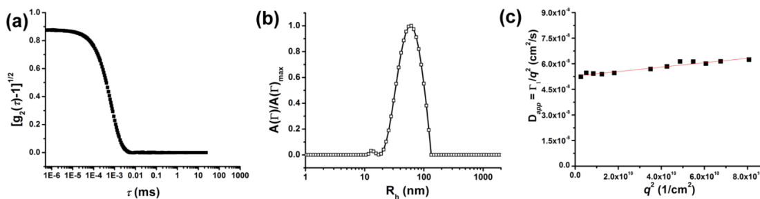
Figure A-10. Light intensity autocorrelation function (a), hydrodynamic radii, R_h , distributions (b) and apparent diffusion coefficient D_{app} versus q^2 (c) for sample S5 in toluene at c = 1.0 mg/mL.
