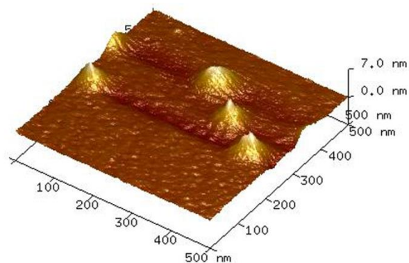
Figure A-34. 3D AFM image of disperse micelles made by drop-casting from S7 toluene solution at c = 3.0 \mu g/mL on a silicon substrate.
