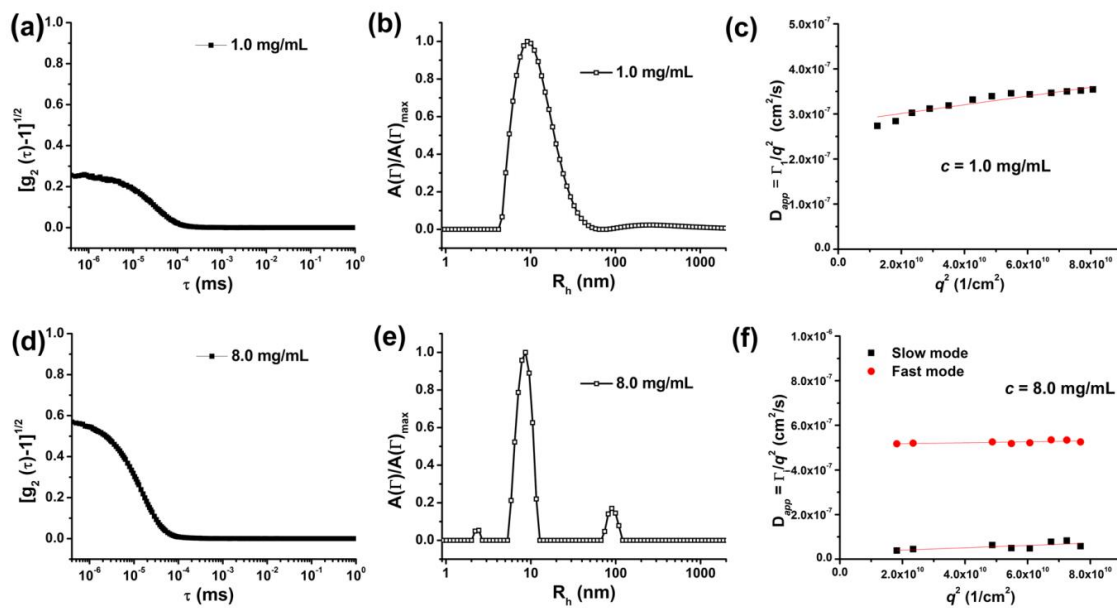
Figure A-4. Light intensity autocorrelation function (a, d), hydrodynamic radii, R_h , distributions (b, e) and apparent diffusion coefficient D_{\text{app}} versus q^2 (c, f) for sample T2 in toluene at c = 1.0 mg/mL (a, b, c) and at c = 8.0 mg/mL (d, e, f).
