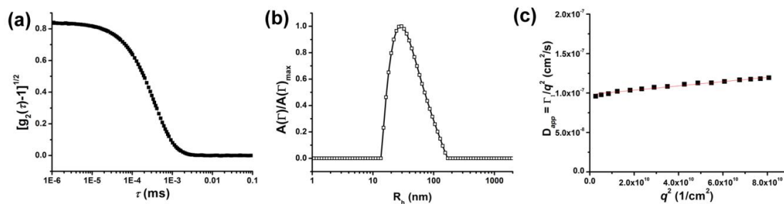
Figure A-9. Light intensity autocorrelation function (a), hydrodynamic radii, R_h , distributions (b) and apparent diffusion coefficient D_{app} versus q^2 (c) for sample S4 in toluene at c = 1.0 mg/mL.
