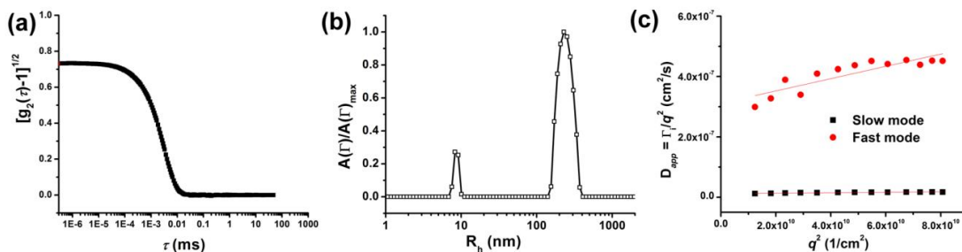
Figure A-16. Light intensity autocorrelation function (a), hydrodynamic radii, R_h , distributions (b) and apparent diffusion coefficient D_{app} versus q^2 (c) for mixture D1+T2 in toluene at c = 8.0 mg/mL.
