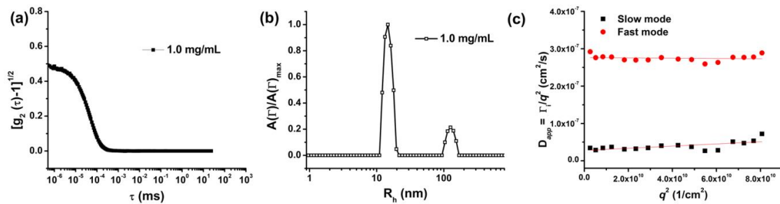
Figure A-3. Light intensity autocorrelation function (a), hydrodynamic radii, R_h , distributions (b) and apparent diffusion coefficient D_{\text{app}} versus q^2 (c) for sample D3 in toluene at c = 1.0 mg/mL.
