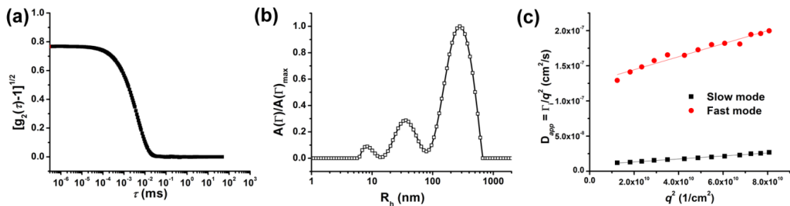
Figure A-21. Light intensity autocorrelation function (a), hydrodynamic radii, R_h , distributions (b) and apparent diffusion coefficient D_{app} versus q^2 (c) for mixture D1+S4 in toluene at c = 8.0 mg/mL.
