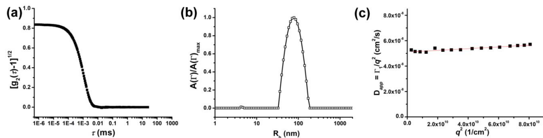
Figure A-14. Light intensity autocorrelation function (a), hydrodynamic radii, R_h , distributions (b) and apparent diffusion coefficient D_{app} versus q^2 (c) for sample S9 in toluene at c = 1.0 mg/mL.
