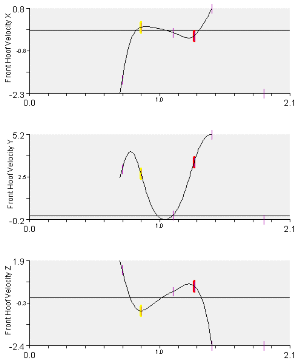
Figure A-5: Graphs of Front Hoof Velocities in All Three Axes. Bolded marks on line are left front heel strike and left front toe off (left to right).
