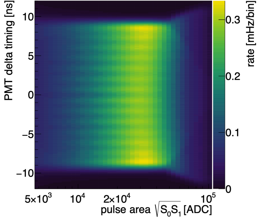
Figure 5.5: The “Hobbes effect” from corner clipping muons for z -position calibration. The map shows the PMT timing differential dt distribution. Source:[92]
