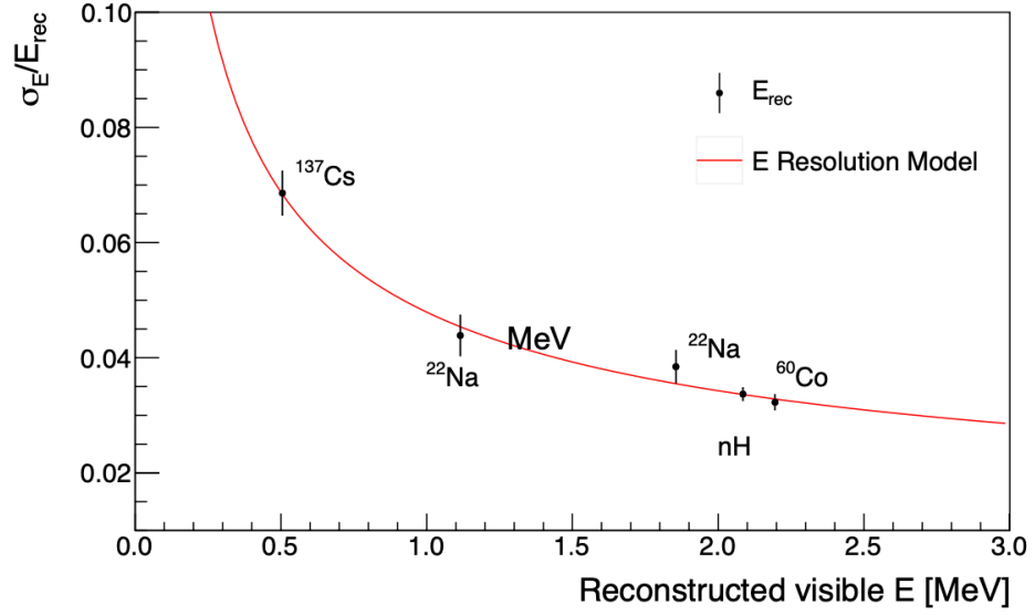
Figure 5.15: The best-fitted energy resolution from calibration sources. Source:[92]
