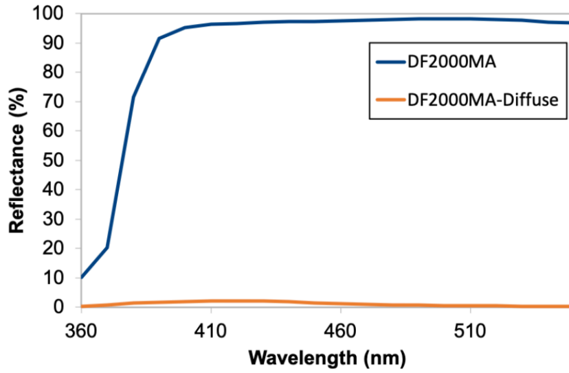
Figure 4.8: Total and diffuse reflectance of DF2000MA in the wavelength range above 360 nm. Source:[86]
