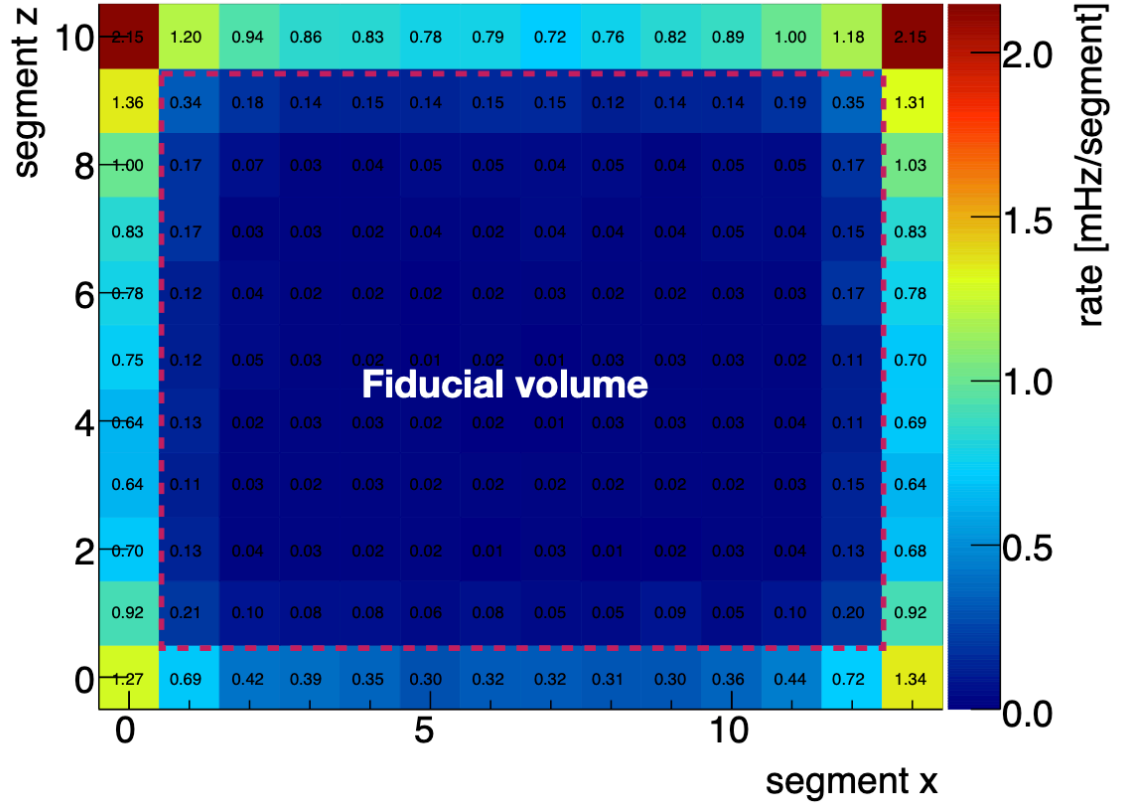
Figure 6.3: Illustration of the fiducial volume to reduce to cosmogenic backgrounds. Segments with higher cosmic ray related neutron rates are excluded in the IBD selection. A 140 mm fiducial layer is also defined along the length of the segment. Adapted from [76].
