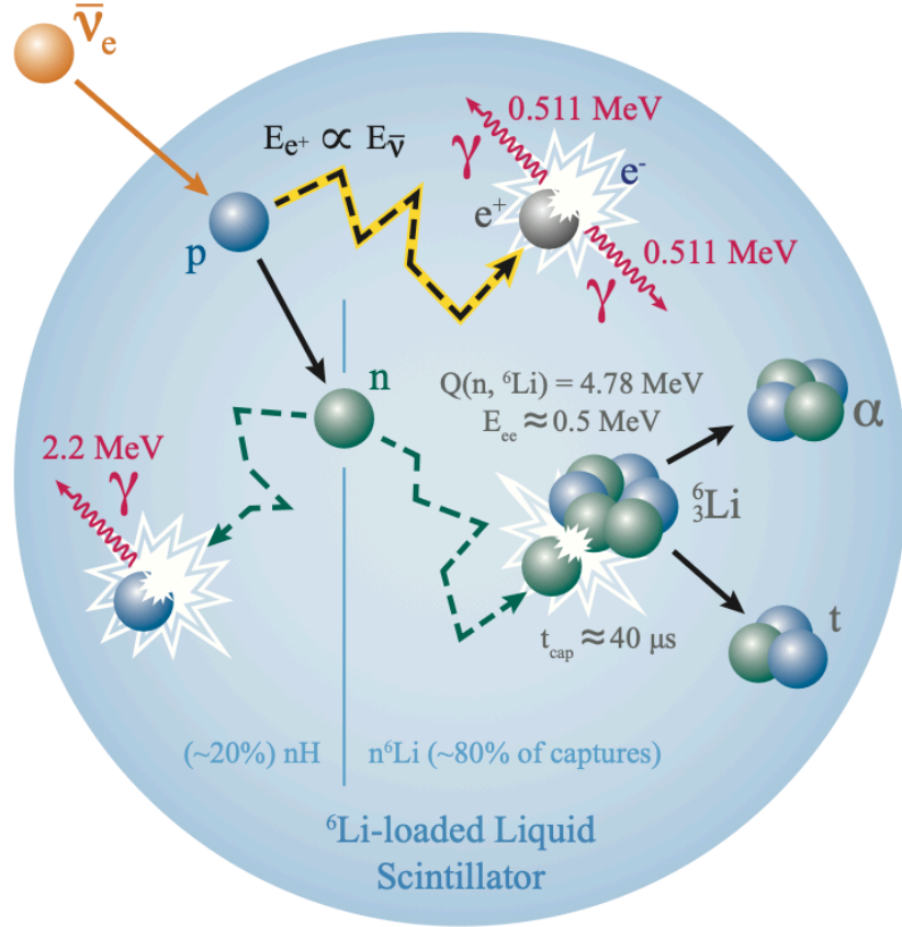
Figure 5.1: The schematics of the IBD process and particle interactions in the {}^6\text{LiLS} . An IBD interaction consists of an energetic prompt positron signal and a delayed neutron capture on {}^6\text{Li} within 50 \mu\text{s} , generating \sim 0.55 \text{ MeV} electron equivalent.
