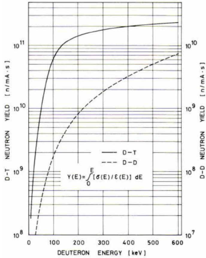
Figure 9.2: Comparison of the neutron yield as a function of deuteron energy for DD and DT reactions. Source:[129]
