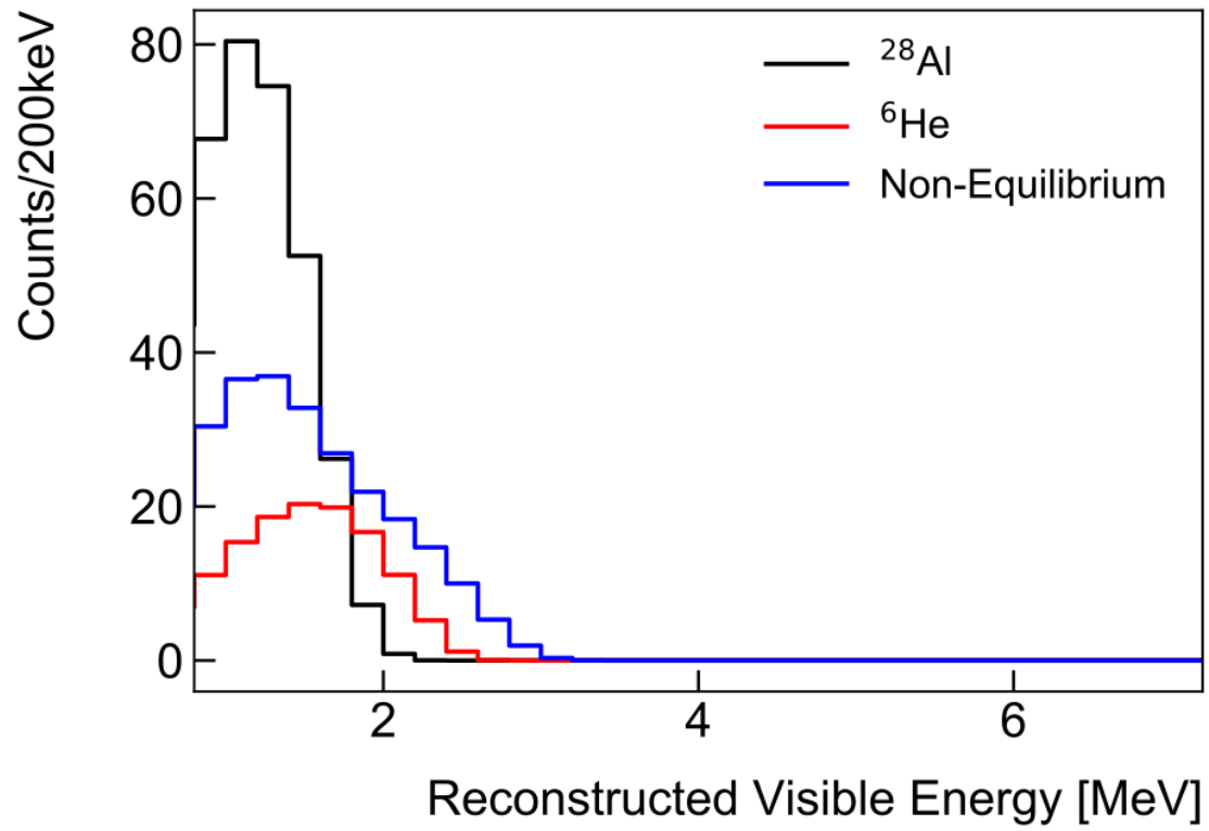
Figure 6.22: Non-fuel contributions to the ^{235}\text{U} neutrino spectrum. These neutrino sources contribute less than 1% of the total neutrino flux and limited to the low energy regions. Source:[92]
