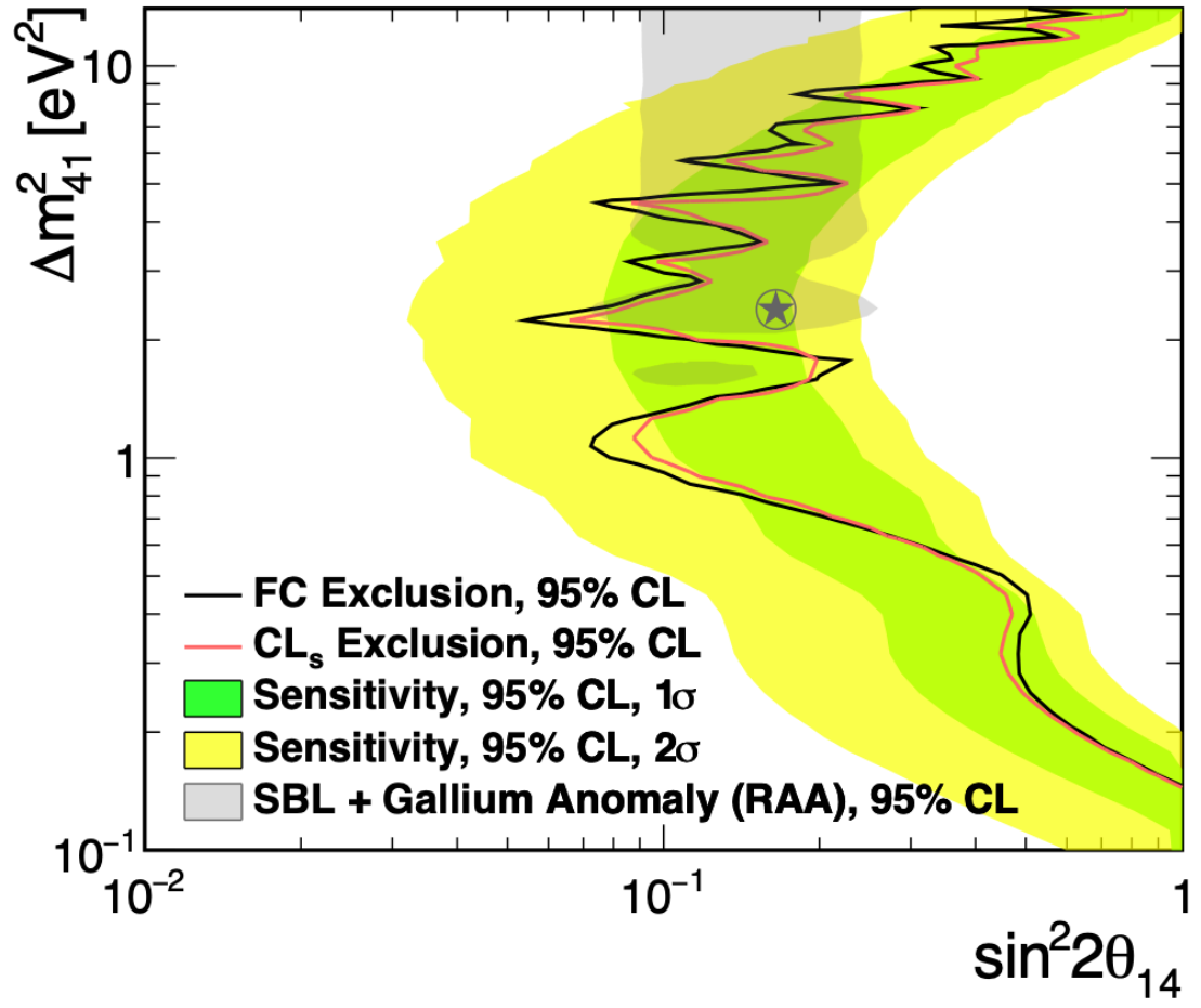
Figure 6.28: Exclusion curves generated via both Gaussian \text{CL}_s and Feldman-Cousins frequentist, as well as the best-fit RAA. The 1\sigma and 2\sigma (green and yellow) exclusion ranges are generated by PROSPECT toy simulations. Source:[92]
