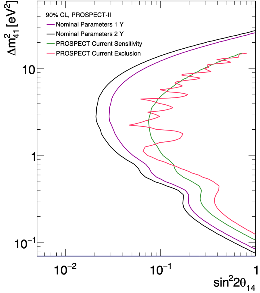
Figure 7.1: Projected sensitivities for PROSPECT-II with nominal detector parameters with one year and two years' detector data-taking time. Current PROSPECT sensitivity is also shown for comparison. Source:[117]
