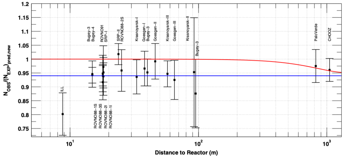
Figure 3.5: Ratio of measured \bar{\nu}_e flux to the new reevaluated model prediction. The global average in blue line indicated a \sim 6\% deficit, the so-called Reactor Antineutrino Anomaly (RAA). A possible explanation is the inclusion of a fourth sterile neutrino in the three neutrino paradigm, with mixing parameters |\Delta m_{41}^2| \gg 1 \text{ eV}^2 and \sin^2 2\theta_{14} = 0.12 . Source:[61]
