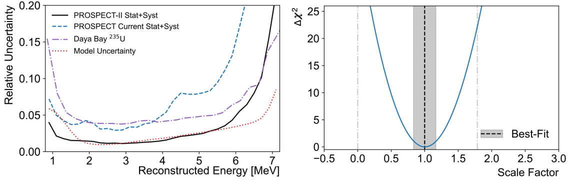
Figure 7.4: Left: Improvement to PROSPECT-II ^{235}\text{U} spectrum measurement uncertainties after two years of data-taking. Right: PROSPECT-II hypotheses testing for bump-like feature in the 4-6 MeV prompt energy region observed by Daya Bay at high confidence level. n=0 represents no contribution from ^{235}\text{U} and n=1.78 represents entire contribution from ^{235}\text{U} . Source:[117]
