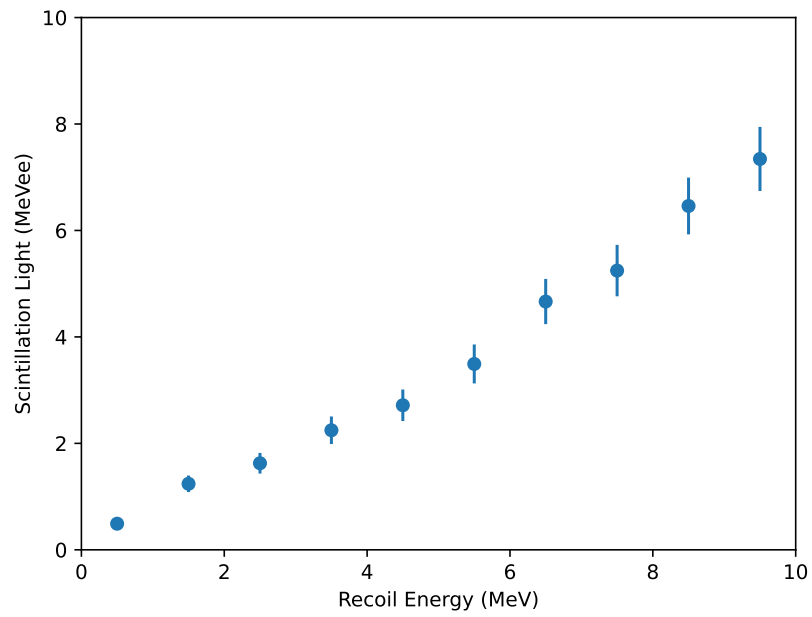
Figure 9.5: Scintillation light as a function of recoil energy. The recoil energy is calculated in Equation 9.7.
