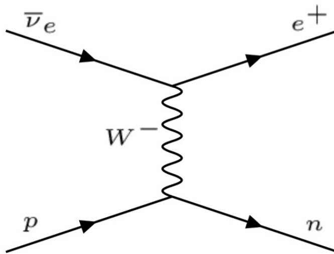
Figure 3.3: Feynman diagram of the Inverse Beta Decay process
