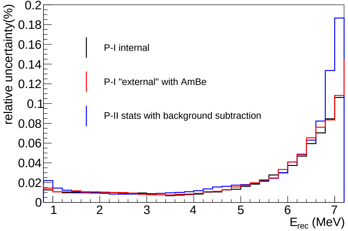
Figure 8.8: Relative systematic uncertainty from the energy scale model is plotted in the energy range where most IBD events fall. P-I internal in black represents the uncertainty from the P-I internal calibration without the AmBe source. P-I “external” in red represents the uncertainty from the P-II type external calibration study with the AmBe source. P-II signal statistics with background subtraction in blue includes the estimated statistical uncertainty from the expected IBD statistics in the P-II detector and estimated background statistics.
