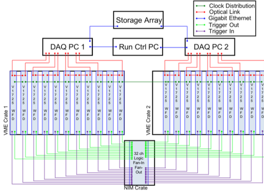
Figure 4.17: Schematics of the PROSPECT DAQ system. Source:[76]
