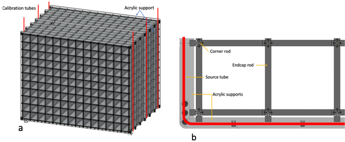
Figure 7.7: Left: Illustration of the external calibration source tubes along the perimeter of the segment array. Right: Side view of the reflector panels supported by corner rods and endcap rods. The outermost reflector are spaced by acrylic spacers from the inner containment wall, allowing for calibration source tubes. Source:[117]
