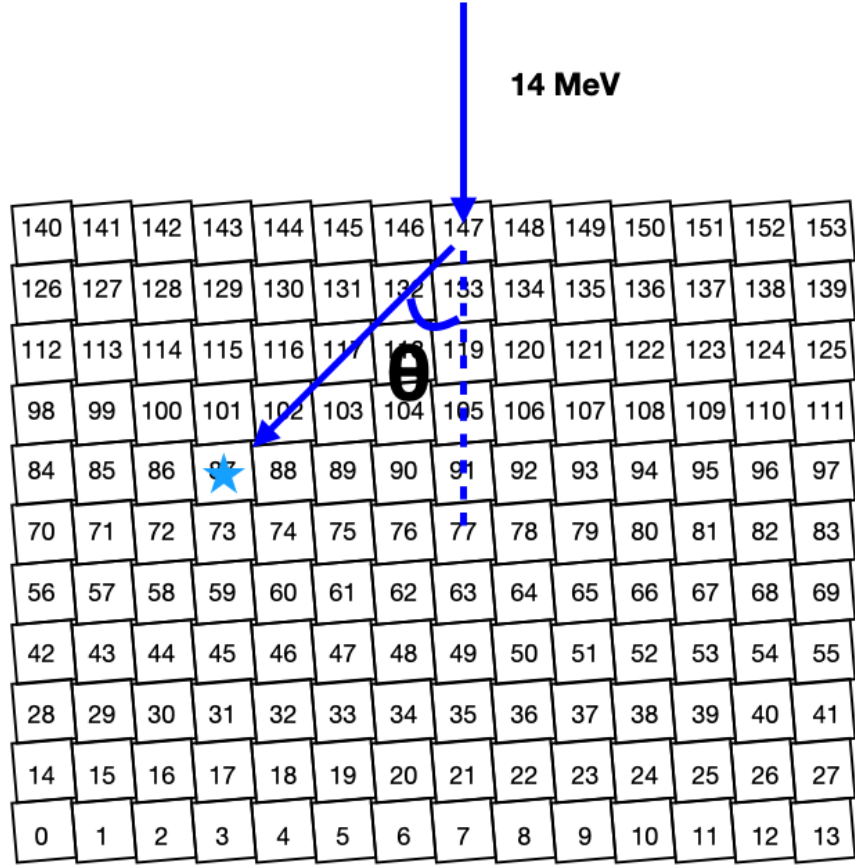
Figure 9.4: Schematic of neutron scattering in the highly segmented PROSPECT detector. Mono-energetic neutrons from the DT generator are incident from the top of the detector. The neutron scatters off the entry segment 147 and subsequently on segment 87, with a scattering angle \theta . The star represents the STOP segment used for determination of the scattering angle.
