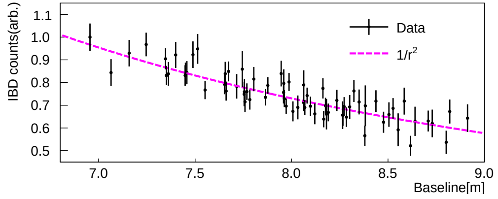
Figure 6.18: Clear baseline-dependence of physics-correlated IBD candidates within [0.8, 7.2] MeV is fitted with 1/r^2 trend. IBD counts are normalized by IBD counts in the shortest baseline bin. Efficiency variations at various baselines are accounted for. \chi^2/\text{DOF} \sim 72.43/69 .
