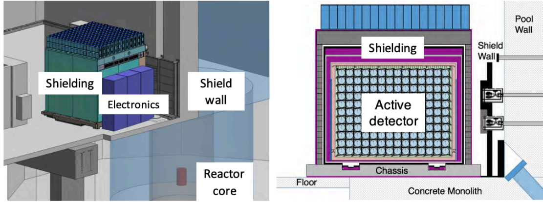
Figure 4.2: Left: schematic of the AD in the experimental hall relative to the reactor core, with an average baseline of 7 m. Right: schematic sideview of the AD shielding against reactor related background. Source:[76]
