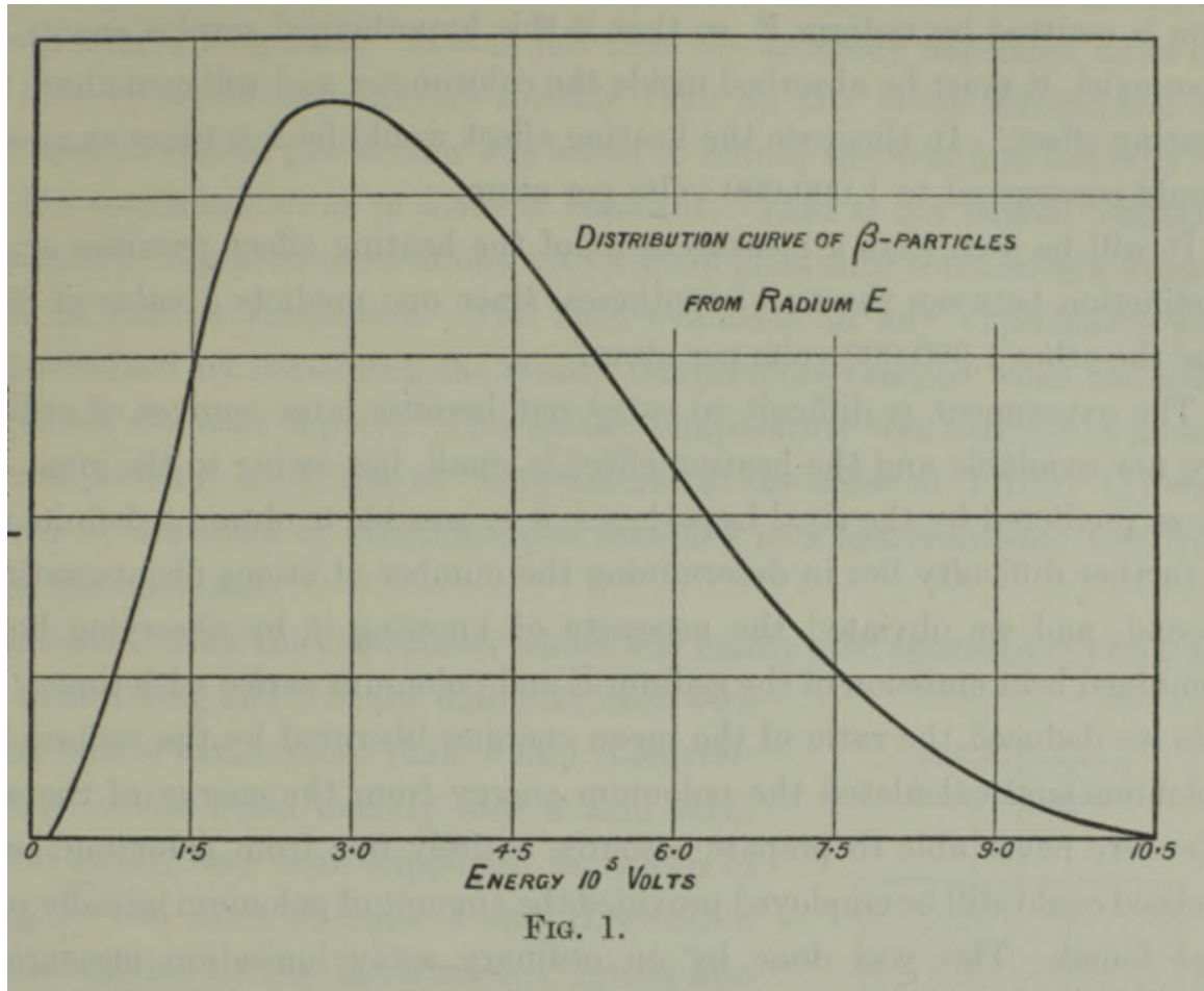
Figure 2.1: \beta spectral measurement of the Radium-E( ^{210}\text{Bi} ) by Ellis and Wooster in 1927. Source: [3]
