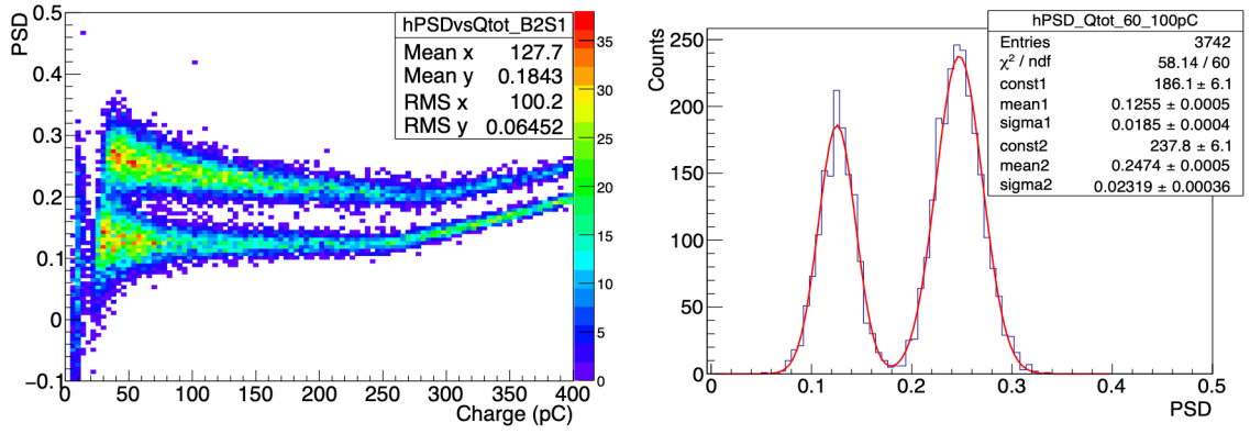
Figure 4.4: PSD distributions of the PROSPECT ^6\text{LiLS} . Right: PSD distribution fit to Figure of Merit (FOM) at 540 keV visible energy. Source:[82]
