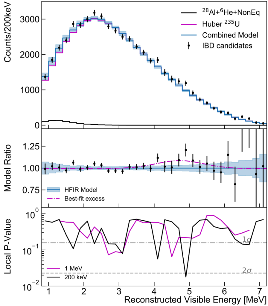
Figure 6.23: Comparison of the ^{235}\text{U} predicted spectrum to the measured PROSPECT data. Middle panel shows the ratio of the measured spectrum to the predicted; Bottom panel shows local deviations of the measured spectrum from the predicted in terms of p-value for two types of sliding window analysis with 200 keV and 1 MeV width. Source:[92]
