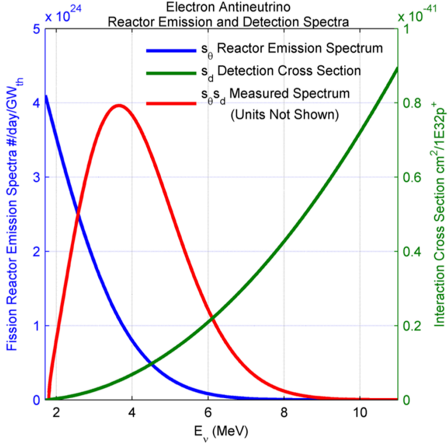
Figure 3.4: Illustration of a typical reactor neutrino spectrum using detector techniques based on the IBD interaction. Note the neutrino energy starts from the IBD threshold described in Equation 3.4. Source:[37]
