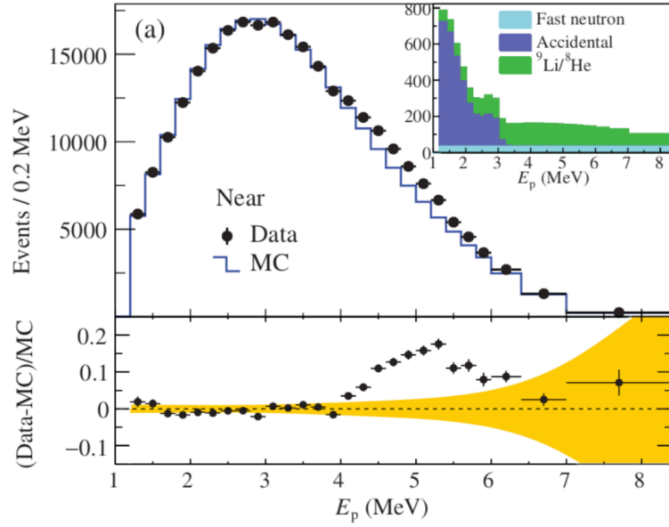
Figure 3.8: Visible energy spectrum reported by RENO experiment. The ratio of measurement to the Huber-Mueller model prediction is shown. Source:[60]
