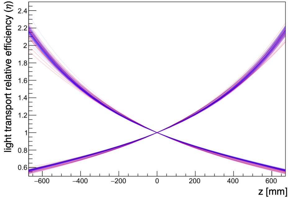
Figure 5.10: An example of z -dependence of light collection efficiency from all Hamamatsu (blue) and ET PMTs (red). Source:[100]
