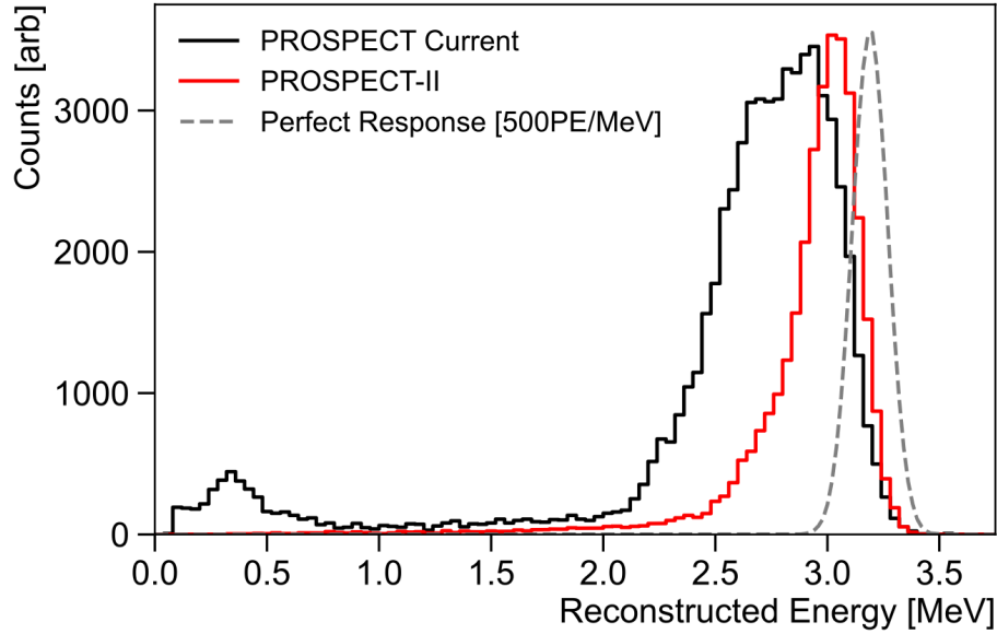
Figure 7.5: Comparison of simulated detector response to monoenergetic 4 MeV \bar{\nu}_e for the PROSPECT-II detector (red) and the current PROSPECT detector (black). Source:[117]
