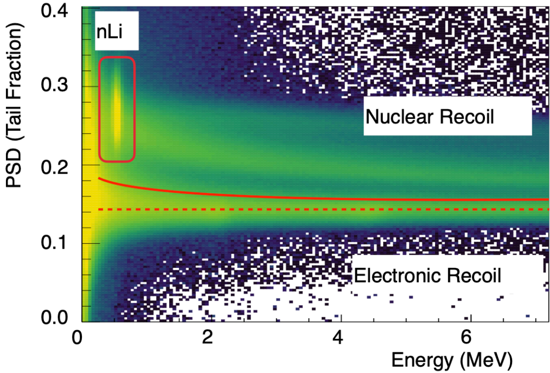
Figure 6.2: Illustration of the various particle types in PSD vs E space, allowing identification for prompt and delayed IBD products. Neutron captures on {}^6\text{Li} are concentrated in the red box. The additional high PSD band is likely caused by recoils of heavier charged particles other than protons. Adapted from [76].
