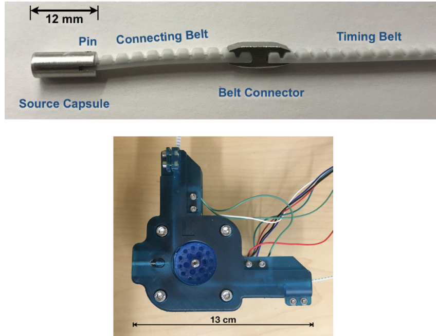
Figure 4.13: Pictures of drive belt (top) and stepper motor(bottom). Source:[88]
