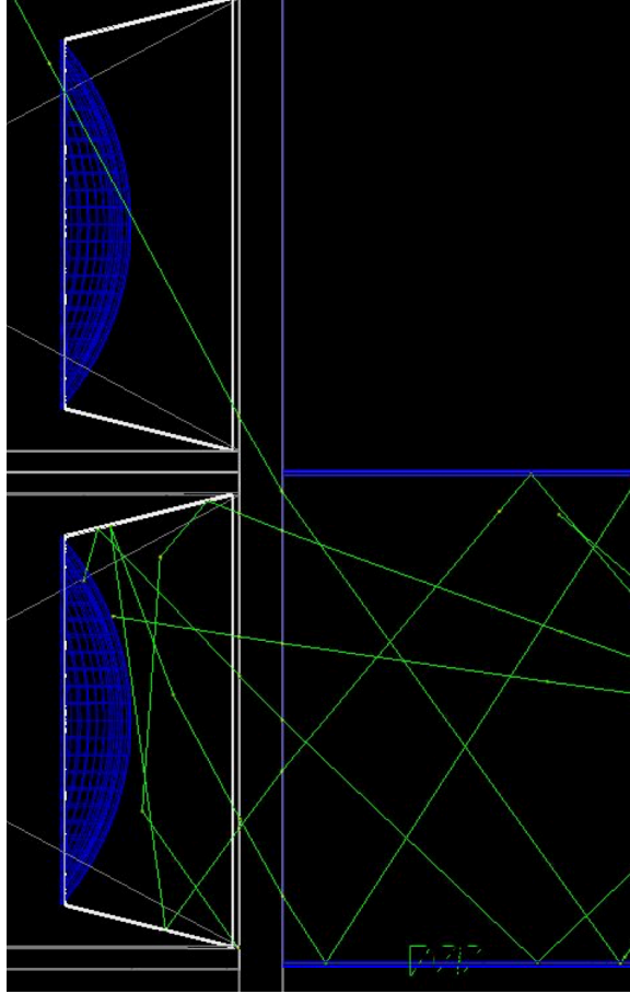
Figure 8.12: MC simulations of neighbor cross-talk introduced by the acrylic window. The \gamma -ray tracks are illustrated in green, two neighbor PMT surfaces are located on the left. The acrylic window was the middle piece with 1/4 inches thickness. Source:[117]
