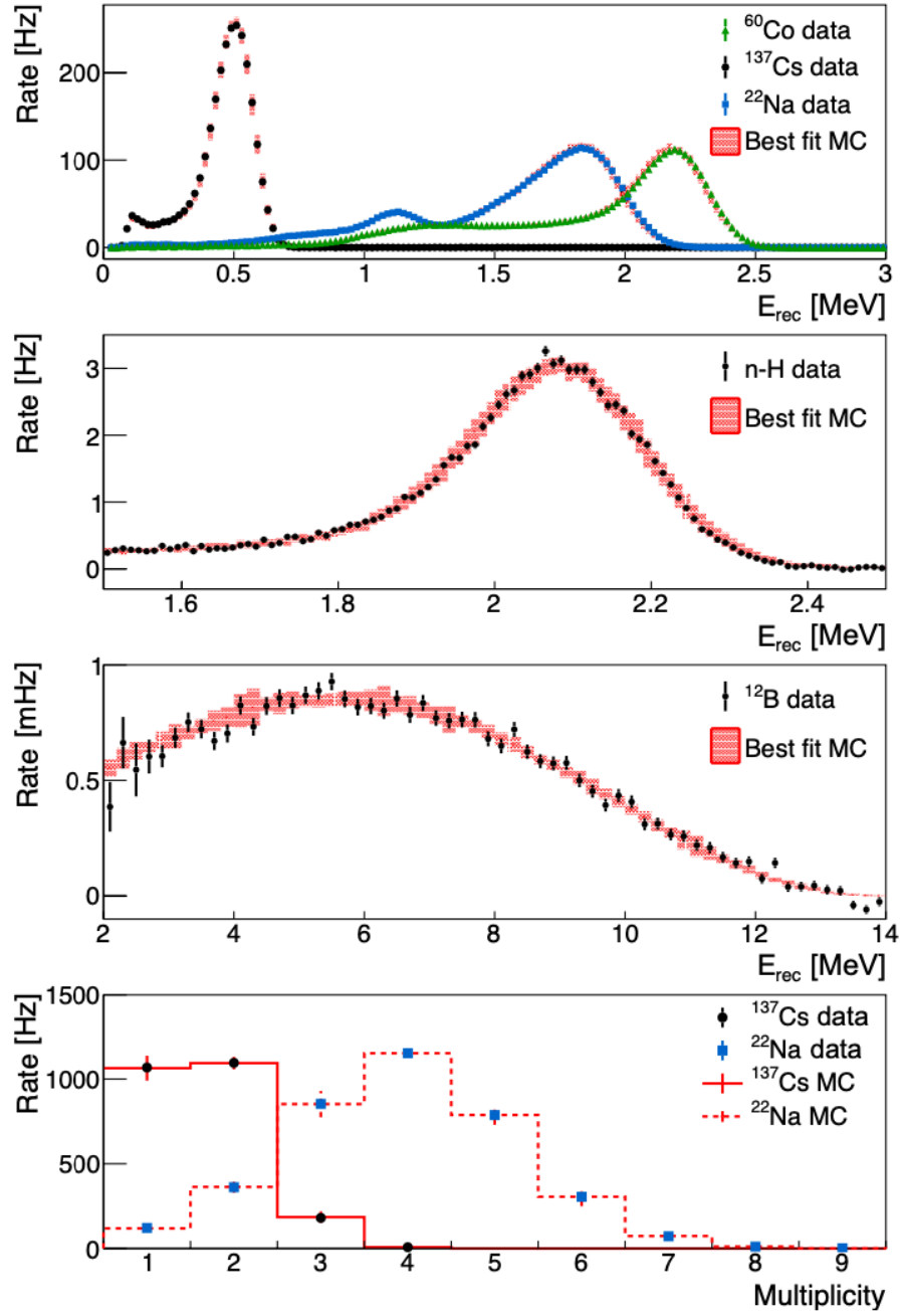
Figure 5.12: Best-fit energy scale model comparisons with calibration data. Source:[92]
