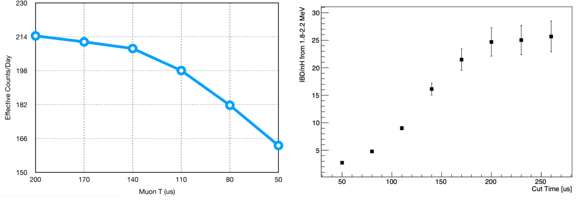
Figure 6.10: Muon veto cut optimization. The right plot shows signal to background ration in the nH region.
