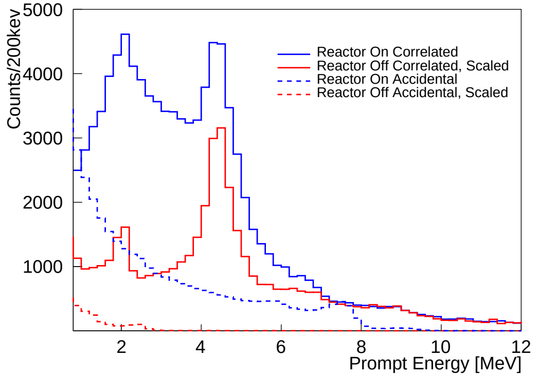
Figure 6.14: The measured reconstructed prompt energy spectrum of reactor-off/on correlated and accidental candidates up to 12 MeV to show three main contributions from n-H capture, nC inelastic scattering and a variety of neutron processes. Scaled accidental events are plotted in corresponding colors for reactor on and off.
