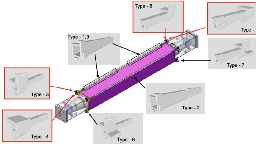
Figure 4.9: Various types of support PLA rods and their assembly location along the segments. Center rods, such as 1,2,9, are used to seal the segments. The end rods, such as 3-8 are used support thick and rigid spacing between PMT housings and center rods [86].
