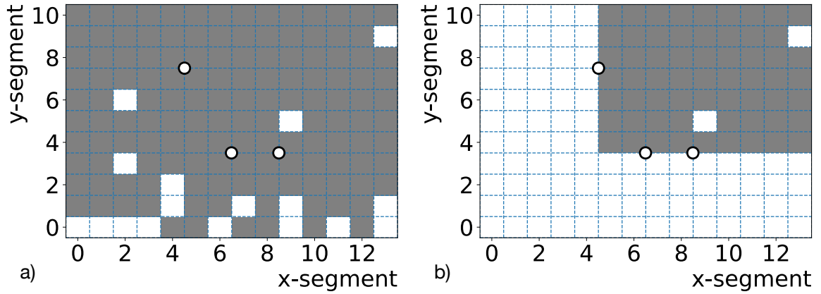
Figure 8.2: Illustration of the actual PROSPECT-II external calibration performance evaluation using PROSPECT-I data and simulation. This differs from the idealized case of Figure 8.1 due to a number of PMT failures at the time of calibration campaign. The white circles indicate available source locations and only one source was deployed at a time. a) Actual PROSPECT-I radioactive source and segment layout. b) Configuration used in this work to mimic external calibration.
