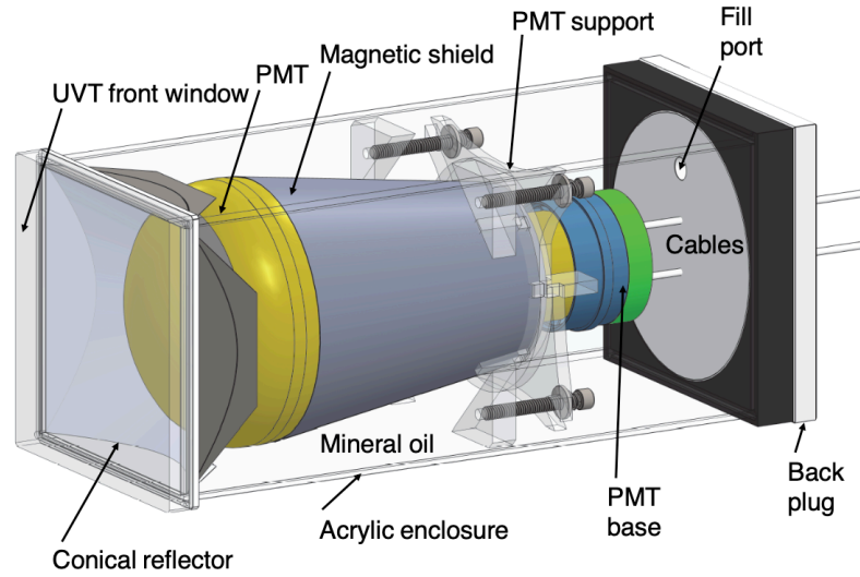
Figure 4.11: Schematic of the PMT module. Source:[76]
