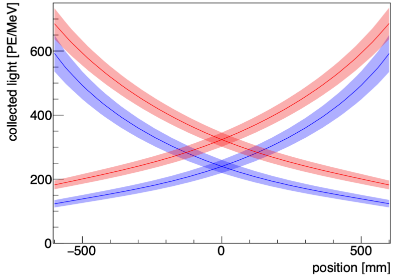
Figure 5.3: Position dependence of light collection in the PROSPECT AD segment. The blue and red band indicates the RMS spread between segments and the performance of the liquid scintillator at the beginning (red) and end (blue). Source: [92]
