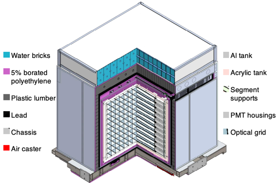
Figure 4.3: A cutaway view of the detector and shielding assembly. Top water bricks shields the cosmic ray related backgrounds. Lead and borated polyethylene in purple shields the inner acrylic vessel from the reactor related backgrounds. The active detector volume is optically segmented by reflective grids into 14 \times 11 uniform segments. Source:[76]
