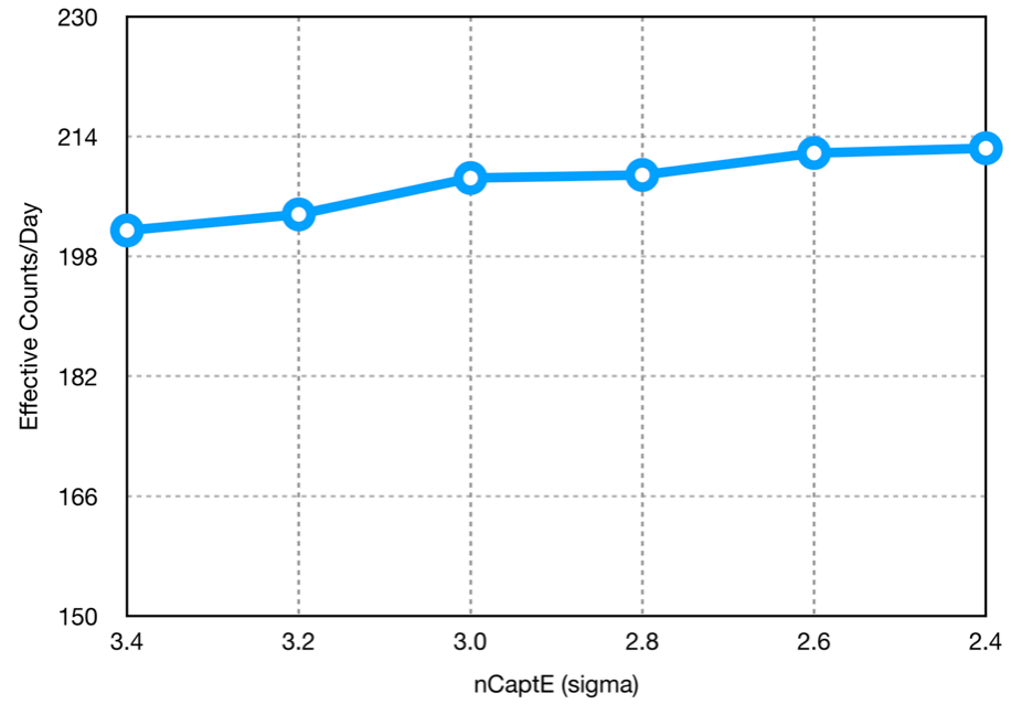
Figure 6.5: Neutron capture E cut optimization.
