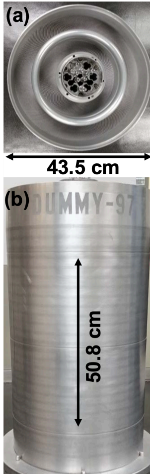
Figure 4.1: Photographs of a dummy HFIR reactor core showing (a) the diameter and (b) the height. Source:[76]
