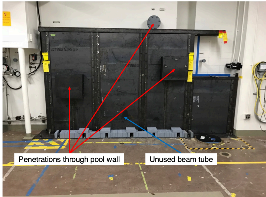
Figure 4.15: Photograph of the lead wall between the detector and reactor pool. Source:[76]
