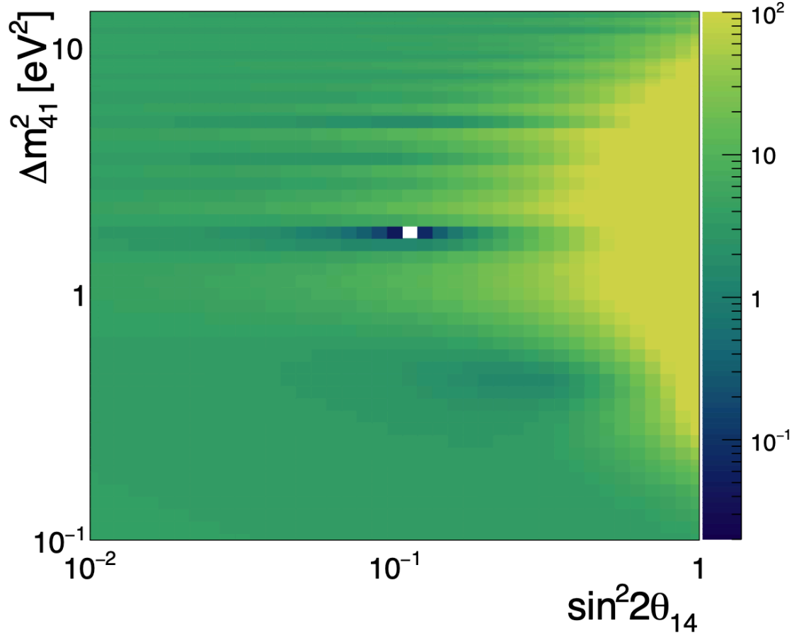
Figure 6.27: The distribution of \Delta\chi^2 in phase space (\sin^2 2\theta_{14}, \Delta m_{41}^2) with respect to the best fit point (white square) (0.11, 1.78 \text{ eV}^2) . Source:[92]
