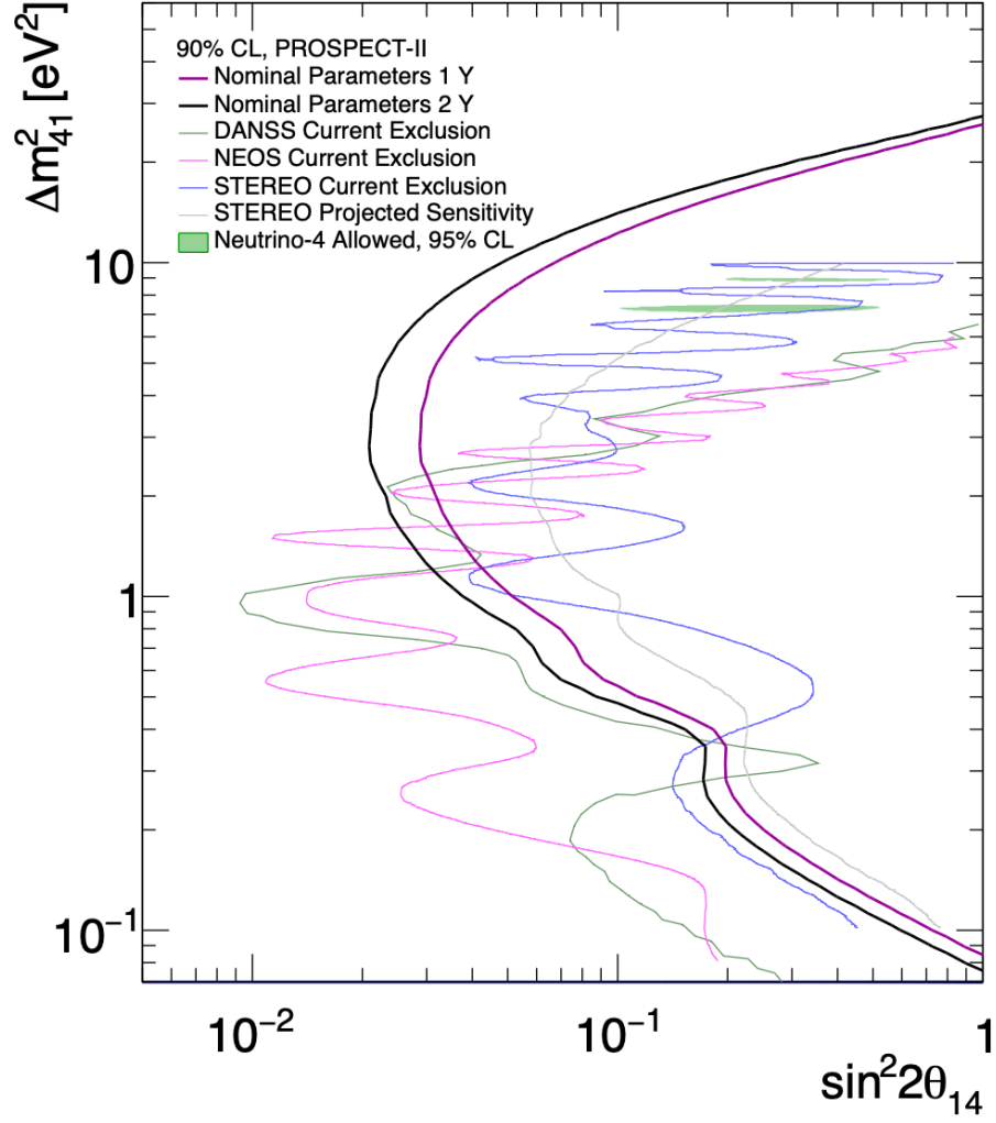
Figure 7.2: Projected sensitivities for PROSPECT-II with nominal detector parameters with one year and two years' detector data-taking time. Other short-baseline neutrino experiment contours are overlapped in comparison [70, 68, 118, 109]. Source:[117]
