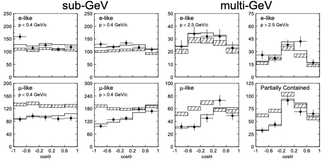
Figure 2.3: Super-Kamiokande event distribution (black dots) for sub-GeV and multi-GeV category as a function of \cos \theta . \cos \theta = -1 represents upward-going events and \cos \theta = 1 represents downward-going events. Electron-like events in the top panel showed agreement with the MC expectation (shaded areas). However, muon-like events deviated from the non-oscillated MC simulations (shaded regions) and can be best-fitted for \nu_\mu \leftrightarrow \nu_\tau as highlighted in solid lines. Source:[9]
