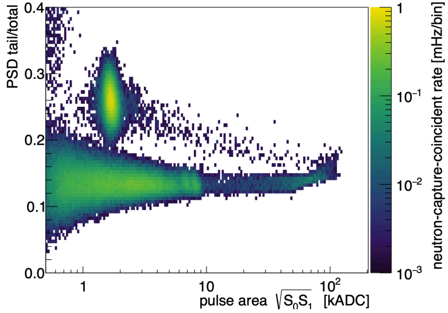
Figure 5.8: Calibrated pulse PSD for {}^6\text{Li} -captured spallation neutrons vs signal amplitude in time coincidence with cosmic muon signals. Neutron captures on {}^6\text{Li} are clearly visible and localized above the gamma band. Source:[92]
