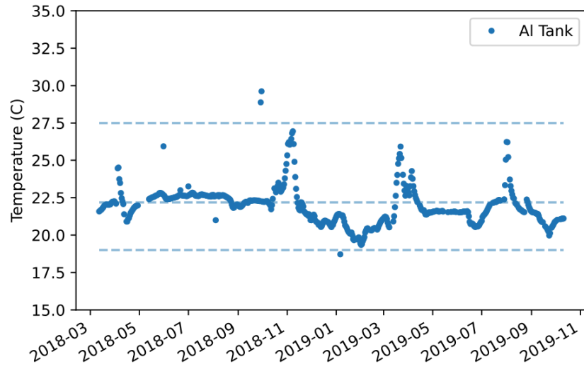
Figure 4.16: Environment temperature fluctuations. The spikes are caused by temporary shut down of AC at the experimental hall at HFIR. Source:[91]
