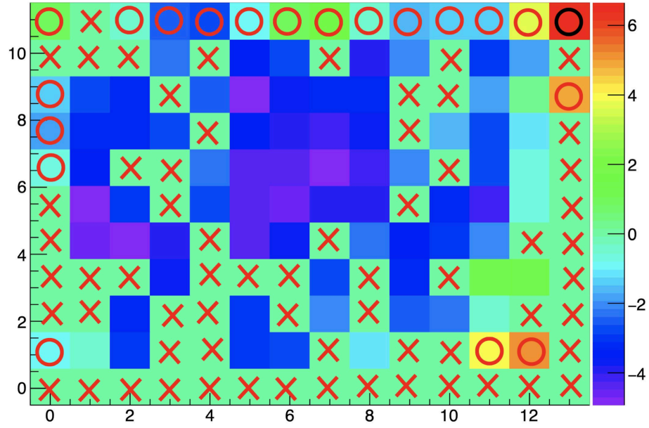
Figure 6.13: The segment lists of the fiducial volume. The segments marked by cross are turned off due to PMT failures. The segments marked by circle are excluded by the optimization process. The color bar represents the change of effective counts if the segment was fiducialized.
