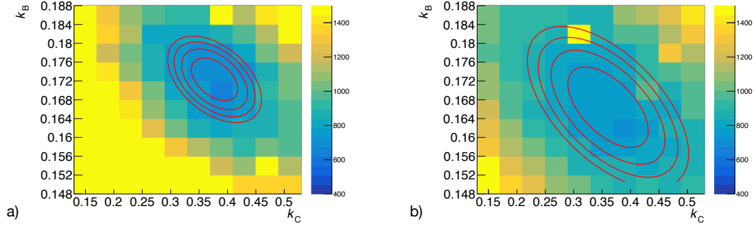
Figure 8.5: \chi^2 distribution in energy scale parameter space for a) internal calibration and b) external calibration. Each \chi^2(k_B, k_C) on the grid represents the corresponding detector response deviation from the calibration data with the optimized A value. The contours are generated with \Delta\chi^2 = 30 increments for illustration purposes. Note the intervals in the contours are larger for the external calibration. Thus, the best-fit is less well-constrained compared to the internal case, but is still well-defined.
