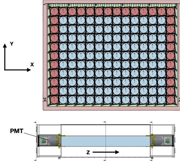
Figure 4.10: Schematics of the PROSPECT AD and PMTs. The red represents the installation of 68 ET PMTs and the blue for the 240 Hamamatsu PMTs. Source:[76]
