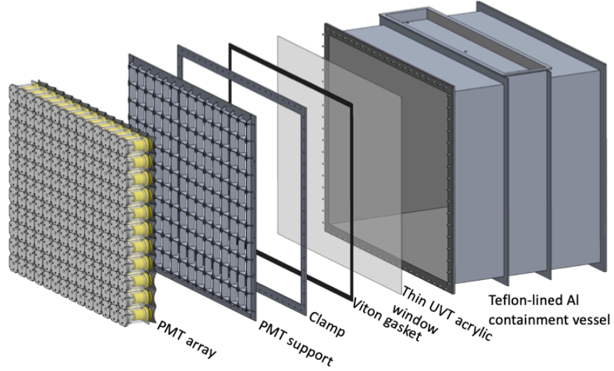
Figure 7.6: Exploded-view of the redesigned inner detector. The PMTs arrays and LiLS volume is separated by the thin acrylic window. The whole inner detector will be submerged in mineral oils filled within the outer containment vessel. Source:[117]
