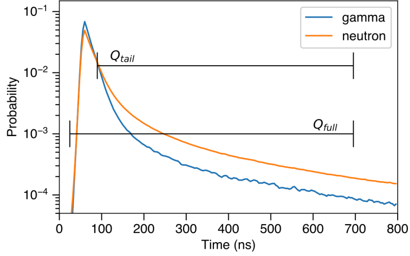
Figure 5.2: Example pulse shapes for electronic recoils and nuclear recoils. The total and tail fraction of the pulse integral are also illustrated.
