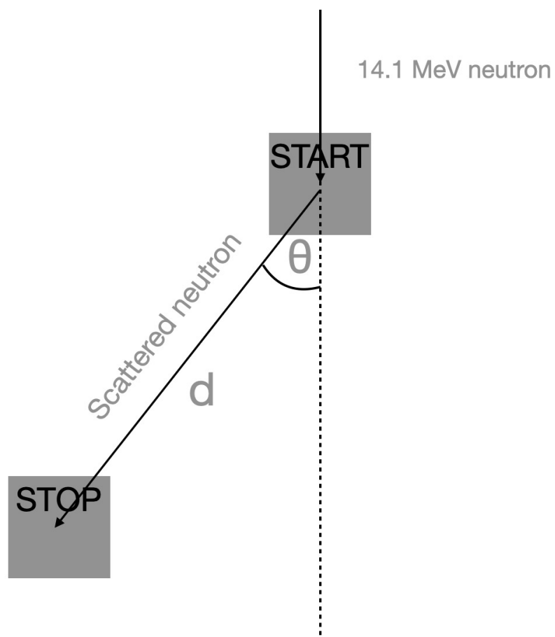
Figure 9.3: Schematics of the experimental setup of liquid scintillator neutron response. The START is the liquid scintillator and the STOP is the neutron detector placed at d distance that provides both timing and angle information.
