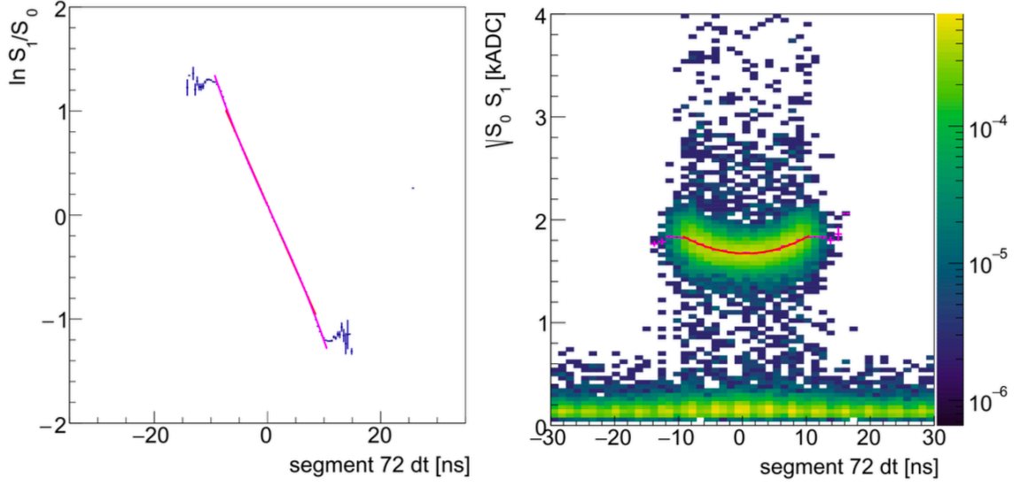
Figure 5.9: Examples of R(dt) and S(dt) . Left: \ln R(dt) was fitted to dt in a cubic polynomial fit (magenta), better than a linear fit (red). The data is in blue. Right: S(dt) distribution from neutron captures on {}^6\text{Li} with a quadratic polynomial fit in magenta. Source:[100]
