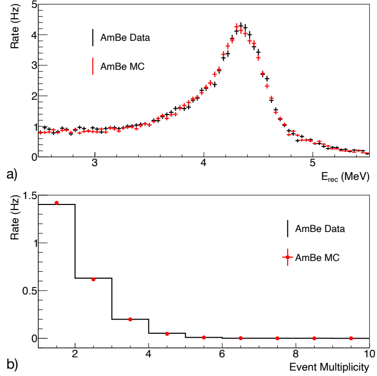
Figure 8.7: AmBe 4.4 MeV \gamma -ray energy spectrum in a) and event multiplicity distribution in b) using the external energy scale model obtained with AmBe calibration.
