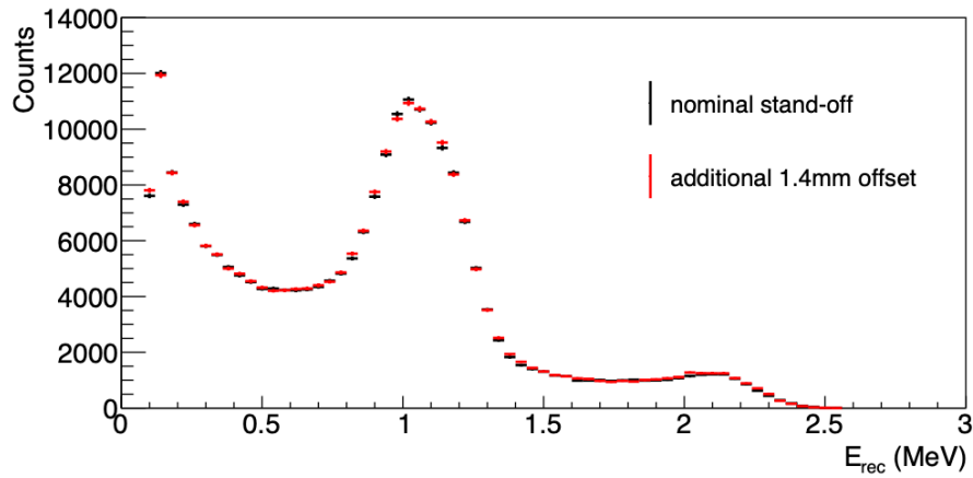
Figure 8.10: MC ^{60}\text{Co} spectrum externally deployed with a stand-off distance of 1.4 mm further away from the nominal position, with a \chi^2/\text{ndf}=250.6/245 .
