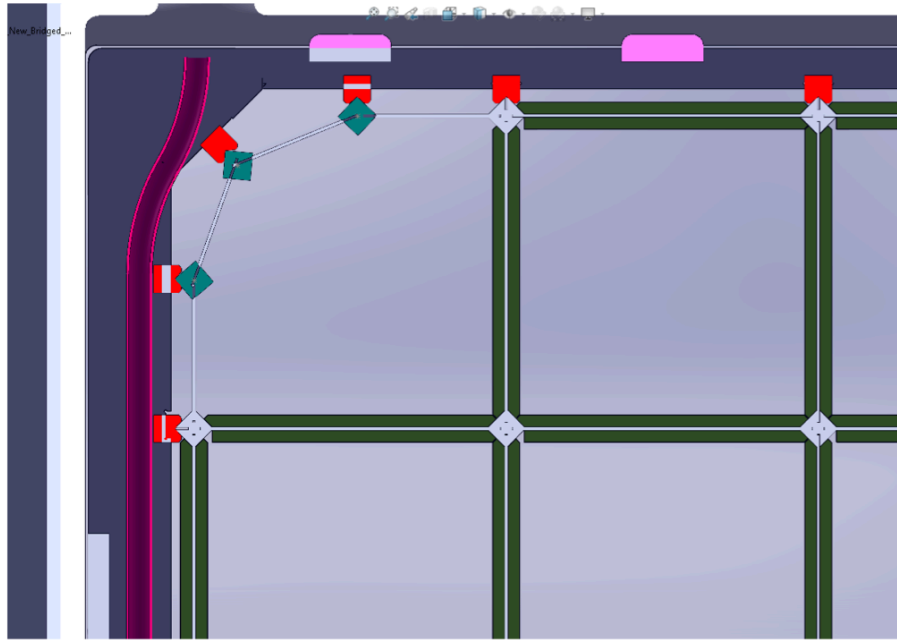
Figure 8.9: The schematic shows the stand-off distance introduced in the upgraded PROSPECT-II detector. The 3/8 inches calibration source tube can be inserted from the top of the detector, shown in red. The green are supporting rods that house the reflective panels. The center of the source tube to the boundary of the active liquid scintillator volume is estimated to be \sim 3 cm.
