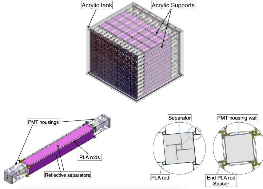
Figure 4.6: Schematics of the PROSPECT optical grid. The top panel shows the optical grid system inside the inner acrylic tank. The left panel shows the individual optical segment, enclosed by double PMTs on the ends. The right panel shows the interlock mechanism between the specular reflective separators and PLA rods. The hollow PLA rods allow for the calibration tube access. Source:[86]
