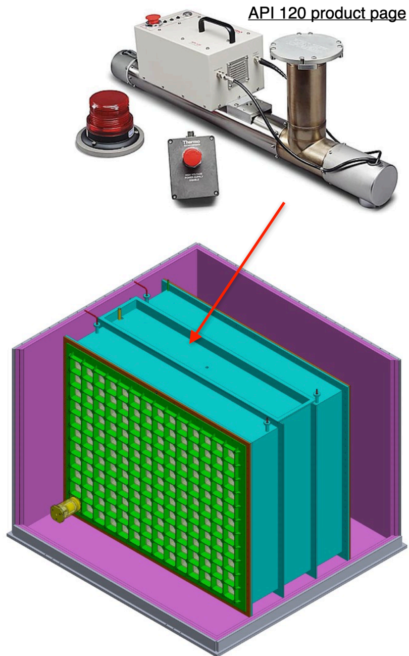
Figure 9.1: Illustrations of the DT neutron generator installed on top the PROSPECT-II detector. Portable API 120 commercial neutron generator [128] is displayed as an example.
