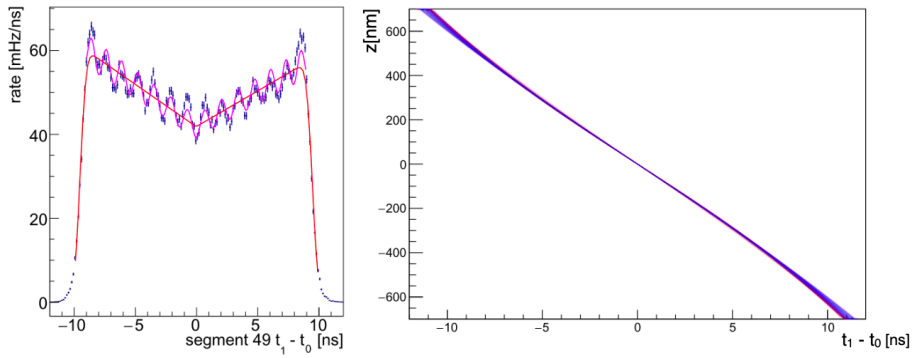
Figure 5.6: Left: fitted results of the dt data for segment 49. Right: z(dt) data from 154 segments, blue (red) for Hamamatsu (ET) PMTs. Source:[100]
