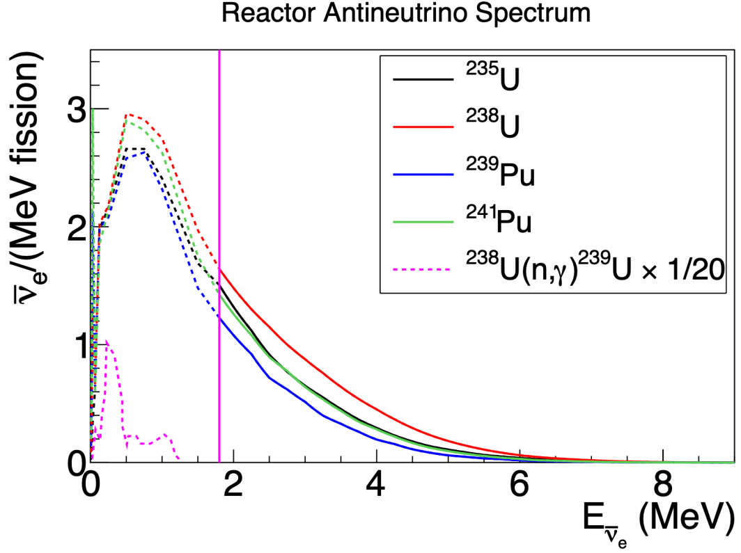
Figure 3.1: Neutrino energy distributions from the main four fissile isotopes, ^{235}\text{U} , ^{238}\text{U} , ^{239}\text{Pu} , ^{241}\text{Pu} . The vertical pink line represents the energy threshold of IBD detection. The antineutrino spectrum from fissions induced by fast neutron captures on ^{238}\text{U} are below the IBD energy threshold and scaled by a factor of 20, which is not interesting from a IBD detection perspective. Source:[28]
