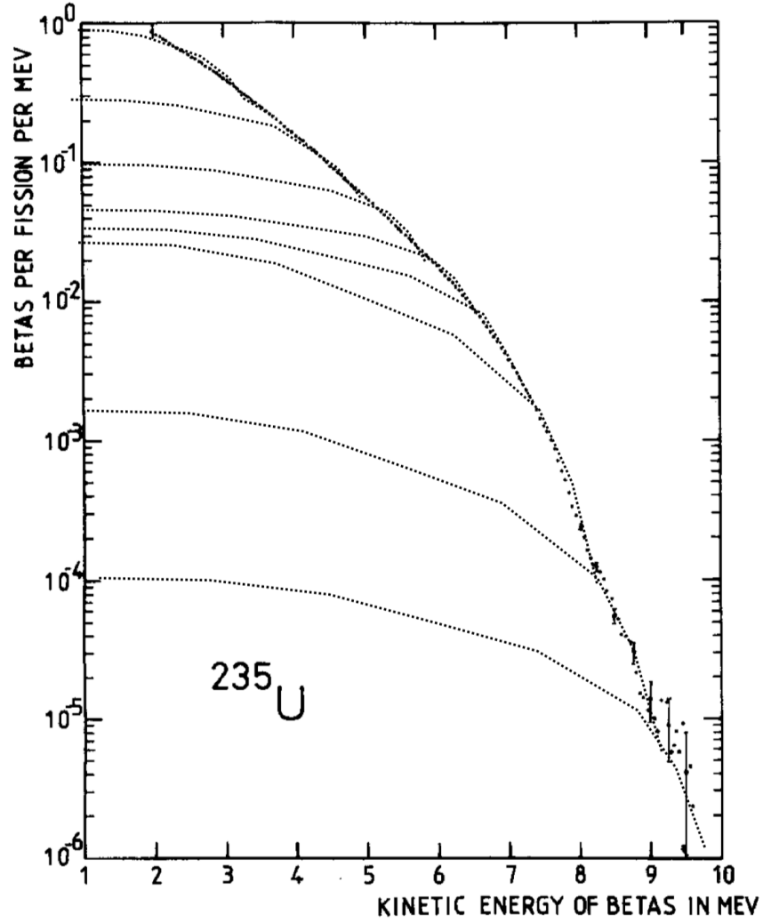
Figure 3.2: Illustration of virtual beta decay branch fitting for ^{235}\text{U} beta spectrum, reported from [30]. The dotted lines are the fitted virtual beta branches for the final conversion of the neutrino spectrum.
