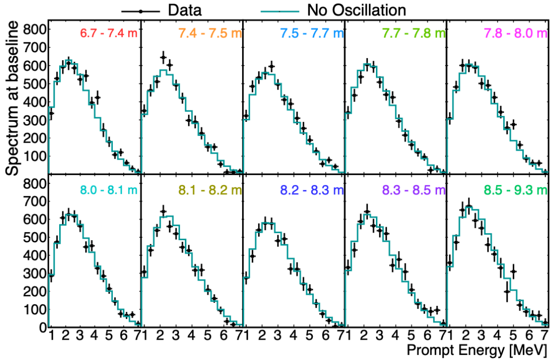
Figure 6.26: IBD spectral at different baselines. No oscillation predictions are in solid line. The predicted spectra are normalized to match the baseline-summed IBD signal. Source:[92]
