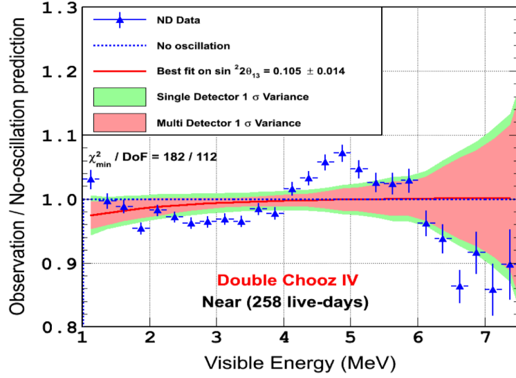
Figure 3.7: Visible energy spectrum reported by Double Chooz experiment. The ratio of measurement to the Huber-Mueller model prediction is shown. Source:[59]
