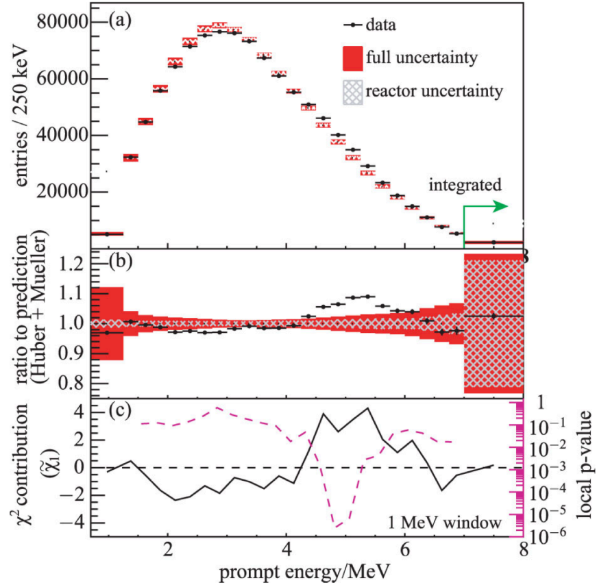
Figure 3.6: Visible spectrum reported by Daya Bay experiment. The ratio of measurement to the Huber-Mueller model prediction is shown in the middle panel. Source:[58]
