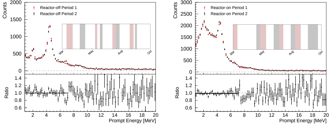
Figure 6.16: The reconstructed visible prompt energy E_{rec} spectral are compared at two periods for reactor-on (right) and reactor-off (left) respectively. Top panel : Reconstructed visible prompt energy from two periods. Bottom panel : The ratio of spectra.
