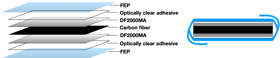
Figure 4.7: Left: The sandwich structure of a separator; Right: heat sealed folded FEP films. Source:[86]
