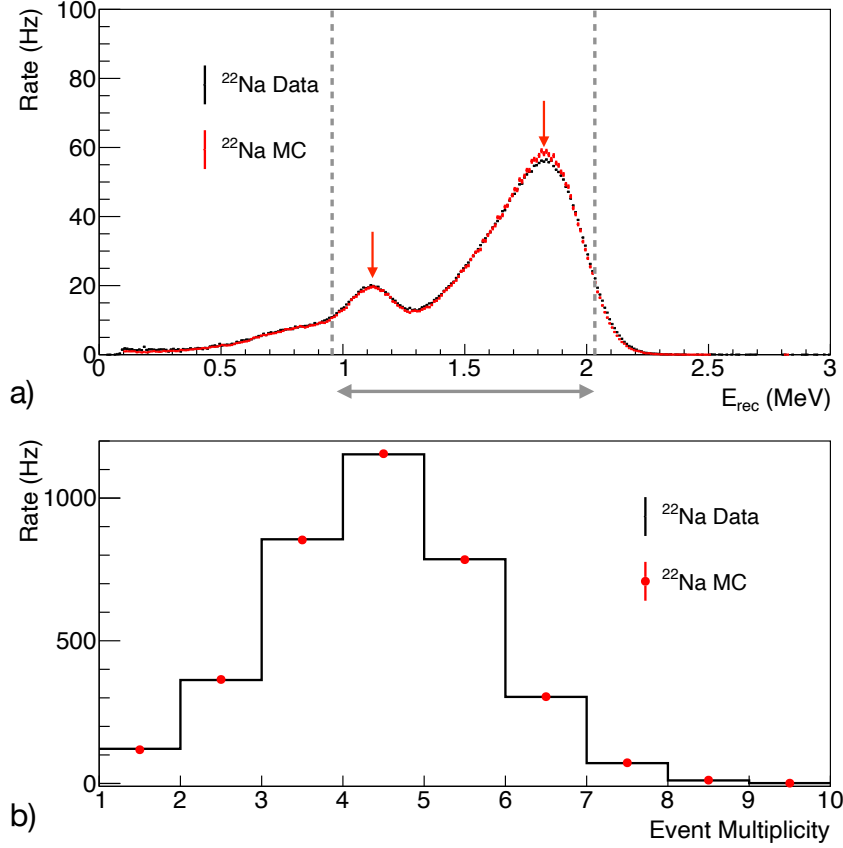
Figure 8.4: Here we show ^{22}\text{Na} data and MC comparison for an internal energy scale model, corresponding to the best-fit set of nonlinearity model parameters. The reconstructed energy E_{\text{rec}} represents scintillator quenched visible energy, which is typically shifted to lower energy compared to the true gamma energies. The gray lines in a) indicate the energy range for \chi^2 calculation. They are determined by the peak location and energy resolution as described above. The range for event multiplicity is between 1 and 9, as shown in b).
