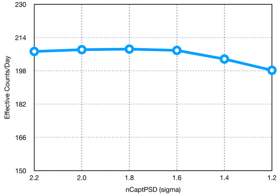
Figure 6.6: Neutron capture PSD cut optimization.
