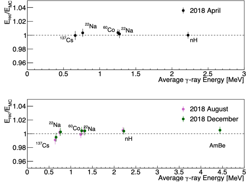
Figure 5.13: Ratio of \gamma -ray calibration between data and best-fit simulation. Top: calibration sources used in energy scale model determination; Bottom: ratio of calibration source in from all campaigns. Source:[92]
