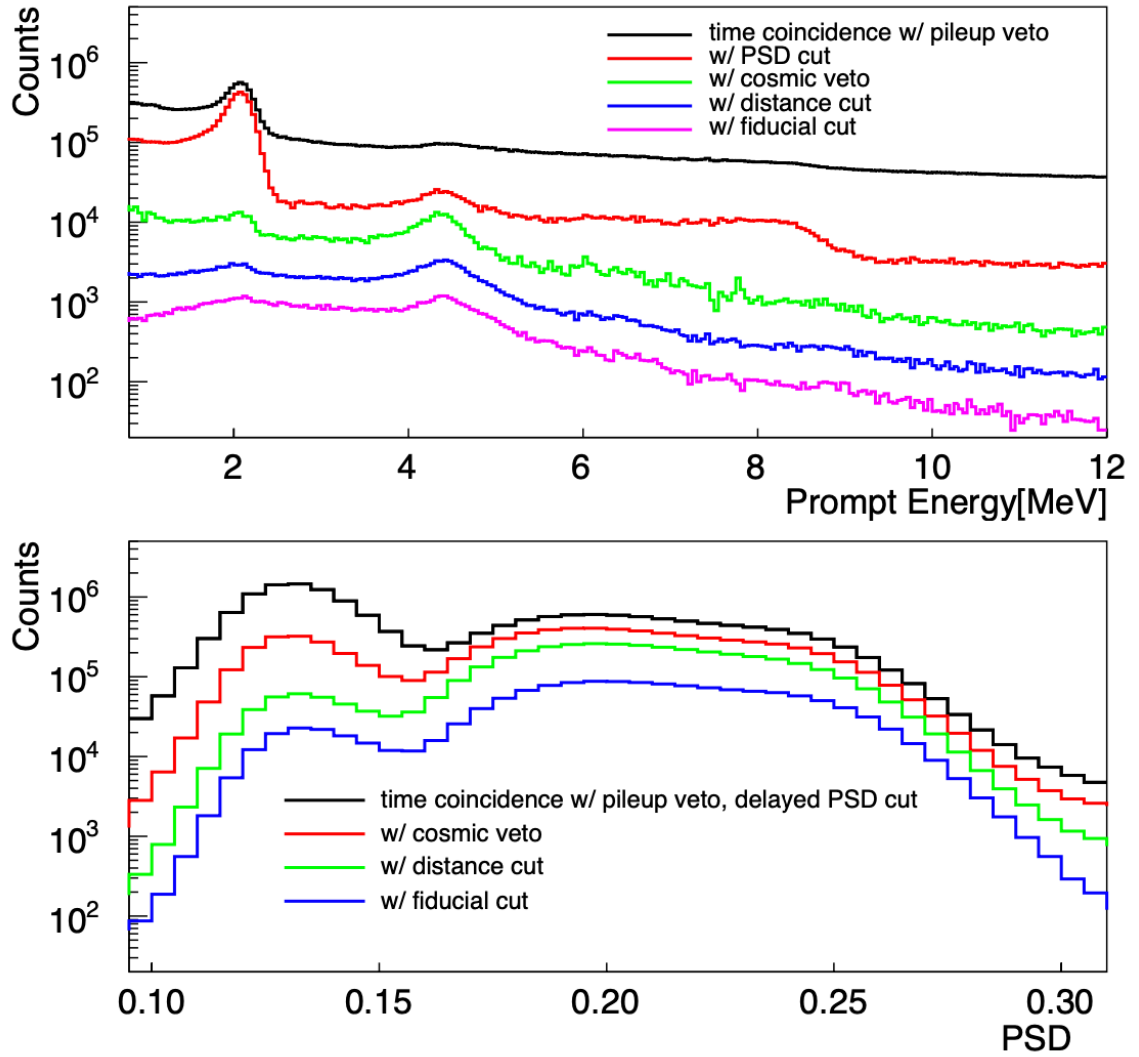
Figure 6.1: Illustrations of sequential application of IBD selection cuts in the reconstructed energy and PSD space.
