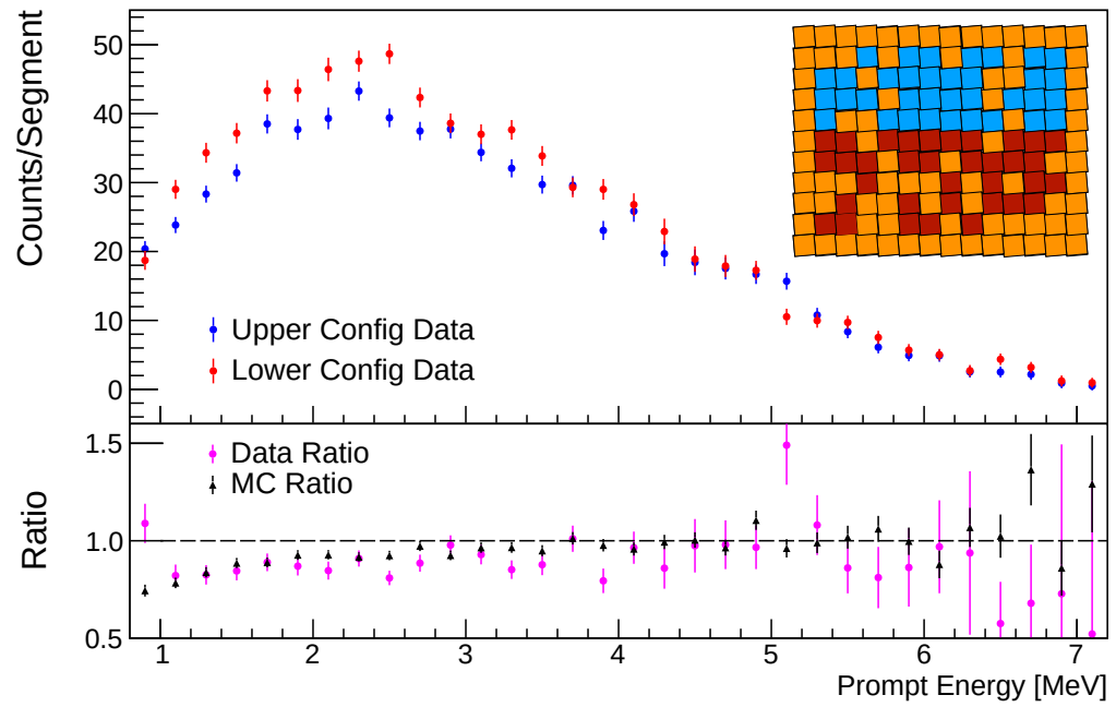
Figure 6.19: Spectra from upper/lower configurations are compared. Counts are normalized to per segment for relative comparison. Top panel : spectra of IBD candidate events (statistical errors only) from upper/lower region. Bottom panel : Ratio of two spectra bin-by-bin from Data/MC.
