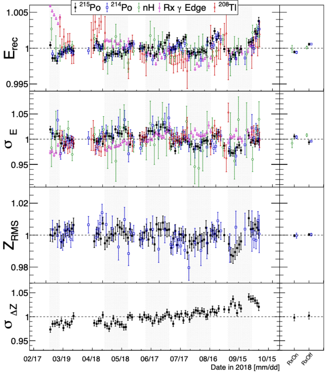
Figure 5.11: Time stability of energy, position and PSD calibration using various background events. Stability over time for both reactor-on and reactor-off. RnPo events in black, ^{214}\text{BiPo} events in blue, n-H capture \gamma -rays in green, reactor neutron capture on metal in pink and ^{208}\text{Tl} decay \gamma -rays in red. Source:[92]
