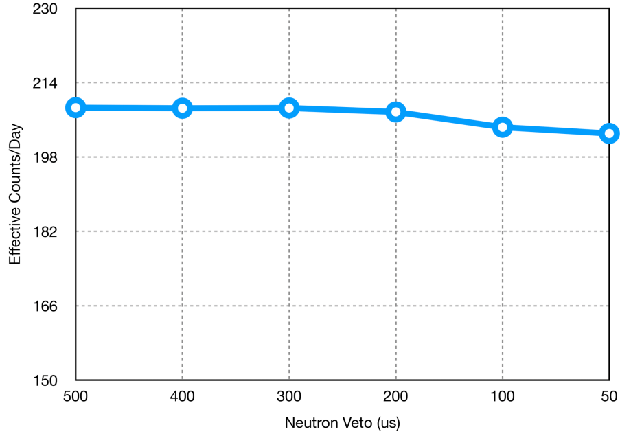
Figure 6.11: Neutron veto cut optimization. The 400 \mu s cut provides the most IBD counts.
