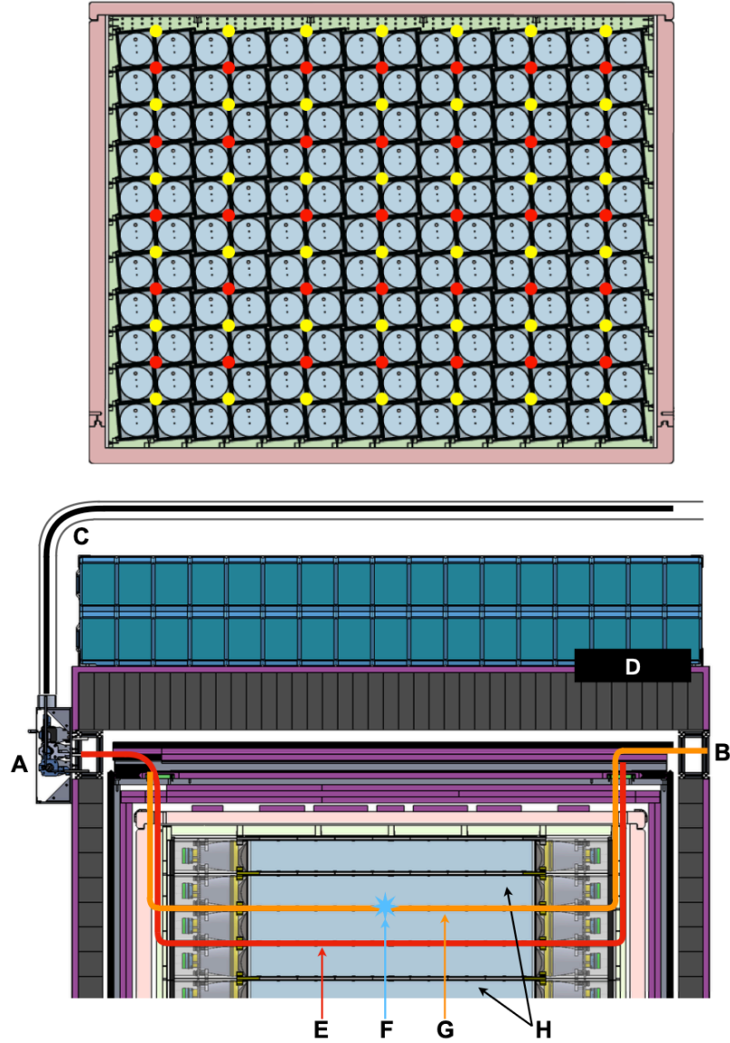
Figure 4.12: The sideview of the PROSPECT AD calibration system. Top: the optical calibration system inserts shown in yellow dots and the radioactive source calibration inserts shown in red. Bottom: AD calibration system details along the axial direction of segments. (A) source drive motors, (B) optical fiber connector panel, (C) belt storage tube, (D) shielding, (E) source deployment tube, (F) light injection point, (G) fiber tube, (H) detector segments. Source:[76]
