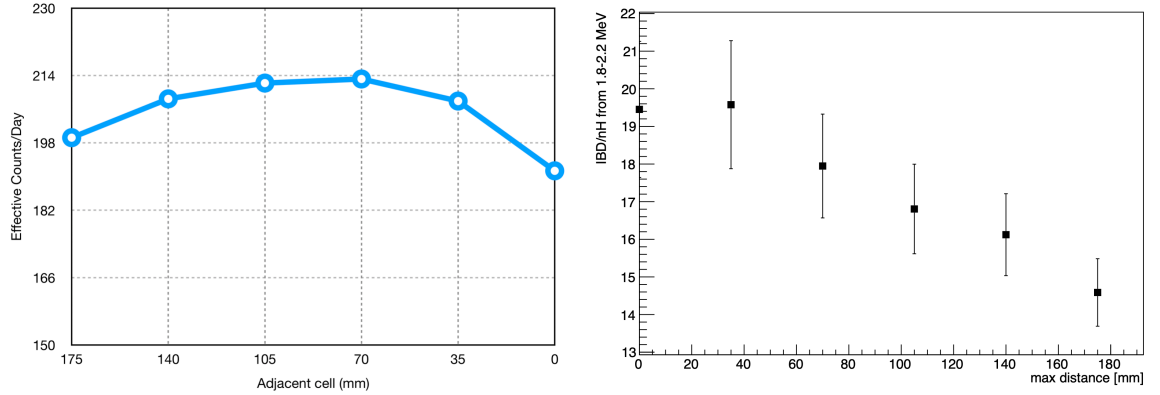
Figure 6.9: Prompt and delayed distance coincidence cut optimization in the adjacent segment. The right plot shows signal to background ratio in the nH region.
