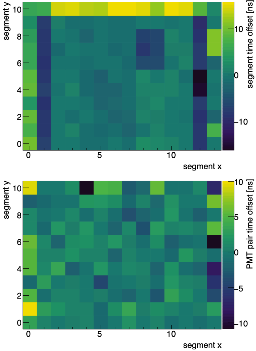
Figure 5.4: PMT timing calibration constants from one of March 2018 physics run. Top: \bar{t}_i segment map; clear features visible between ET and Hamamatsu PMTs, originating from the clock offsets and systematic differences. Bottom; d\bar{t}_i segment map. Source:[92]
