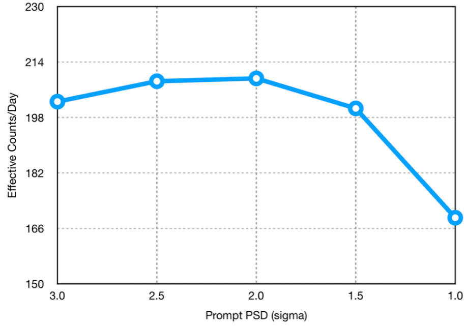
Figure 6.4: Prompt PSD optimization
