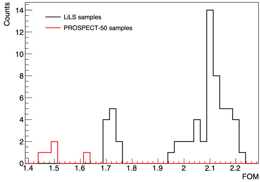
Figure 4.5: QA measurements of the figure of merit of the produced {}^6\text{LiLS} compared to the prototype PROSPECT-50 requirement. Source:[84]
