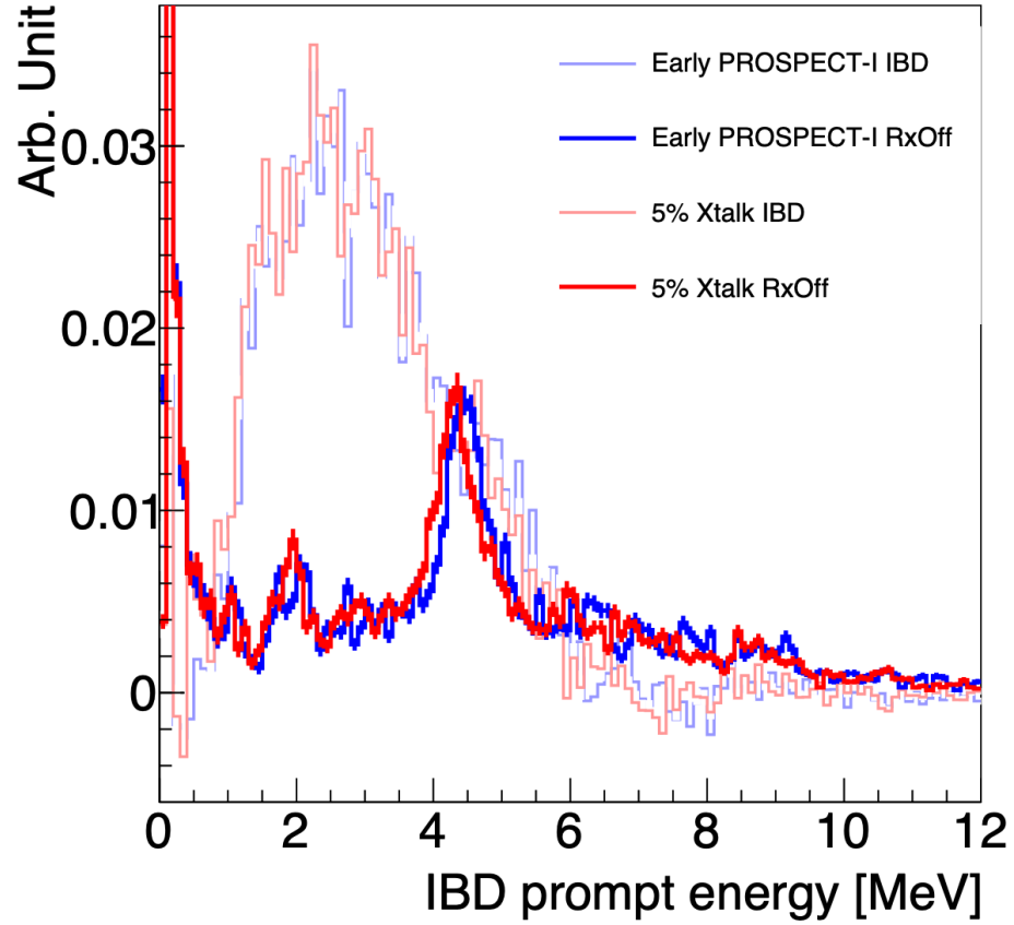
Figure 7.8: Using PROSPECT-I early dataset, the IBD-like prompt spectra are shown for reactor-off periods and reactor-on periods with full background subtraction. The blue is the original dataset without cross-talk and the red is applied with artificial cross-talk. Source:[117]
