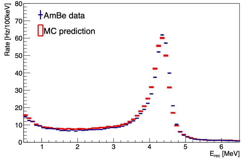
Figure 5.14: Spectrum comparison between data and best-fit energy scale model for AmBe source. Source:[92]
