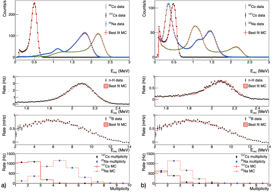
Figure 8.6: Data-simulation comparison of calibration source spectra and event multiplicity for a) best-fit internal energy scale model and b) best-fit external energy scale model. The reconstructed energy E_{\text{rec}} represents scintillator quenched visible energy, which is shifted to lower energy compared to the true gamma energies. External calibration events generally have lower event statistics and decreased event multiplicity due to smaller solid angle coverage. The external calibration spectra show more pronounced single- \gamma -ray photopeaks, with lower rates of total \gamma -ray photopeaks. The total \chi^2 from both energy scale models are listed in Table 8.2.
