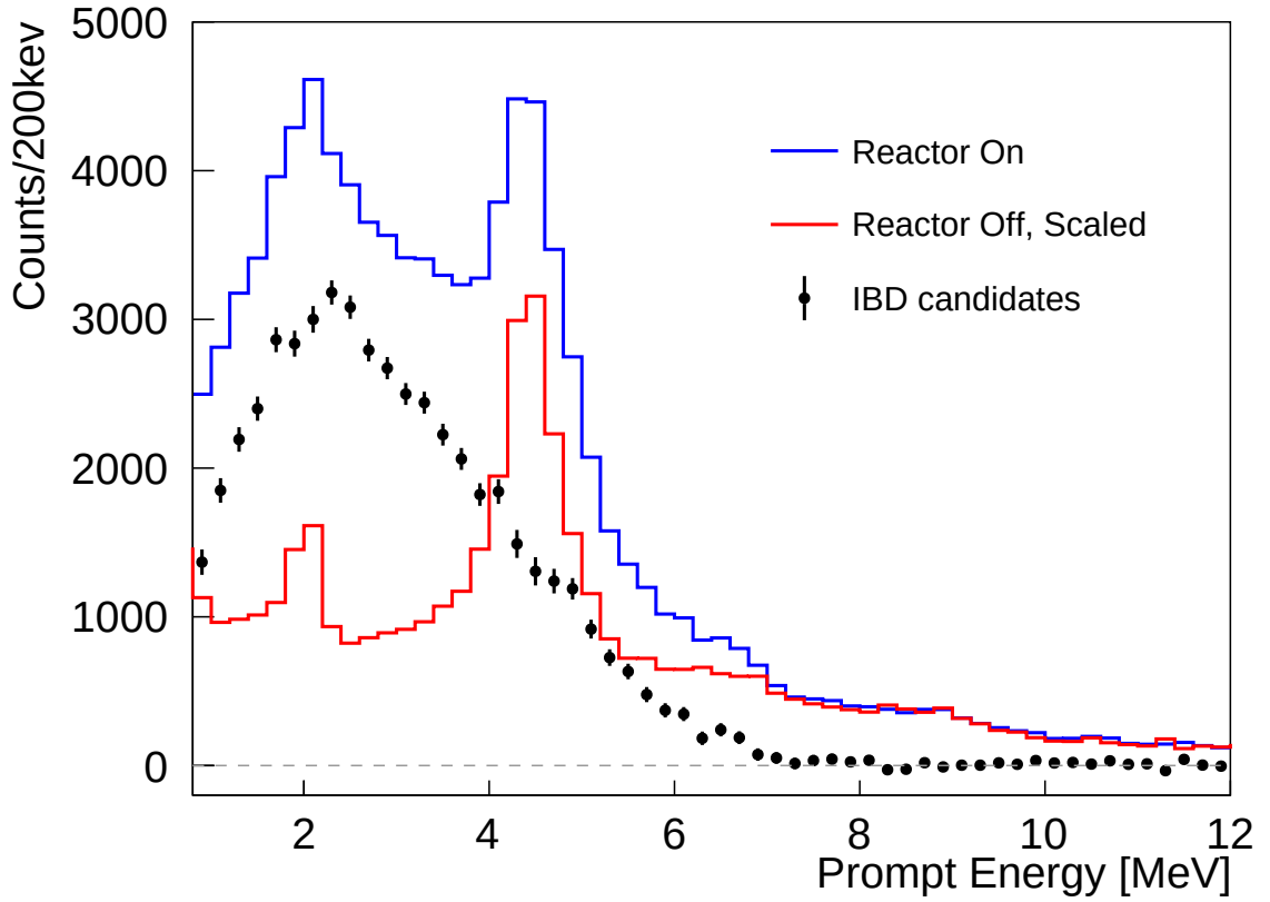
Figure 6.15: The reconstructed visible prompt energy E_{rec} (black marker) spectrum of IBD candidates (statistical error only) in addition to reactor-on( blue solid ) and reactor-off (red solid) correlated candidates. The reactor-off spectrum is properly scaled to match reactor-on live time. Atmosphere scaling is also included to scale reactor-off background and all accidental events have been subtracted in the above spectra.
