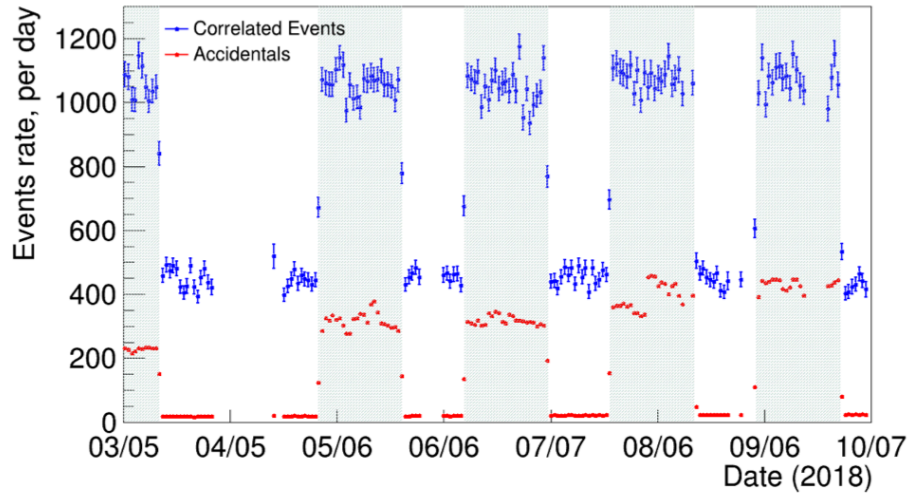
Figure 6.17: Time dependence of correlated IBD candidate rates. The rates are integrated between 0.8 and 7.2 MeV energy range. Source:[92]
