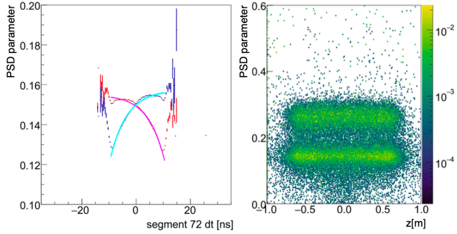
Figure 5.7: Left: Position dependent PSD vs dt for a particular segment. The blue and red are PSD data. Cyan and magenta represents the fits described in Equation 5.13. Right: PSD values after the position correction. Source:[101]
