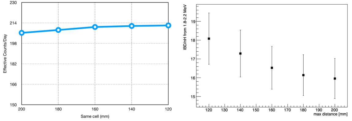
Figure 6.8: Prompt and delayed distance coincidence cut optimization in the same segment. The right plot shows signal to background ratio in the nH region.
