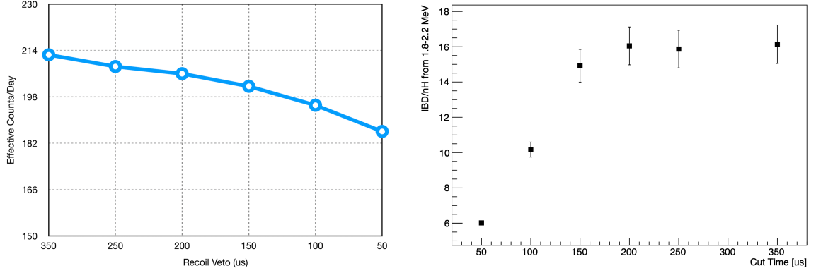
Figure 6.12: Recoil veto cut optimization. The right plot shows signal to background ration in the nH region.
