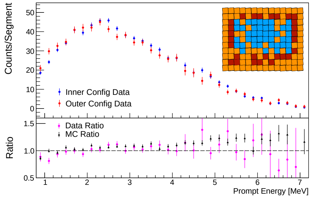
Figure 6.20: Spectra from inner/outer configurations are compared. Counts are normalized to per segment for relative comparison. Top panel : spectra of IBD candidate events (statistical errors only) from inner/outer region. Bottom panel : Ratio of two spectra bin-by-bin from Data/MC.
