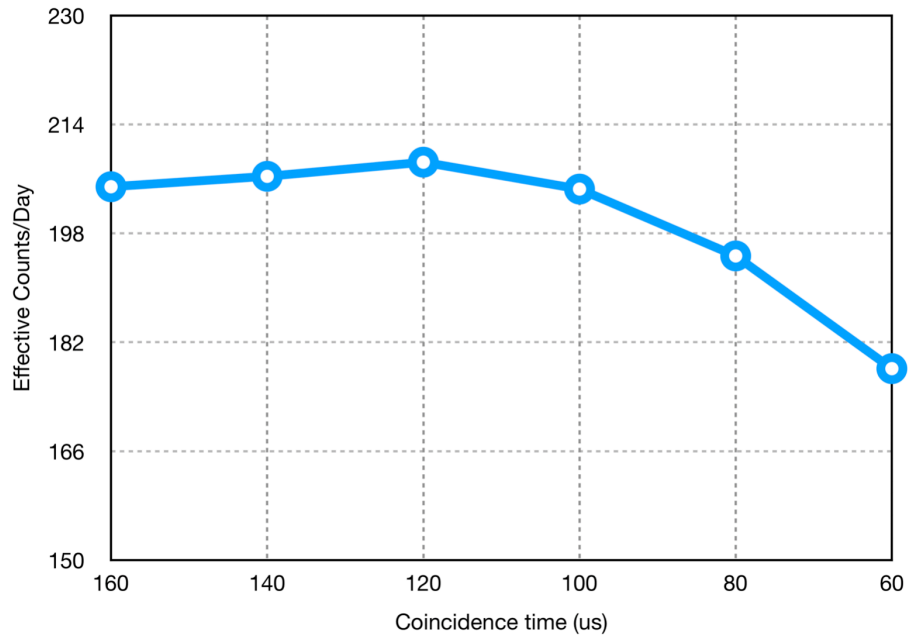
Figure 6.7: Prompt and delayed timing coincidence cut optimization.
