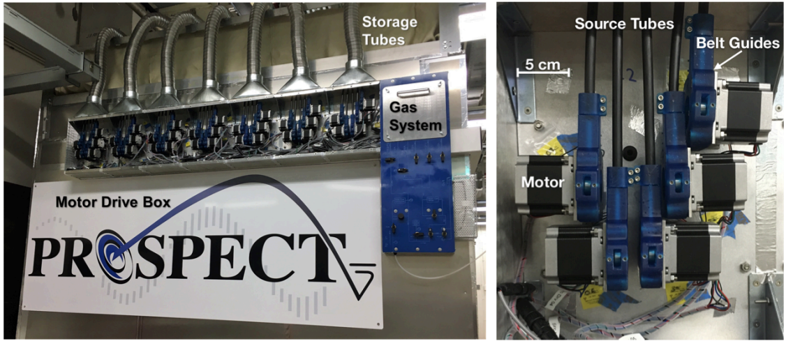
Figure 4.14: Pictures of fully installed radioactive source calibration system, mounted on the side of the detector exterior. The right picture shows a close-up view of the stepper motor modules and calibration tubes. Source:[88]
