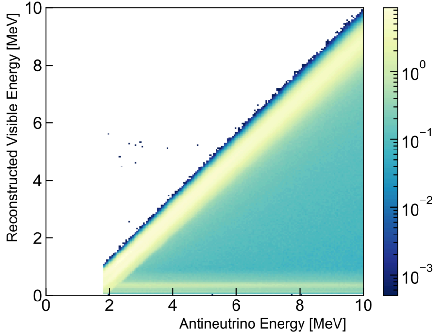
Figure 5.16: The PROSPECT AD response matrix that converts incident neutrino spectrum to prompt visible energy spectrum. Source:[92]
