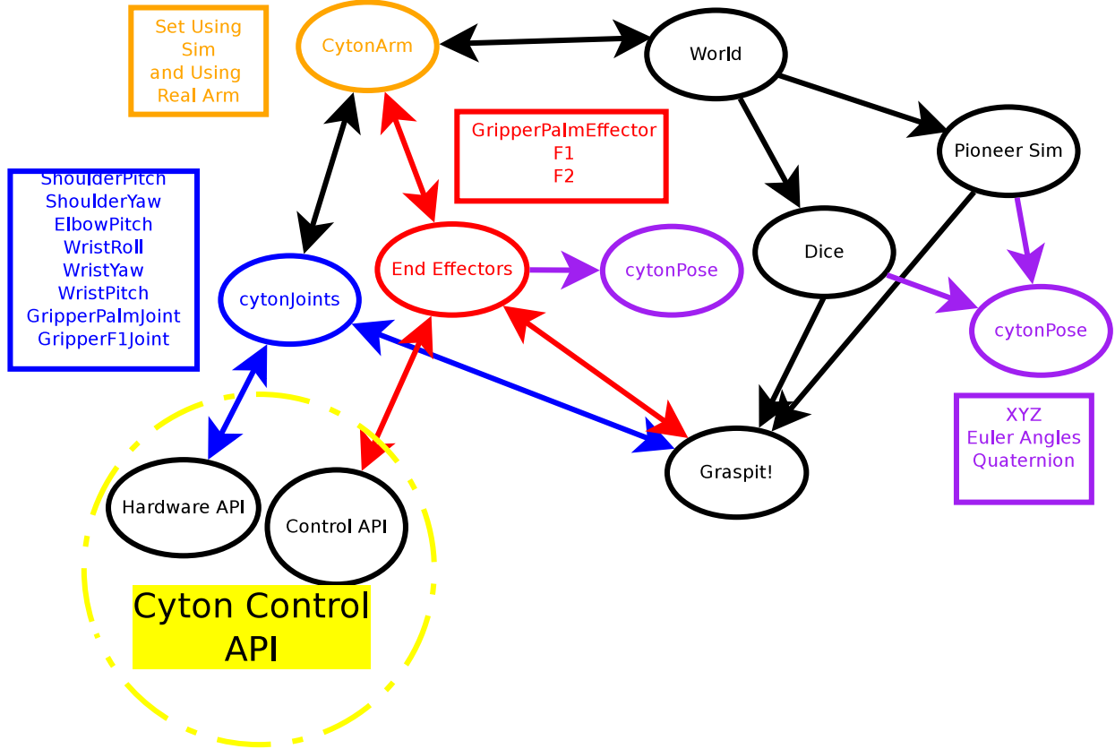
Figure 3.3: cytonGrasp Layout
