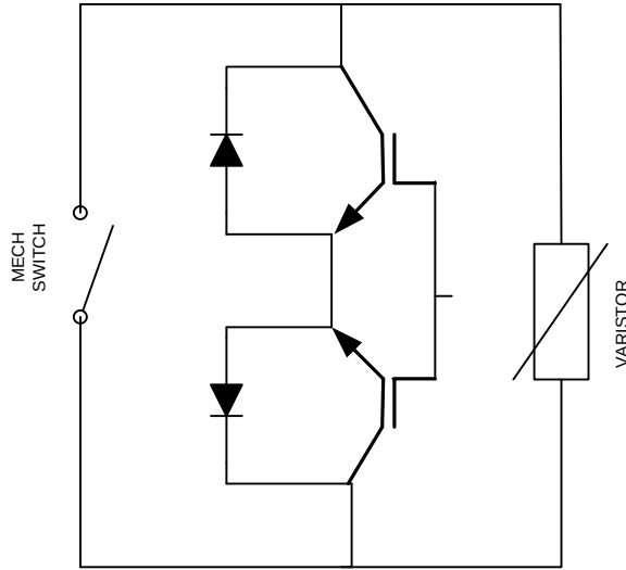
Figure 3.6 DC hybrid circuit for fault interruption [47].
