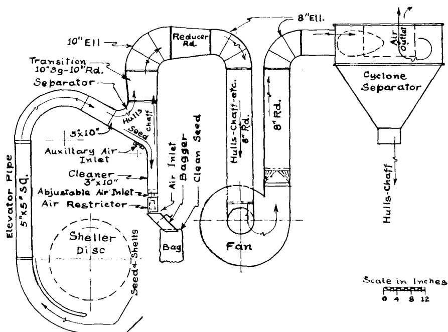
Fig. 5—Diagrammatic layout of elevator-separator-cleaner unit.
