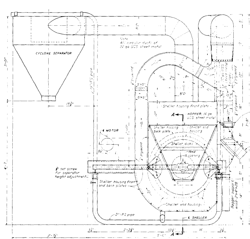
Fig. 2—Assembly layout.
