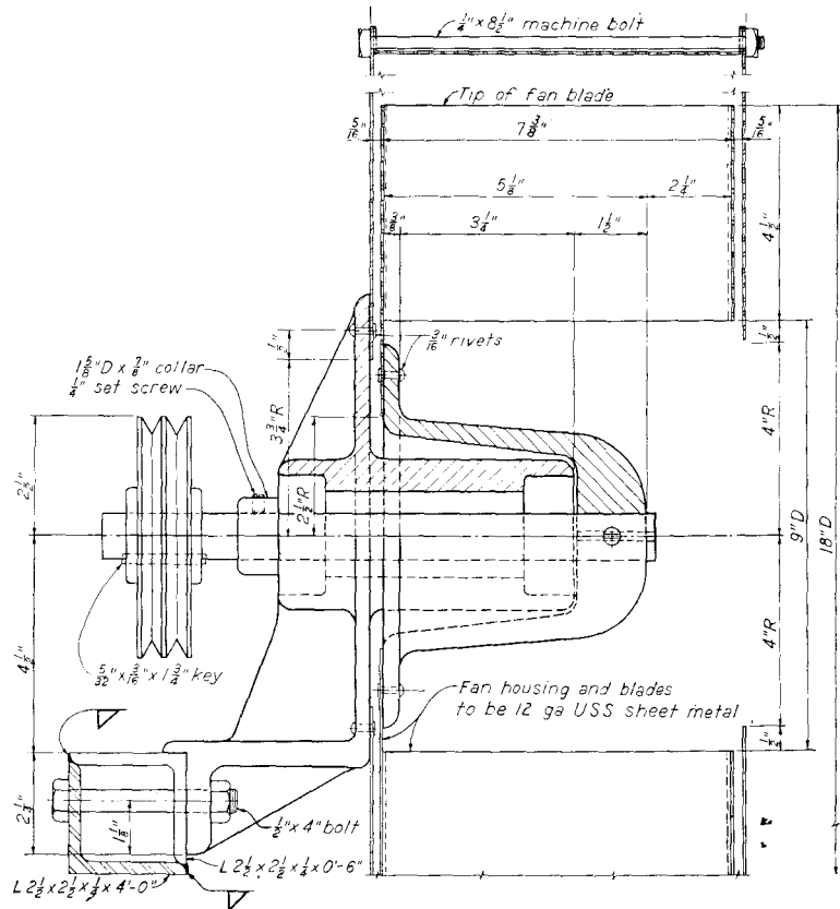
Fig. 4—Fan details.
