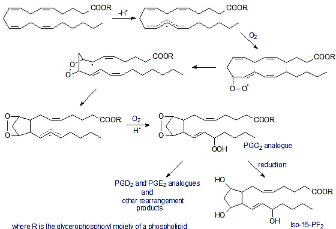
Figure 1.5 Formation of 15- F 2 isoprostane from arachidonic acid. A reactive oxygen species abstracts a hydrogen atom from a methylene group under aerobic conditions. Since this radical generation is not enzymatic, all methylene groups between two cis double bonds can potentially be involved. After hydrogen extraction, the radical formed combines with an oxygen molecule to generate a peroxy radical which rearranges. The bicyclic endoperoxy radical reacts on either face of the side chain with a further oxygen molecule to produce racemic hydroperoxy bicyclic endoperoxy radicals. The radical chain is terminated by abstraction of hydrogen from an appropriate donor. Analogous reactions can occur to produce isoprostanes with the hydroxyl group in positions 5, 8 or 12.
