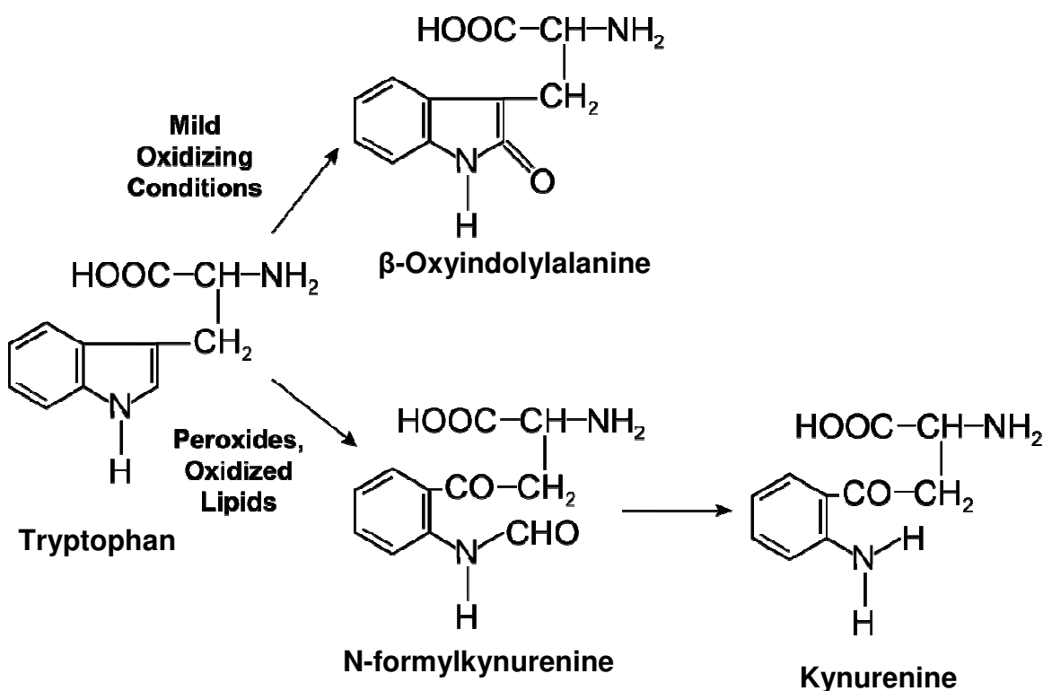
Figure 1.14 Tryptophan derivatives from food processing. Under mild oxidizing conditions, tryptophan is oxidized to \beta -Oxyindolylalanine. Under more severe oxidizing conditions, tryptophan is oxidized to N-formylkynurenine and kynurenine.
