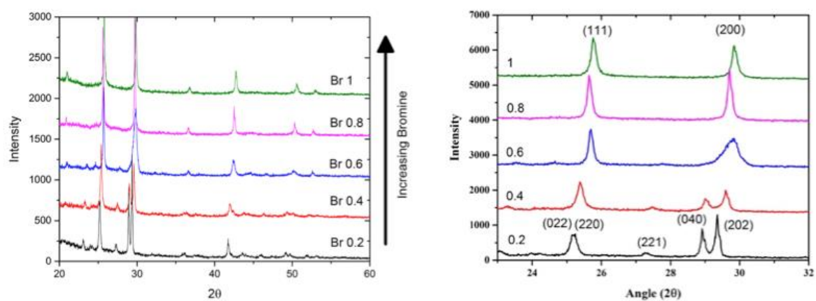
Figure 18: Powder XRD patterns for the five \text{CsCaBr}_x\text{I}_{3-x}:\text{Eu} crystals (left) and a zoomed in region of interest (right).
