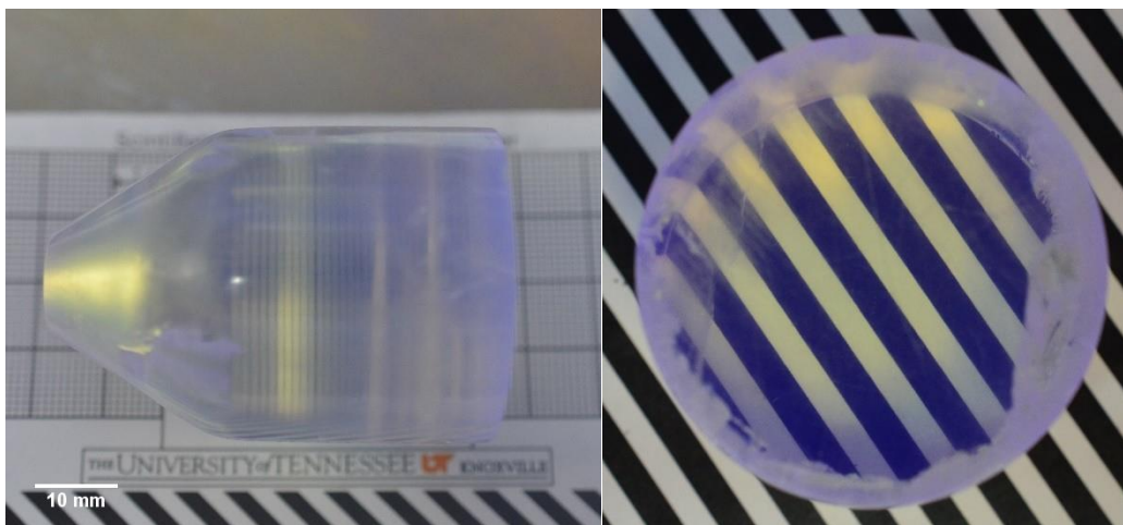
Figure 32: \varnothing 38 mm \text{CsCaBr}_{0.8}\text{I}_{2.2}:\text{Eu} crystal full boule (left) and 34 mm tall cylinder (right). The cut crystal shows only minor surface cracking.
