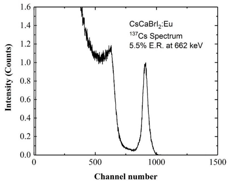
Figure 23: ^{137}\text{Cs} Spectrum measured with the \text{CsCaBr}_2:\text{Eu} slab.
