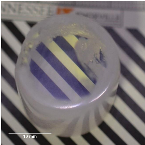
Figure 25: Full boule of \text{CsCaBr}_{0.8}\text{I}_{2.2}:\text{Eu} 2% (left) and a 1 cm cube sourced from the crystal.
