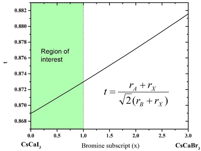
Figure 8: Goldschmidt tolerance factor for \text{CsCaX}_3 (I,Br) and the region of interest for this work.
