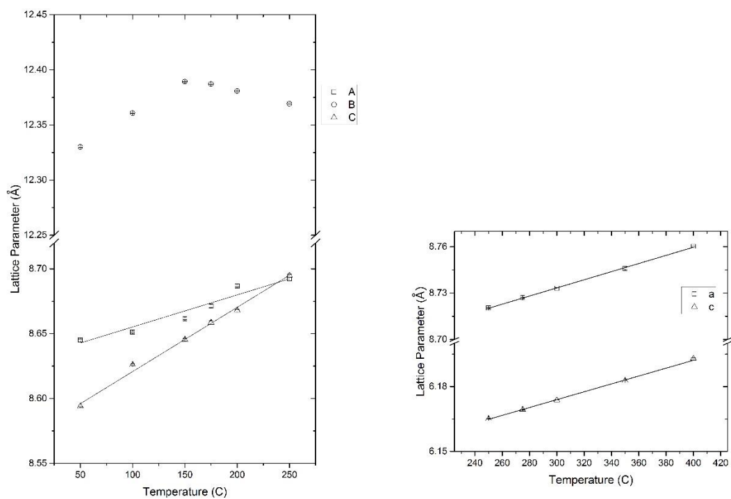
Figure 13: Lattice parameters and linear fits for the low temperature and high temperature phases of \text{CsCaI}_3:\text{Eu} .
