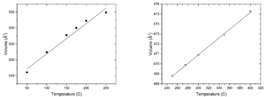
Figure 14: Unit Cell volume and linear fits for the low and high temperature phases of \text{CsCa}_{13}\text{Eu} .
