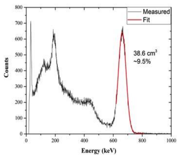
Figure 33: ^{137}\text{Cs} Spectrum of the \varnothing 38 mm \text{CsCaBr}_{0.8/2.2}:\text{Eu} crystal. Crystal volume and energy resolution are shown next to the full energy peak.
