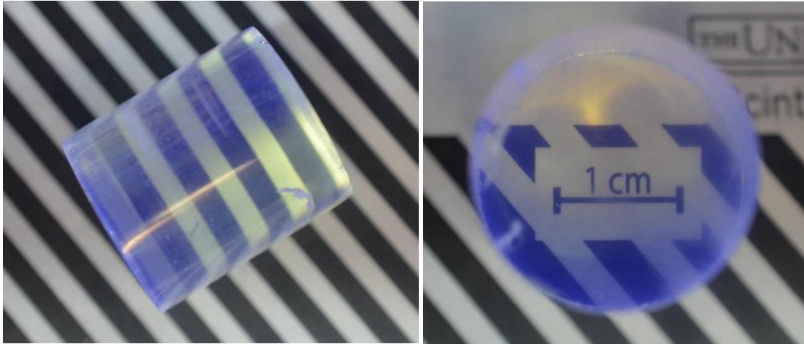
Figure 29: Cut and polished boule of \text{CsCaBr}_{0.8/2.2}:\text{Eu} grown in a transparent furnace.
