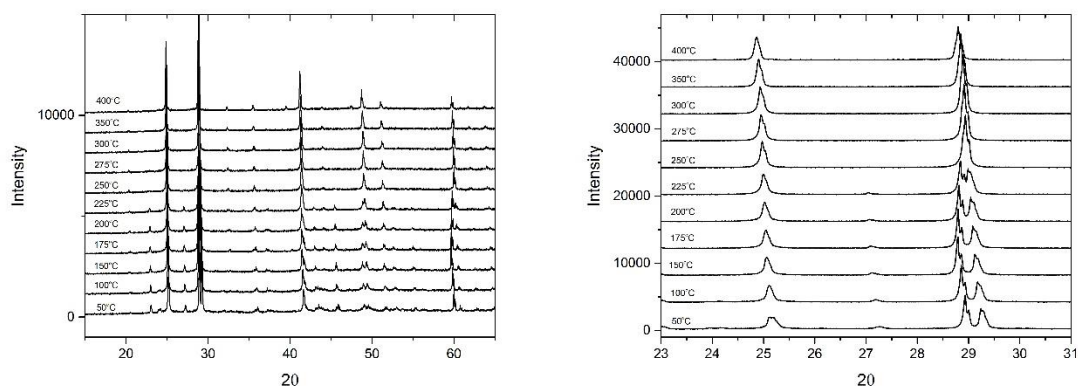
Figure 12: Powder XRD scans for \text{CsCa}_{13}\text{:Eu} for the entire range (left) and a close up on a region of interest (right). The orthorhombic phase can be seen at temperatures below 250^\circ\text{C} , while a tetragonal phase is observed above this temperature.
