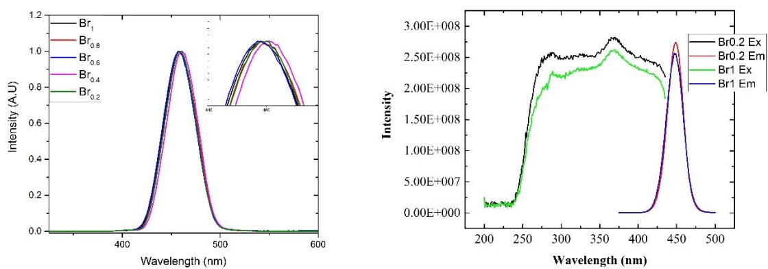
Figure 22: Radioluminescence of the five \text{CsCaBr}_{3-x}\text{:Eu} slabs (left) and Photoluminescence of the two end point crystals (right).
