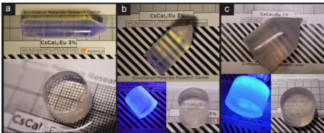
Figure 5: Single crystal boules of \text{CsCaI}_3:\text{Eu} at \varnothing 15 mm (a), \varnothing 22 mm (b) and \varnothing 35 mm (c). The transparency of the material degrades as the thickness of the boule increases.
