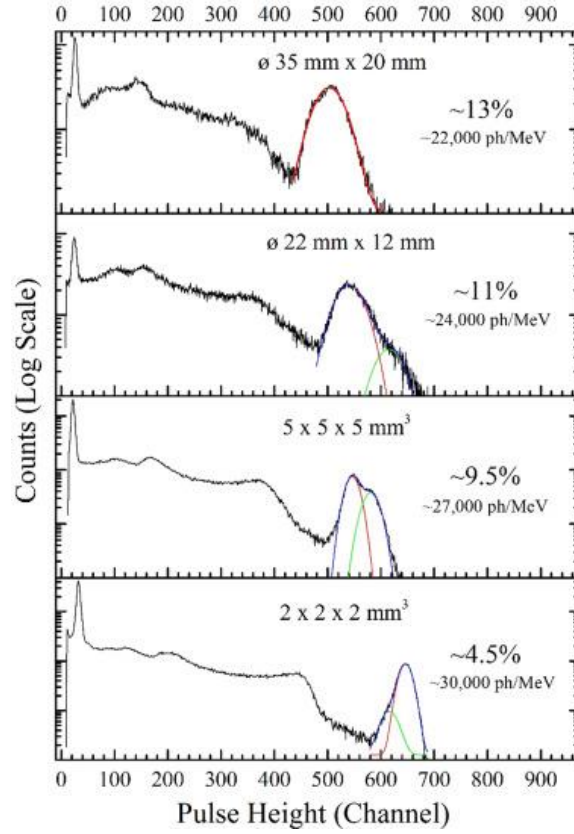
Figure 6: ^{137}\text{Cs} Spectra for various size crystals of \text{CsCaI}_3:\text{Eu} [32]. The performance of \text{CsCaI}_3:\text{Eu} degrades as the sample size increases.
