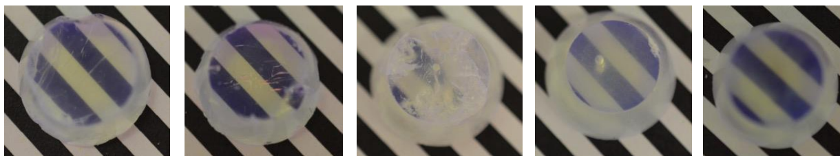
Figure 16: Crystals as removed from their ampoules and polished (above) and 5 mm slabs cut from their cone regions. The samples of the left have the highest bromine and the best optical quality, while the samples on the right have the lowest bromine and are less transparent.
