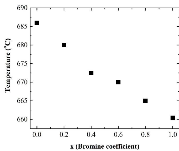
Figure 17: Melting temperature of CsCaBr x I 3-x :Eu as measured with Differential Scanning Calorimetry.
