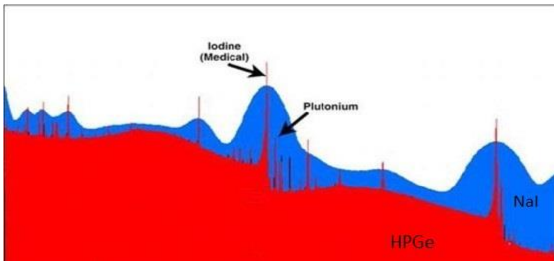
Figure 4: Pulse Height Spectrum comparing resolutions HPGe (red) and NaI:TI (blue) [8].
