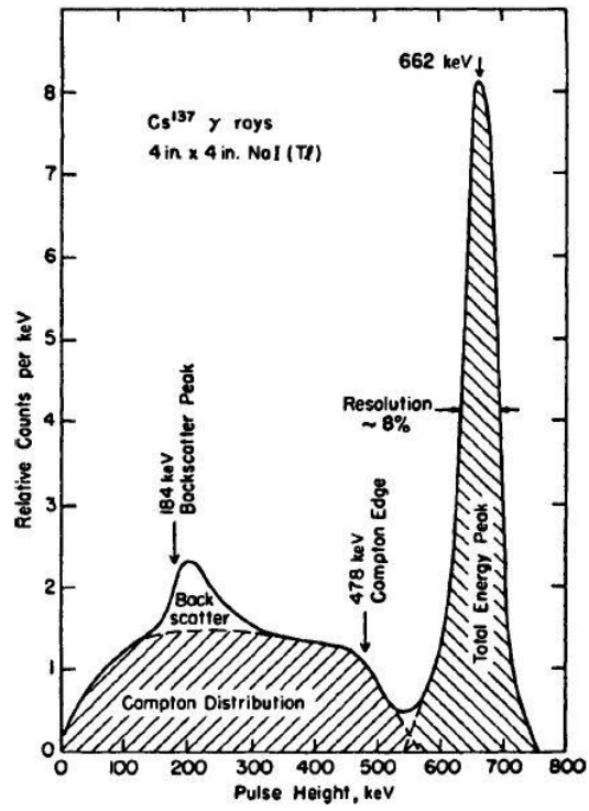
Figure 3: Pulse Height Spectrum from a NaI(Tl) Scintillator irradiated with a ^{137}\text{Cs} source [2].
