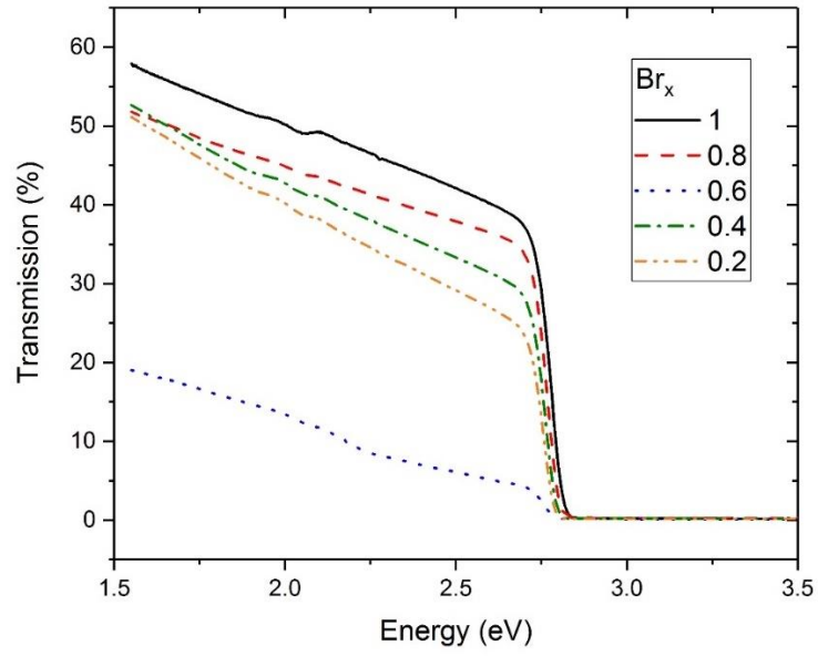
Figure 21: Transmission measurement for 1 mm thick slabs of \text{CsCaBr}_x\text{I}_{3-x} . The value shown in the figure legend represents the bromine coefficient in the chemical composition.
