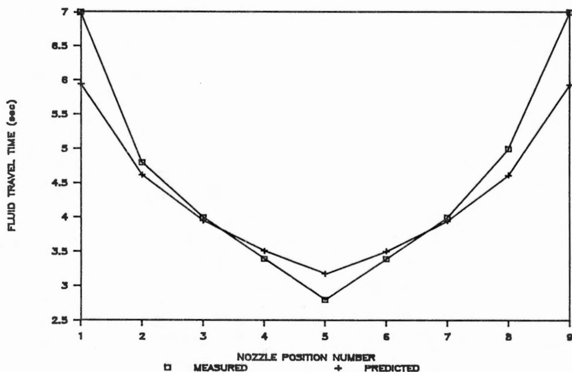
Figure 9. Measured and predicted transient times for fluid travel in a direct injection boom-type sprayer with the injection point at the upstream side of the sprayer system pump and the operating pressure maintained at 275 kPa.
