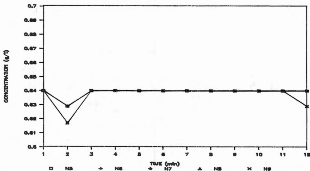
Figure 22. Variation in chemical concentration in the effluent of nozzles 5 through 9 as a function of time. Chemical injection with the FMI pump was immediately upstream of the system pump. Sampling began at time = 1 min, and system pressure was 275 kPa.
