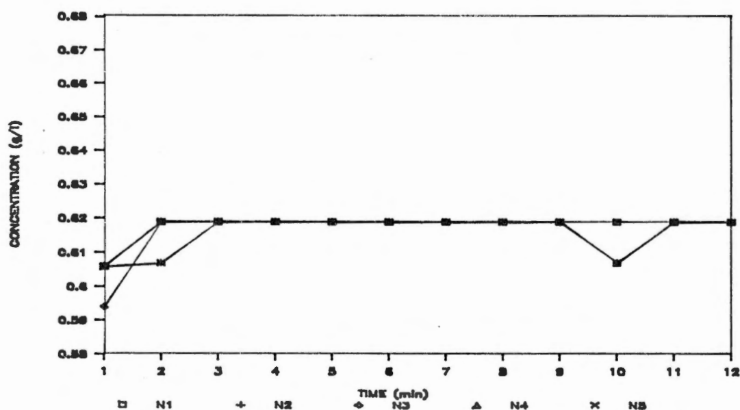
Figure 19. Variation in chemical concentration in the effluent of nozzles 1 through 5 as a function of time. Chemical injection with the Scienco pump was immediately upstream of the system pump. Sampling began at time = 1 min, and system pressure was 275 kPa.
