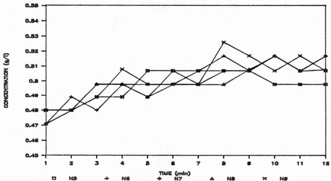
Figure 33. Variation in chemical concentration of the effluent of nozzles 5 through 9 as a function of time. Chemical injection with the Scienco pump was immediately downstream of the system pump. Sampling began at time = 1 min, and system pressure was 275 kPa.
