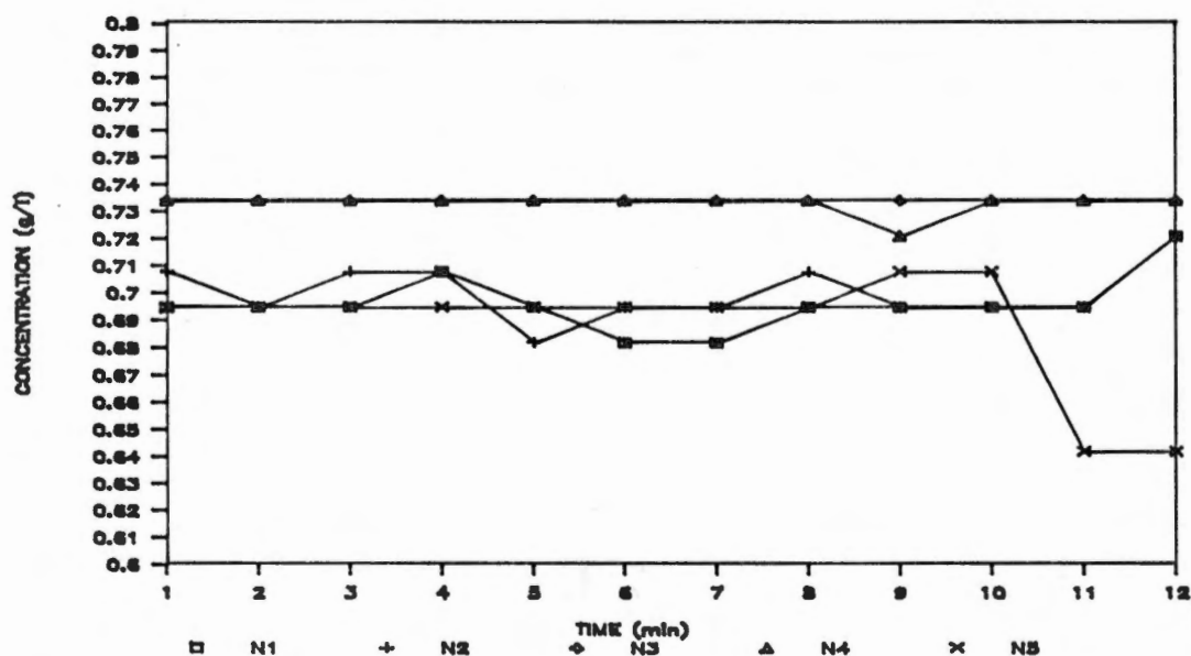
Figure 54. Variation in chemical concentration in the effluent of nozzles 1 through 5 as a function of time. Chemical injection with the FMI pump was at the individual nozzles, and fluid entrance to the boom was slightly to the side of nozzle 5. Sampling began at time = 1 min, and system pressure was 171 kPa.
