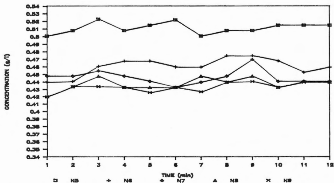
Figure 49. Variation in chemical concentration in the effluent of nozzles 5 through 9 as a function of time. Chemical injection with the Scienco pump was at the individual nozzles, and fluid entrance to the boom was slightly to the side of nozzle 5. Sampling began at time = 1 min, and system pressure was 275 kPa.
