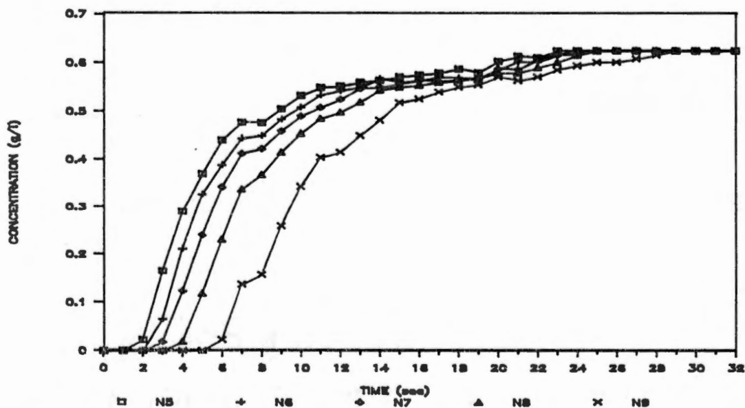
Figure 12. Variation in chemical concentration in the effluent of nozzles 5 through 9 as a function of time. Chemical injection with the peristaltic pump was immediately upstream of the system pump. Injection began at time = 0, and system pressure was 275 kPa.
