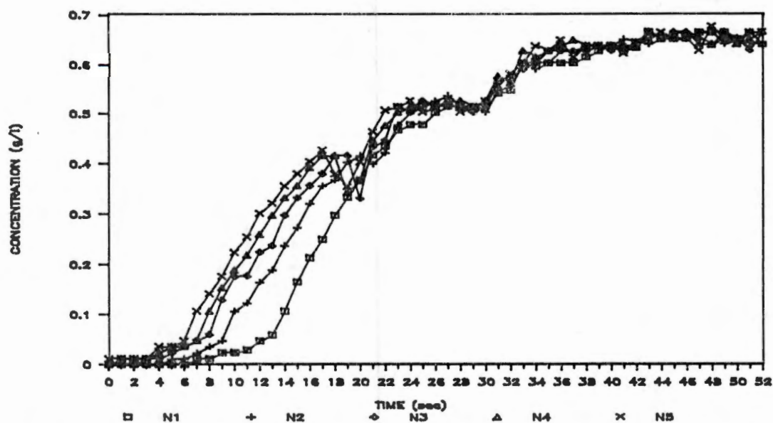
Figure 24. Variation in chemical concentration in the effluent of nozzles 1 through 5 as a function of time. Chemical injection with the FMI pump was immediately downstream of the system pump. Injection began at time = 0, and system pressure was 275 kPa.
