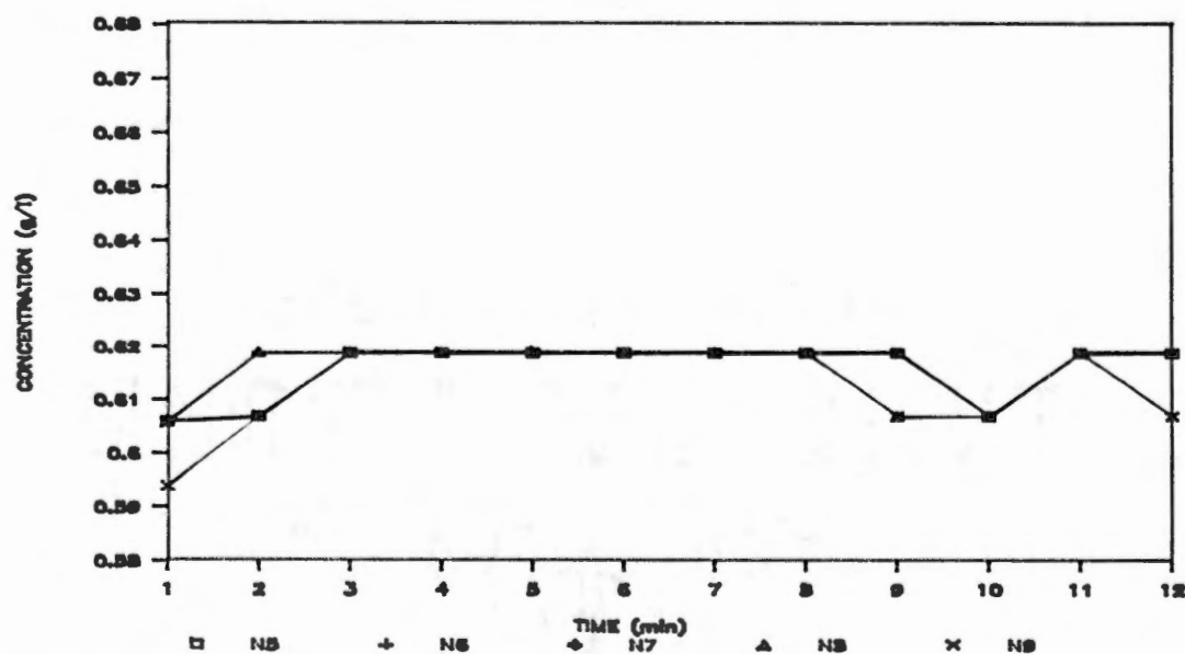
Figure 20. Variation in chemical concentration in the effluent of nozzles 5 through 9 as a function of time. Chemical injection with the Scienco pump was immediately upstream of the system pump. Sampling began at time = 1 min, and system pressure was 275 kPa.
