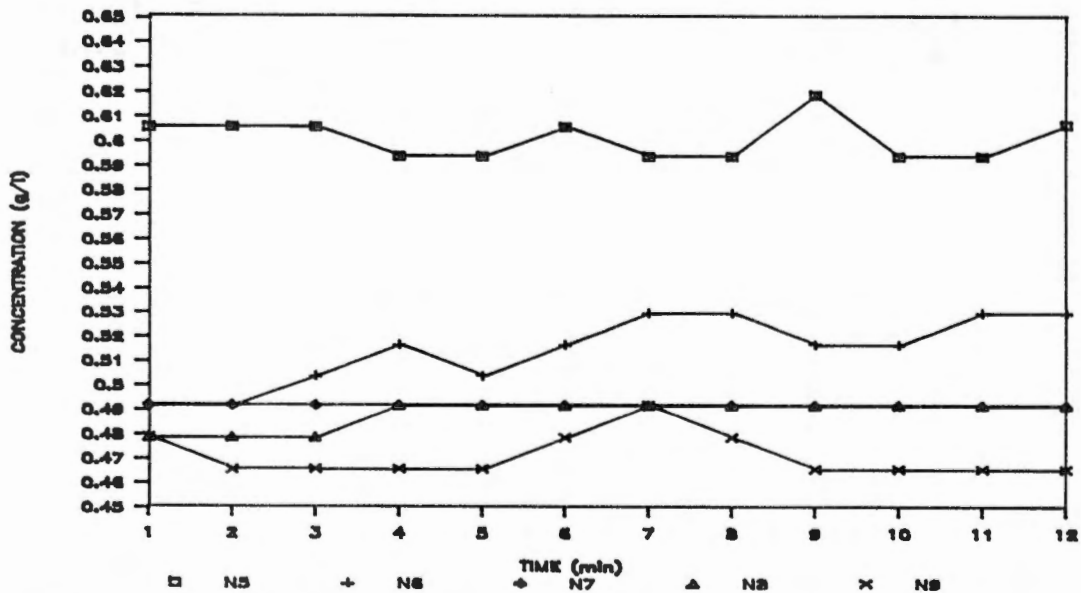
Figure 59. Variation in chemical concentration in the effluent of nozzles 5 through 9 as a function of time. Chemical injection with the FMI pump was at the individual nozzles, and fluid entrance to the boom was slightly to the side of nozzle 5. Sampling began at time = 1 min, and system pressure was 378 kPa.
