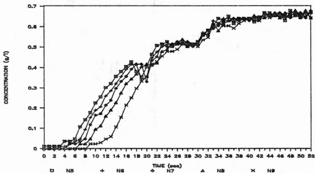
Figure 25. Variation in chemical concentration in the effluent of nozzles 5 through 9 as a function of time. Chemical injection with the FMI pump was immediately downstream of the system pump. Injection began at time = 0, and system pressure was 275 kPa.
