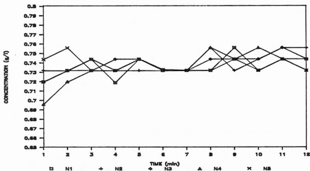
Figure 34. Variation in chemical concentration in the effluent of nozzles 1 through 5 as a function of time. Chemical injection with the FMI pump was immediately downstream of the system pump. Sampling began at time = 1 min, and system pressure was 171 kPa.
