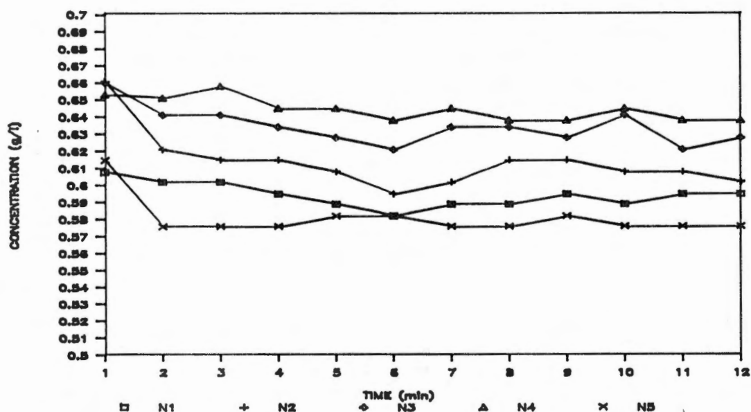
Figure 50. Variation in chemical concentration in the effluent of nozzles 1 through 5 as a function of time. Chemical injection with the FMI pump was at the individual nozzles, and fluid entrance to the boom was slightly to the side of nozzle 5. Sampling began at time = 1 min, and system pressure was 275 kPa.
