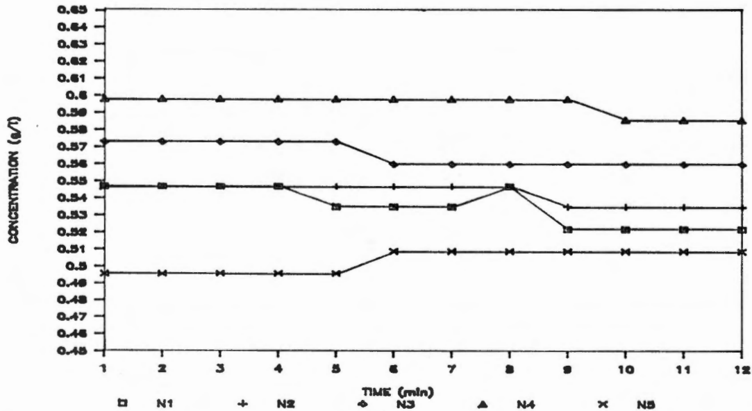
Figure 56. Variation in chemical concentration in the effluent of nozzles 1 through 5 as a function of time. Chemical injection with the Scienco pump was at the individual nozzles, and fluid entrance to the boom was slightly to the side of nozzle 5. Sampling began at time = 1 min, and system pressure was 378 kPa.
