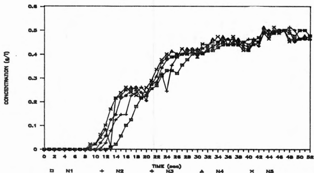
Figure 26. Variation in chemical concentration in the effluent of nozzles 1 through 5 as a function of time. Chemical injection with the Scienco pump was immediately downstream of the system pump. Injection began at time = 0, and system pressure was 275 kPa.
