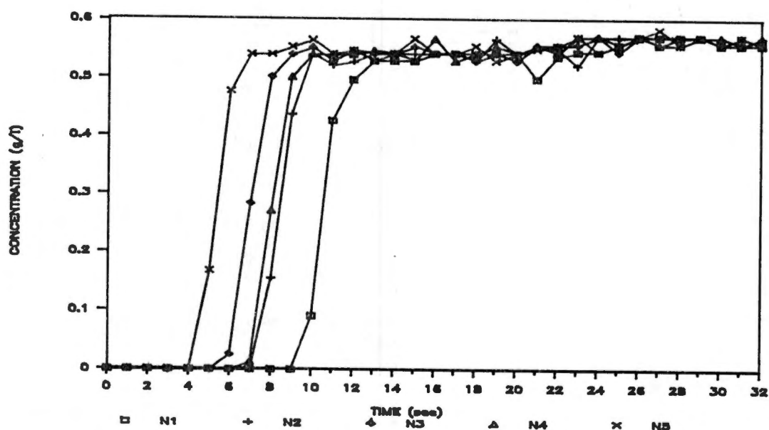
Figure 28. Variation in chemical concentration in the effluent of nozzles 1 through 5 as a function of time. Chemical injection with the Scienco pump was immediately downstream of the system pump. A smaller check valve was included. Injection began at time = 0, and system pressure was 275 kPa.
