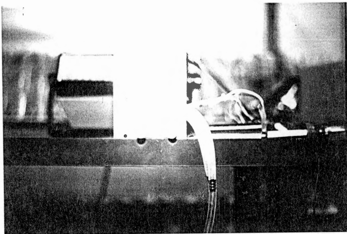
Figure 3. Master Flex TM peristaltic pump, manufactured by Cole-Parmer Instrument Company, used for direct chemical injection on the low-pressure side of the sprayer system pump.
