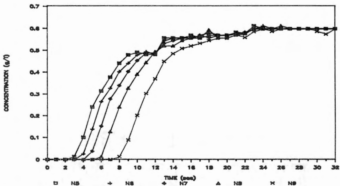
Figure 14. Variation in chemical concentration in the effluent of nozzles 5 through 9 as a function of time. Chemical injection with the Scienco pump was immediately upstream of the system pump. Injection began at time = 0, and system pressure was 275 kPa.
