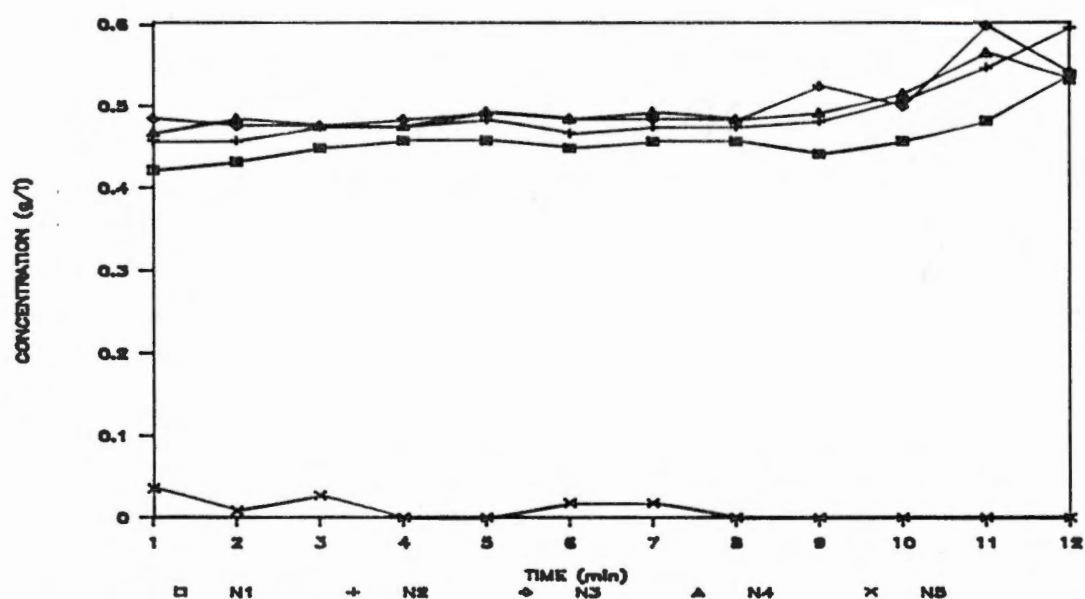
Figure 45. Variation in chemical concentration in the effluent of nozzles 1 through 5 as a function of time. Chemical injection with the Scienco pump was at the individual nozzles. Sampling began at time = 1 min, and system pressure was 275 kPa.
