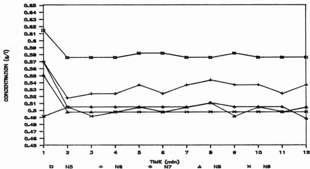
Figure 51. Variation in chemical concentration in the effluent of nozzles 5 through 9 as a function of time. Chemical injection with the FMI pump was at the individual nozzles, and fluid entrance to the boom was slightly to the side of nozzle 5. Sampling began at time = 1 min, and system pressure was 275 kPa.
