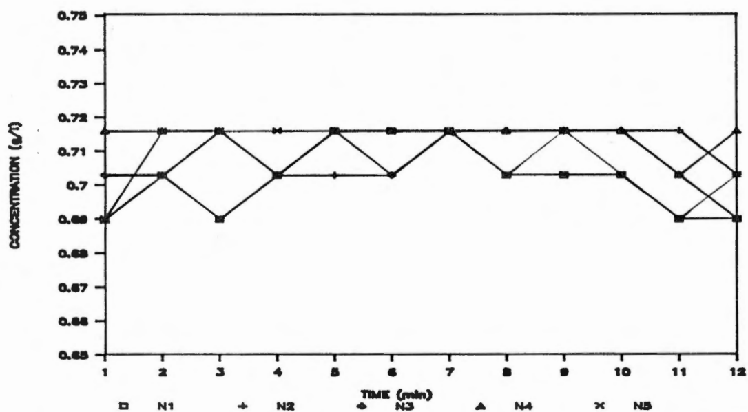
Figure 65. Variation in chemical concentration in the effluent of nozzles 1 through 5 as a function of time with a conventional application system at a pressure of 171 kPa. Sampling began at 1 min.
