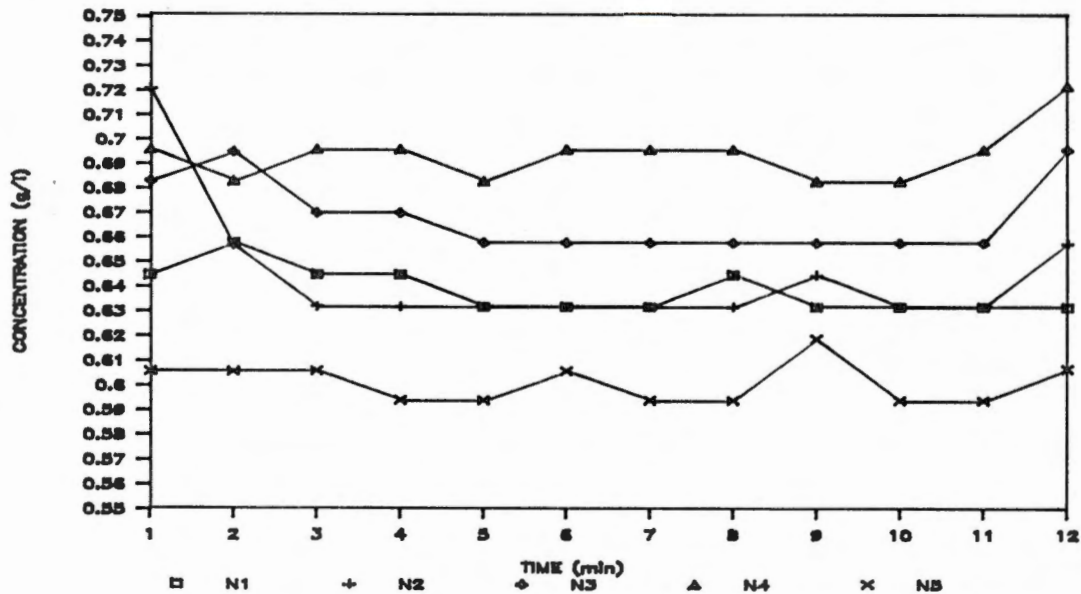
Figure 58. Variation in chemical concentration in the effluent of nozzles 1 through 5 as a function of time. Chemical injection with the FMI pump was at the individual nozzles, and fluid entrance to the boom was slightly to the side of nozzle 5. Sampling began at time = 1 min, and system pressure was 378 kPa.
