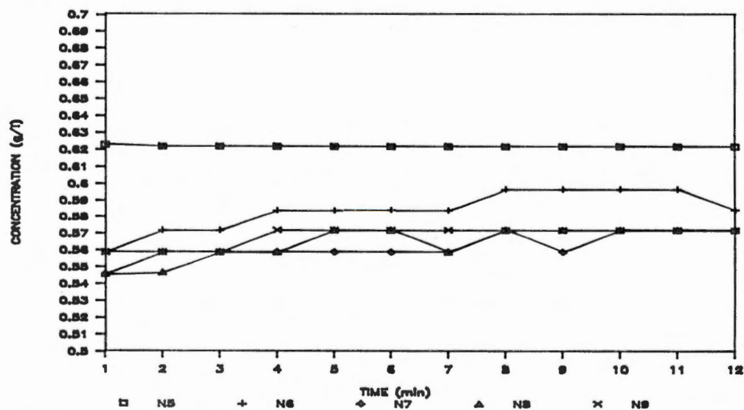
Figure 53. Variation in chemical concentration in the effluent of nozzles 5 through 9 as a function of time. Chemical injection with the Scienco pump was at the individual nozzles, and fluid entrance to the boom was slightly to the side of nozzle 5. Sampling began at time = 1 min, and system pressure was 171 kPa.
