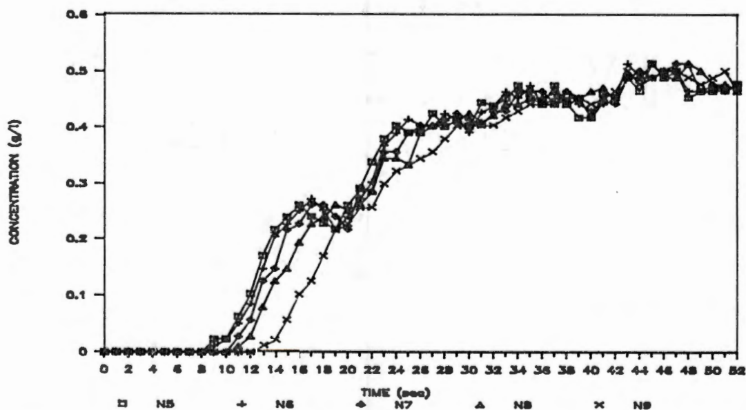
Figure 27. Variation in chemical concentration in the effluent of nozzles 5 through 9 as a function of time. Chemical injection with the Scienco pump was immediately downstream of the system pump. Injection began at time = 0, and system pressure was 275 kPa.
