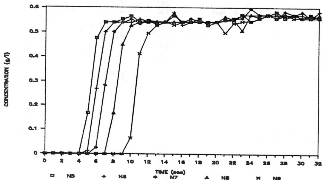
Figure 29. Variation in chemical concentration in the effluent of nozzles 5 through 9 as a function of time. Chemical injection with the Scienco pump was immediately downstream of the system pump. A smaller check valve was included. Injection began at time = 0, and system pressure was 275 kPa.
