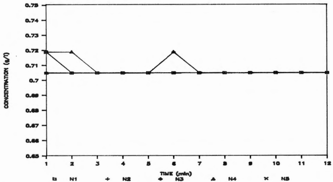
Figure 63. Variation in chemical concentration in the effluent of nozzles 1 through 5 as a function of time with a conventional application system at a pressure of 275 kPa. Sampling began at 1 min.
