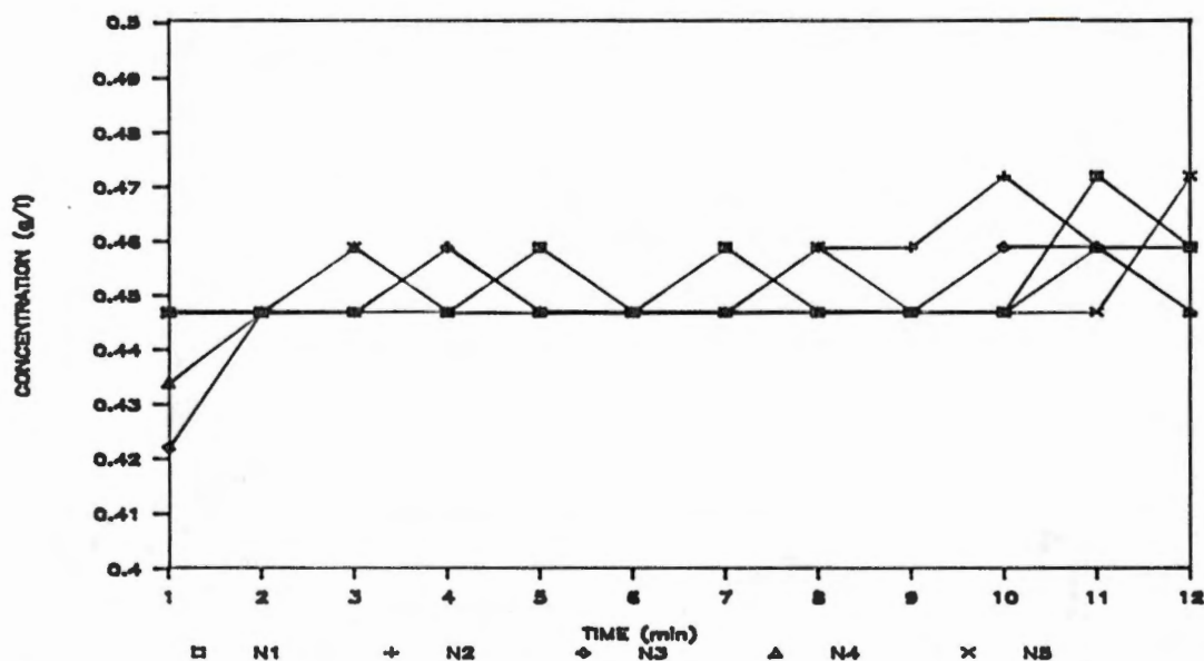
Figure 40. Variation in chemical concentration in the effluent of nozzles 1 through 5 as a function of time. Chemical injection with the Scienco pump was immediately downstream of the system pump. Sampling began at time = 1 min, and system pressure was 378 kPa.
