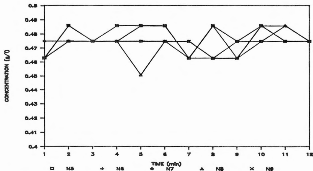
Figure 39. Variation in chemical concentration in the effluent of nozzles 5 through 9 as a function of time. Chemical injection with the FMI pump was immediately downstream of the system pump. Sampling began at time = 1 min, and system pressure was 378 kPa.
