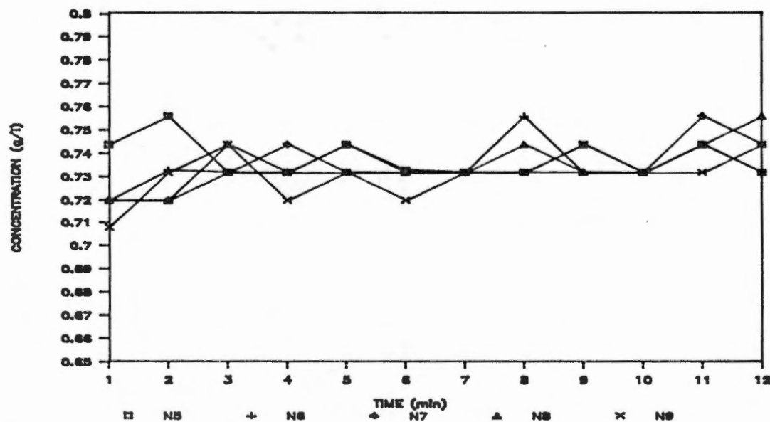
Figure 35. Variation in chemical concentration in the effluent of nozzles 5 through 9 as a function of time. Chemical injection with the FMI pump was immediately downstream of the system pump. Sampling began at time = 1 min, and system pressure was 171 kPa.
