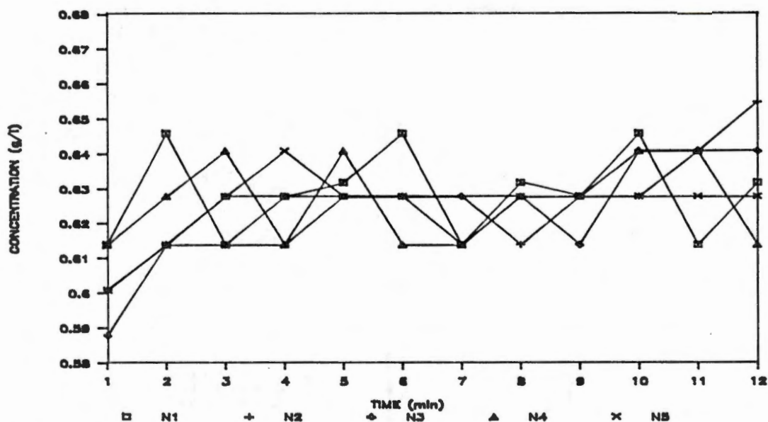
Figure 36. Variation in chemical concentration in the effluent of nozzles 1 through 5 as a function of time. Chemical injection with the Scienco pump was immediately downstream of the system pump. Sampling began at time = 1 min, and system pressure was 171 kPa.
