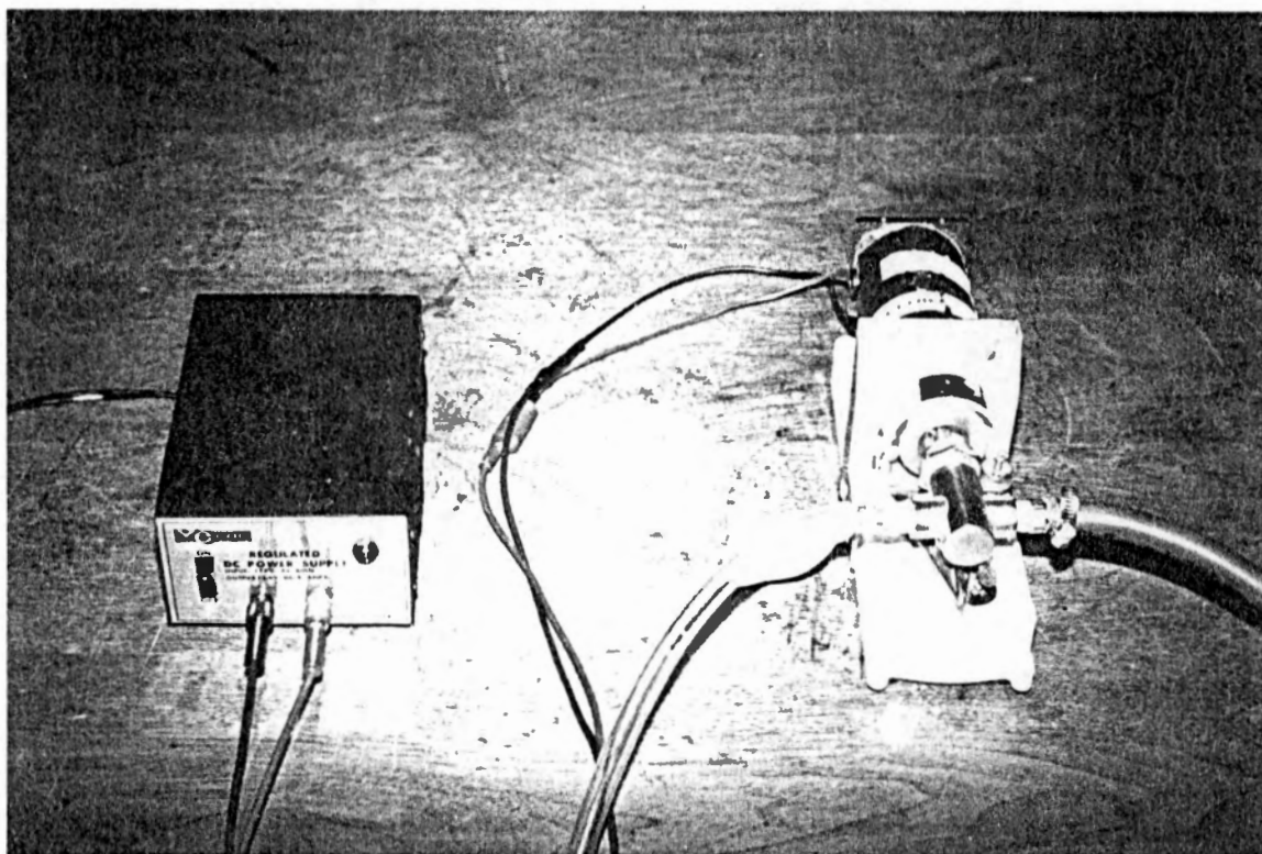
Figure 5. Fluid Metering Inc. piston pump and power supply used for chemical direct injection at both low-pressure and high-pressure sides of the sprayer system pump.
