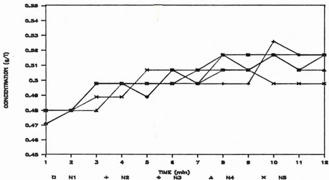
Figure 32. Variation in chemical concentration in the effluent of nozzles 1 through 5 as a function of time. Chemical injection with the Scienco pump was immediately downstream of the system pump. Sampling began at time = 1 min, and system pressure was 275 kPa.
