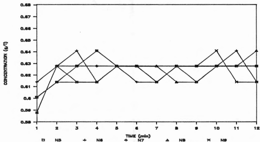
Figure 37. Variation in chemical concentration in the effluent of nozzles 5 through 9 as a function of time. Chemical injection with the Scienco pump was immediately downstream of the system pump. Sampling began at Time = 1 min, and system pressure was 171 kPa.
