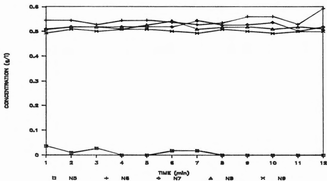
Figure 46. Variation in chemical concentration in the effluent of nozzles 5 through 9 as a function of time. Chemical injection with the Scienco pump was at the individual nozzles. Sampling began at time = 1 min, and system pressure was 275 kPa.
