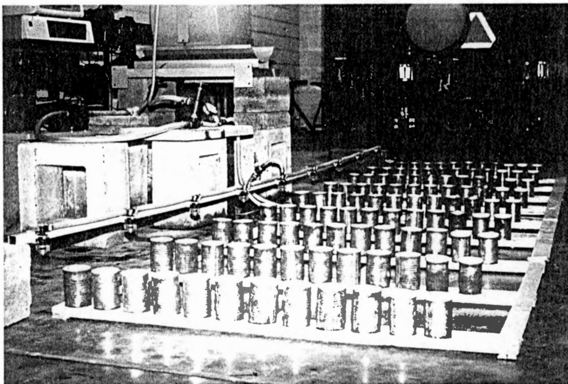
Figure 6. Laboratory setup including the experimental direct injection sprayer and sampling system.
