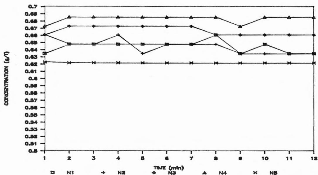
Figure 52. Variation in chemical concentration in the effluent of nozzles 1 through 5 as a function of time. Chemical injection with the Scienco pump was at the individual nozzles, and fluid entrance to the boom was slightly to the side of nozzle 5. Sampling began at time = 1 min, and system pressure was 171 kPa.
