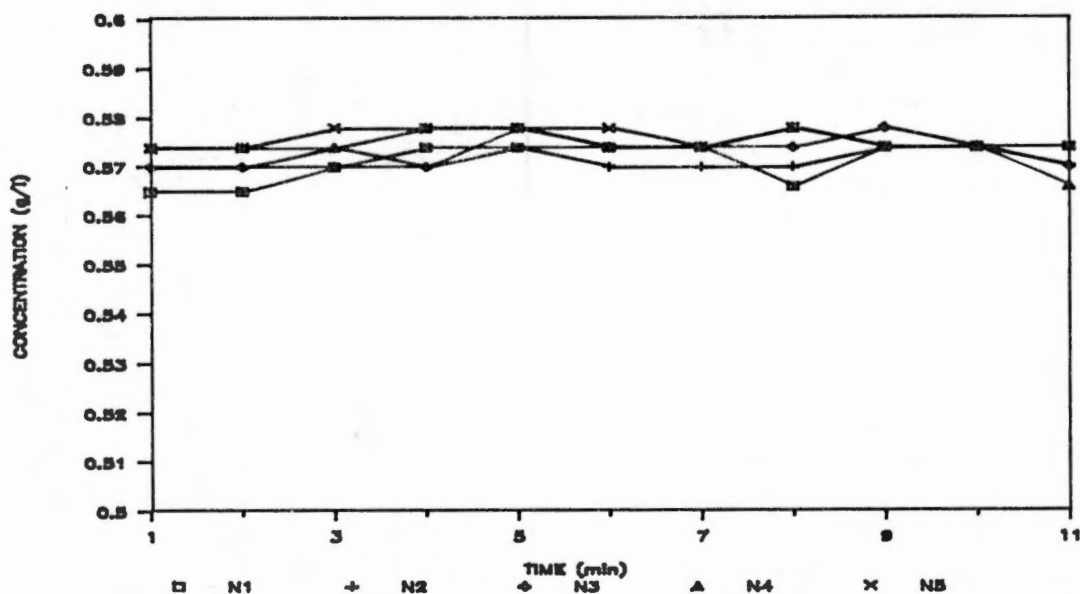
Figure 17. Variation in chemical concentration in the effluent of nozzles 1 through 5 as a function of time. Chemical injection with the peristaltic pump was immediately upstream of the system pump. Sampling began at time = 1 min, and system pressure was 275 kPa.
