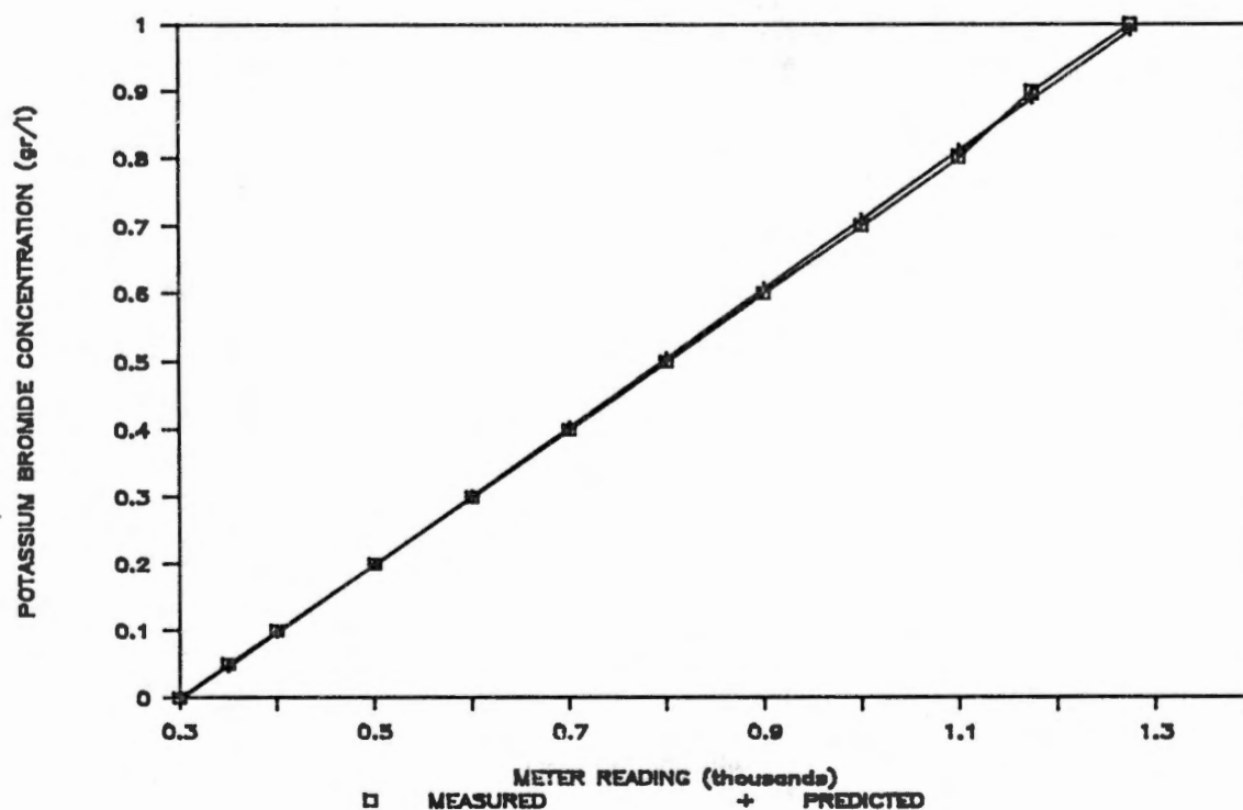
Figure 8. Comparison of actual potassium bromide concentrations and predicted concentrations based upon conductivity meter readings. Comparison is typical of all calibrations performed.
