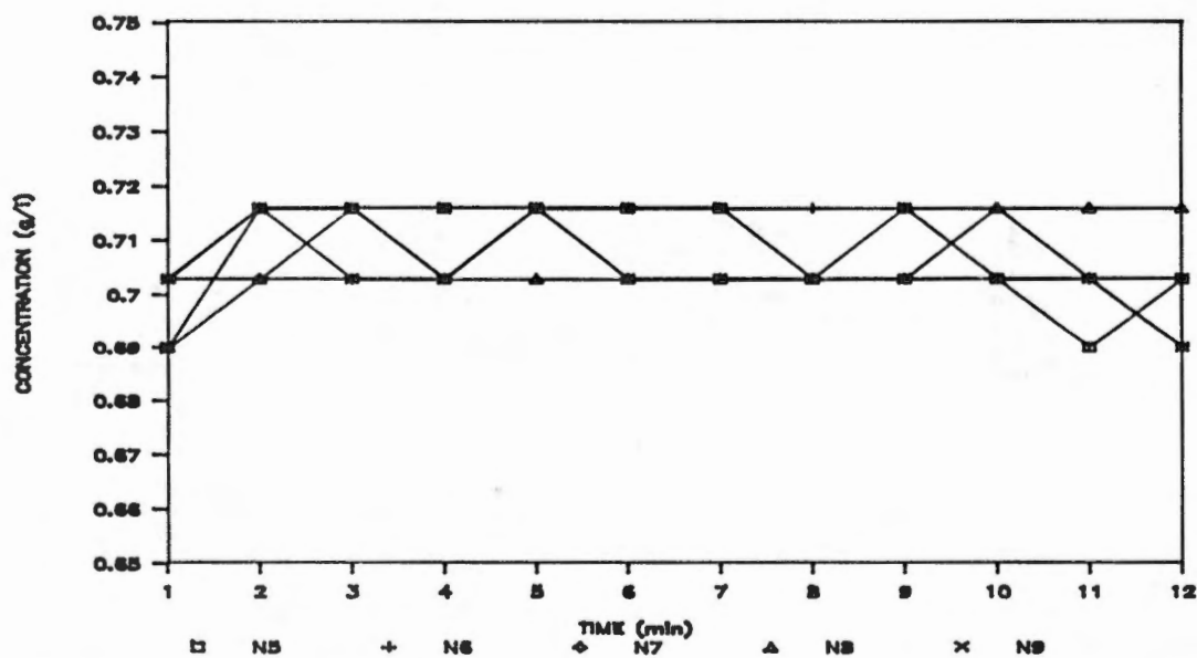
Figure 66. Variation in chemical concentration in the effluent of nozzles 5 through 9 as a function of time with a conventional application system at a pressure of 171 kPa. Sampling began at 1 min.
