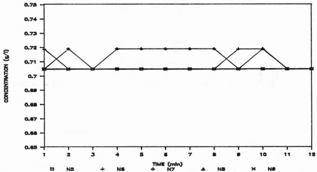
Figure 64. Variation in chemical concentration in the effluent of nozzles 5 through 9 as a function of time with a conventional application system at a pressure of 275 kPa. Sampling began at 1 min.
