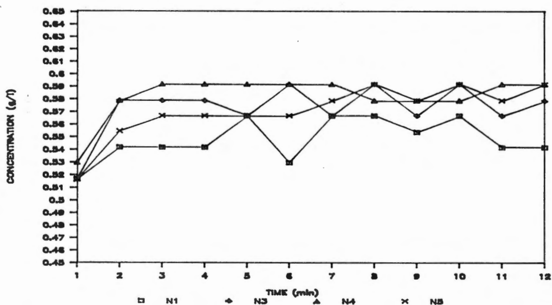
Figure 61. Variation in chemical concentration in the effluent of nozzles 1 through 5 as a function of time. Chemical injection with the Scienco pump was at the individual nozzles for an eight-nozzle boom. Sampling began at time = 1 min, and system pressure was 275 kPa.
