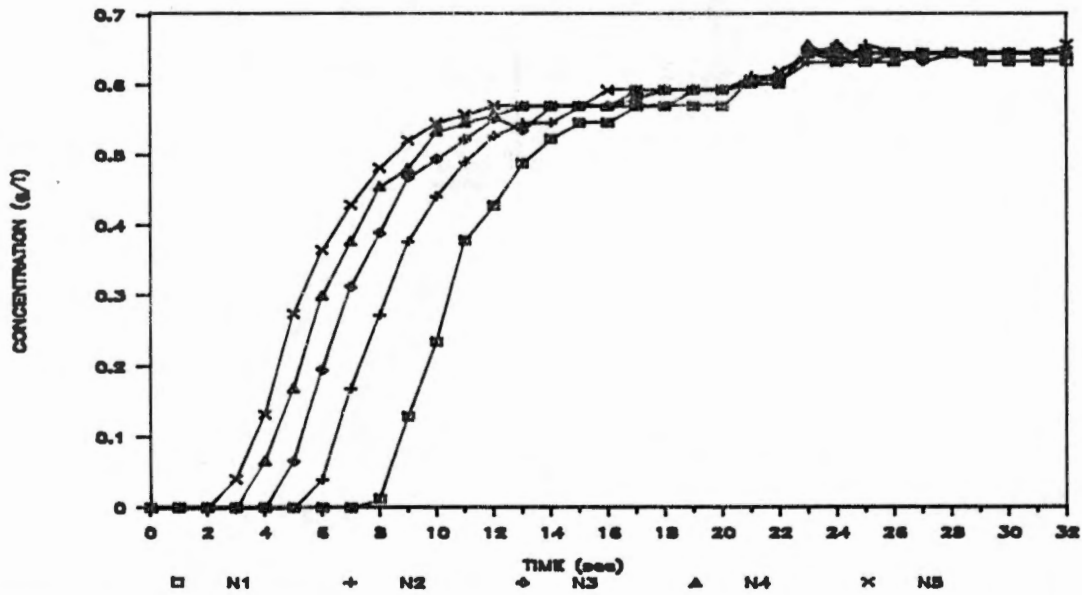
Figure 15. Variation in chemical concentration in the effluent of nozzles 1 through 5 as a function of time. Chemical injection with the FMI pump was immediately upstream of the system pump. Injection began at time = 0, and system pressure was 275 kPa.
