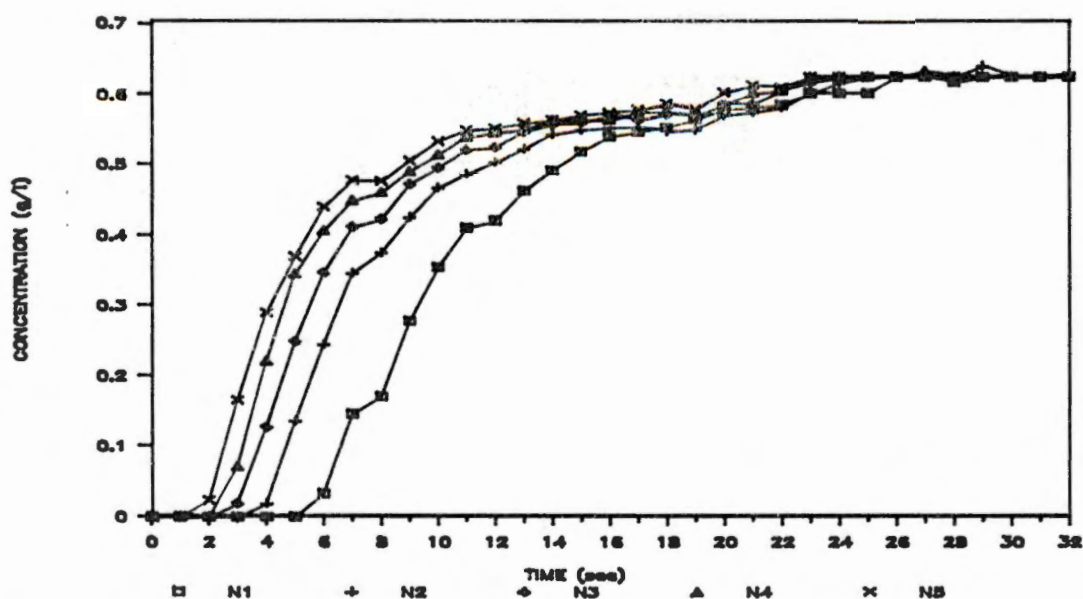
Figure 11. Variation in chemical concentration in the effluent of nozzles 1 through 5 as a function of time. Chemical injection with the peristaltic pump was immediately upstream of the system pump. Injection began at time = 0, and system pressure was 275 kPa.
