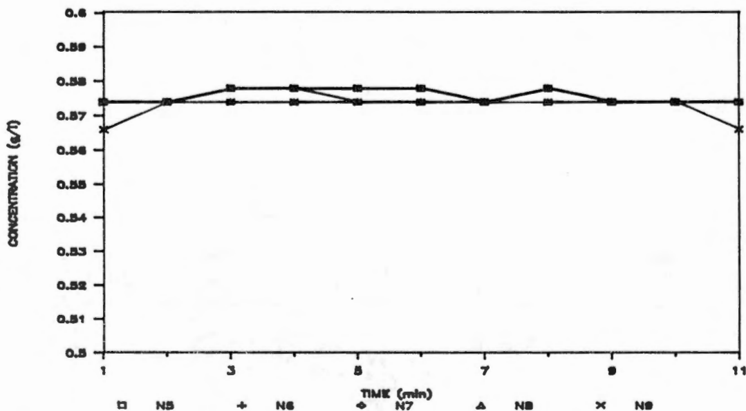
Figure 18. Variation in chemical concentration in the effluent of nozzles 5 through 9 as a function of time. Chemical injection with the peristaltic pump was immediately upstream of the system pump. Sampling began at time = 1 min, and system pressure was 275 kPa.
