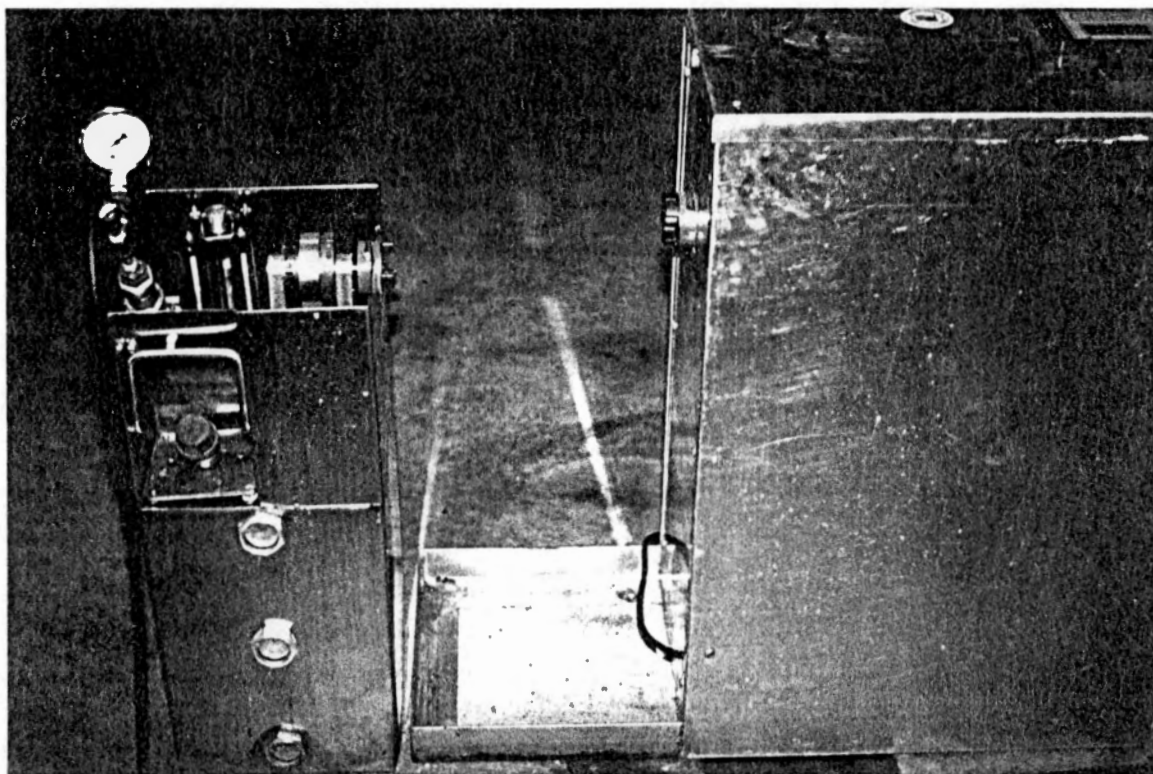
Figure 4. Scienco Inc. piston pump and calibration stand used for direct chemical injection at both low-pressure and high-pressure sides of the sprayer system pump.
