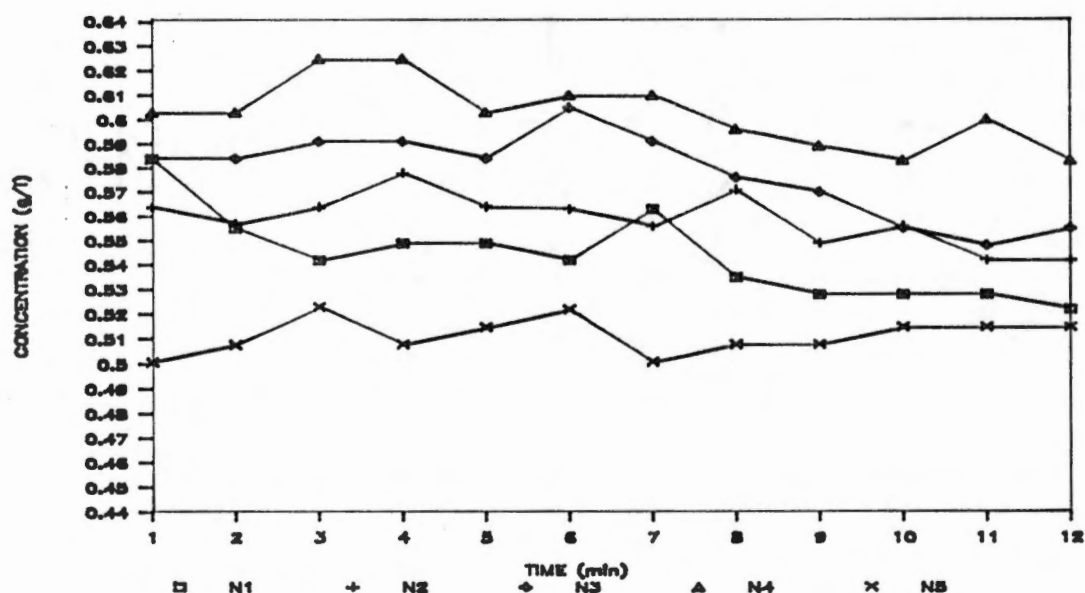
Figure 48. Variation in chemical concentration in the effluent of nozzles 1 through 5 as a function of time. Chemical injection with the Scienco pump was at the individual nozzles, and fluid entrance to the boom was slightly to the side of nozzle 5. Sampling began at time = 1 min, and system pressure was 275 kPa.
