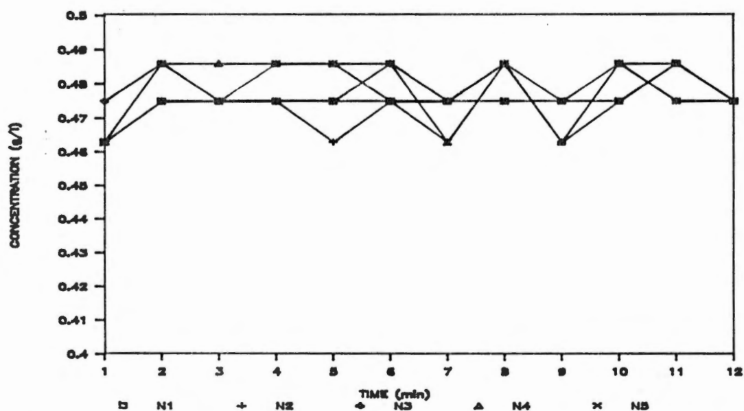
Figure 38. Variation in chemical concentration in the effluent of nozzles 1 through 5 as a function of time. Chemical injection with the FMI pump was immediately downstream of the system pump. Sampling began at time = 1 min, and system pressure was 378 kPa.
