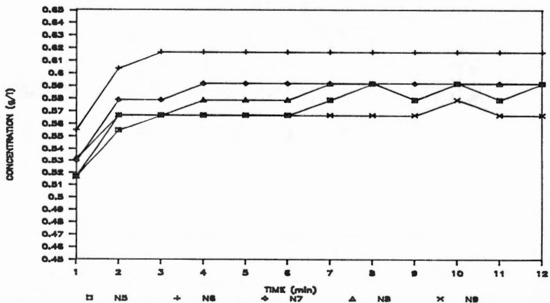
Figure 62. Variation in chemical concentration in the effluent of nozzles 5 through 9 as a function of time. Chemical injection with the Scienco pump was at the individual nozzles for an eight-nozzle boom. Sampling began at time = 1 min, and system pressure was 275 kPa.
