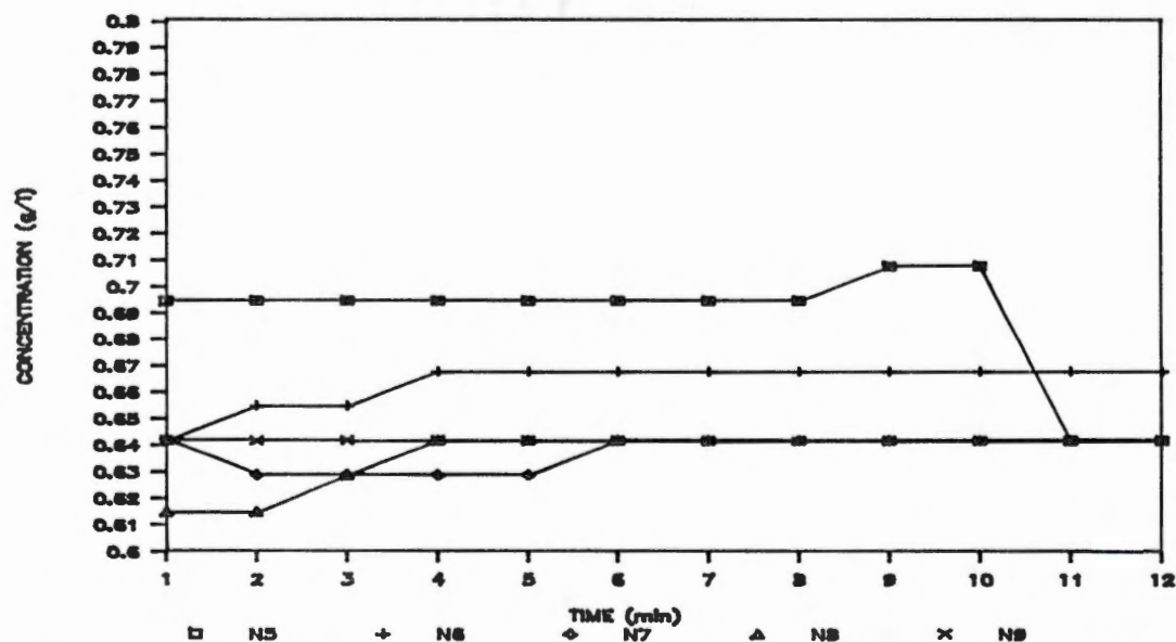
Figure 55. Variation in chemical concentration in the effluent of nozzles 5 through 9 as a function of time. Chemical injection with the FMI pump was at the individual nozzles, and fluid entrance to the boom was slightly to the side of nozzle 5. Sampling began at time = 1 min, and system pressure was 171 kPa.
