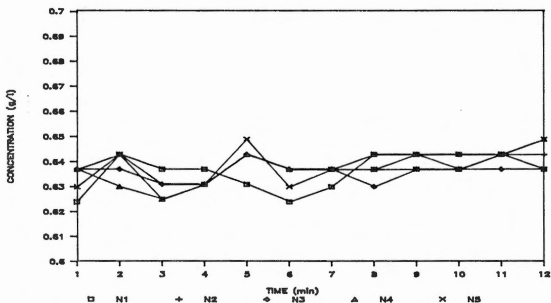
Figure 30. Variation in chemical concentration in the effluent of nozzles 1 through 5 as a function of time. Chemical injection with the FMI pump was immediately downstream of the system pump. Sampling began at time = 1 min, and system pressure was 275 kPa.
