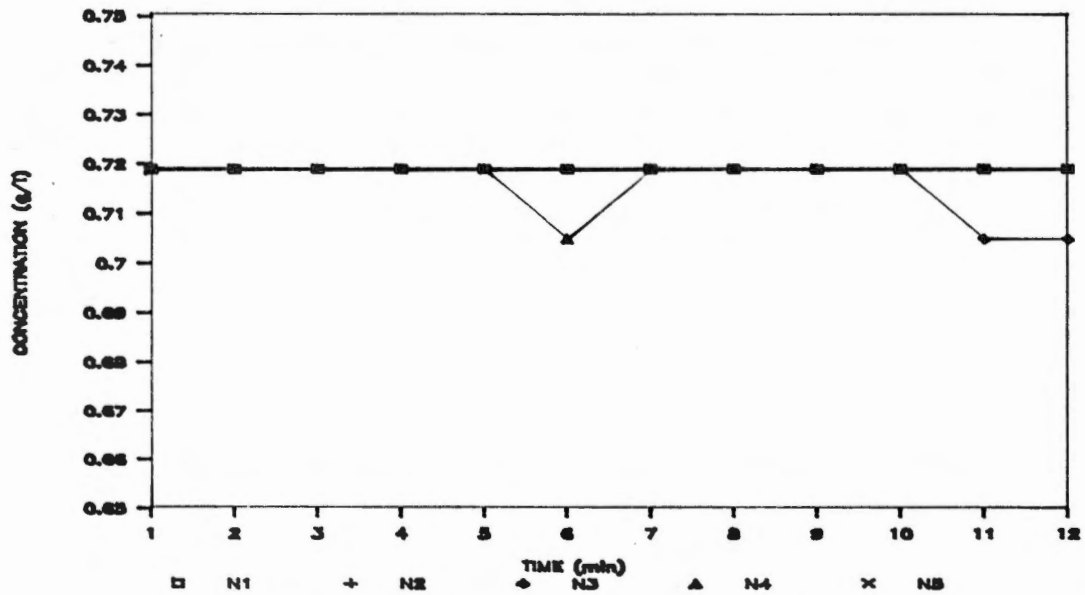
Figure 67. Variation in chemical concentration in the effluent of nozzles 1 through 5 as a function of time with a conventional application system at a pressure of 378 kPa. Sampling began at 1 min.
