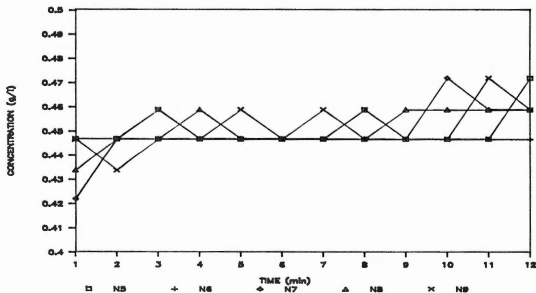
Figure 41. Variation in chemical concentration in the effluent of nozzles 5 through 9 as a function of time. Chemical injection with the Scienco pump was immediately downstream of the system pump. Sampling began at time = 1 min, and system pressure was 378 kPa.
