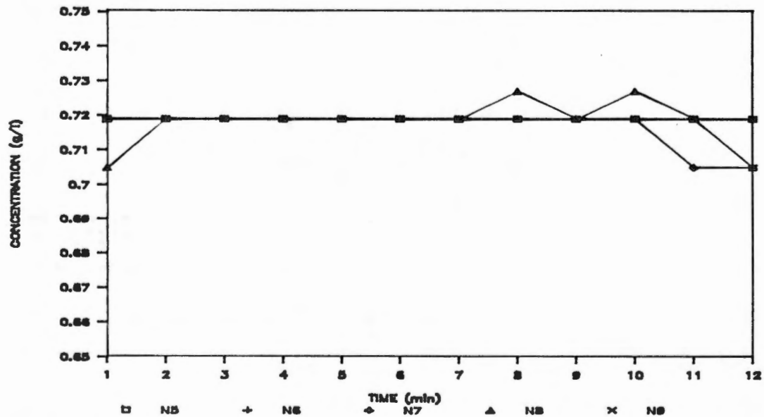
Figure 68. Variation in chemical concentration in the effluent of nozzles 5 through 9 as a function of time with a conventional application system at a pressure of 378 kPa. Sampling began at 1 min.
