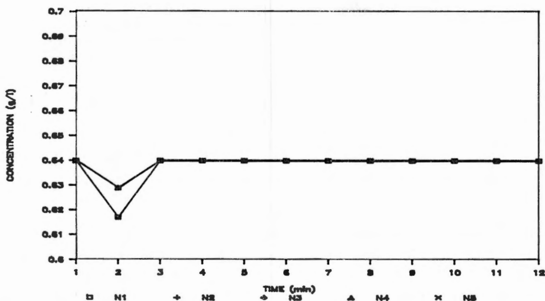
Figure 21. Variation in chemical concentration in the effluent of nozzles 1 through 5 as a function of time. Chemical injection with the FMI pump was immediately upstream of the system pump. Sampling began at time = 1 min, and system pressure was 275 kPa.
