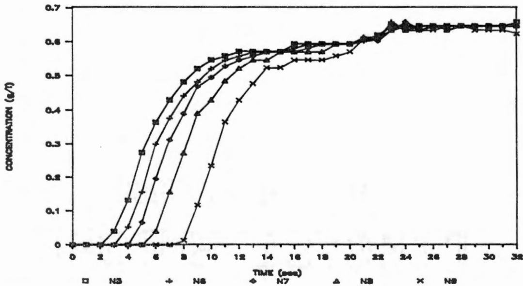
Figure 16. Variation in chemical concentration in the effluent of nozzles 5 through 9 as a function of time. Chemical injection with the FMI pump was immediately upstream of the system pump. Injection began at time = 0, and system pressure was 275 kPa.
