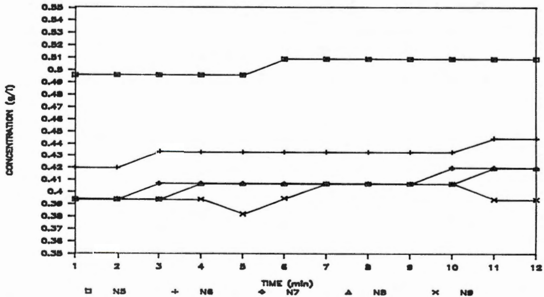
Figure 57. Variation in chemical concentration in the effluent of nozzles 5 through 9 as a function of time. Chemical injection with the Scienco pump was at the individual nozzles, and fluid entrance to the boom was slightly to the side of nozzle 5. Sampling began at time = 1 min, and system pressure was 378 kPa.
