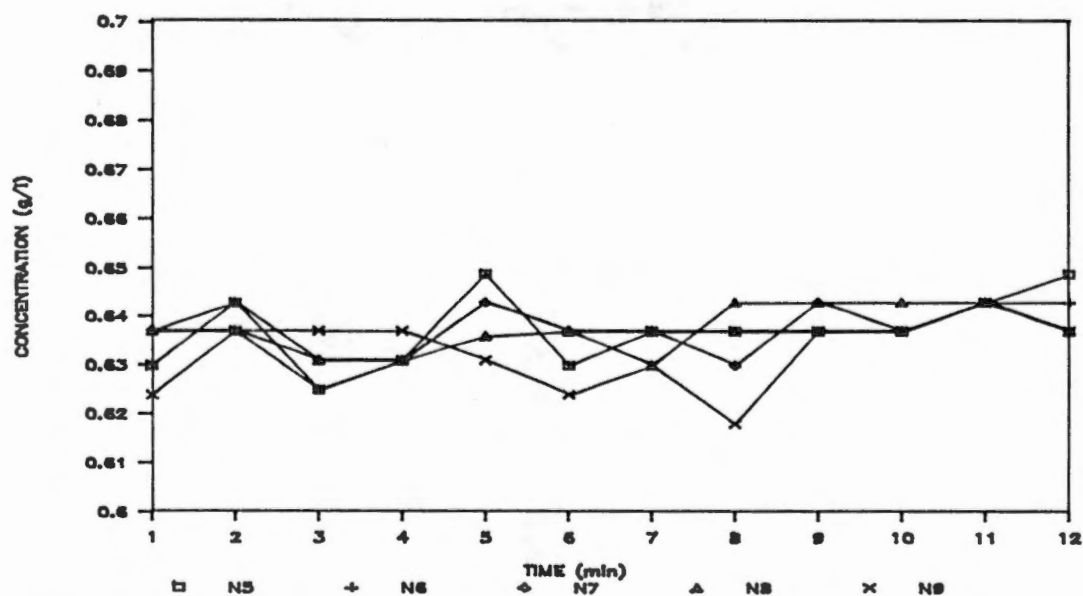
Figure 31. Variation in chemical concentration in the effluent of nozzles 5 through 9 as a function of time. Chemical injection with the FMI pump was immediately downstream of the system pump. Sampling began at time = 1 min, and system pressure was 275 kPa.
