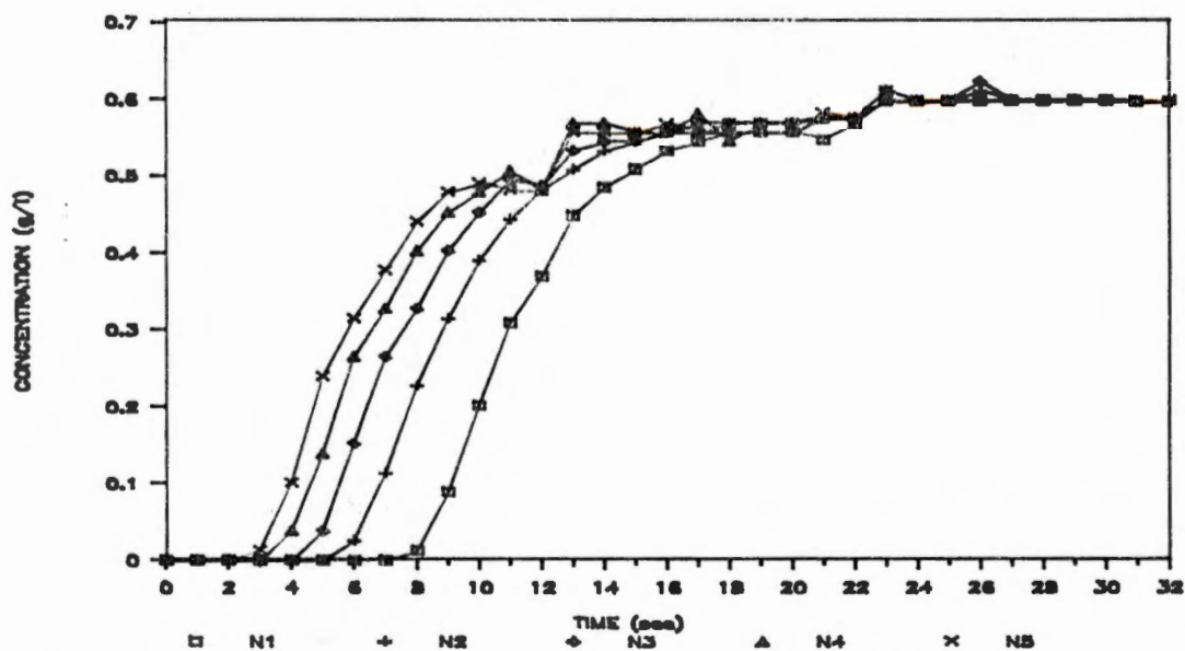
Figure 13. Variation in chemical concentration in the effluent of nozzles 1 through 5 as a function of time. Chemical injection with the Scienco pump was immediately upstream of the system pump. Injection began at time = 0, and system pressure was 275 kPa.
