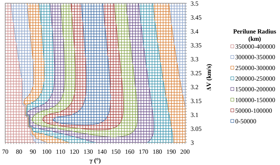
Figure A4. Radius of Perilune for Varying \Delta V and \gamma , Point-mass Gravitational Model, A = 400 km.
