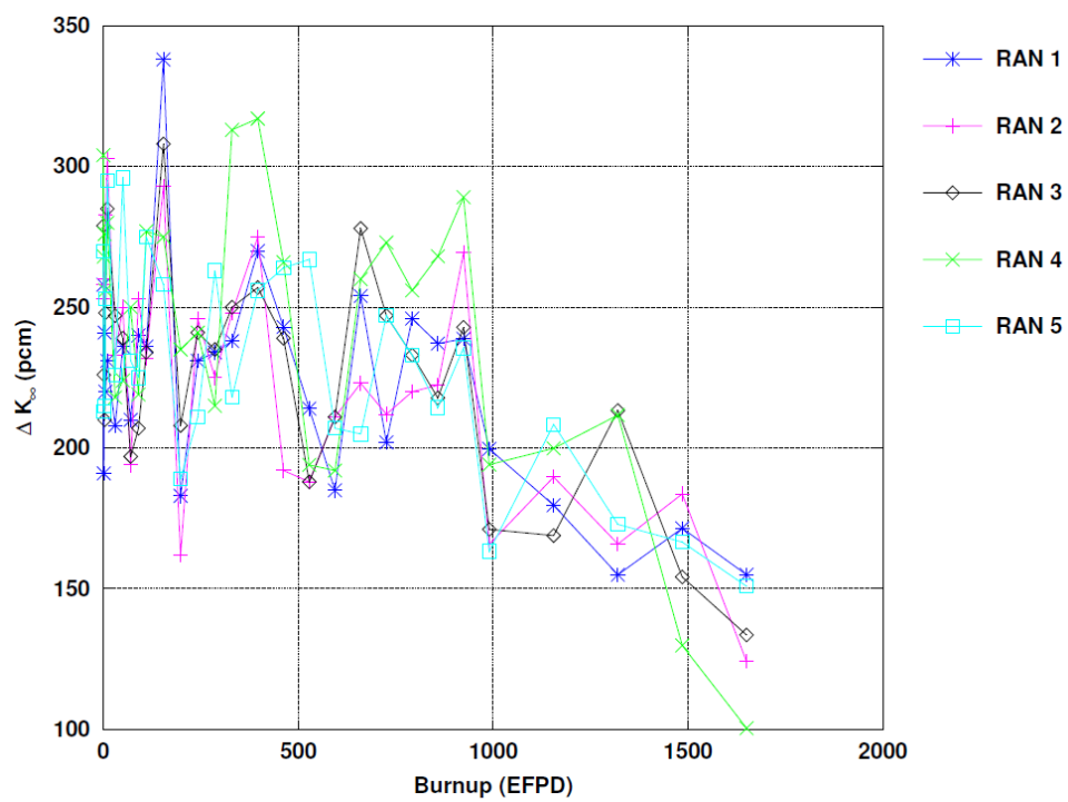
Figure 2-4 K-infinity Difference between Regular Lattice and Random Dispersion
