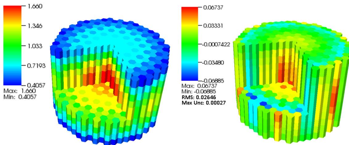
Figure 3-10 3-D Full Core with Control Blades Inserted NESTLE Relative Power Distributions (Left), SERPENT 2 minus NESTLE Node Averaged Power Distribution Differences (Right)
