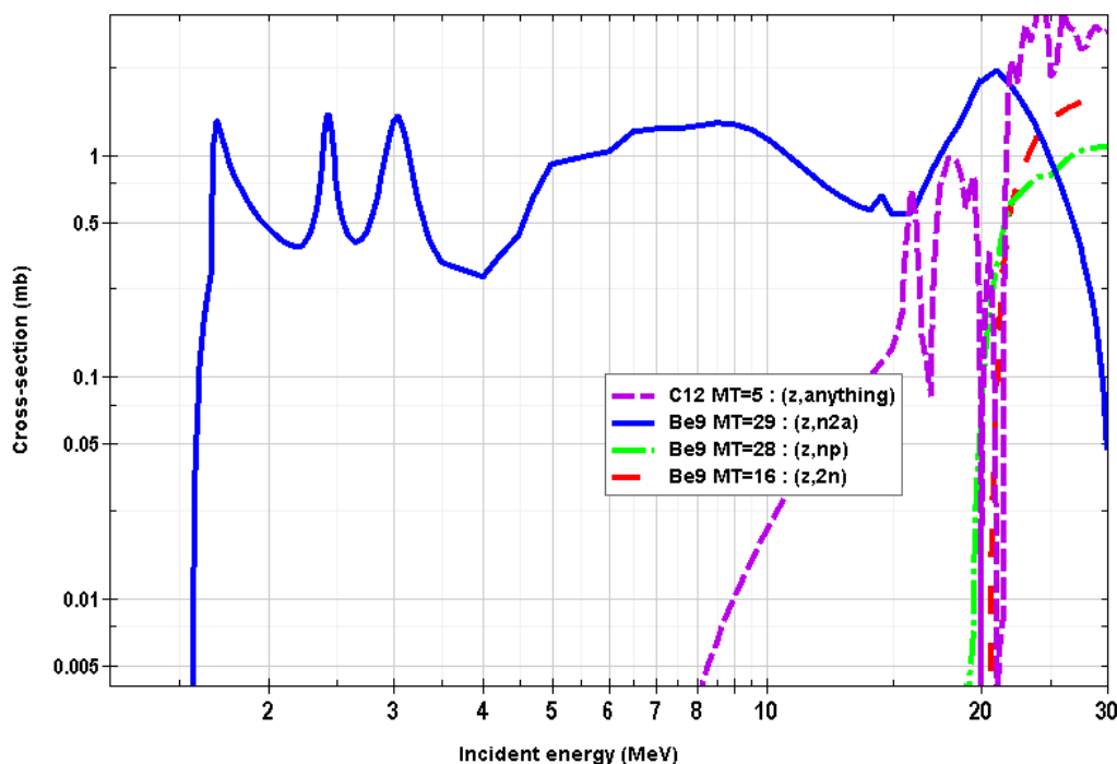
Figure 2-9 Gamma Cross Sections of Interest for AHTR [31]
