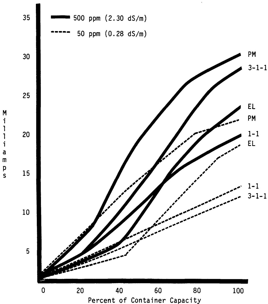
Figure 2. The influence of soluble salt treatments (50 and 500 ppm %N) in four media and six moisture levels on milliamperage readings averaged across container types.
