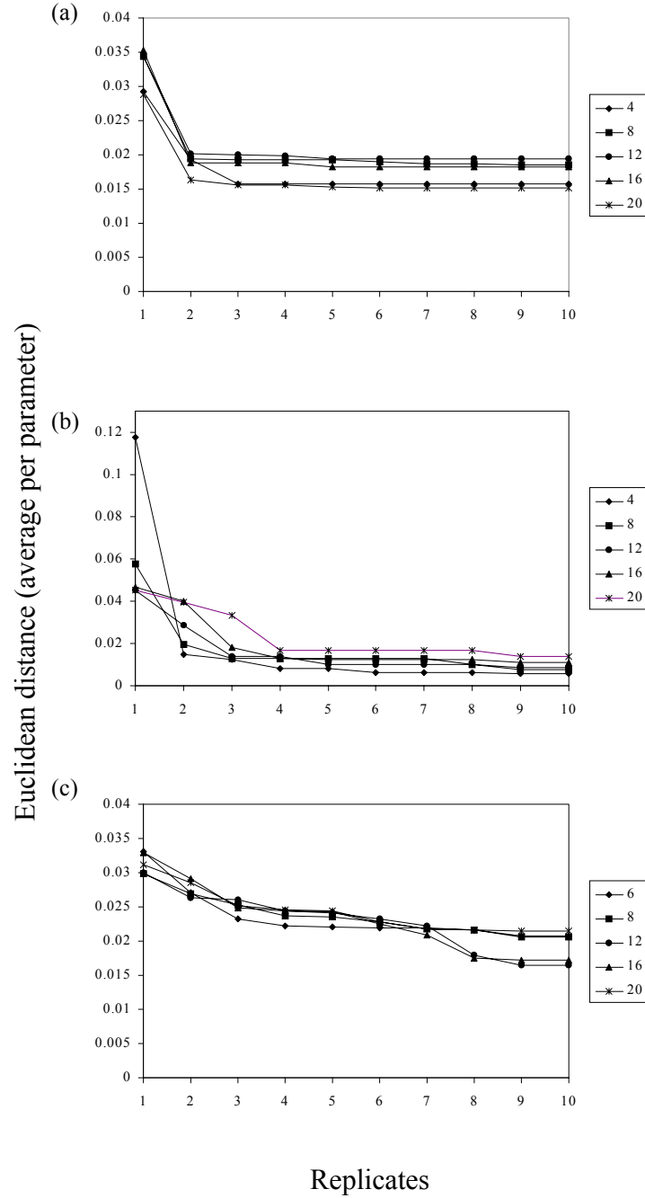
Figure 4.5: Euclidean distance of estimated Markov set-chains from true set-chain parameters for a system with (a) two states, (b) three states, (c) four states. Note that the scale for the three-state set-chain is different from the others. Adding replicates beyond four does not improve the estimate. For all system sizes, the average distance with ten replicates is near 0.02.
