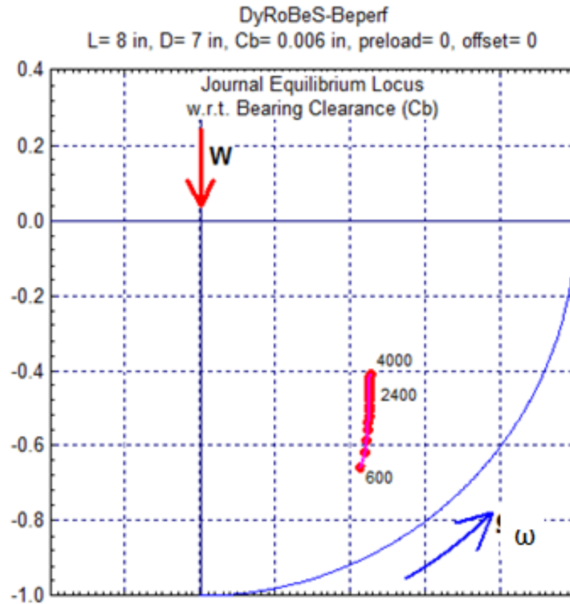
Figure 21 – Pressure Dam Bearing Journal Equilibrium Locus
