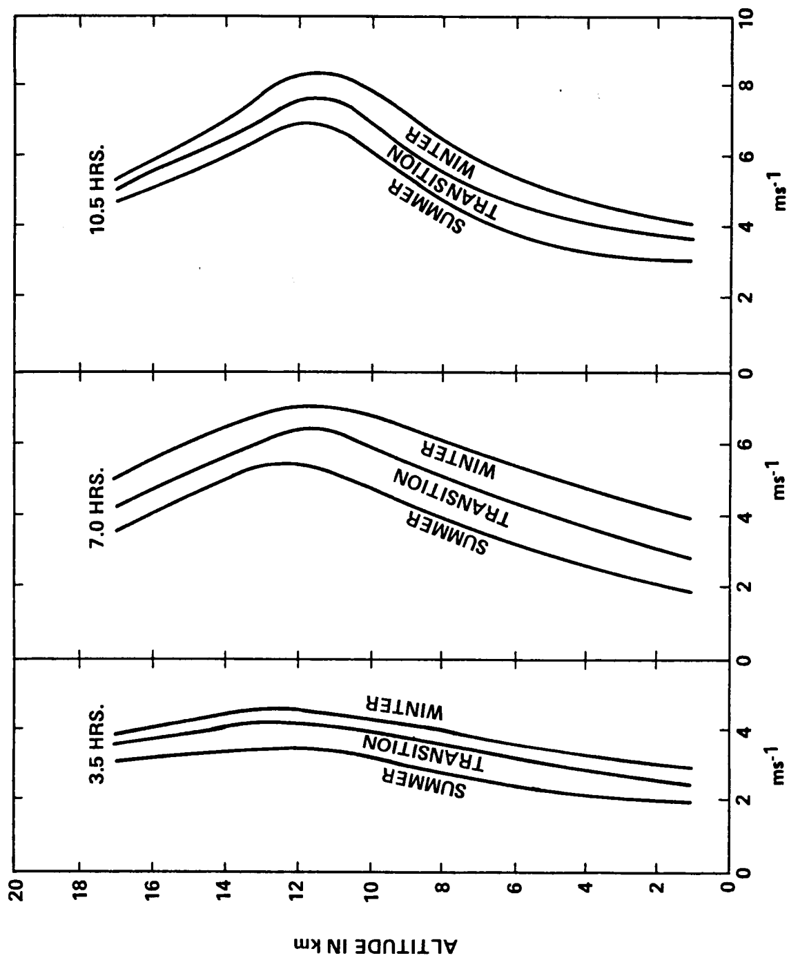
Figure 3.1. Standard deviation of the u component from paired profile differences for given seasons and time intervals.
