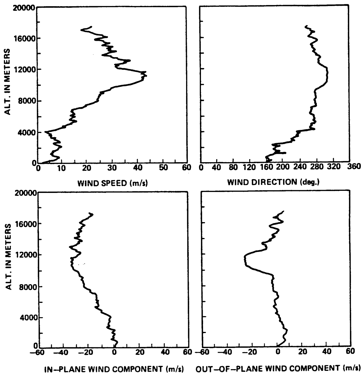
Figure A.39. STS-11 prelaunch/launch jimsphere profiles of wind speed, wind direction, in-plane and out-of-plane wind components, 0930 GMT February 3, 1984.
