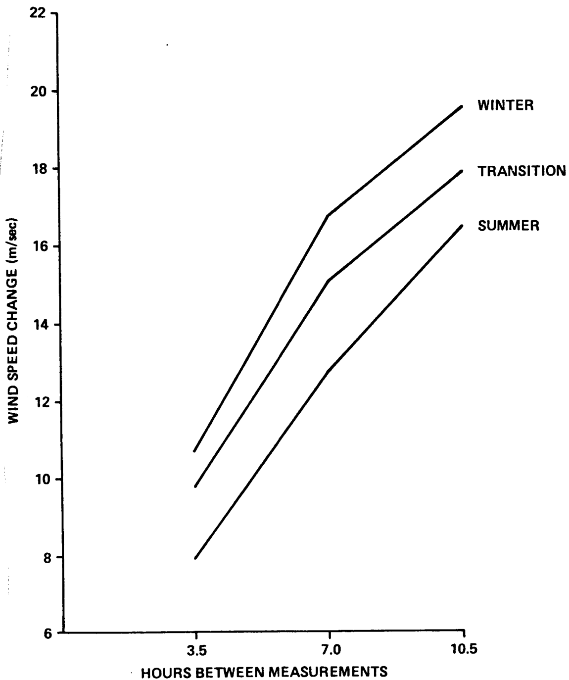
Figure 3.5. One percent risk of u wind component change at 12 km altitude for Kennedy Space Center, Florida.
