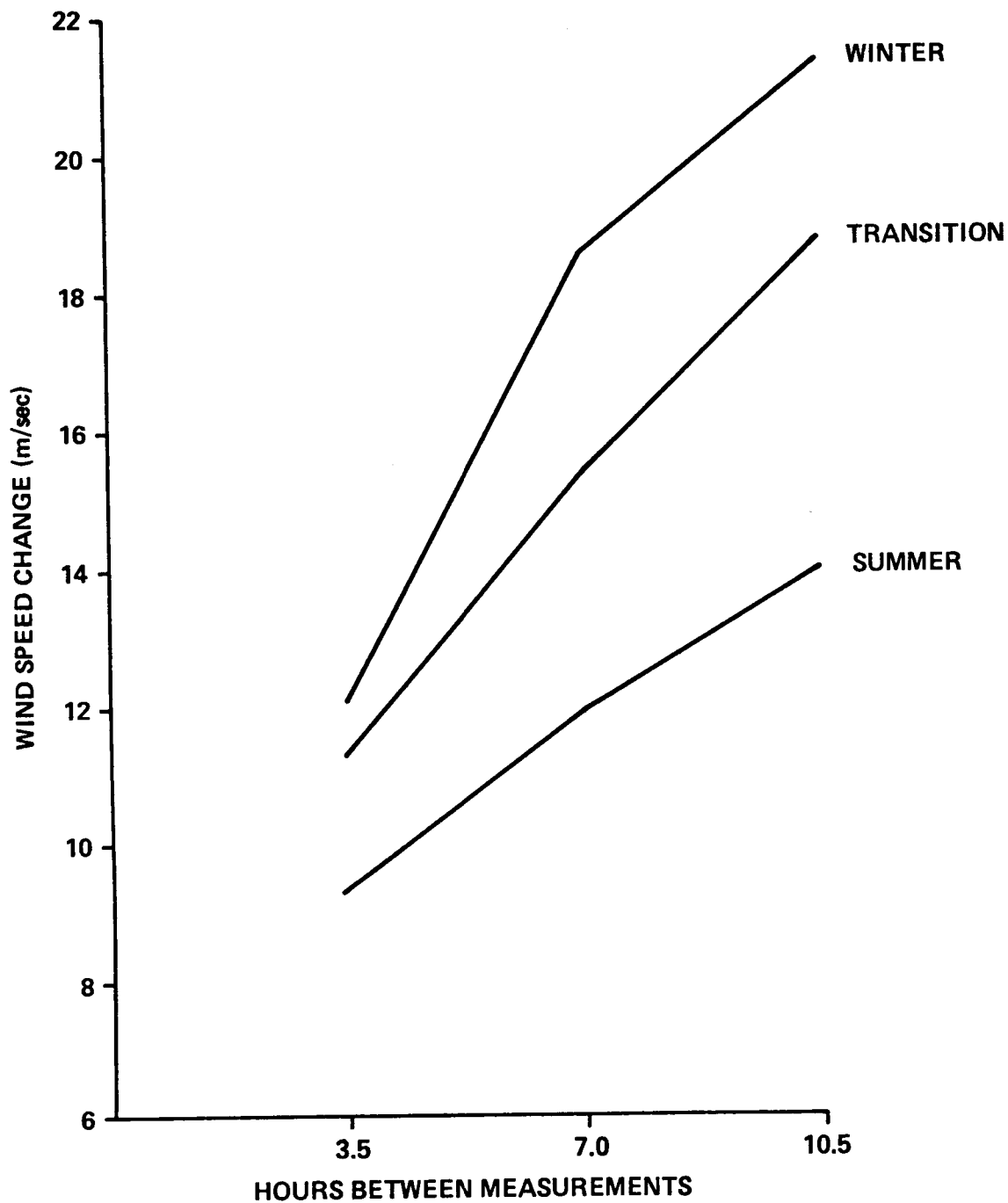
Figure 3.6. One percent risk of v wind component change at 12 km altitude for Kennedy Space Center, Florida.
