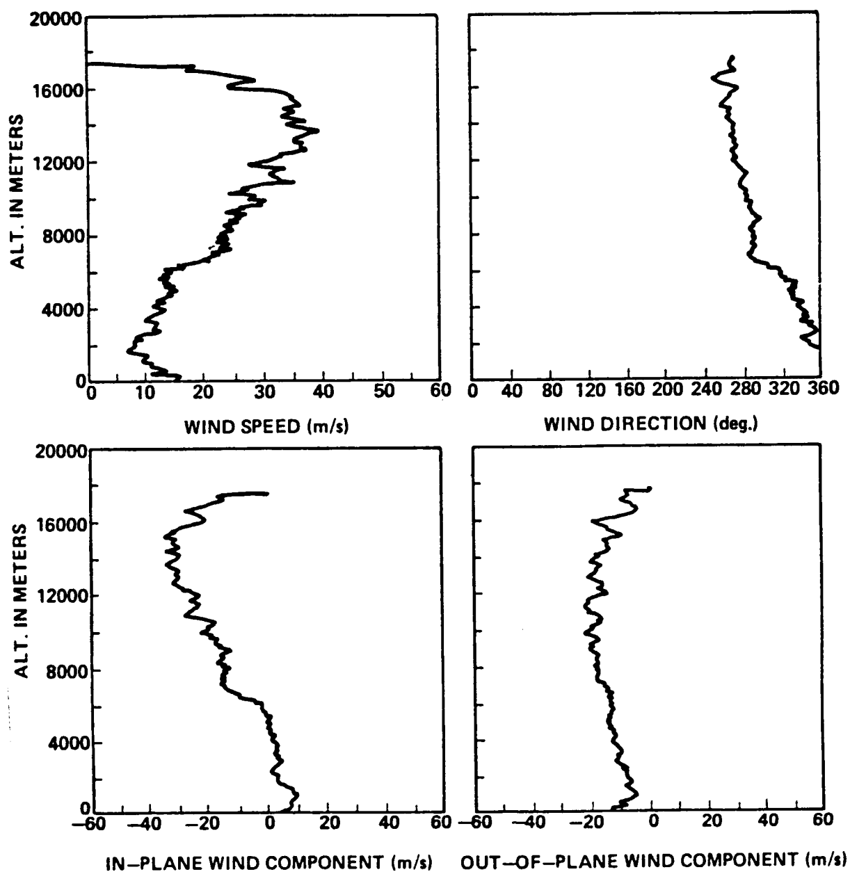
Figure A.3. STS-2 prelaunch/launch jimsphere profiles of wind speed, wind direction, in-plane and out-of-plane wind components, 1130 GMT November 12, 1981.
