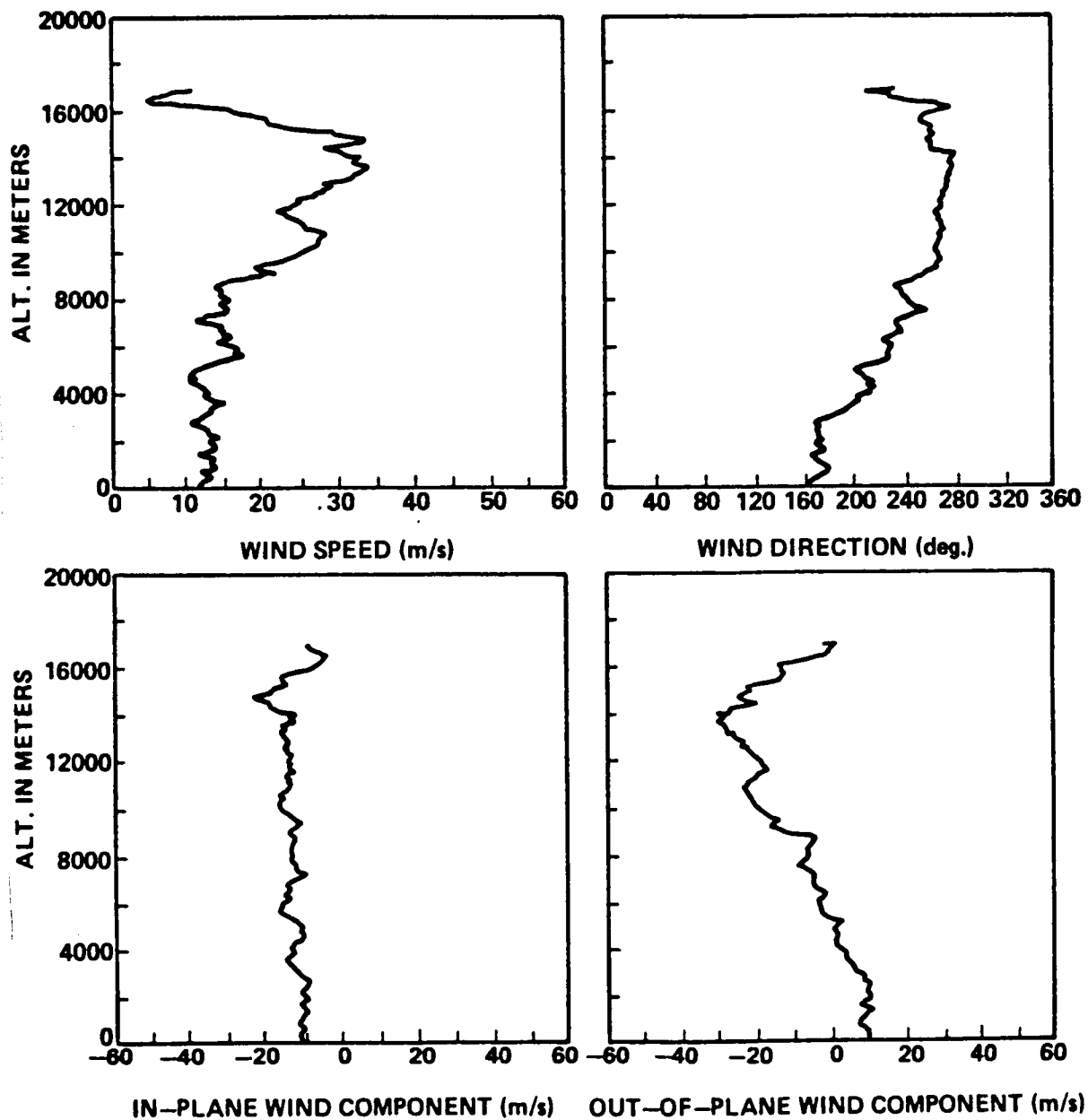
Figure A.33. STS-9 prelaunch/launch jimsphere profiles of wind speed, wind direction, in-plane and out-of-plane wind components, 0300 GMT November 28, 1983.
