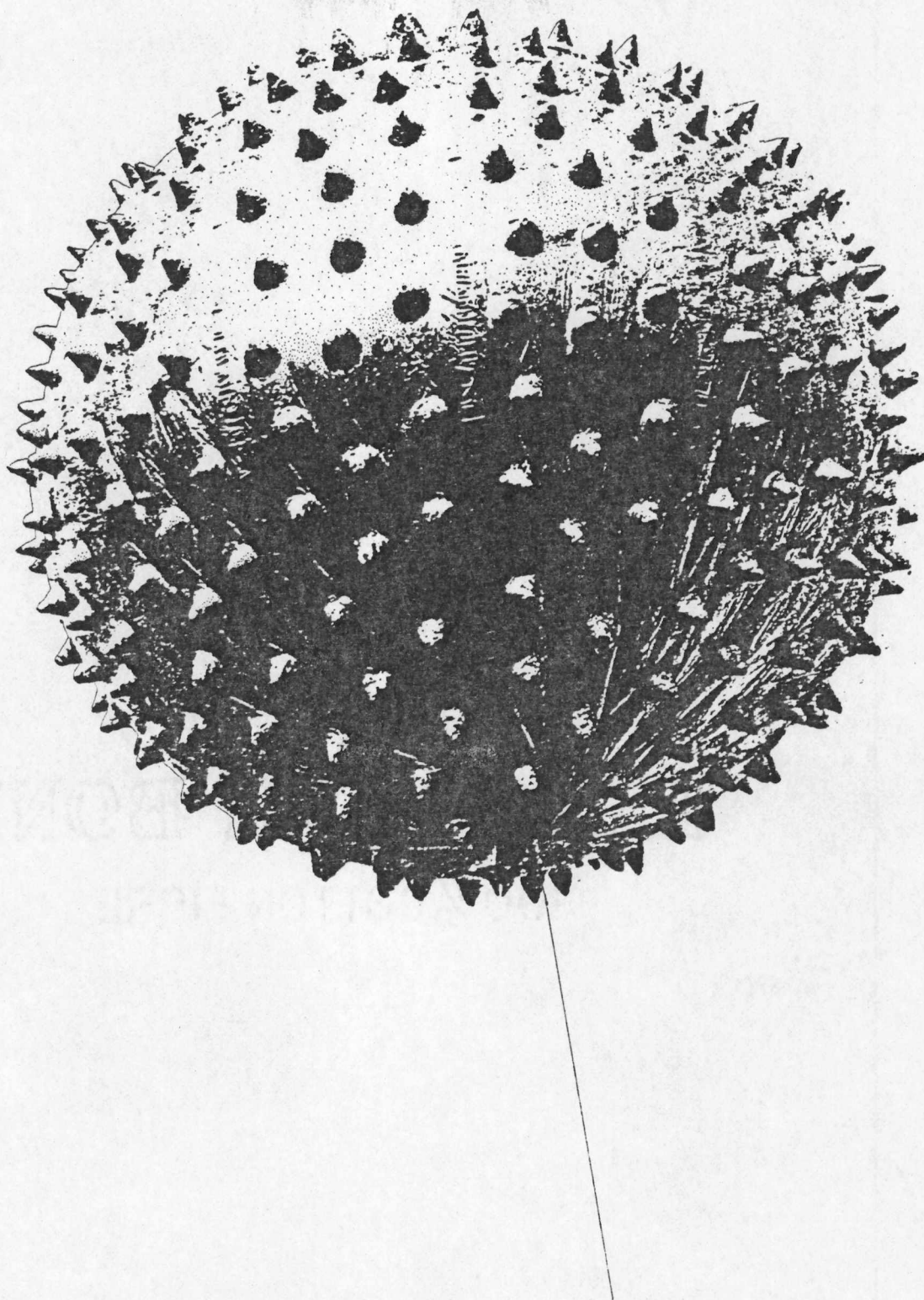
Figure 1.3. Jimsphere sensor.
