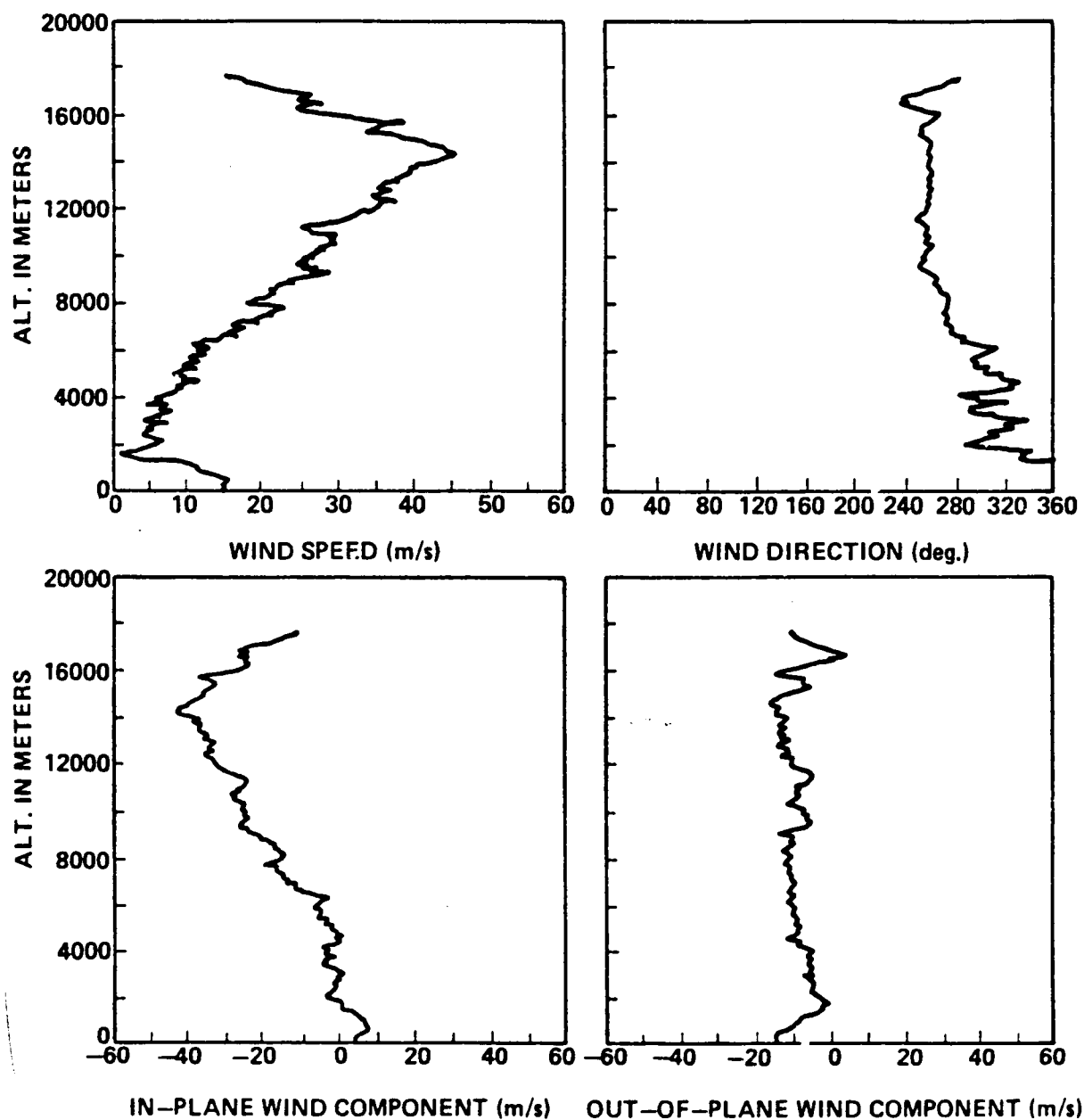
Figure A.1. STS-2 prelaunch/launch jimsphere profiles of wind speed, wind direction, in-plane and out-of-plane wind components, 0430 GMT November 12, 1981.
