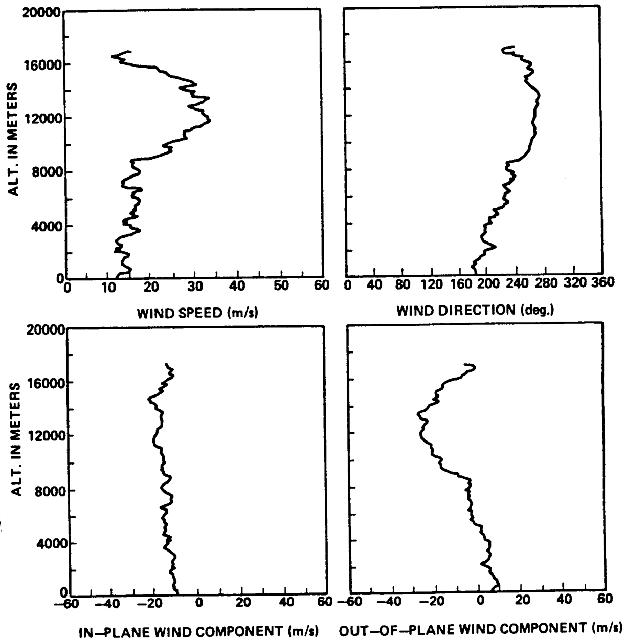
Figure A.34. STS-9 prelaunch/launch jimsphere profiles of wind speed, wind direction, in-plane and out-of-plane wind components, 0845 GMT November 28, 1983.
