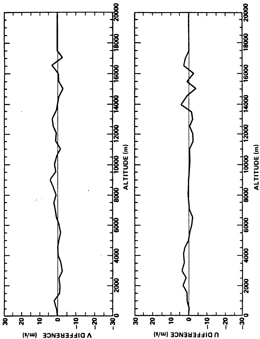
Figure A.54. Jimsphere-measured wind component changes ( u, v ) observed at Kennedy Space Center, Florida, between 1130 GMT and 1515 GMT June 27, 1982, during NASA's STS-4 countdown.
