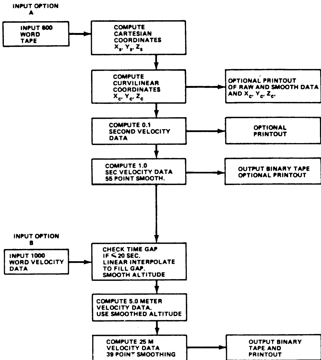
Figure 2.1. Flowchart of the FPS-16/jimsphere master reduction process.
