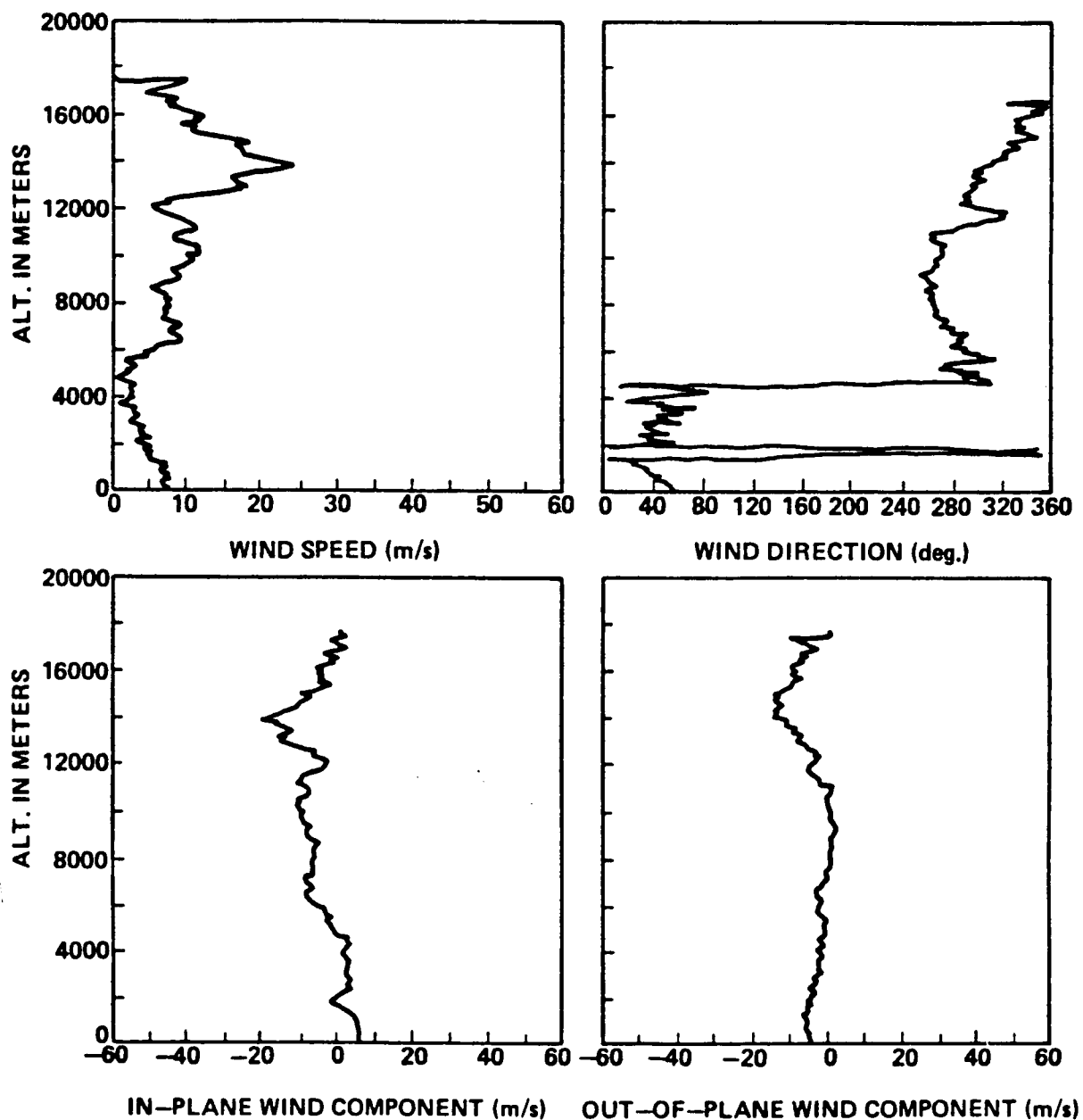
Figure A.25. STS-7 prelaunch/launch jimsphere profiles of wind speed, wind direction, in-plane and out-of-plane wind components, 2133 GMT June 17, 1983.
