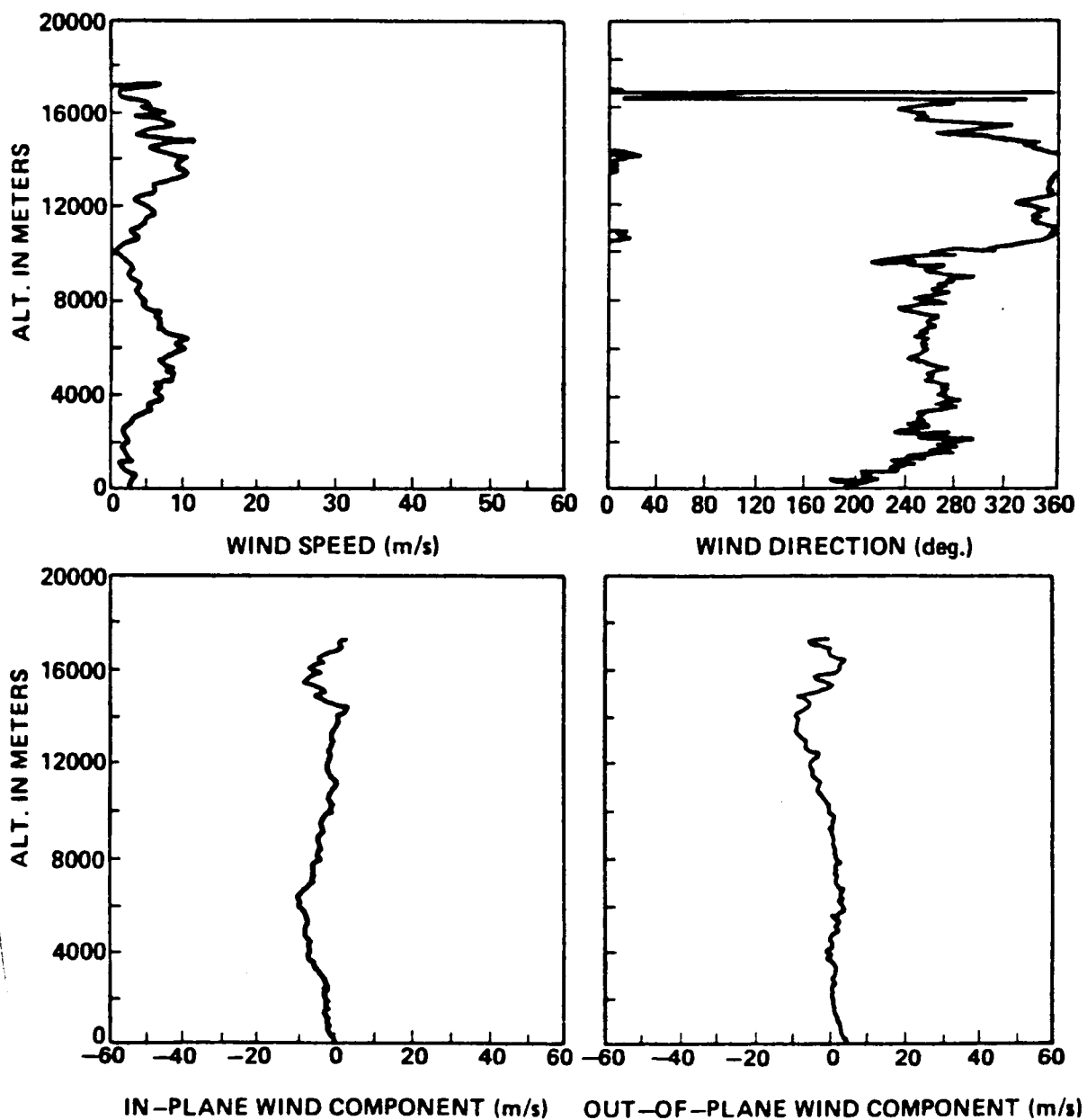
Figure A.14. STS-4 prelaunch/launch jimsphere profiles of wind speed, wind direction, in-plane and out-of-plane wind components, 1515 GMT June 27, 1982.
