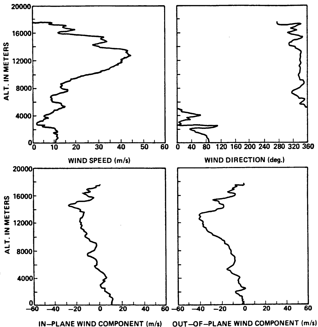
Figure A.19. STS-5 prelaunch/launch jimsphere profiles of wind speed, wind direction, in-plane and out-of-plane wind components, 1235 GMT November 11, 1982.
