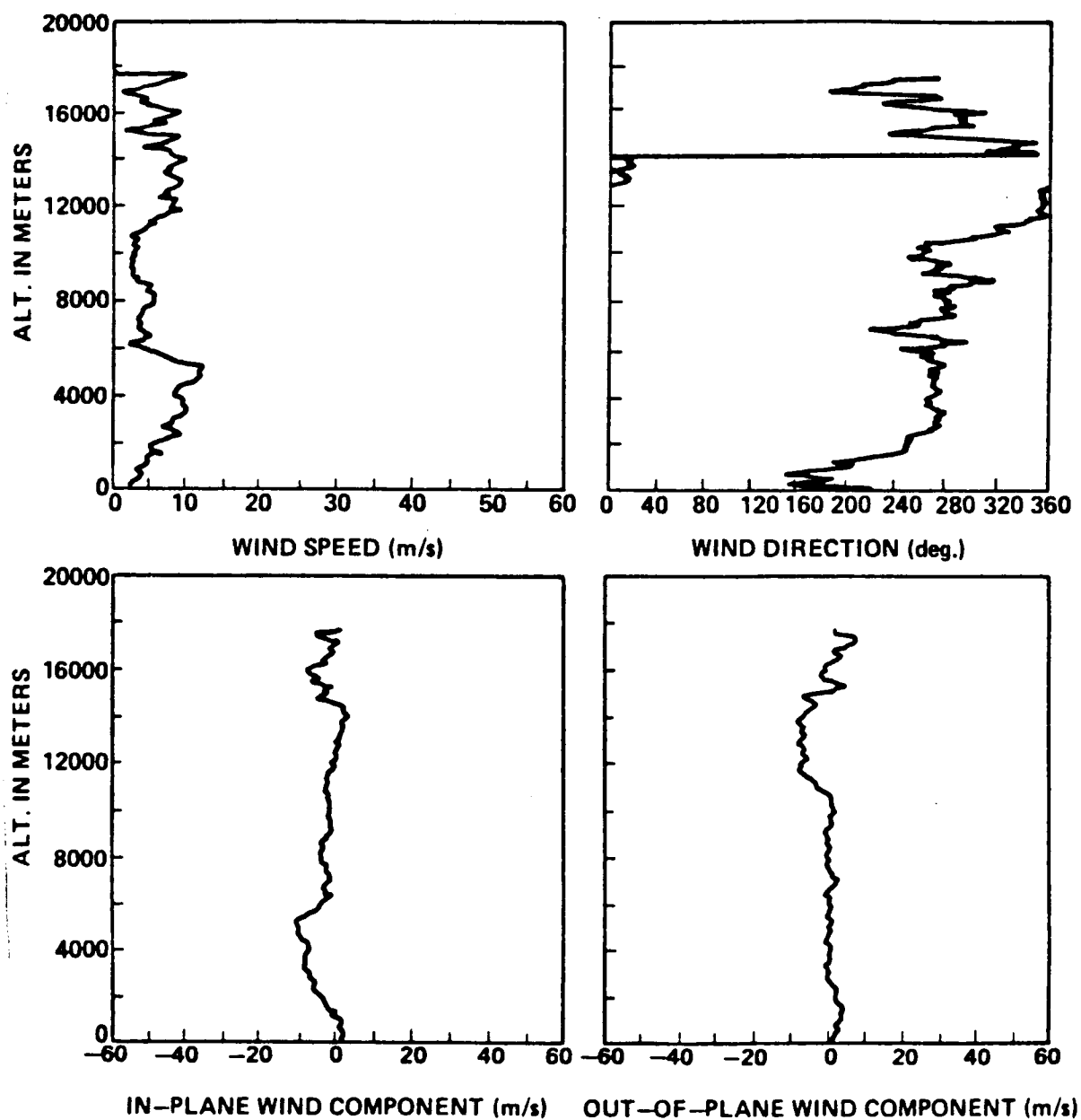
Figure A.11. STS-4 prelaunch/launch jimsphere profiles of wind speed, wind direction, in-plane and out-of-plane wind components, 0330 GMT June 27, 1982.
