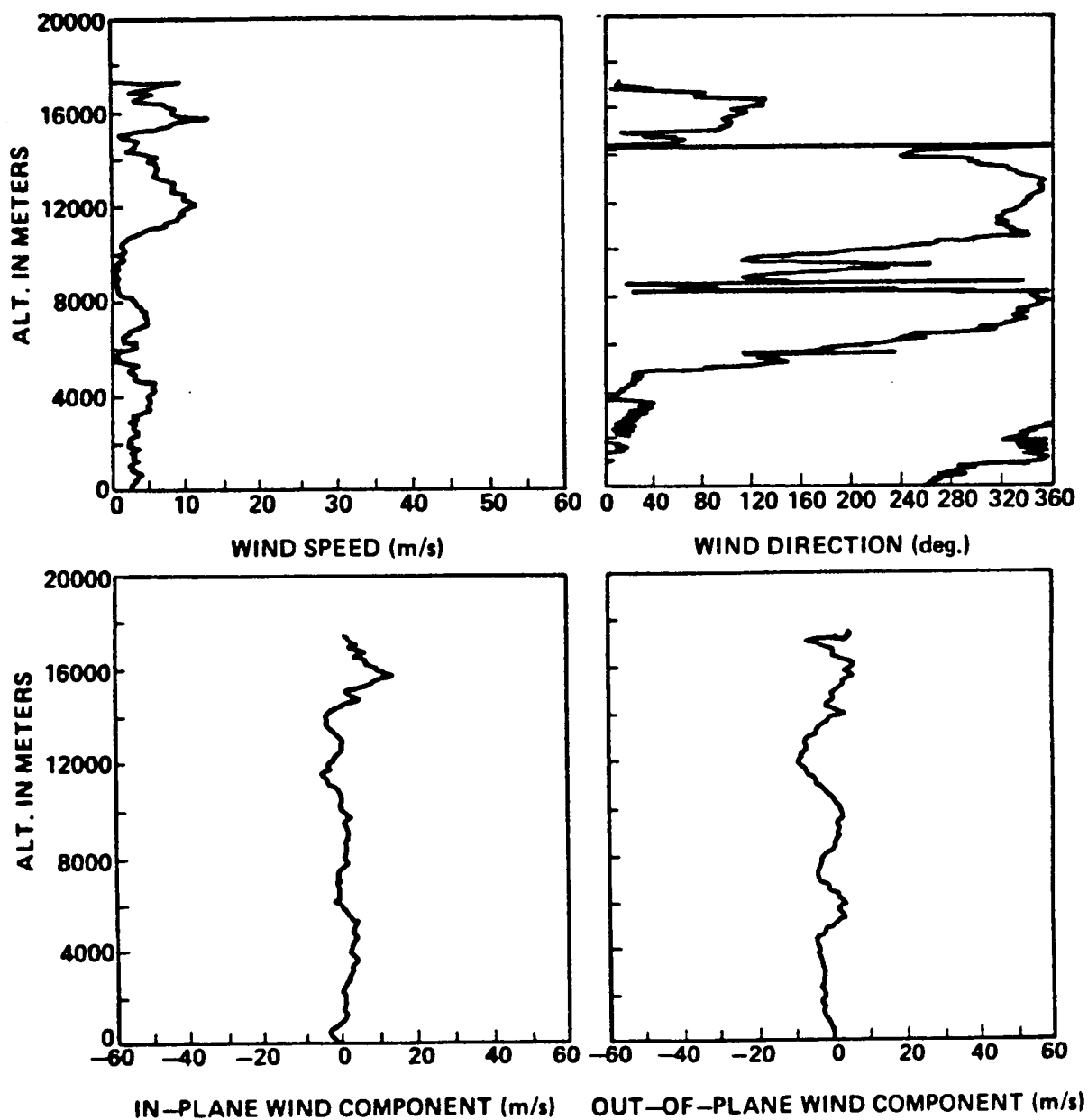
Figure A.31. STS-8 prelaunch/launch jimsphere profiles of wind speed, wind direction, in-plane and out-of-plane wind components, 2300 GMT August 29, 1983.
