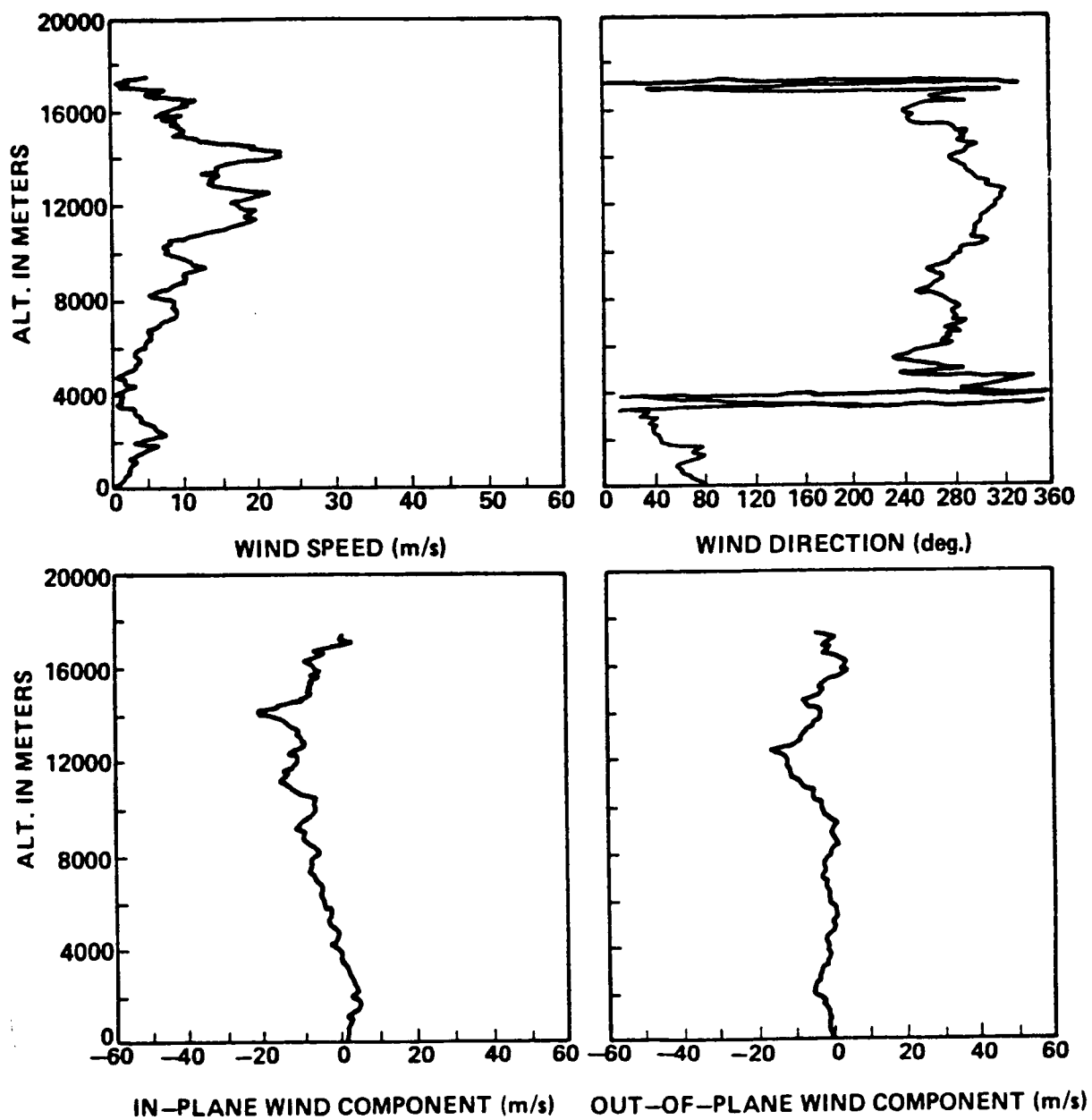
Figure A.29. STS-7 prelaunch/launch jimsphere profiles of wind speed, wind direction, in-plane and out-of-plane wind components, 1150 GMT June 18, 1983.
