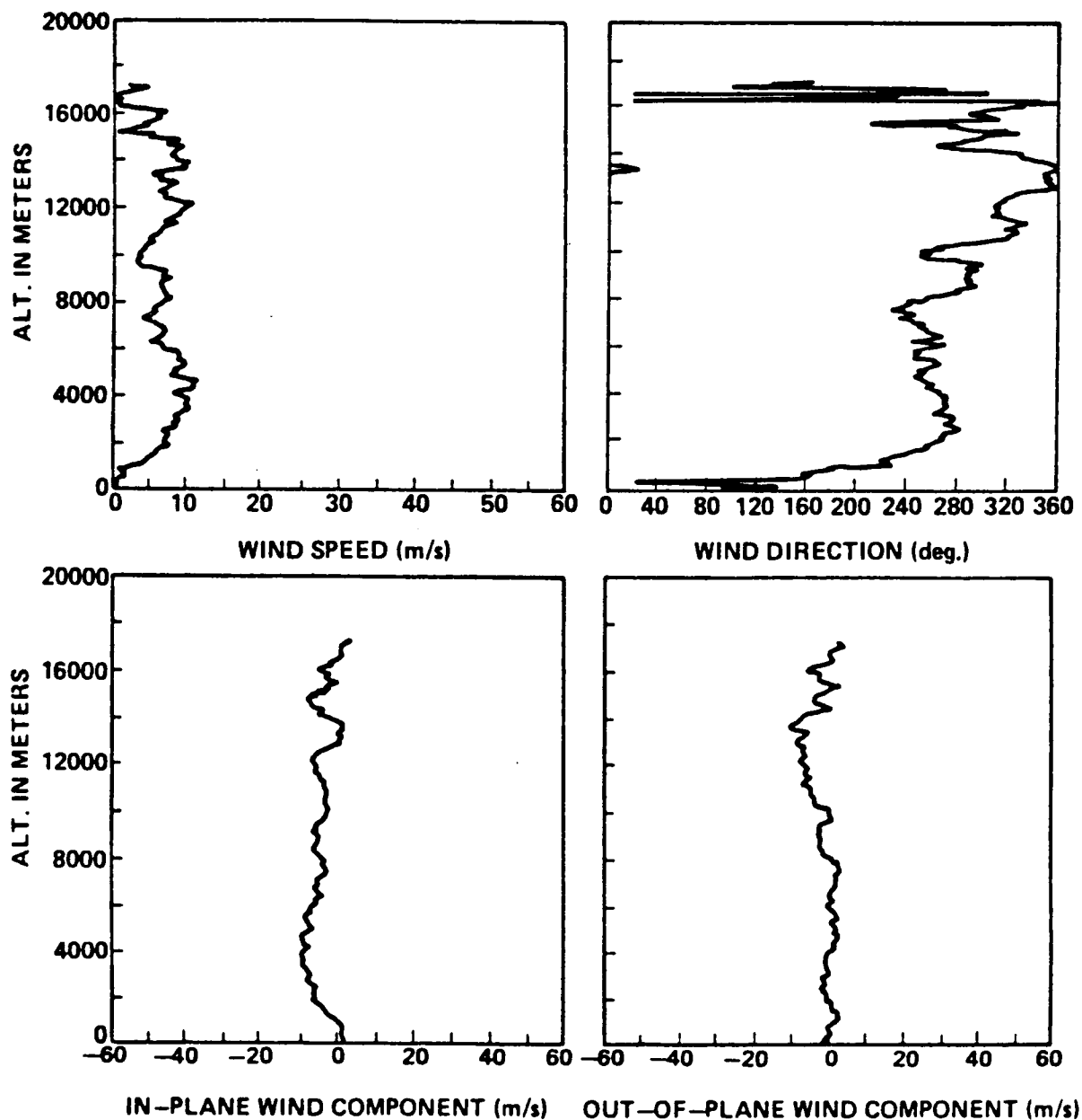
Figure A.10. STS-4 prelaunch/launch jimsphere profiles of wind speed, wind direction, in-plane and out-of-plane wind components, 0100 GMT June 27, 1982.
