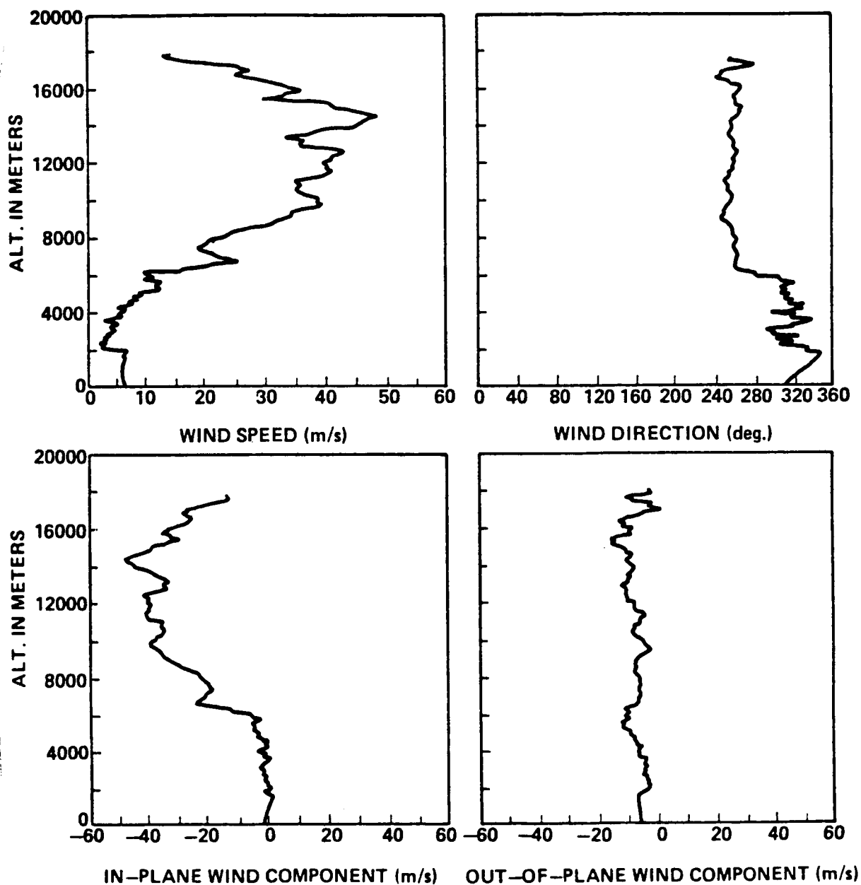
Figure 3.3. STS-2 prelaunch/launch jimpshere profiles of wind speed, wind direction, in-plane and out-of-plane wind components, 0200 GMT November 12, 1981.
