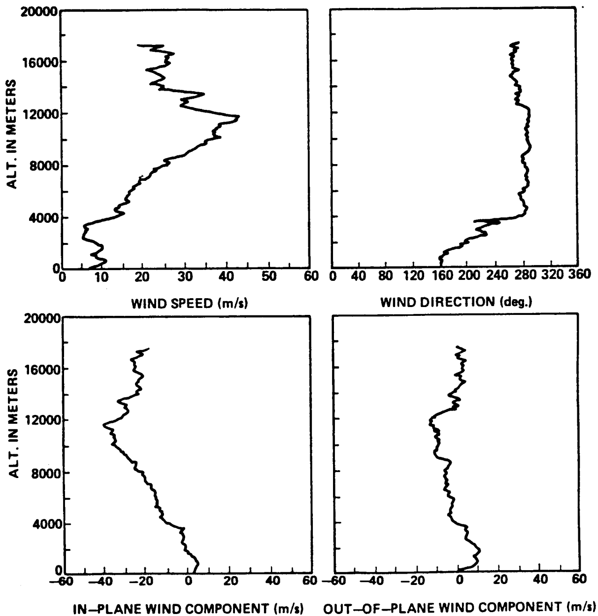
Figure A.40. STS-11 prelaunch/launch jimsphere profiles of wind speed, wind direction, in-plane and out-of-plane wind components, 1320 GMT February 3, 1984.
