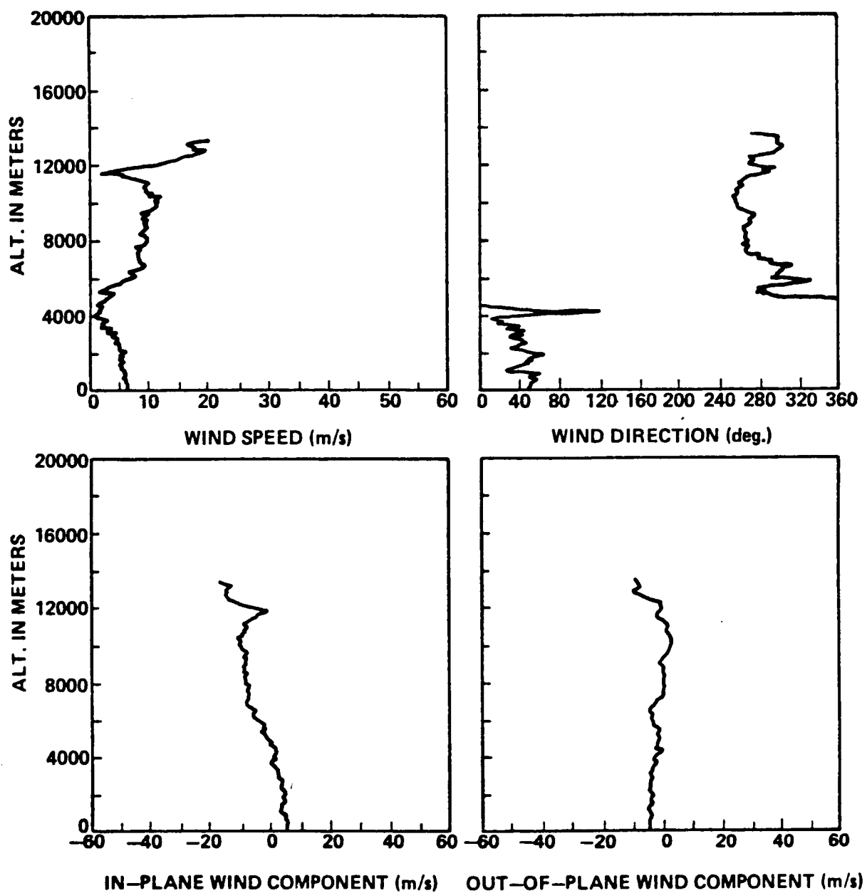
Figure A.26. STS-7 prelaunch/launch jimsphere profiles of wind speed, wind direction, in-plane and out-of-plane wind components, 2333 GMT June 17, 1983.
