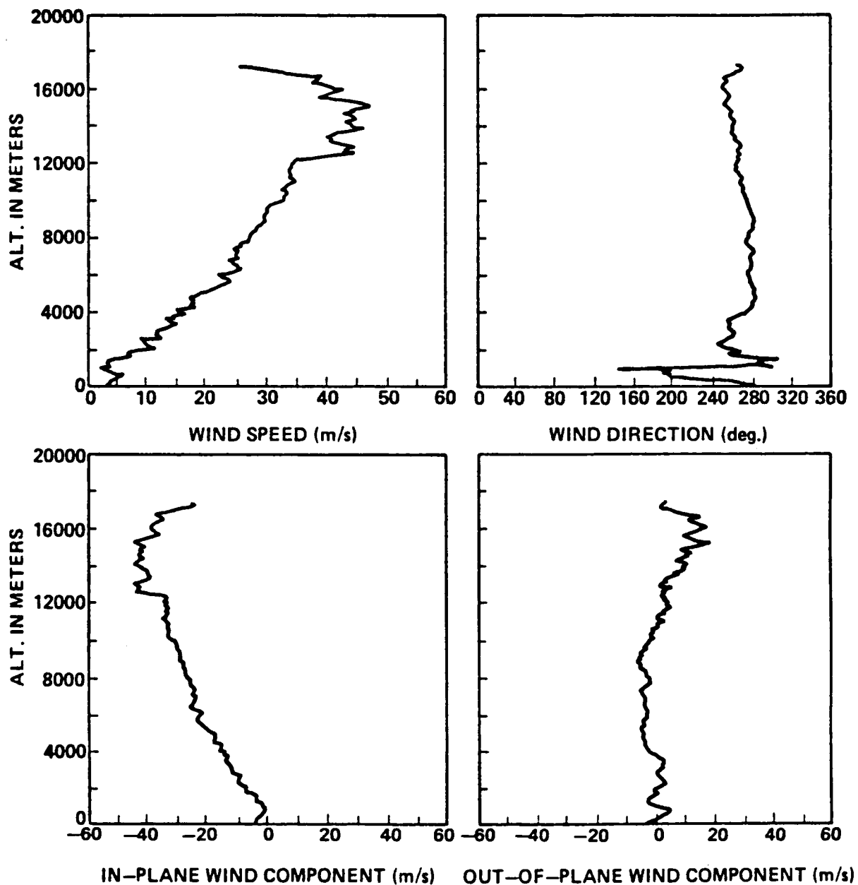
Figure A.20. STS-6 prelaunch/launch jimsphere profiles of wind speed, wind direction, in-plane and out-of-plane wind components, 0430 GMT April 4, 1983.
