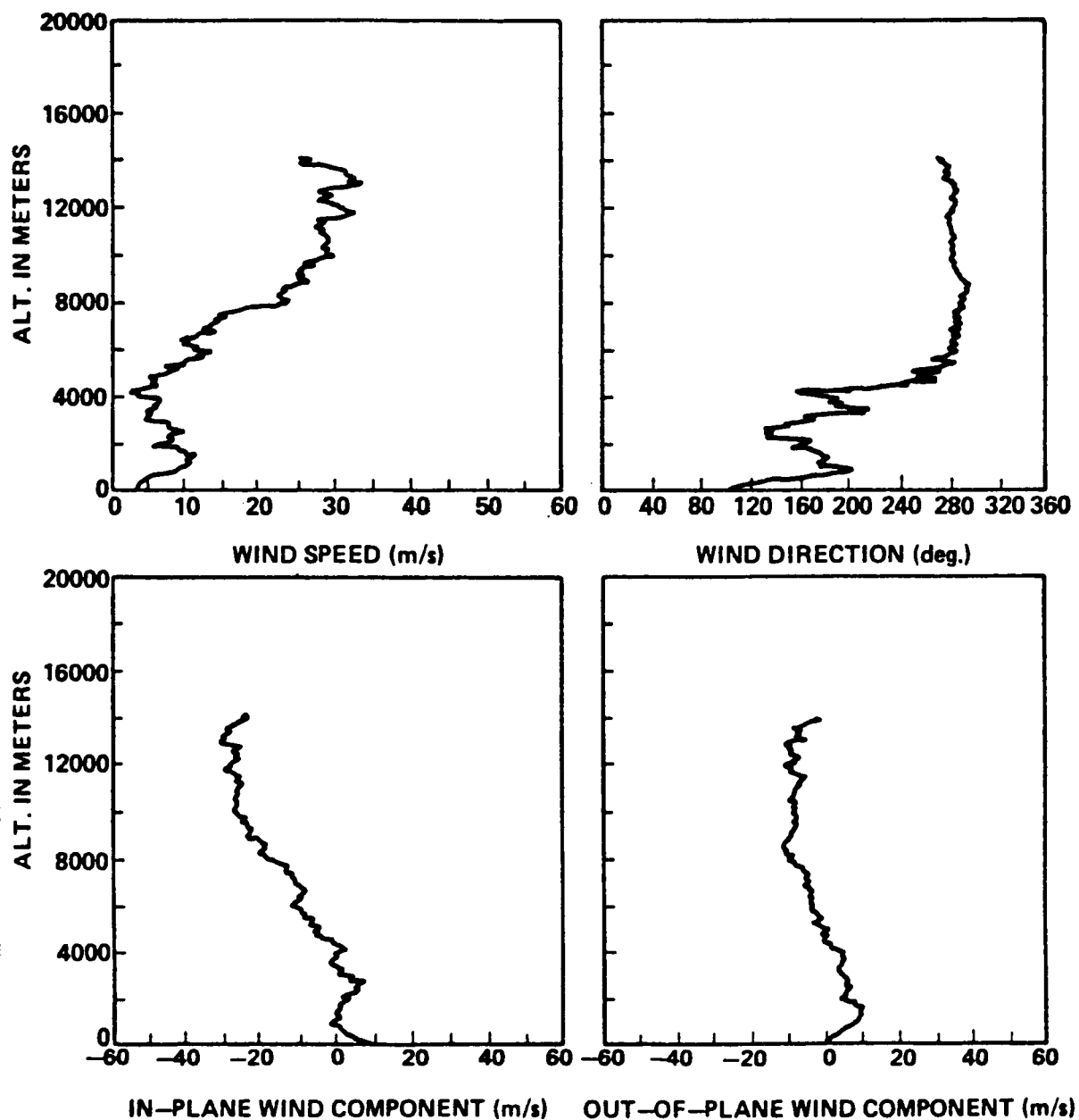
Figure A.38. STS-11 prelaunch/launch jimsphere profiles of wind speed, wind direction, in-plane and out-of-plane wind components, 0545 GMT February 3, 1984.
