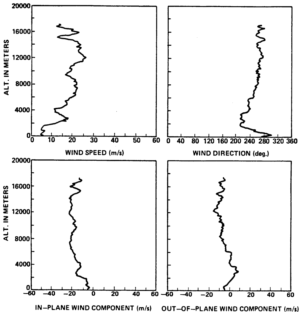
Figure A.6. STS-3 prelaunch/launch jimsphere profiles of wind speed, wind direction, in-plane and out-of-plane wind components, 0430 GMT March 22, 1982.
