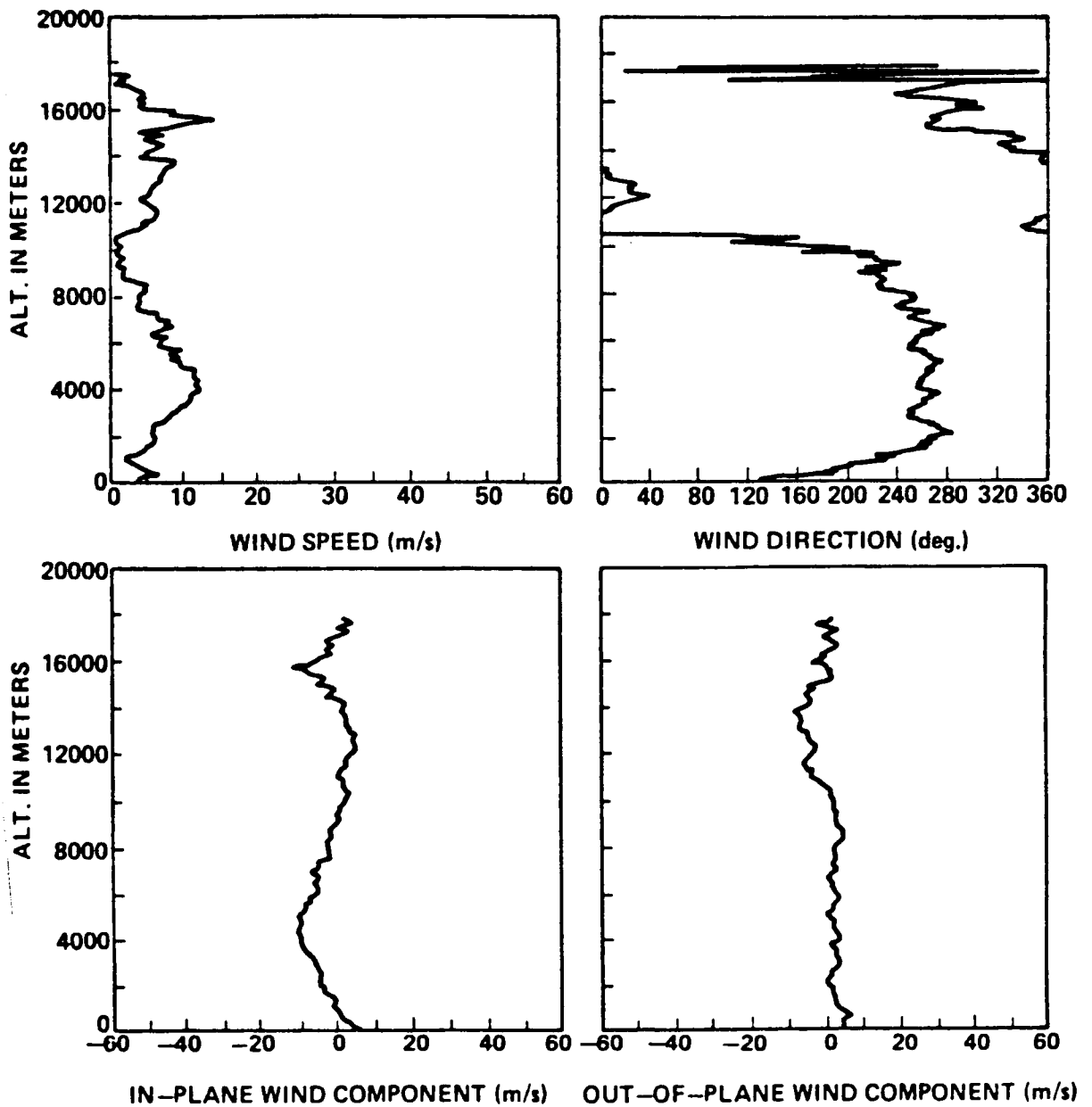
Figure A.12. STS-4 prelaunch/launch jimsphere profiles of wind speed, wind direction, in-plane and out-of-plane wind components, 0745 GMT June 27, 1982.
