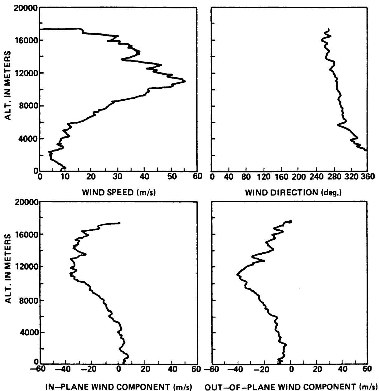
Figure A.4. STS-2 prelaunch/launch jimsphere profiles of wind speed, wind direction, in-plane and out-of-plane wind components, 1558 GMT November 12, 1981.
