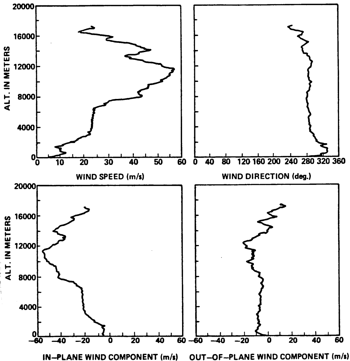
Figure A.43. STS-13 prelaunch/launch jimsphere profiles of wind speed, wind direction, in-plane and out-of-plane wind components, 1028 GMT April 6, 1984.
