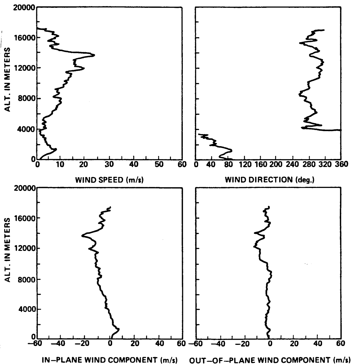
Figure A.28. STS-7 prelaunch/launch jimsphere profiles of wind speed, wind direction, in-plane and out-of-plane wind components, 0803 GMT June 18, 1983.
