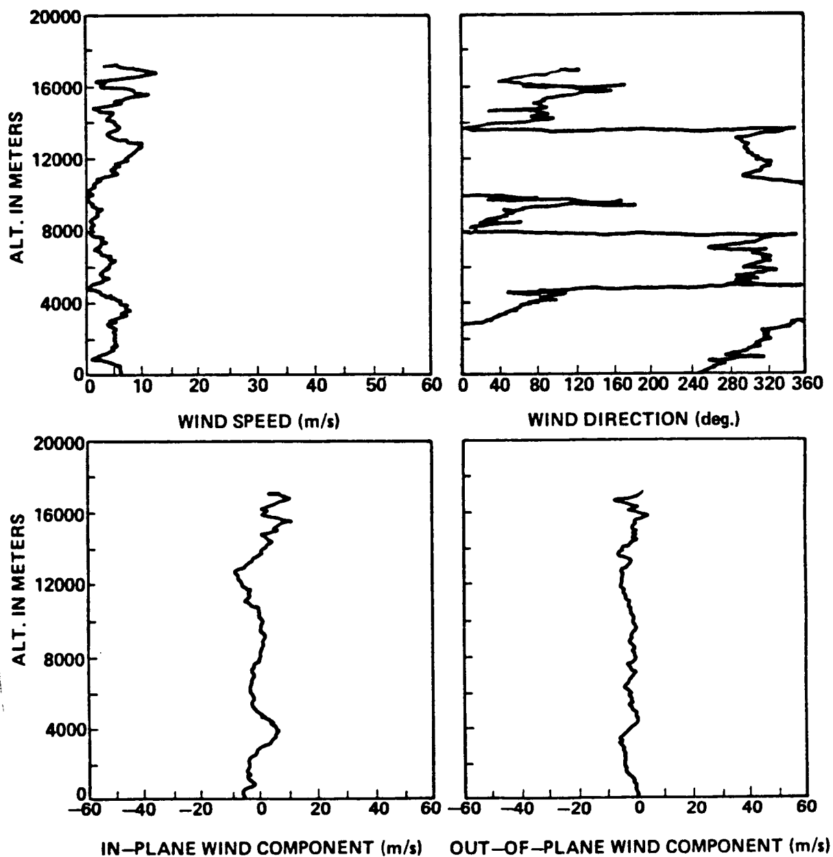
Figure A.30. STS-8 prelaunch/launch jimsphere profiles of wind speed, wind direction, in-plane and out-of-plane wind components, 1750 GMT August 29, 1983.
