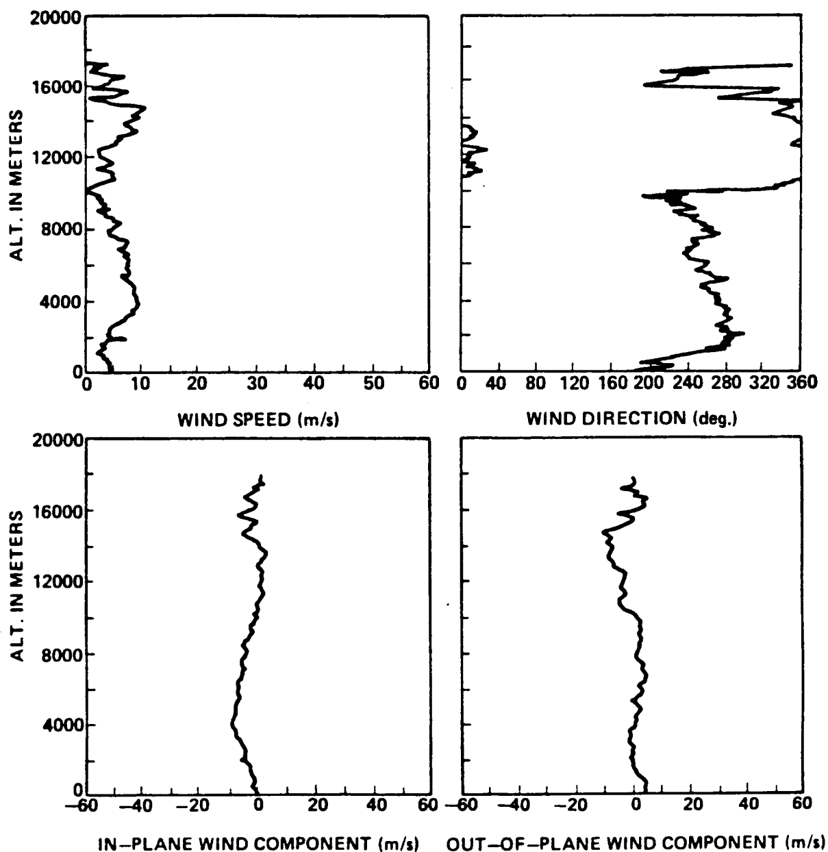
Figure A.13. STS-4 prelaunch/launch jimsphere profiles of wind speed, wind direction, in-plane and out-of-plane wind components, 1130 GMT June 27, 1982.
