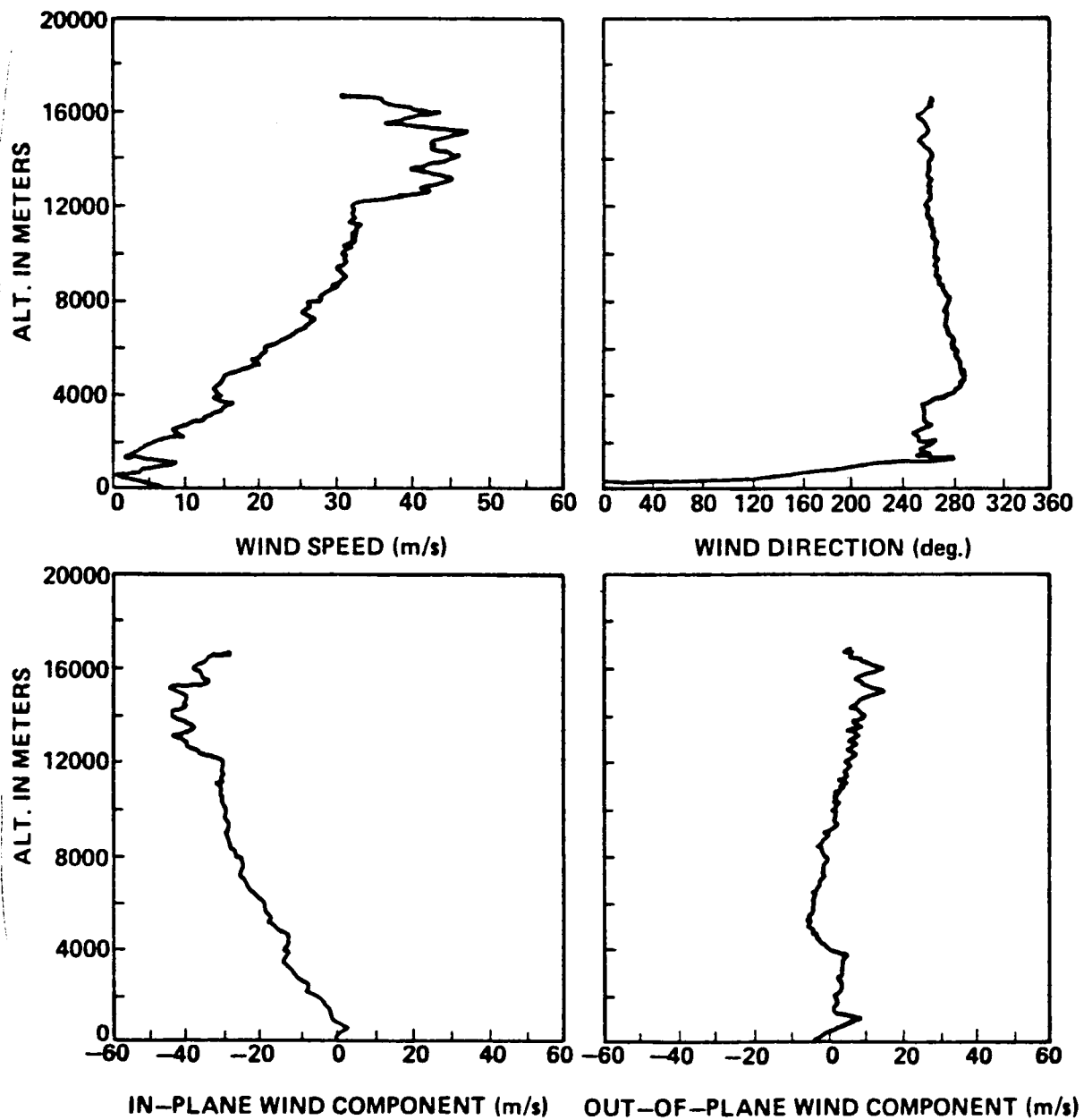
Figure A.21. STS-6 prelaunch/launch jimsphere profiles of wind speed, wind direction, in-plane and out-of-plane wind components, 0630 GMT April 4, 1983.
