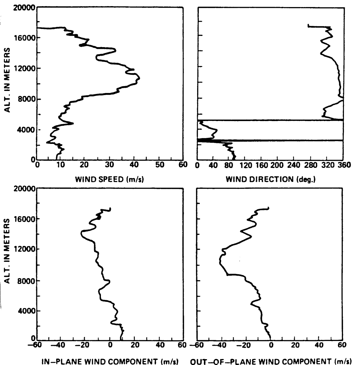
Figure A.17. STS-5 prelaunch/launch jimsphere profiles of wind speed, wind direction, in-plane and out-of-plane wind components, 0504 GMT November 11, 1982.
