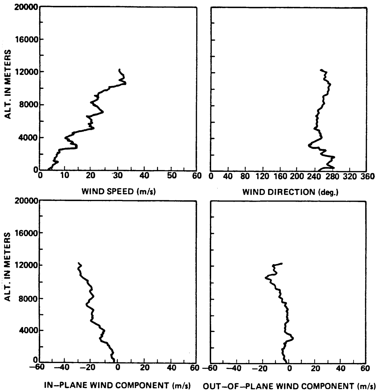
Figure A.9. STS-3 prelaunch/launch jimsphere profiles of wind speed, wind direction, in-plane and out-of-plane wind components, 1417 GMT March 22, 1982.
