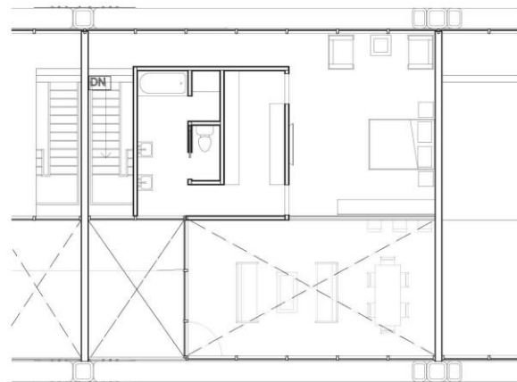
Plan of Sleeping Loft
