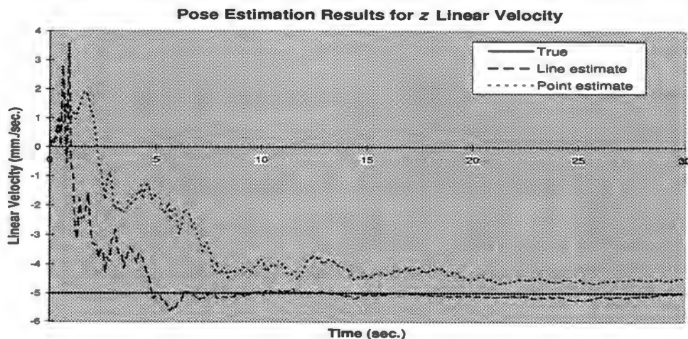
Fig. 5.12. v_z translation velocity pose estimate simulation results with a four-point target showing constant linear velocity over time for the line method, the comparison point method, and the true v_z velocity value of -5 mm./sec. from a sample run. The line method estimates are seen to settle faster to the true value and with less error than the point method.
