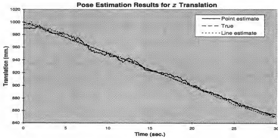
Fig. 5.5. t_z translation pose estimate simulation results with a four-point target showing linear translation over time for the line method, the comparison point method, and the true z translation value from a sample run. More deviation from the true value is seen for this axis than in x and y although the errors are not large.
