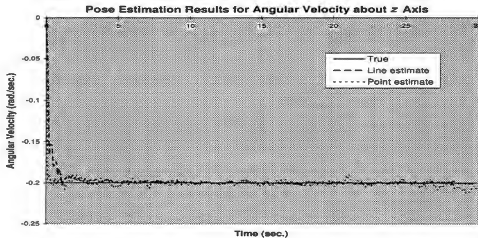
Fig. 5.15. \omega_z angular velocity pose estimate simulation results with a four-point target showing constant angular velocity over time for the line method, the comparison point method, and the true \omega_z angular velocity value of -0.2 rad./sec. from a sample run. Both methods are seen to give good estimation results for this rotation angle after the initial settling time.
