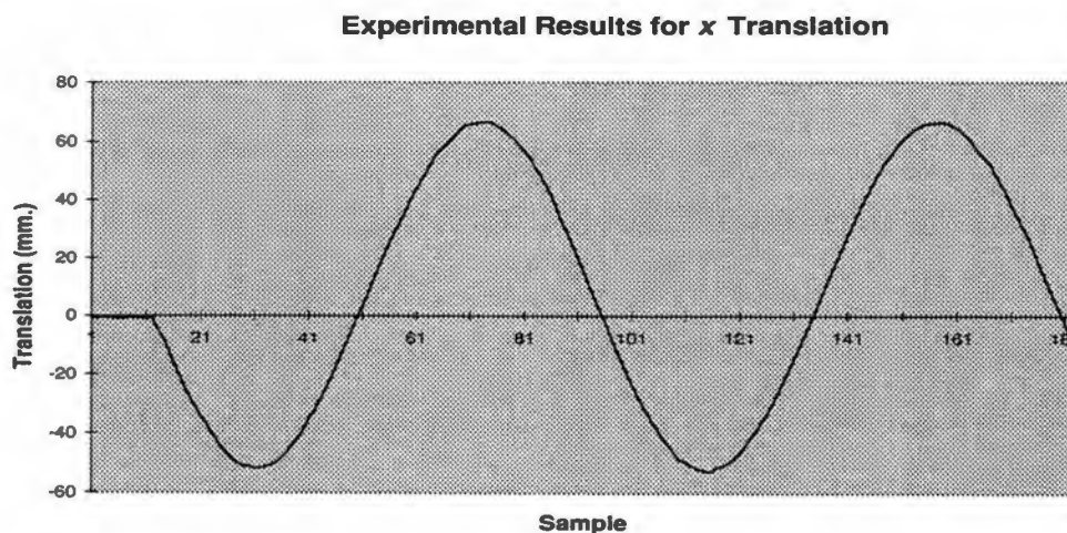
Fig. 5.50. t_x translation pose estimate from experimental testing for constant target motion about the z axis. The estimate shows a sinusoidal variation corresponding to the true x variation of the target. Note the step response at the beginning of the target motion.
