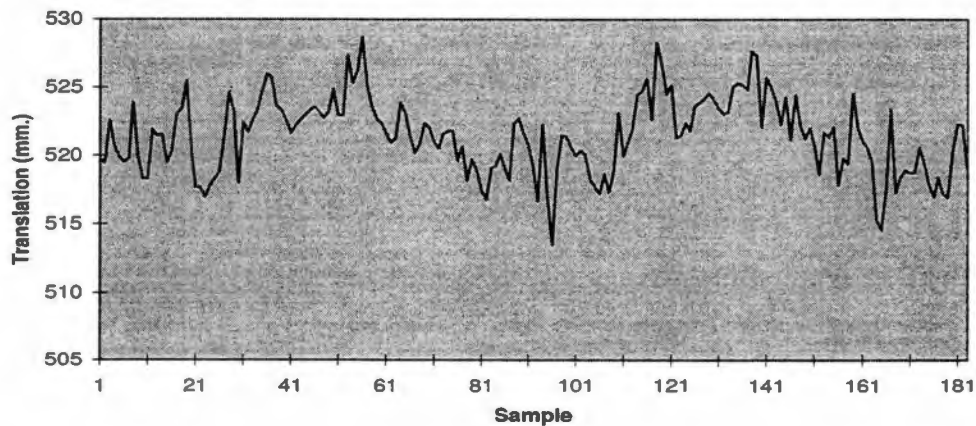
Fig. 5.52. t_z translation pose estimate from experimental testing for constant target motion about z axis. The estimate shows a noisy variation about a mean z value with a small sinusoidal component. The true target z value is nominally constant.
