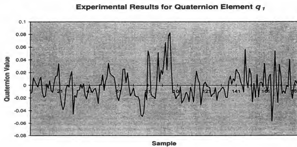
Fig. 5.54. q_1 quaternion pose estimate from experimental testing for constant target motion about the z axis. The estimate shows a relatively small noisy variation about zero in comparison to a true q_1 constant value of zero.
