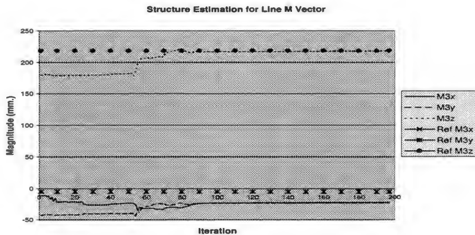
Fig. 5.71. Structure estimate of the three \vec{m} line vector components for line four with motion along the z axis. The true structure values are also shown for comparison. The x and z components have relatively small errors while a constant offset error is present for the y component.
