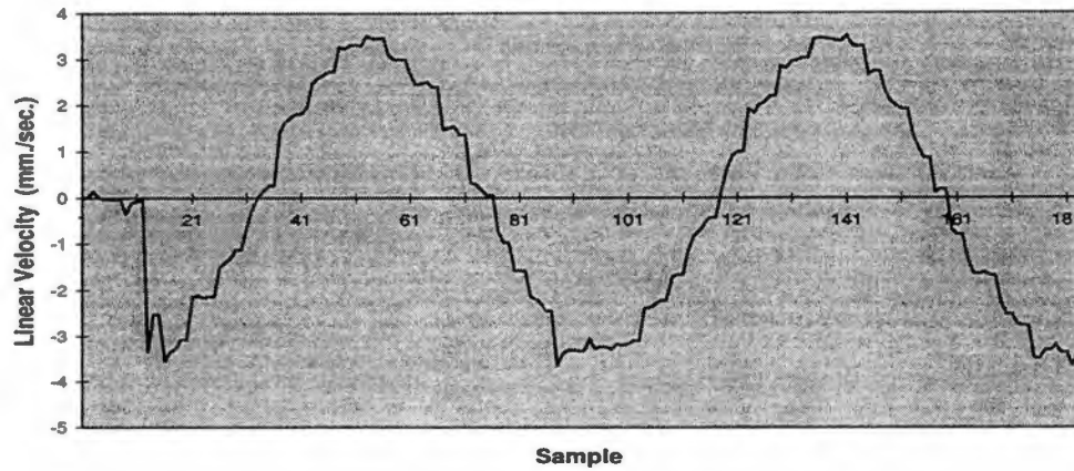
Fig. 5.57. v_x translation velocity pose estimate from experimental testing for constant target motion about the z axis. The estimate shows a noisy sinusoidal variation compared to the true x sinusoidal velocity variation of the target. Note the step response at the beginning of the target motion.
