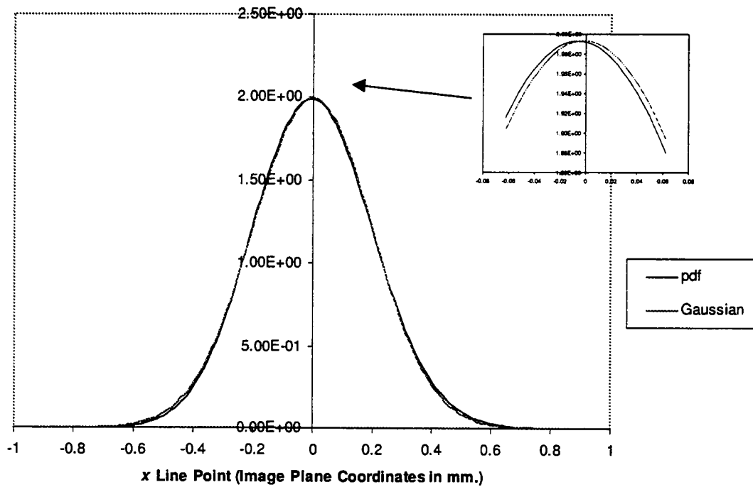
Fig. 4.5. Probability density function of x_{lp} for 1.25 mm. length upward diagonal line at x_s=12.5 mm., y_s=12.5 mm., point noise 0.02 mm. standard deviation. A best-fit Gaussian pdf is also plotted, but the differences are seen to be small.
