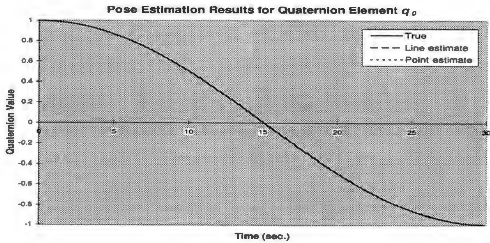
Fig. 5.6. q_0 quaternion pose estimate simulation results with a four-point target showing constant rotation over time for the line method, the comparison point method, and the true q_0 quaternion value from a sample run. Both methods are seen to give good estimation results for this state variable.
