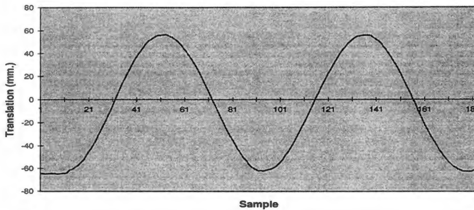
Fig. 5.51. t_y translation pose estimate from experimental testing for constant target motion about the z axis. The estimate shows a sinusoidal variation corresponding to the true y variation of the target. Note the step response at the beginning of the target motion.
