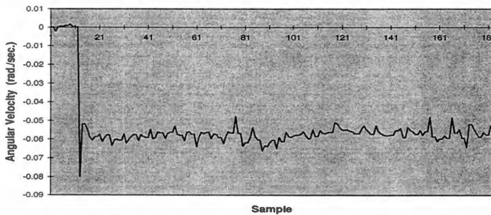
Fig. 5.62. \omega_z angular velocity pose estimate from experimental testing for constant target motion about the z axis. The estimate shows a noisy variation about a mean \omega_z velocity value of -0.06 rad./sec. The true target \omega_z velocity value is nominally constant at -0.06 rad./sec.
