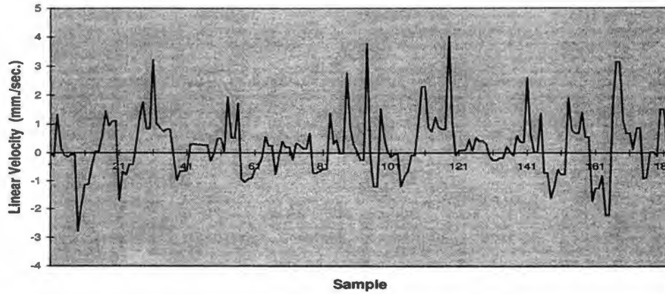
Fig. 5.59. v_z translation velocity pose estimate from experimental testing for constant target motion about z axis. The estimate shows a noisy variation about a mean z velocity value of zero. The true target v_z velocity value is nominally zero.
