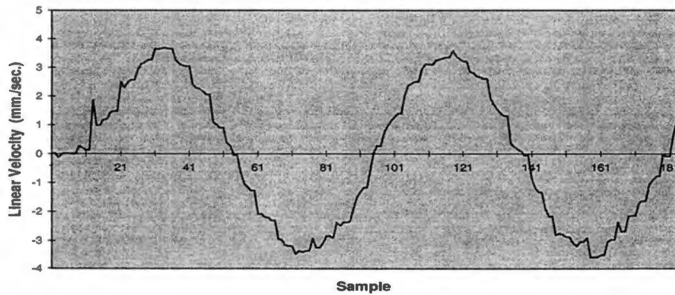
Fig. 5.58. v_y translation velocity pose estimate from experimental testing for constant target motion about the z axis. The estimate shows a noisy sinusoidal variation compared to the true y sinusoidal velocity variation of the target. Note the step response at the beginning of the target motion.
