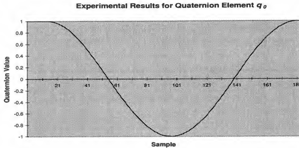
Fig. 5.53. q_0 quaternion pose estimate from experimental testing for constant target motion about the z axis. The estimate shows a full 360 degree sinusoidal variation corresponding to the true q_0 variation of the target as it moves through two complete revolutions.
