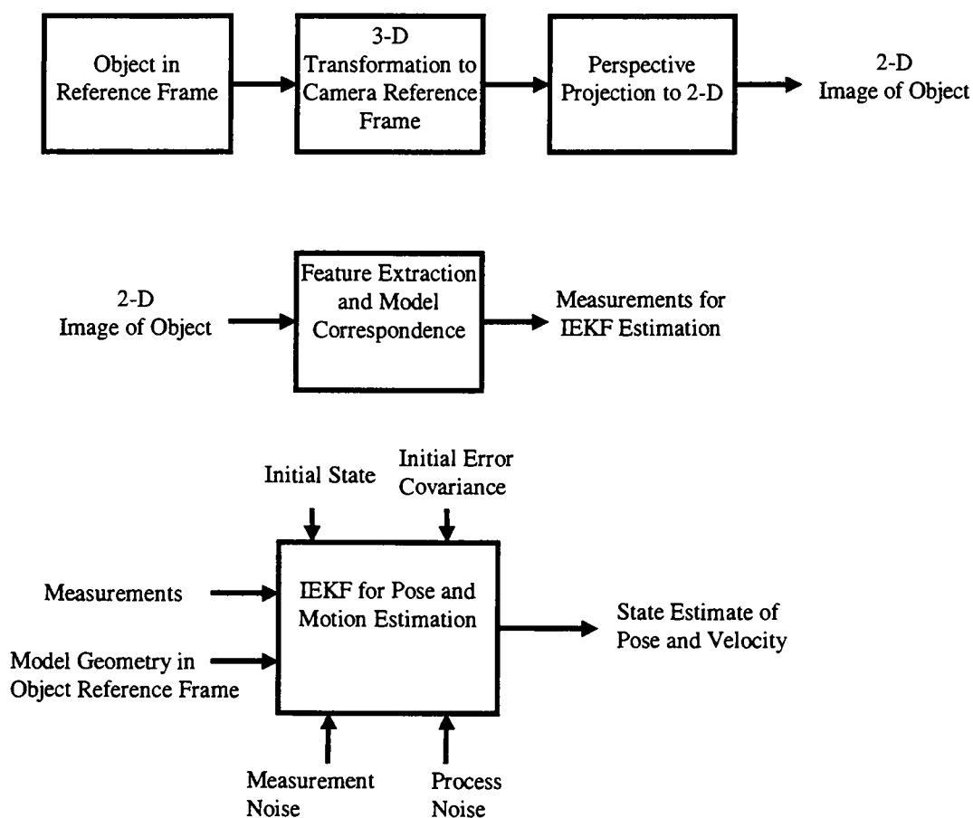
Fig. 5.1. Functional block diagram of the estimation problem showing the operations involved in the pose estimation method from optical imaging to state estimate produced by the iterated extended Kalman filter.
