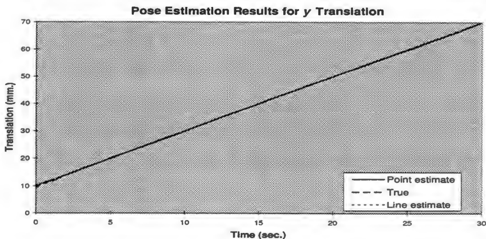
Fig. 5.4. t_y translation pose estimate simulation results with a four-point target showing linear translation over time for the line method, the comparison point method, and the true y translation value from a sample run. Both methods are seen to give good estimation results for this axis.
