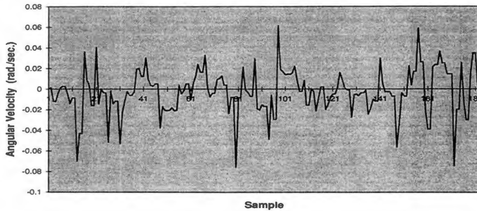
Fig. 5.61. \omega_y angular velocity pose estimate from experimental testing for constant target motion about the z axis. The estimate shows a noisy variation about a mean \omega_y velocity value of zero. The true target \omega_y velocity value is nominally zero.
