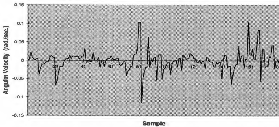
Fig. 5.60. \omega_x angular velocity pose estimate from experimental testing for constant target motion about the z axis. The estimate shows a noisy variation about a mean \omega_x velocity value of zero. The true target \omega_x velocity value is nominally zero.
